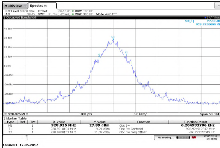
Figure 7.3.2-9: 928.925 MHz – C&amp;I (Half Baud) Mode
