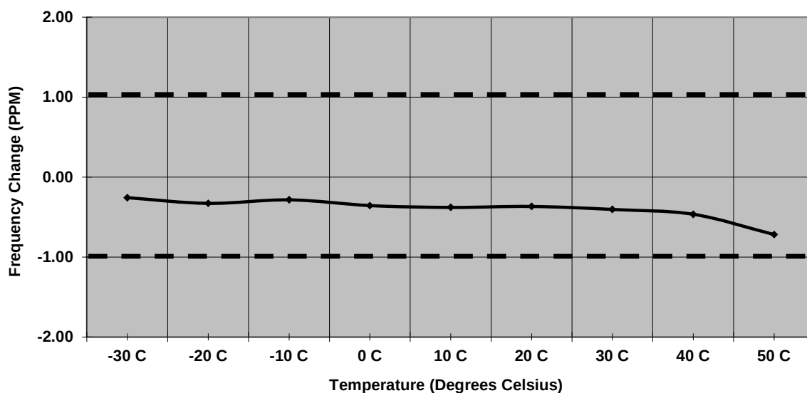
Figure 7.6.2-8: Frequency Stability – 959.925 MHz – KDS/MEA
