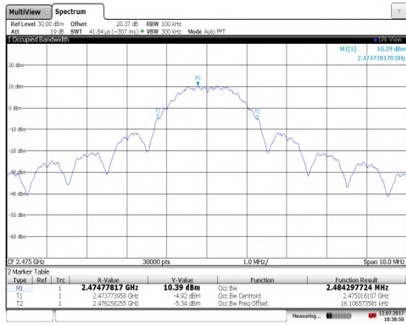
Figure 7.3.2-6: 99% Bandwidth High Adj. Channel
