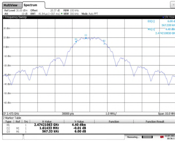
Figure 7.3.2-5: 6dB Bandwidth High adj. Channel
