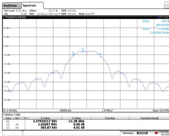
Figure 7.3.2-7: 6dB Bandwidth High Channel
