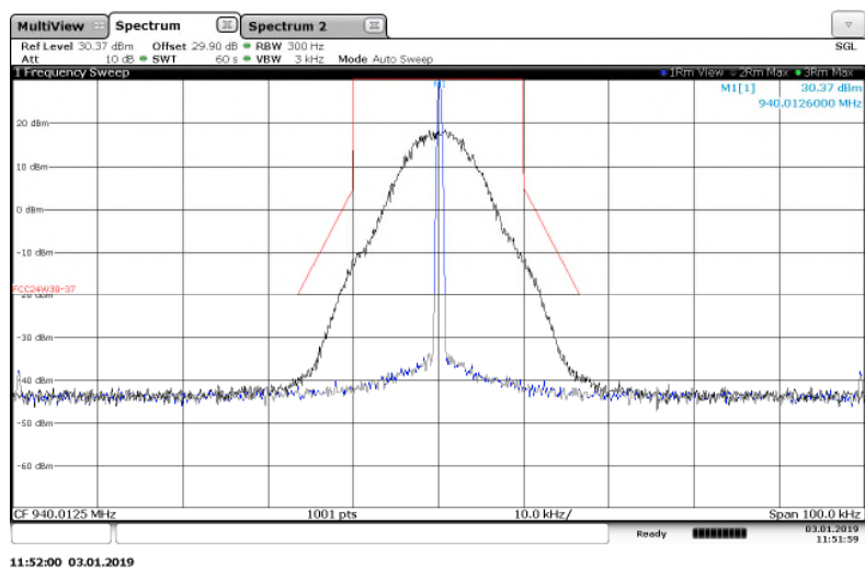
Figure 7.2.2-10: 940.0125 MHz – 25 kHz Channel Spacing – m4Pass20k Mode
