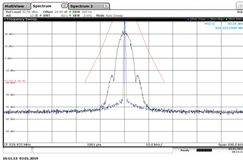
Figure 7.2.2-14: 928.925 MHz -- 25 kHz Channel Spacing – 2FSK (Half Baud) Mode
