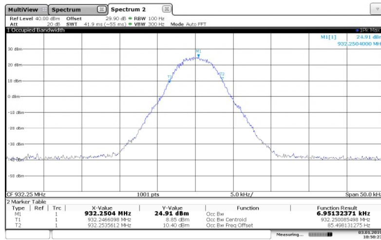
Figure 7.3.2-21: 932.25 MHz -- 4FSK(Half Baud) Mode
