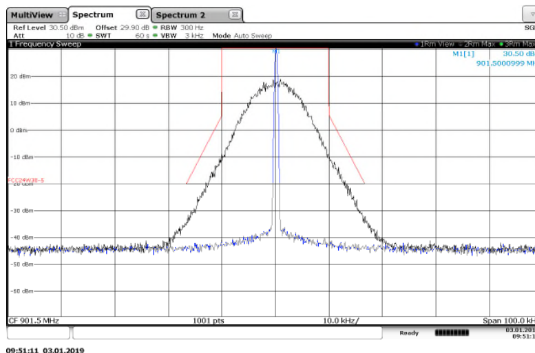
Figure 7.2.2-2: 901.5 MHz – 25 kHz Channel Spacing – 4SFSK Mode
