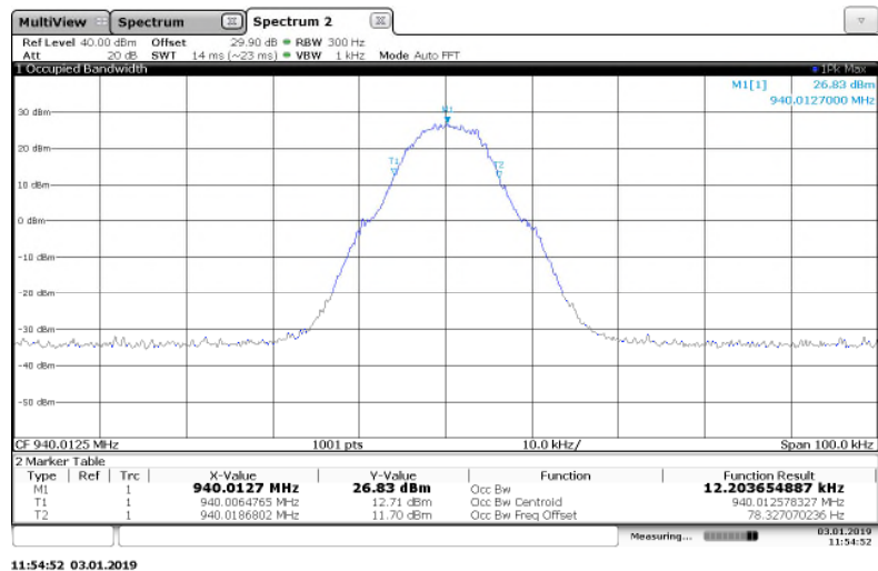
Figure 7.3.2-10: 940.0125 MHz – m4Pass 20k Mode
