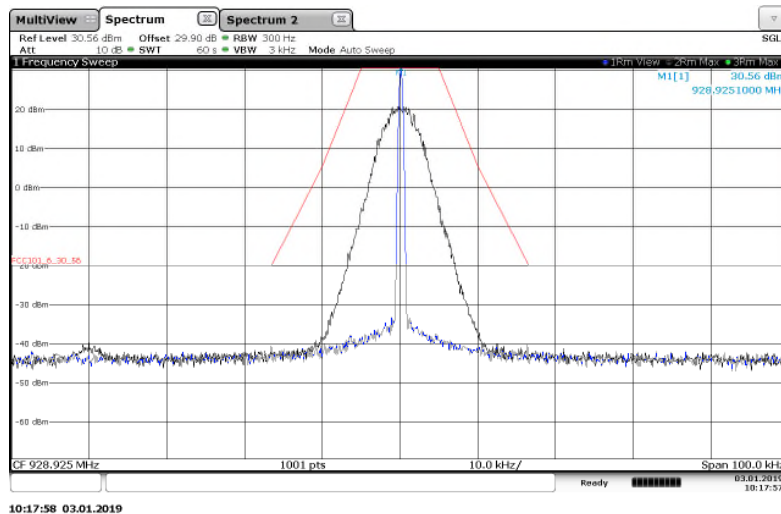
Figure 7.2.2-16: 928.925 MHz -- 25 kHz Channel Spacing – 8FSK (Half Baud) Mode
