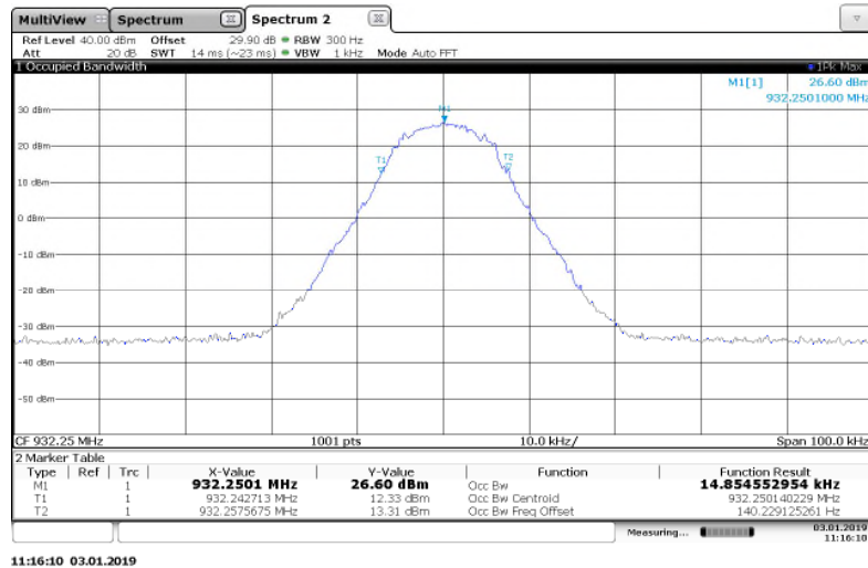
Figure 7.3.2-19: 932.25 MHz – 8FSK Mode
