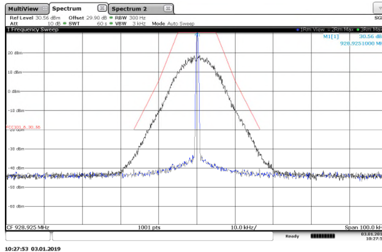
Figure 7.2.2-12: 928.925 MHz – 25 kHz Channel Spacing – 4FSK Mode
