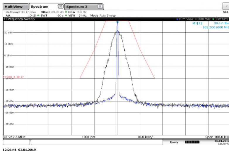
Figure 7.2.2-25: 952.5 MHz - 25 kHz Channel Spacing – m4Pass 10k Mode
