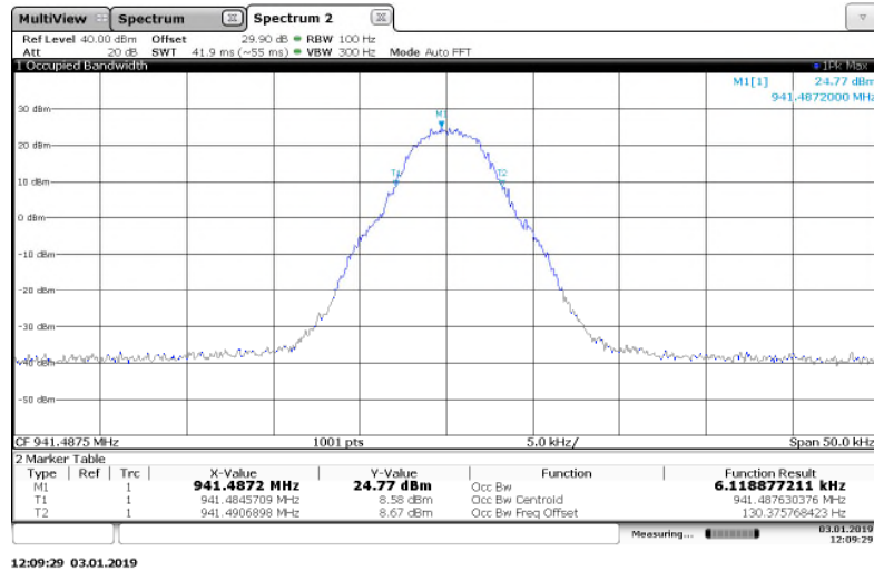
Figure 7.3.2-23: 941.4875 MHz – m4Pass 10k Mode
