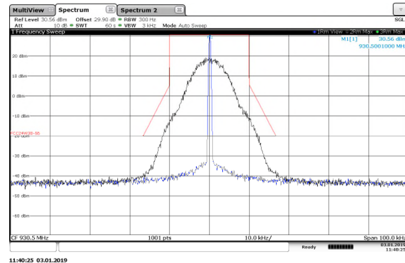
Figure 7.2.2-8: 930.5 MHz – 25 kHz Channel Spacing – m4Pass20k Mode
