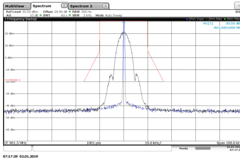
Figure 7.2.2-4: 901.5 MHz – 25 kHz Channel Spacing – 2FSK (Half Baud) Mode
