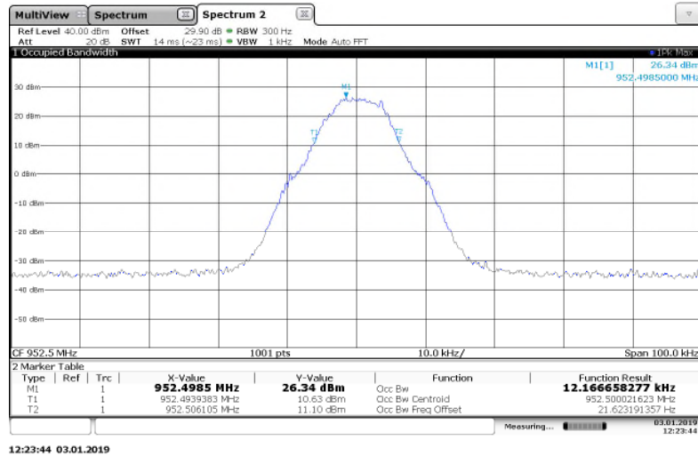
Figure 7.3.2-26: 952.5 MHz – m4Pass 20k Mode
