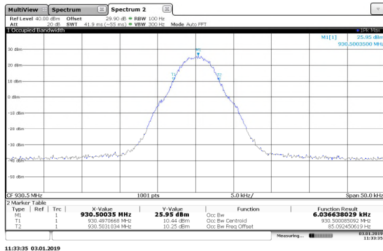
Figure 7.3.2-7: 930.5 MHz – m4Pass 10k Mode
