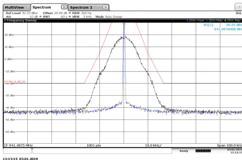
Figure 7.2.2-24: 941.4875 MHz – 25 kHz Channel Spacing – m4Pass 20k Mode
