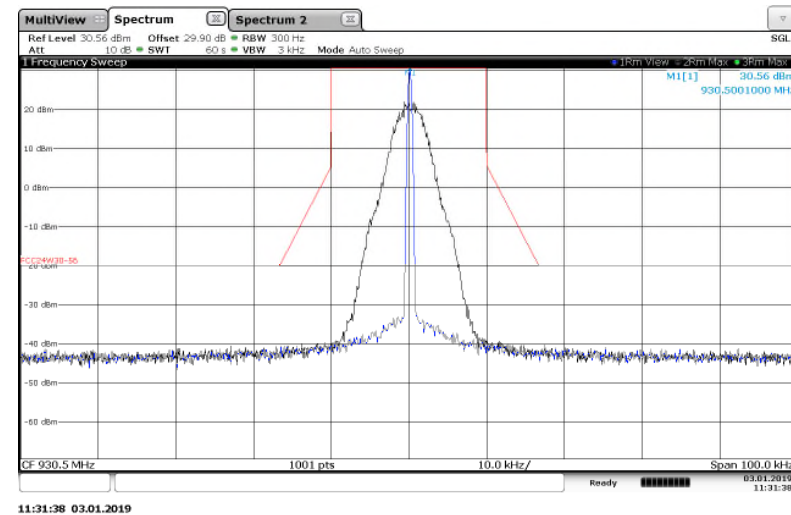
Figure 7.2.2-7: 930.5 MHz – 25 kHz Channel Spacing – m4Pass10k Mode
