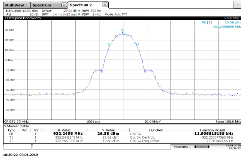
Figure 7.3.2-17: 932.25 MHz – 2FSK Mode
