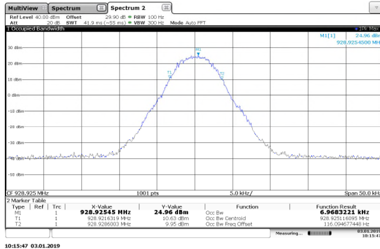
Figure 7.3.2-15: 928.925 MHz – 4FSK (Half Baud) Mode
