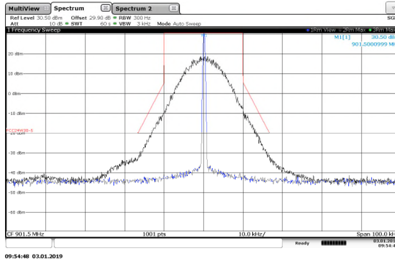
Figure 7.2.2-3: 901.5 MHz – 25 kHz Channel Spacing – 8FSK Mode
