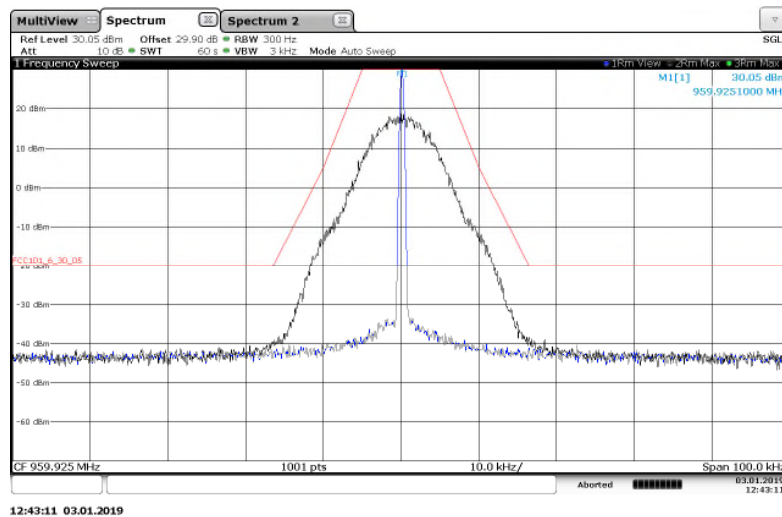
Figure 7.2.2-28: 959.925 MHz – 25 kHz Channel Spacing – m4Pass 20k Mode
