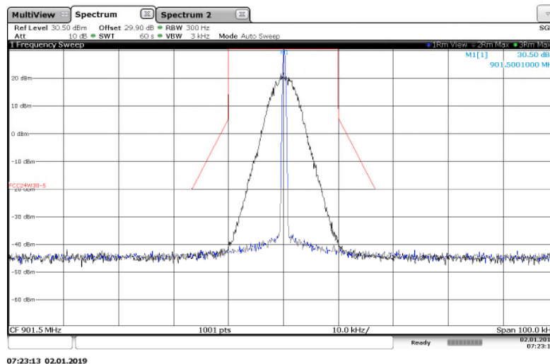
Figure 7.2.2-5: 901.5 MHz – 25 kHz Channel Spacing – 4FSK (Half Baud) Mode
