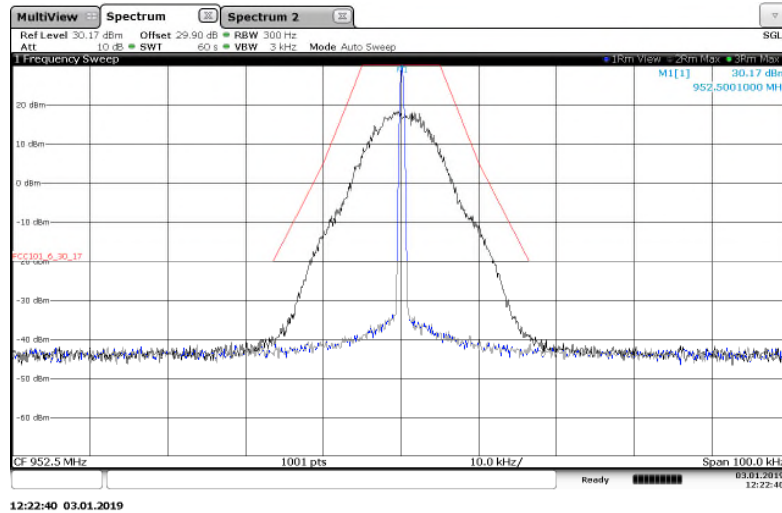
Figure 7.2.2-26: 952.5 MHz – 25 kHz Channel Spacing – m4Pass 20k Mode
