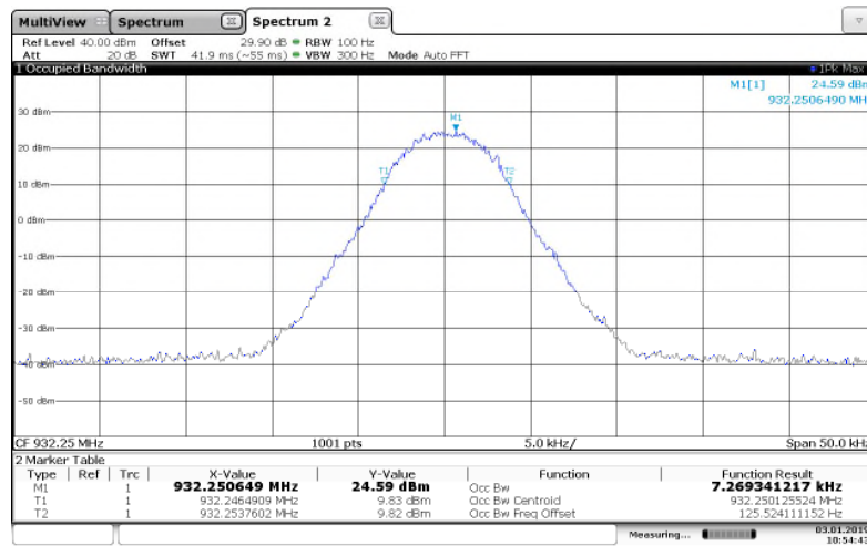
Figure 7.3.2-22: 932.25 MHz -- 8FSK(Half Baud) Mode
