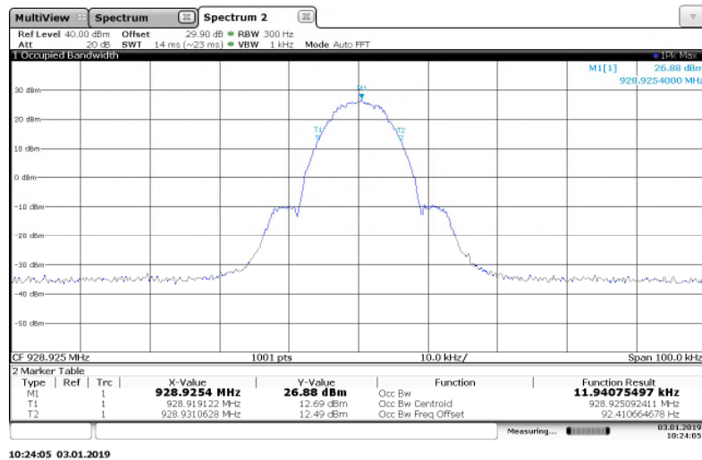
Figure 7.3.2-11: 928.925 MHz – 2FSK Mode
