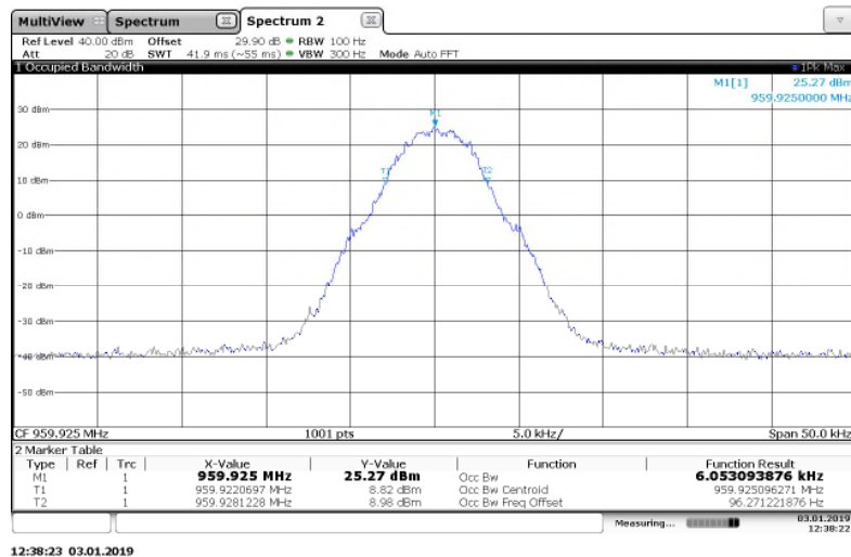
Figure 7.3.2-27: 959.925 MHz– m4Pass 10k Mode
