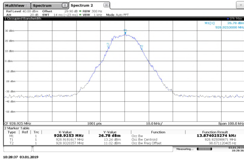
Figure 7.3.2-12: 928.925 MHz – 4FSK Mode
