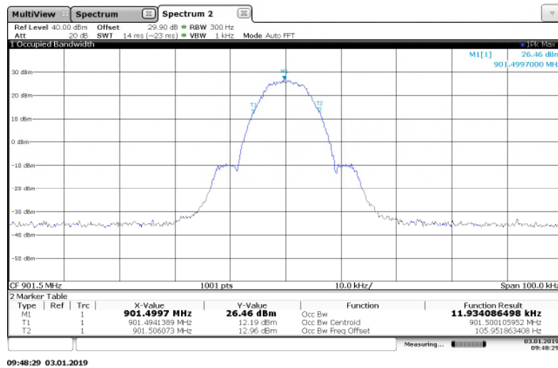
Figure 7.3.2-1: 901.5 MHz – 2FSK Mode
