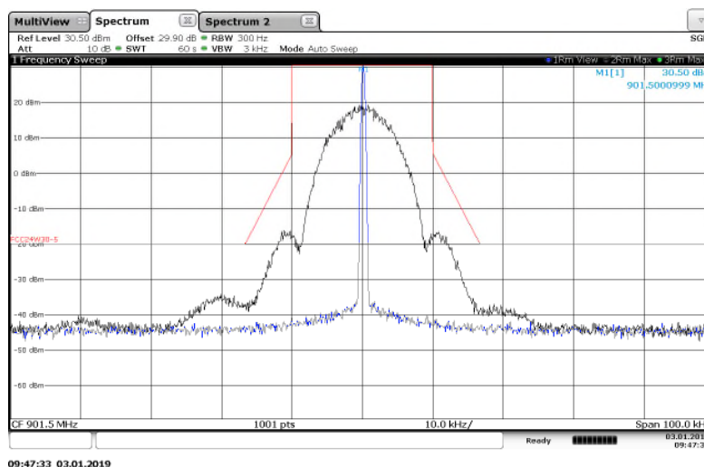
Figure 7.2.2-1: 901.5 MHz – 25 kHz Channel Spacing – 2SFSK Mode
