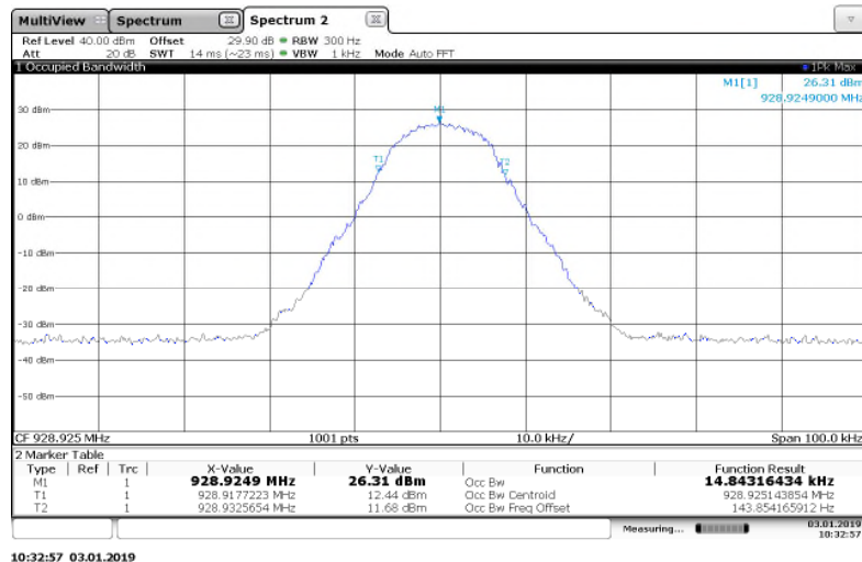
Figure 7.3.2-13: 928.925 MHz – 8FSK Mode
