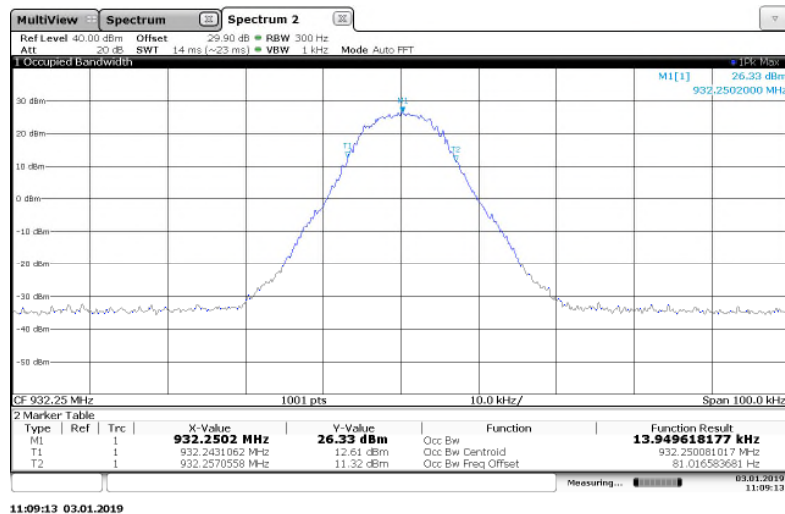
Figure 7.3.2-18: 932.25 MHz – 4FSK Mode
