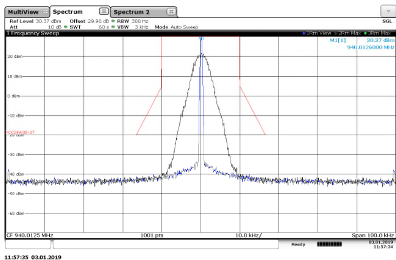
Figure 7.2.2-9: 940.0125 MHz – 25 kHz Channel Spacing – m4Pass10k Mode
