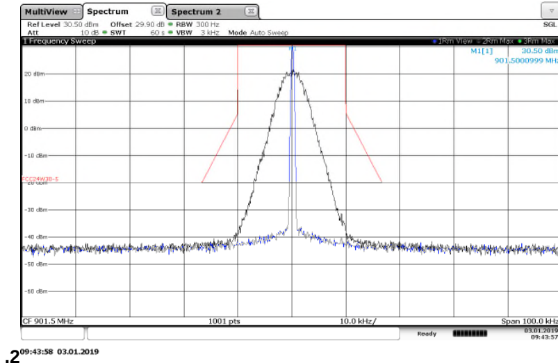
Figure 7.2.2-6: 901.5 MHz – 25 kHz Channel Spacing – 8FSK (Half Baud) Mode
