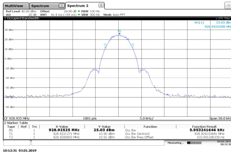
Figure 7.3.2-14: 928.925 MHz – 2FSK (Half Baud) Mode
