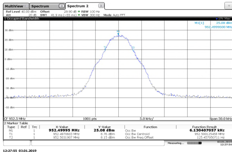
Figure 7.3.2-25: 952.5 MHz – m4Pass 10k Mode
