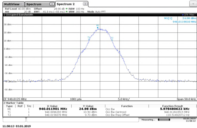
Figure 7.3.2-9: 940.0125 MHz – m4Pass 10k Mode
