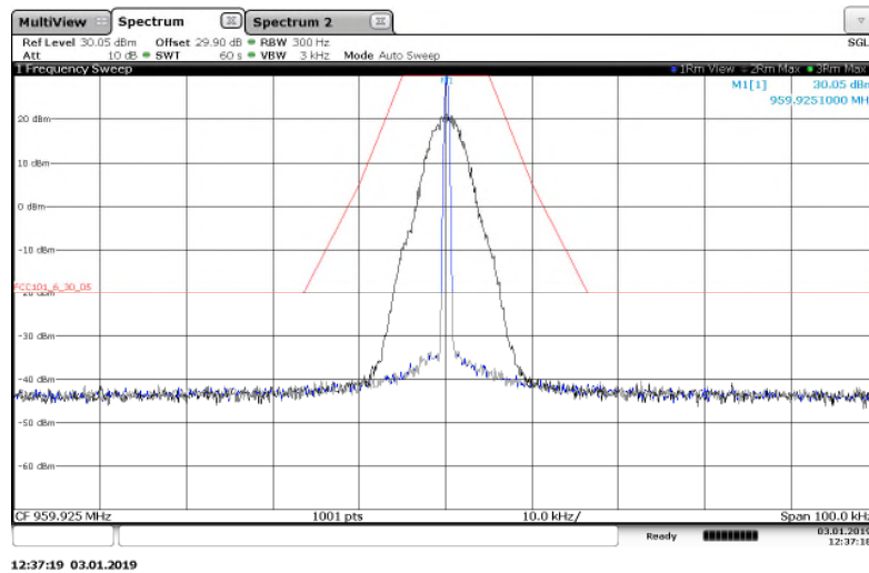
Figure 7.2.2-27: 959.925 MHz - 25 kHz Channel Spacing – m4Pass 10k Mode
