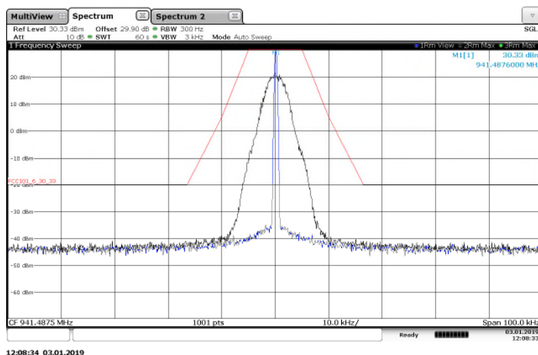
Figure 7.2.2-23: 941.4875 MHz - 25 kHz Channel Spacing – m4Pass 10k Mode
