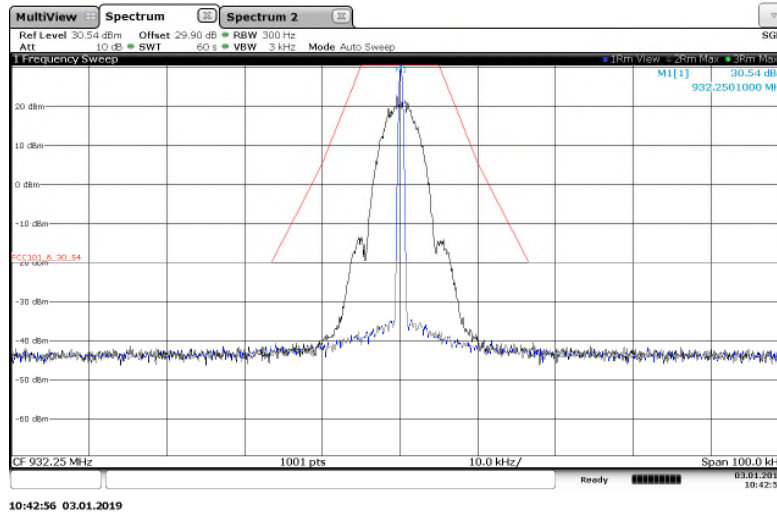
Figure 7.2.2-20: 932.25 MHz -- 25 kHz Channel Spacing – 2FSK (Half Baud) Mode
