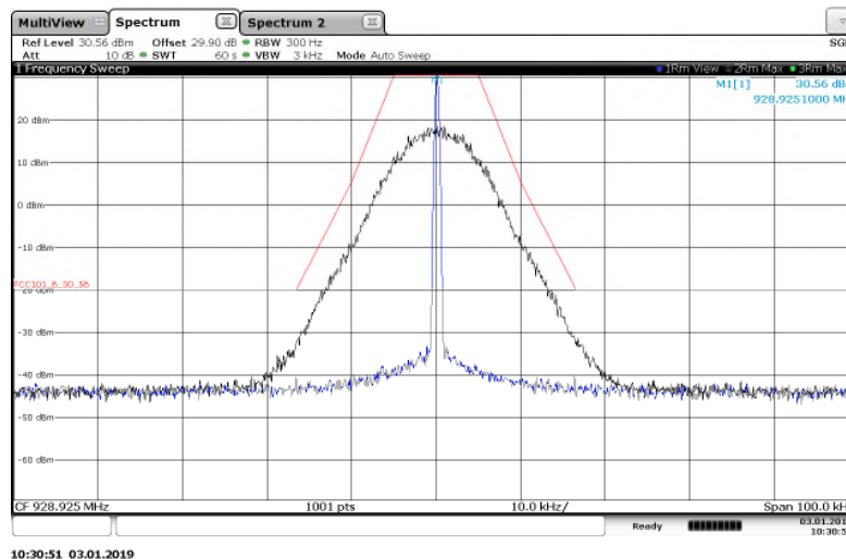
Figure 7.2.2-13: 928.925 MHz – 25 kHz Channel Spacing – 8FSK Mode
