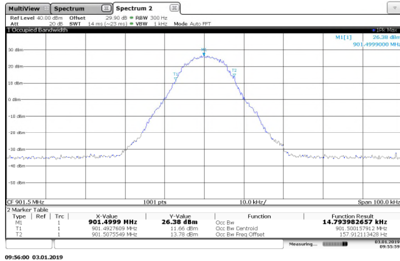
Figure 7.3.2-3: 901.5 MHz – 8FSK Mode
