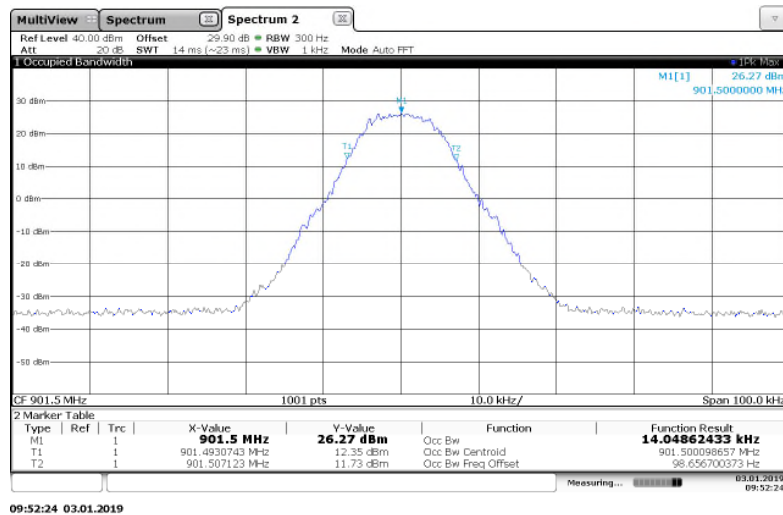
Figure 7.3.2-2: 901.5 MHz – 4FSK Mode
