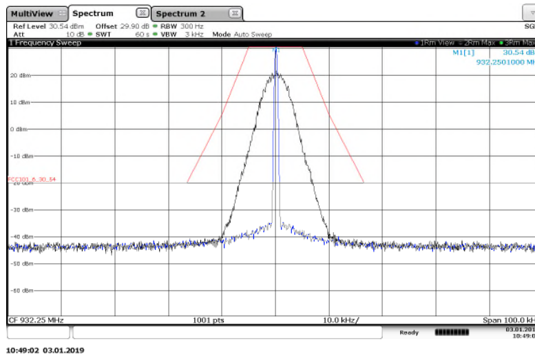
Figure 7.2.2-21: 932.25 MHz -- 25 kHz Channel Spacing – 4FSK (Half Baud) Mode
