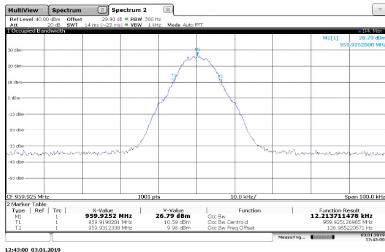
Figure 7.3.2-28: 959.925 MHz– m4Pass 20k Mode
