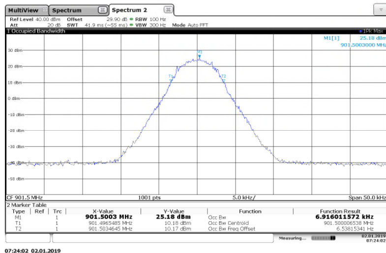
Figure 7.3.2-5: 901.5 MHz – 4FSK (Half Baud) Mode
