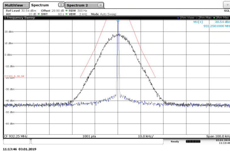
Figure 7.2.2-19: 932.25 MHz – 25 kHz Channel Spacing – 8FSK Mode
