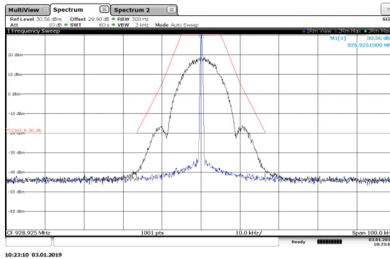
Figure 7.2.2-11: 928.925 MHz – 25 kHz Channel Spacing – 2FSK Mode
