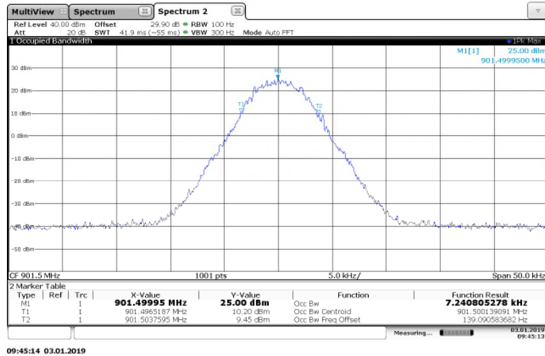
Figure 7.3.2-6: 901.5 MHz – 8FSK (Half Baud) Mode
