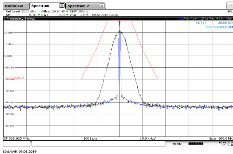
Figure 7.2.2-15: 928.925 MHz -- 25 kHz Channel Spacing – 4FSK (Half Baud) Mode
