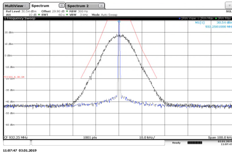
Figure 7.2.2-18: 932.25 MHz – 25 kHz Channel Spacing – 4FSK Mode
