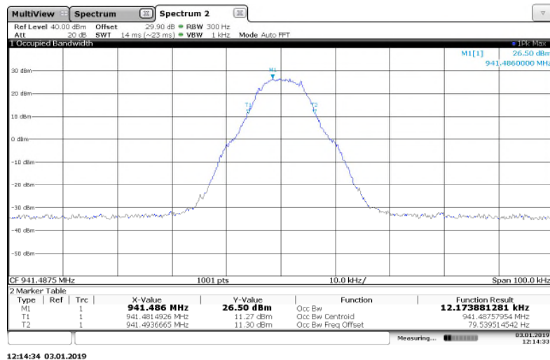
Figure 7.3.2-24: 941.4875 MHz – m4Pass 20k Mode
