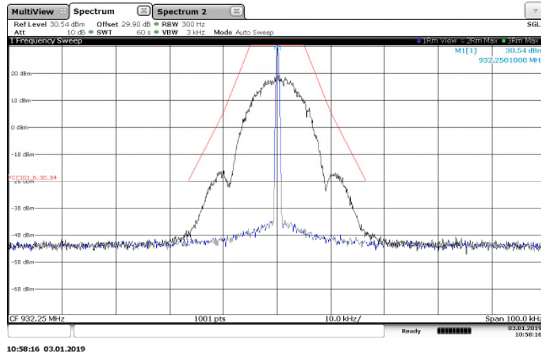
Figure 7.2.2-17: 932.25 MHz – 25 kHz Channel Spacing - 2FSK Mode
