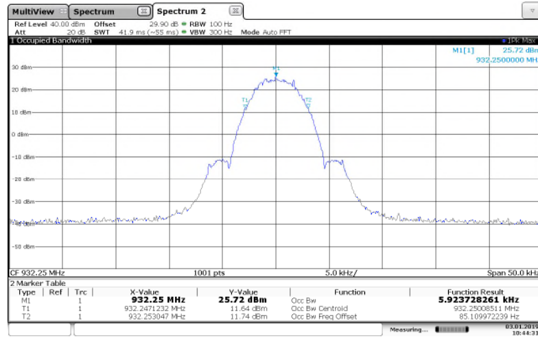
Figure 7.3.2-20: 932.25 MHz -- 2FSK(Half Baud) Mode
