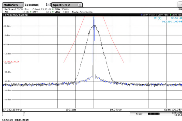
Figure 7.2.2-22: 932.25 MHz -- 25 kHz Channel Spacing – 8FSK (Half Baud) Mode
