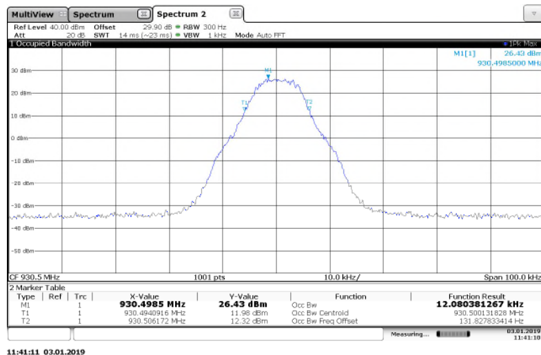
Figure 7.3.2-8: 930.5 MHz – m4Pass 20k Mode
