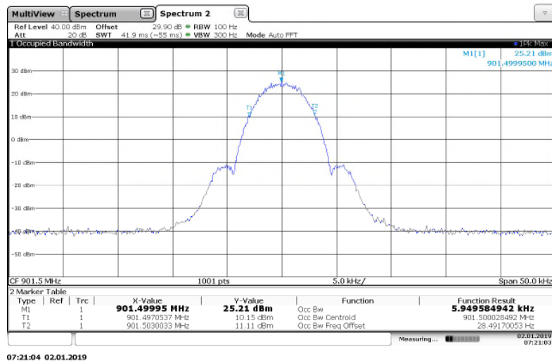
Figure 7.3.2-4: 901.5 MHz – 2FSK (Half Baud) Mode
