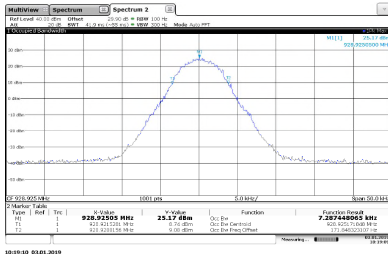
Figure 7.3.2-16: 928.925 MHz – 8FSK (Half Baud) Mode
