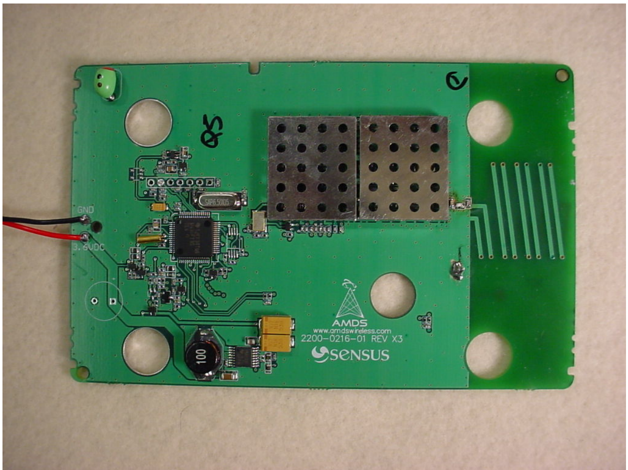
Figure 1: PCB 0216 Front Shields
