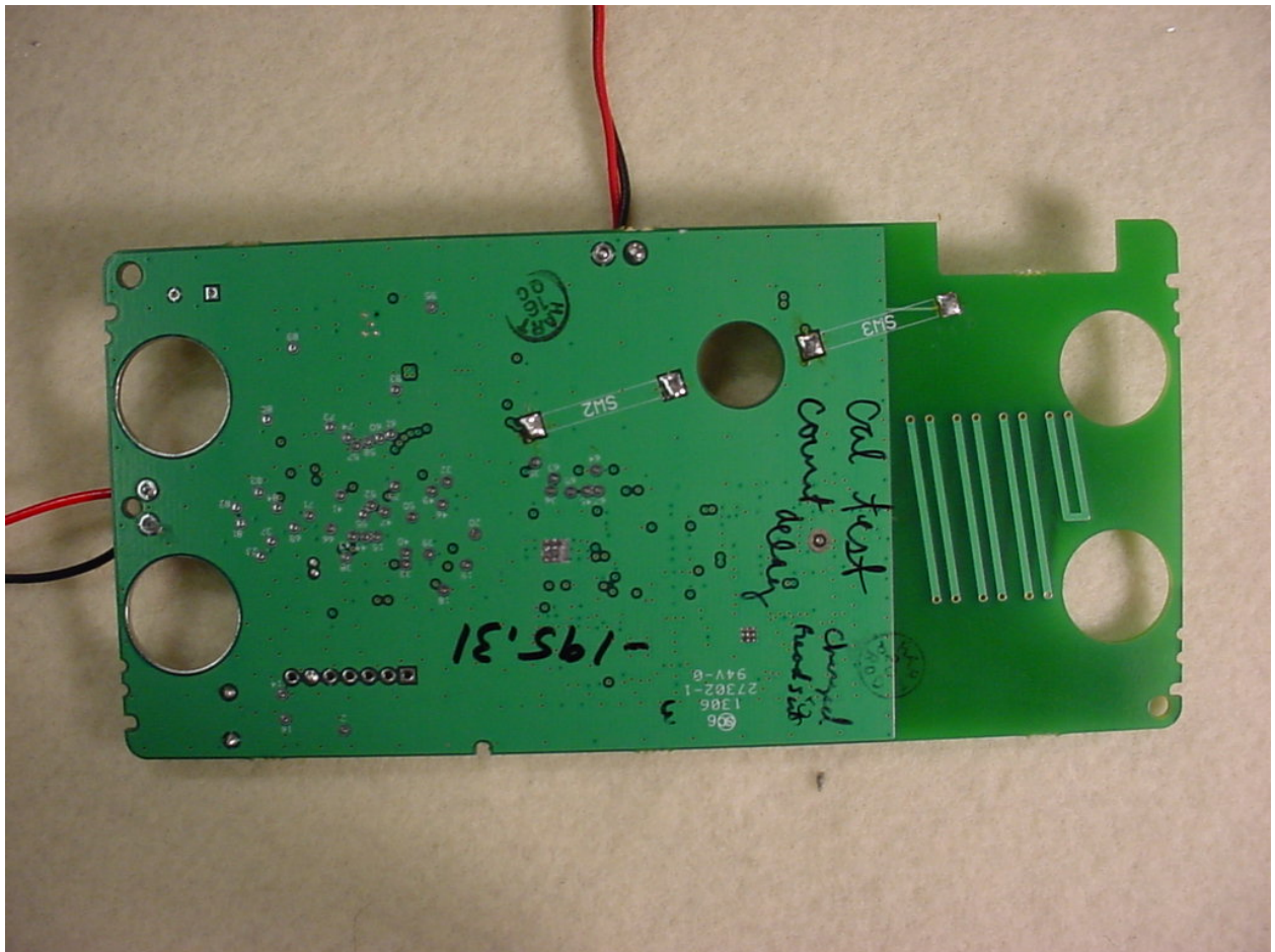
Figure 6: PCB 0217 Back
