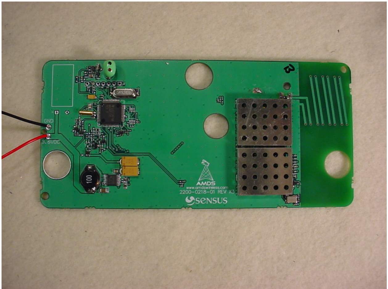
Figure 7: PCB 0218 Front Shields
