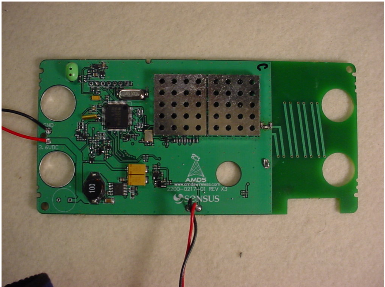
Figure 4: PCB 0217 Front Shields
