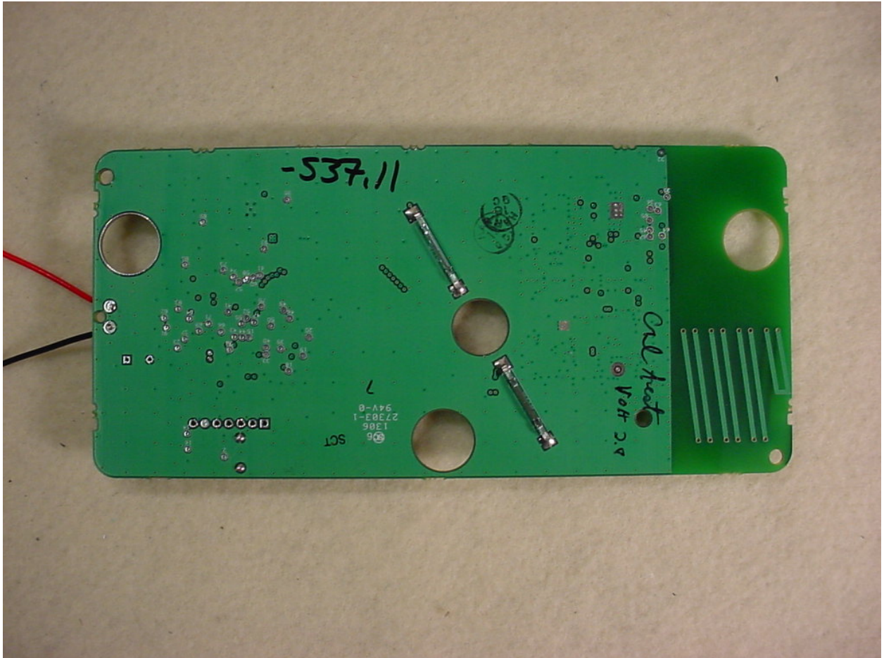
Figure 9: PCB 0218 Back
