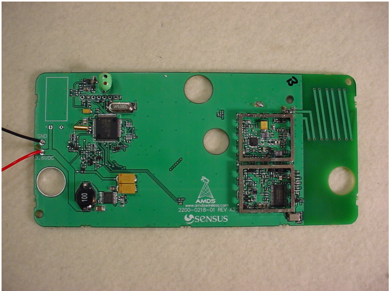
Figure 8: PCB 0218 Front No Shields
