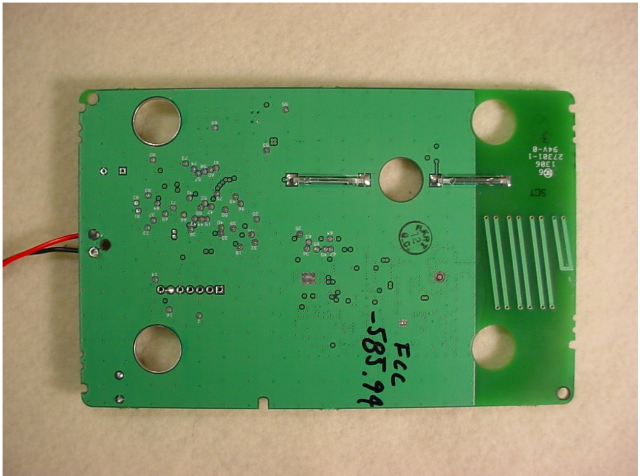
Figure 3: PCB 0216 Back
