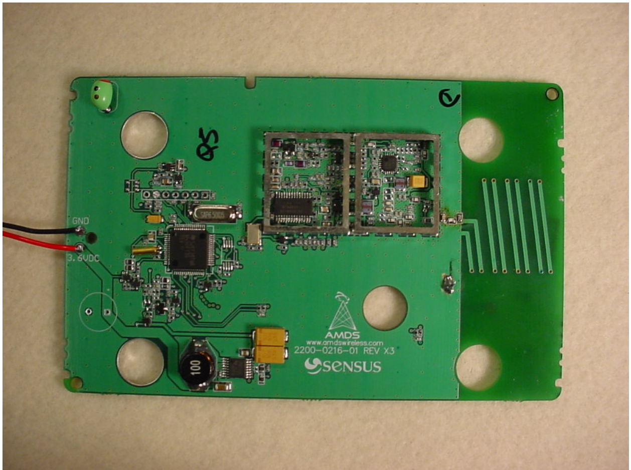
Figure 2: PCB 0216 Front No Shields
