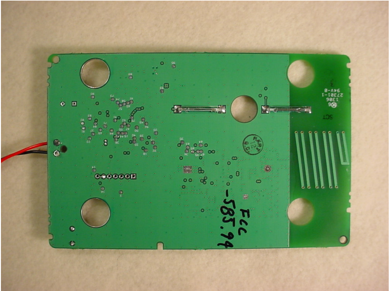
Figure 3: PCB 0216 Back
