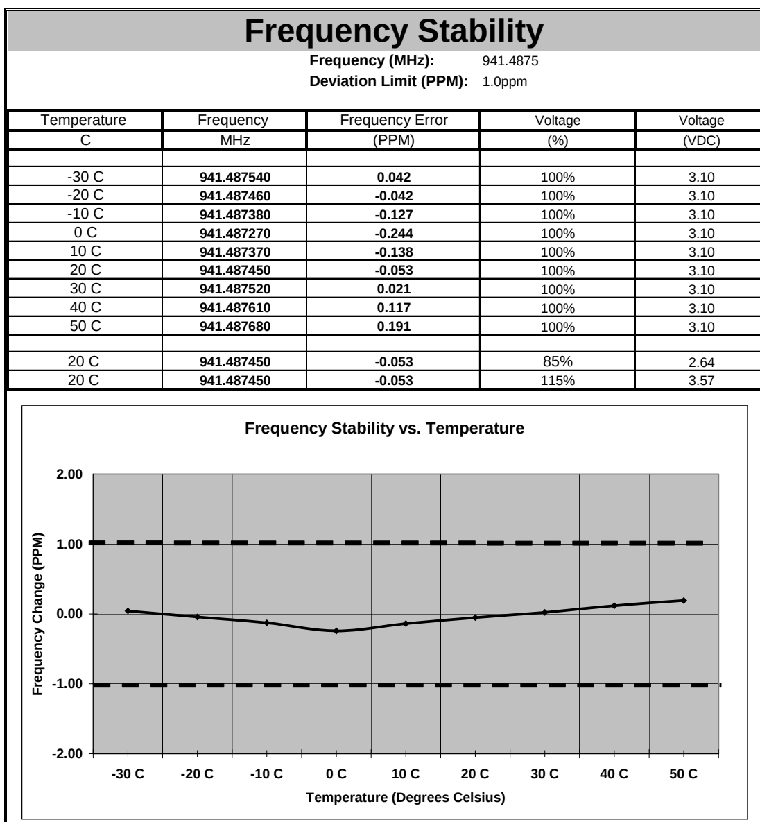
Figure 7.5.2-7: Frequency Stability – 941.4875MHz
