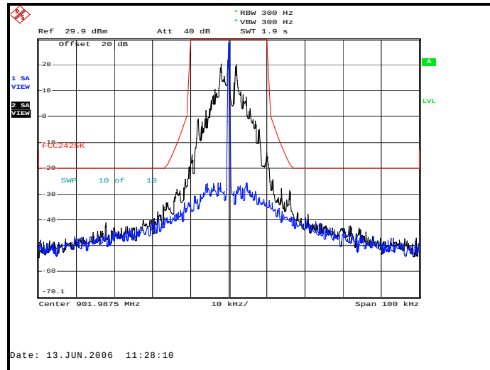
Figure 7.2.2-1: Normal Mode – 901.9875 MHz – 25 kHz Channel
