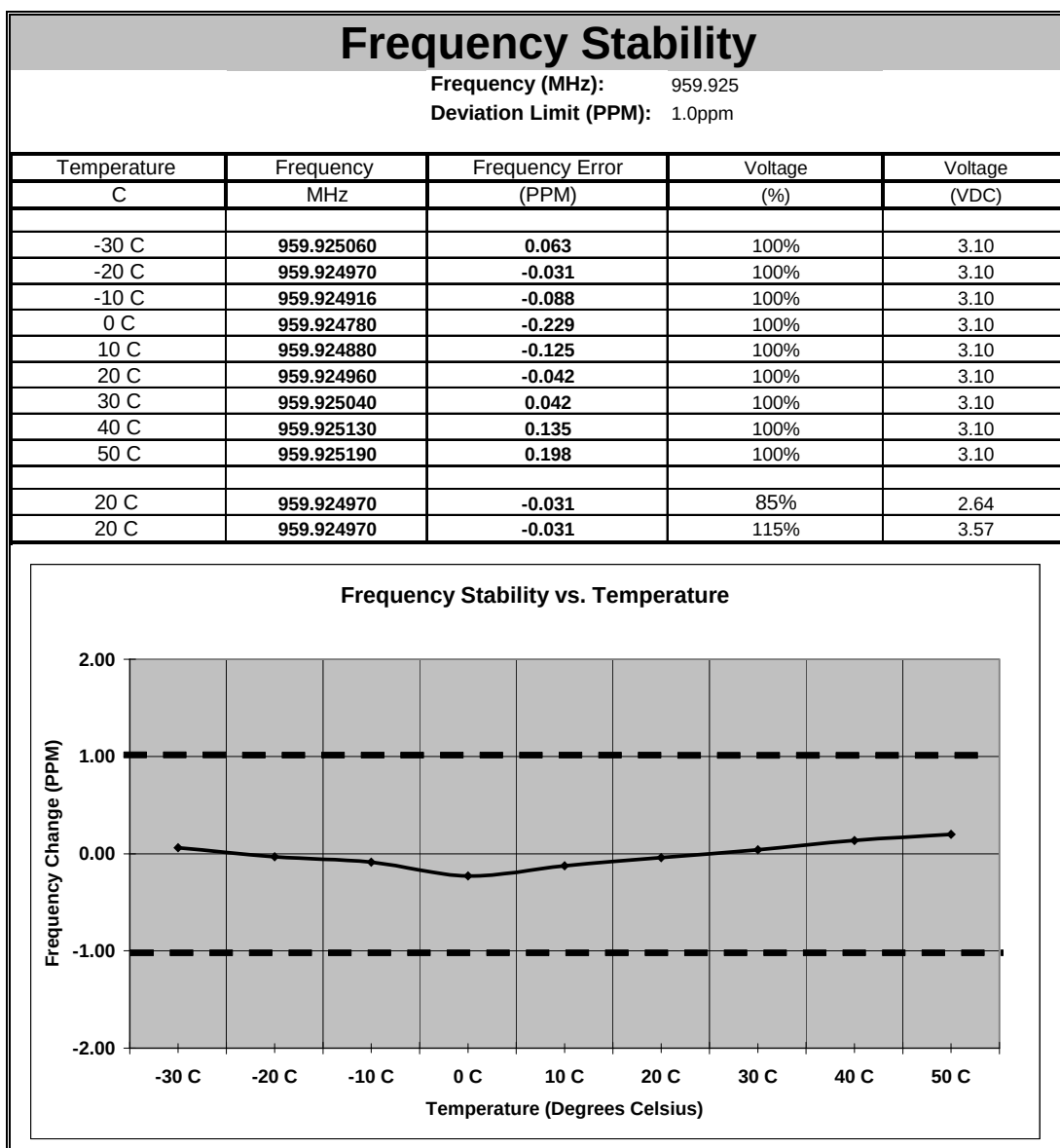
Figure 7.5.2-8: Frequency Stability – 959.925MHz
