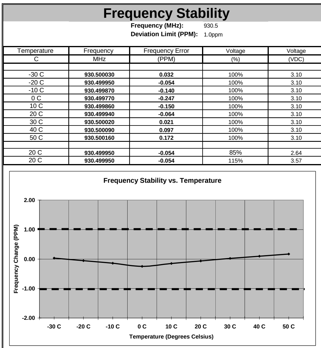
Figure 7.5.2-2: Frequency Stability – 930.5MHz
