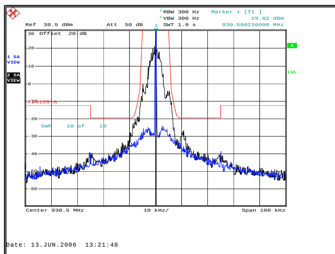
Figure 7.2.2-7: MPass Mode – 930.5 MHz – 12.5 kHz Channel
