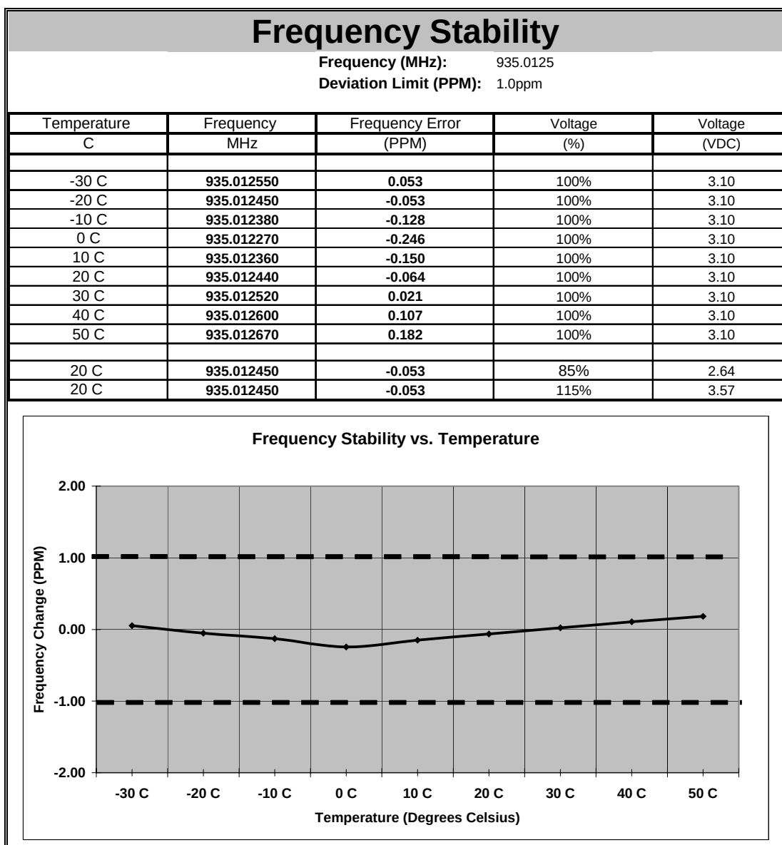
Figure 7.5.2-4: Frequency Stability – 935.0125MHz
