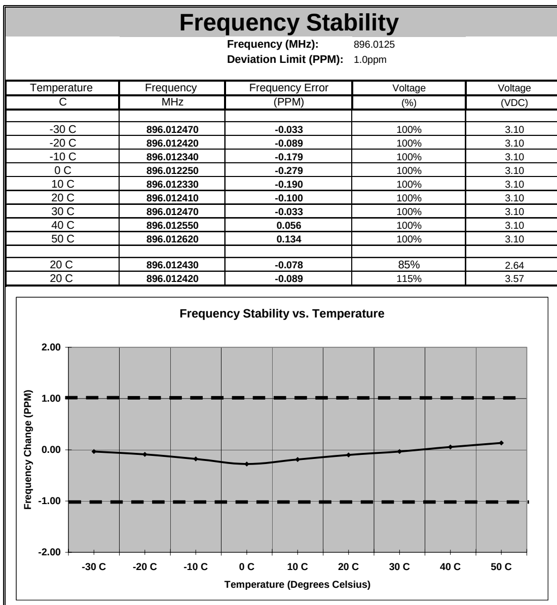
Figure 7.5.2-3: Frequency Stability – 896.0125MHz
