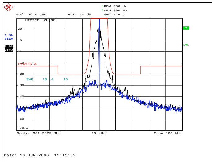
Figure 7.2.2-4: Half-Baud Rate – 901.9875 MHz – 12.5 kHz Channel
