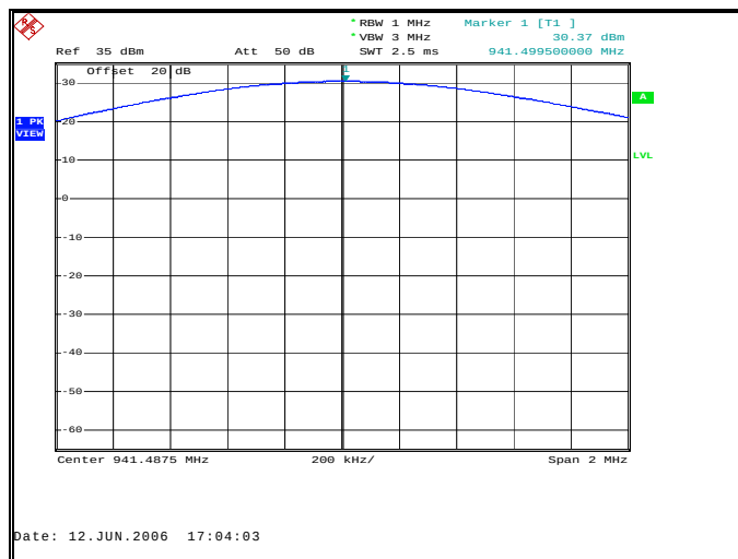
Figure 7.1.2-10: Peak Output Power 941.4875 MHz
