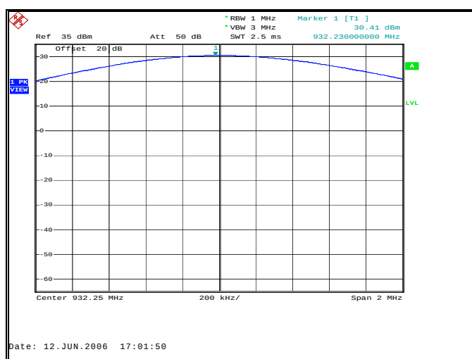
Figure 7.1.2-9: Peak Output Power 932.25 MHz
