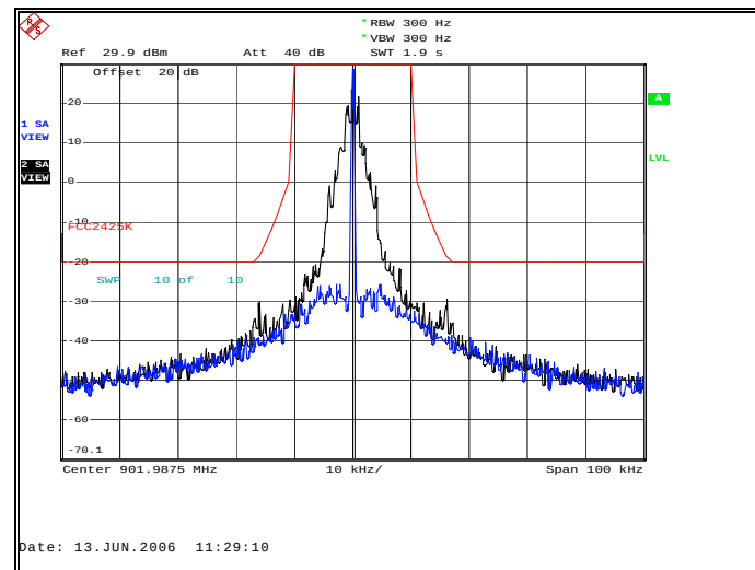
Figure 7.2.2-2: Half-Baud Rate Mode – 901.9875 MHz – 25 kHz Channel
