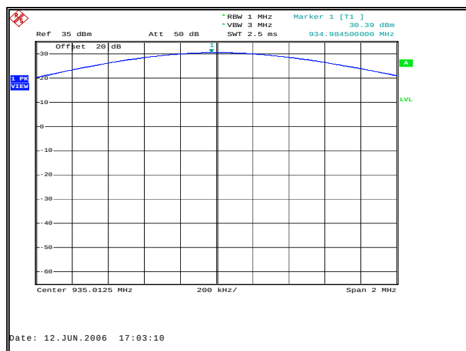
Figure 7.1.2-6: Peak Output Power 935.0125 MHz
