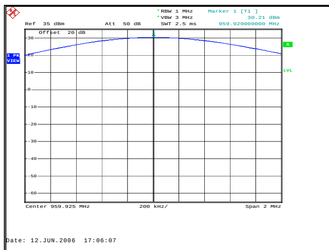
Figure 7.1.2-11: Peak Output Power 959.925 MHz
