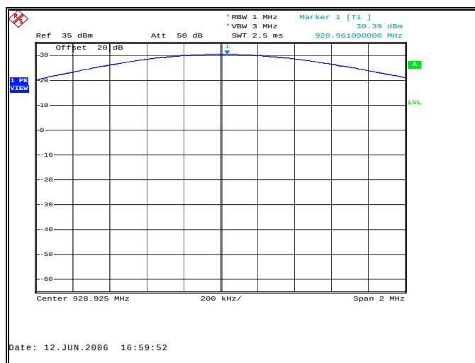
Figure 7.1.2-8: Peak Output Power 928.925 MHz
