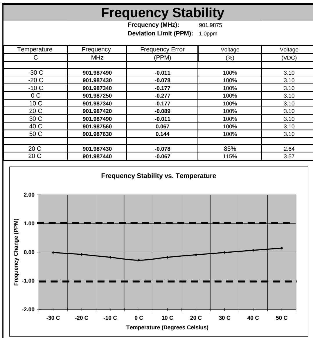
Figure 7.5.2-1: Frequency Stability – 901.9875MHz
