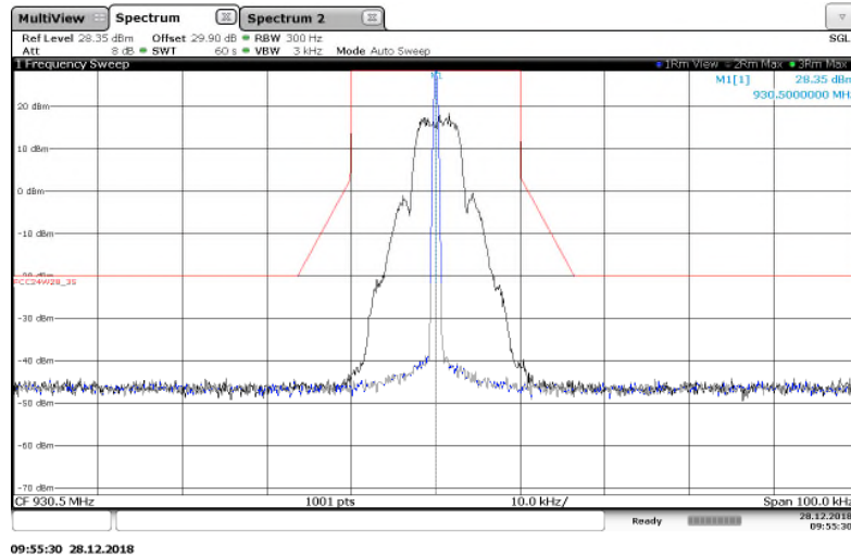
Figure 7.2.2-6: 930.5 MHz – 25 kHz Channel Spacing – mPass 5k Mode
