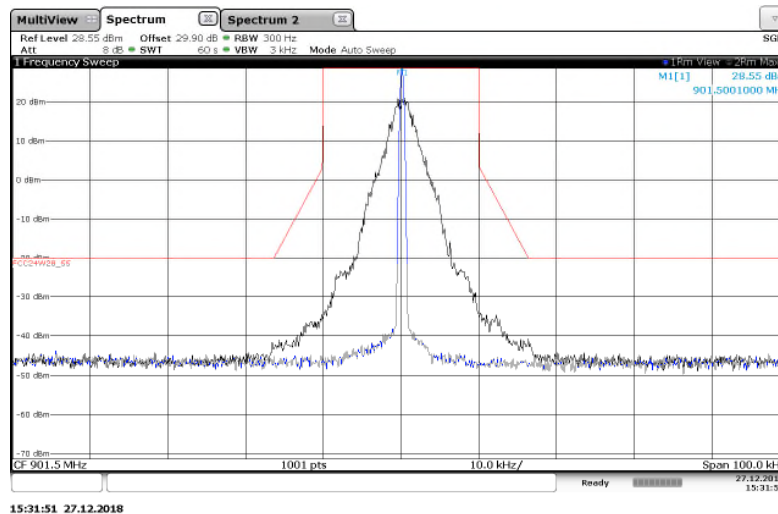
Figure 7.2.2-4: 901.5 MHz – 25 kHz Channel Spacing – Priority Mode
