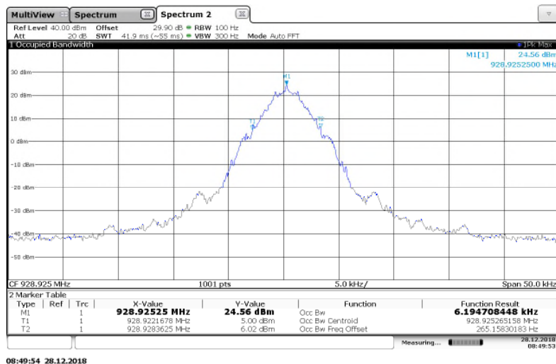
Figure 7.3.2-12: 928.925 MHz – C&I (Half Baud) Mode
