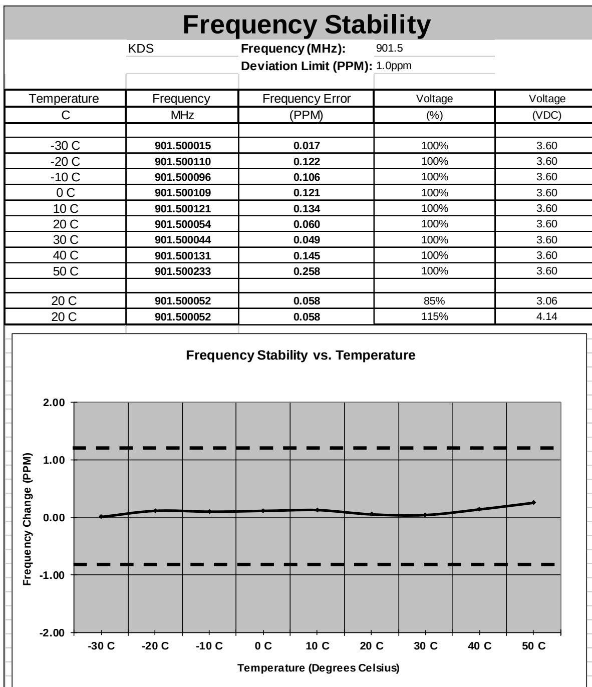
Figure 7.6.2-1: Frequency Stability – 901.5 MHz – KDS
