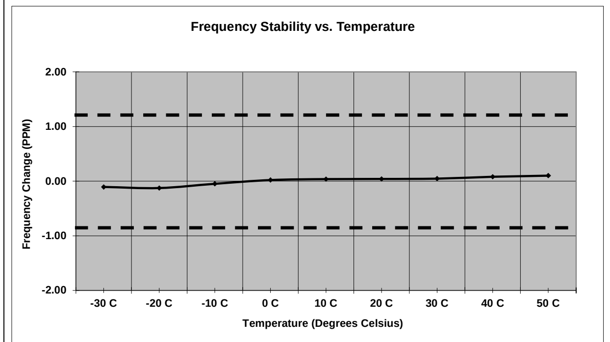
Figure 7.6.2-5: Frequency Stability – 930.5 MHz – ILSI
