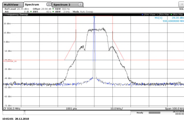
Figure 7.2.2-7: 930.5 MHz –25 kHz Channel Spacing – mPass 10k Mode
