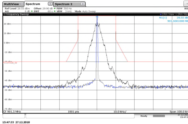
Figure 7.2.2-3: 901.5 MHz – 25 kHz Channel Spacing – C&amp;I (Half Baud) Mode
