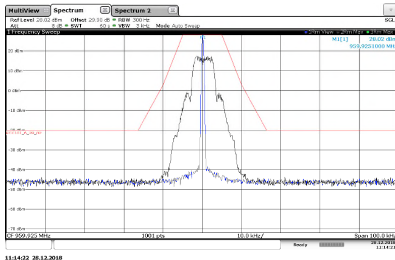
Figure 7.2.2-24: 959.925 MHz – 25 kHz Channel Spacing – mPass 5k Mode
