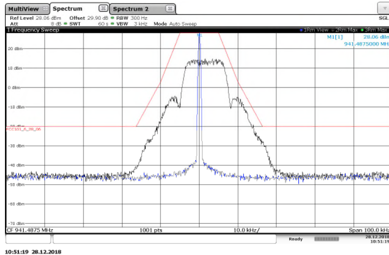
Figure 7.2.2-21: 941.4875 MHz – 25 kHz Channel Spacing – mPass 10k Mode
