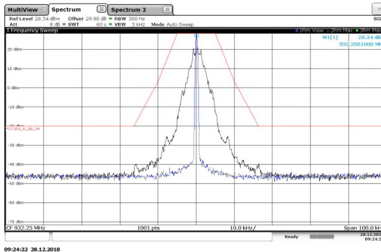
Figure 7.2.2-17: 932.25 MHz – 25 kHz Channel Spacing – C&amp;I (Half Baud) Mode
