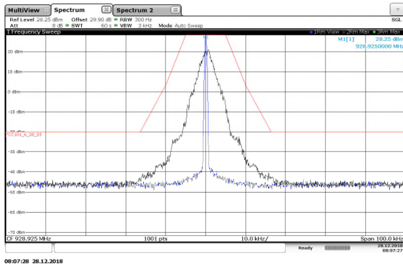
Figure 7.2.2-13: 928.925 MHz – 25 kHz Channel Spacing – Priority Mode
