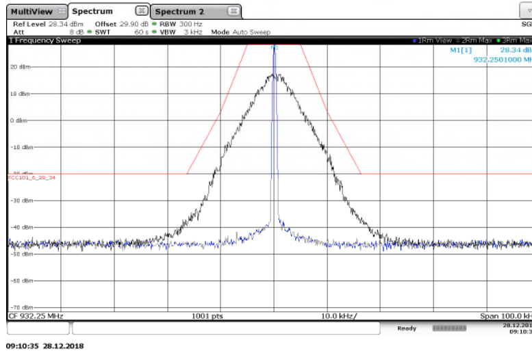
Figure 7.2.2-16: 932.25 MHz – 25 kHz Channel Spacing – Double Density Mode
