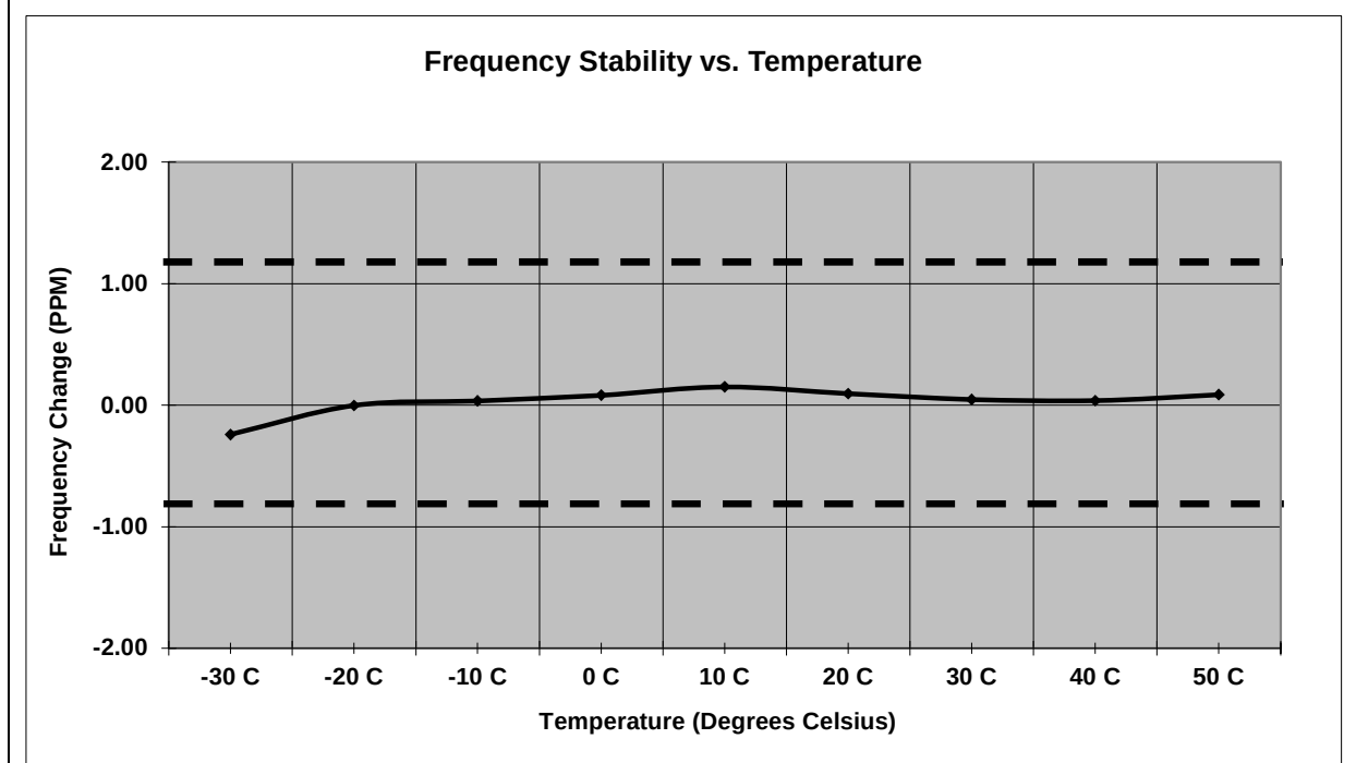
Figure 7.6.2-8: Frequency Stability – 959.925 MHz – ILSI
