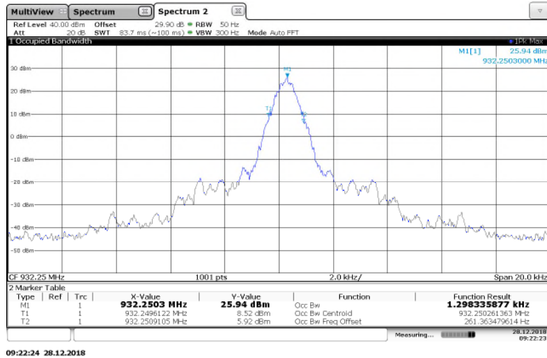
Figure 7.3.2-19: 932.25 MHz – Boost Mode
