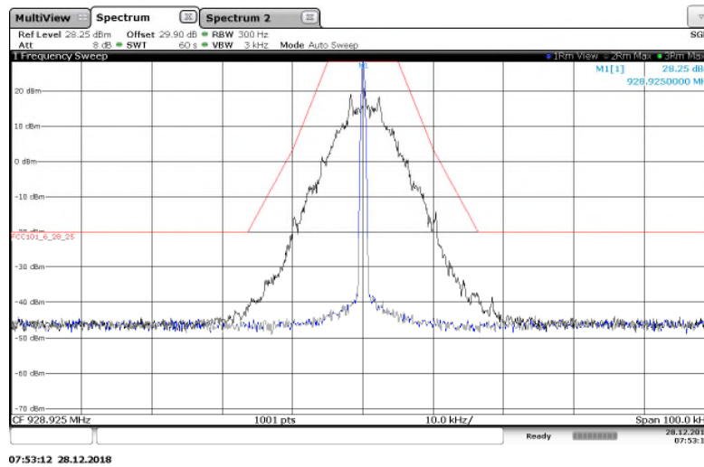
Figure 7.2.2-10: 928.925 MHz – 25 kHz Channel Spacing – Normal Mode
