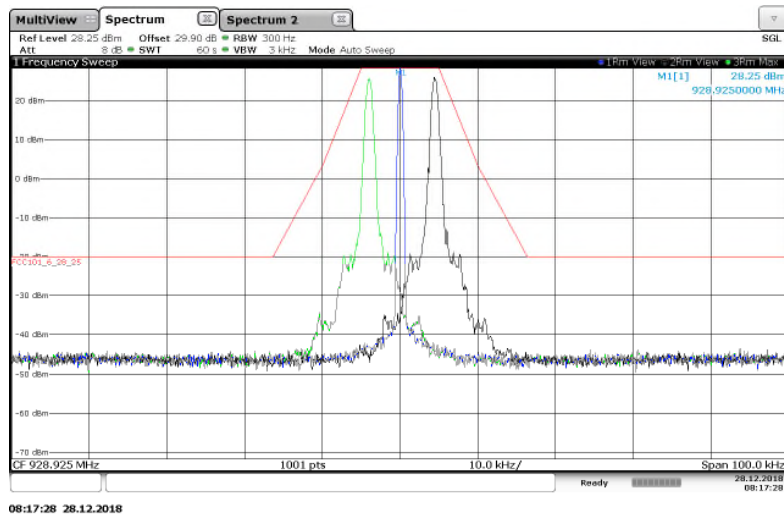
Figure 7.2.2-14: 928.925 MHz – 25 kHz Channel Spacing – Boost Mode
