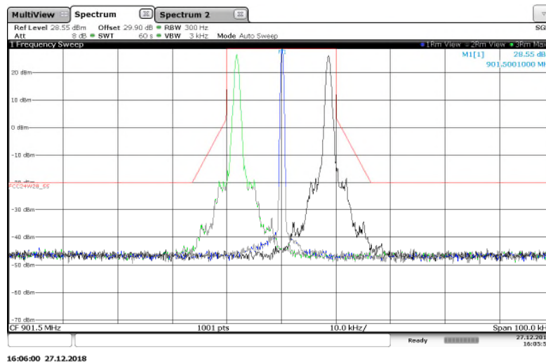
Figure 7.2.2-5: 901.5 MHz – 25 kHz Channel Spacing – Boost Mode
