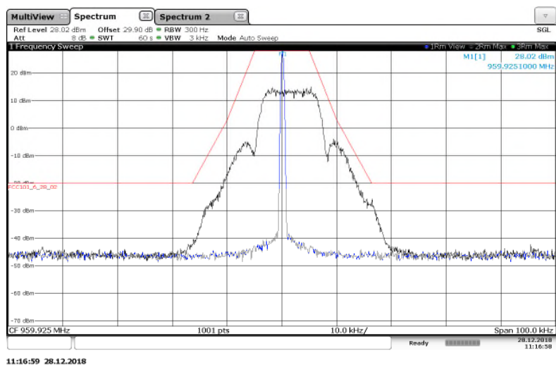
Figure 7.2.2-25: 959.925 MHz – 25 kHz Channel Spacing – mPass 10k Mode
