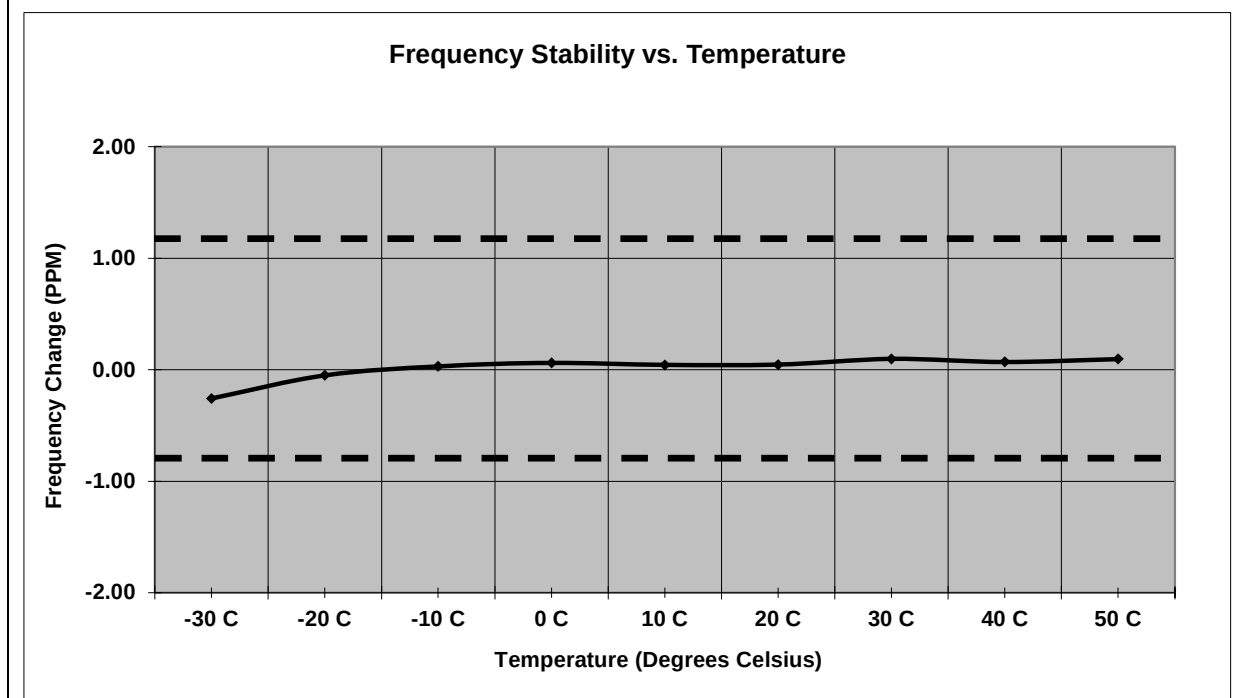
Figure 7.6.2-2: Frequency Stability – 901.5 MHz – ILSI
