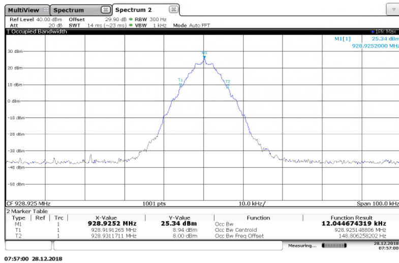
Figure 7.3.2-10: 928.925 MHz – Normal Mode
