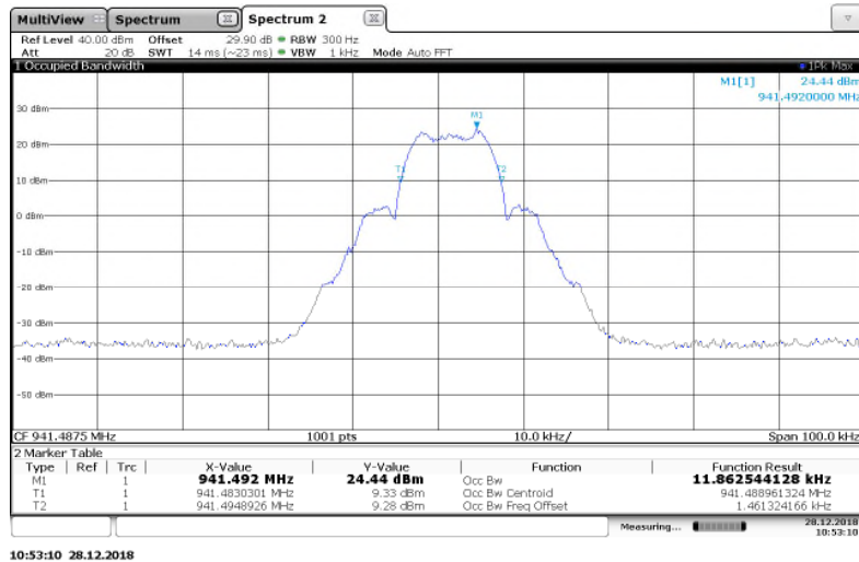
Figure 7.3.2-21: 941.4875 MHz – MPass 10k Mode
