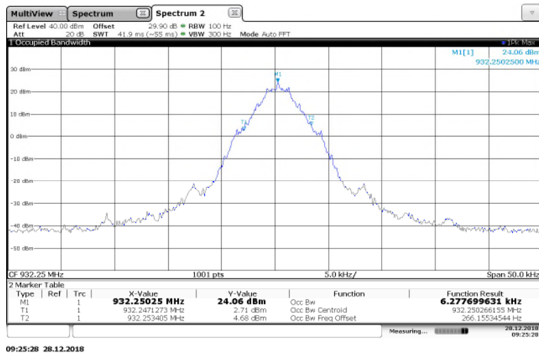
Figure 7.3.2-17: 932.25 MHz – C&amp;I (Half Baud) Mode
