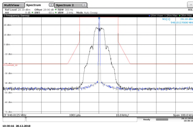
Figure 7.2.2-8: 940.0125 MHz – 25 kHz Channel Spacing – mPass 5k Mode
