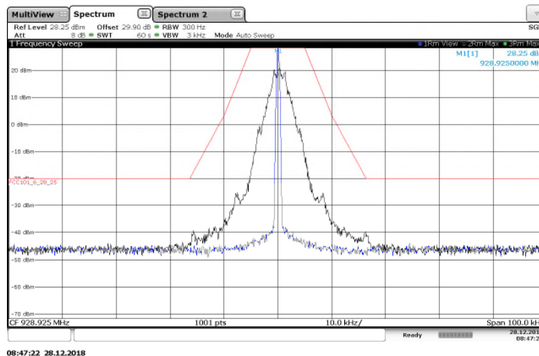
Figure 7.2.2-12: 928.925 MHz – 25 kHz Channel Spacing – C&I (Half Baud) Mode
