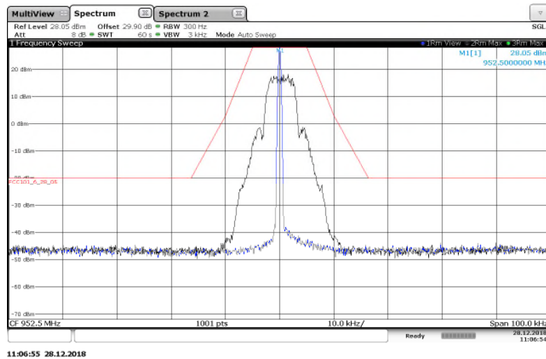
Figure 7.2.2-22: 952.5 MHz – 25 kHz Channel Spacing – mPass 5k Mode
