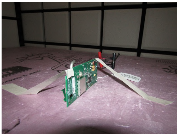
Figure 6: Radiated Emissions – Back – Above 1GHz – YPOS
