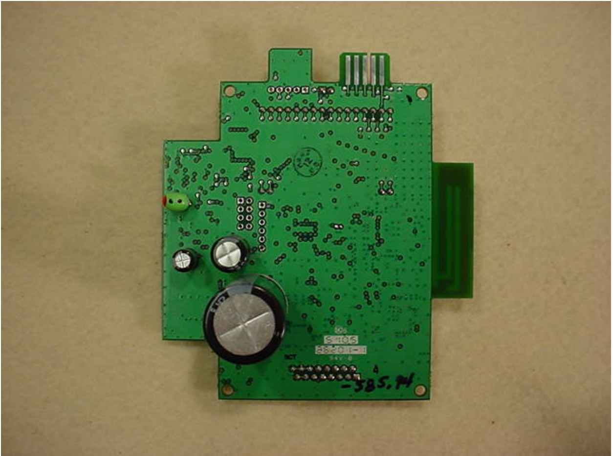
Figure 3: Internal Photographs – Sensus AMDS Integrated Display Transceiver Board (IDTB) - Back
