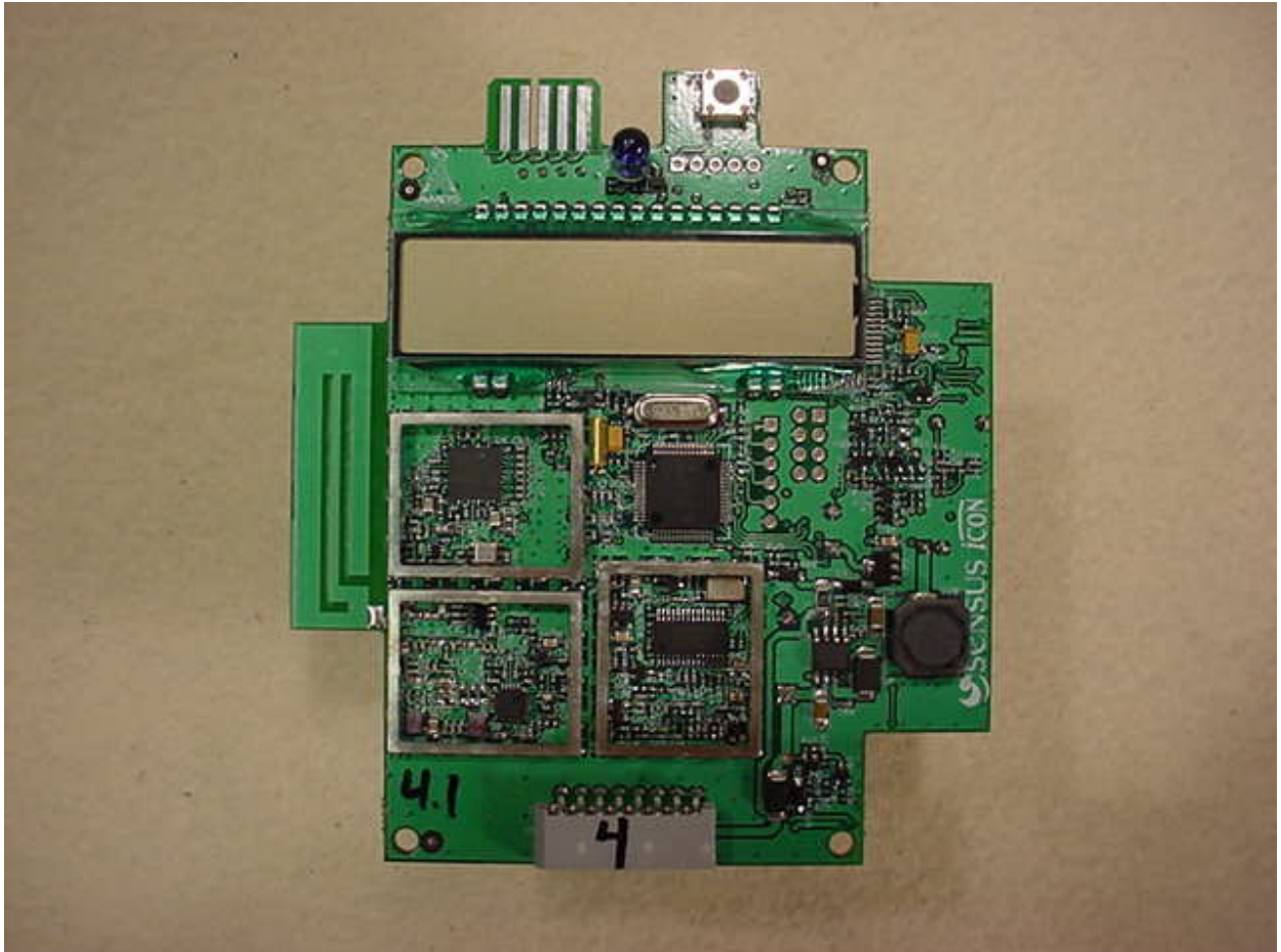
Figure 2: Internal Photographs – Sensus AMDS Integrated Display Transceiver Board (IDTB) -Front
