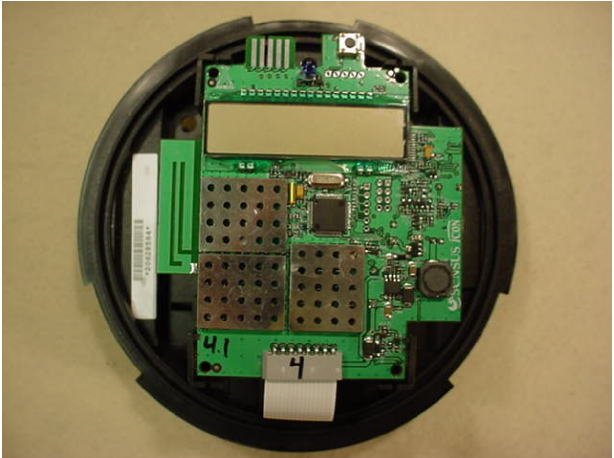
Figure 1: Internal Photographs – Sensus AMDS Integrated Display Transceiver Board (IDTB) -Front
