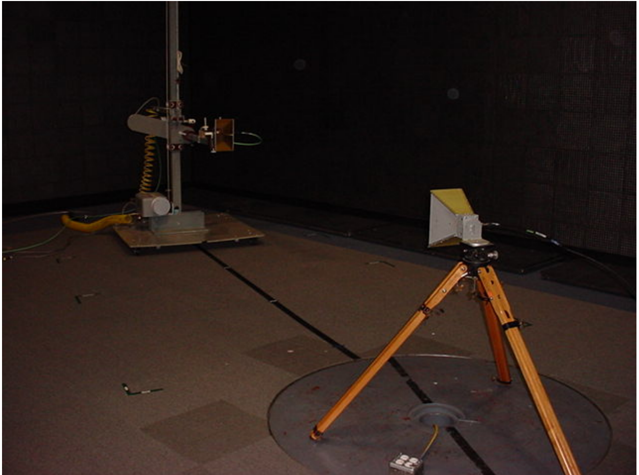
Figure 2: Spurious Emissions – Transmitter
