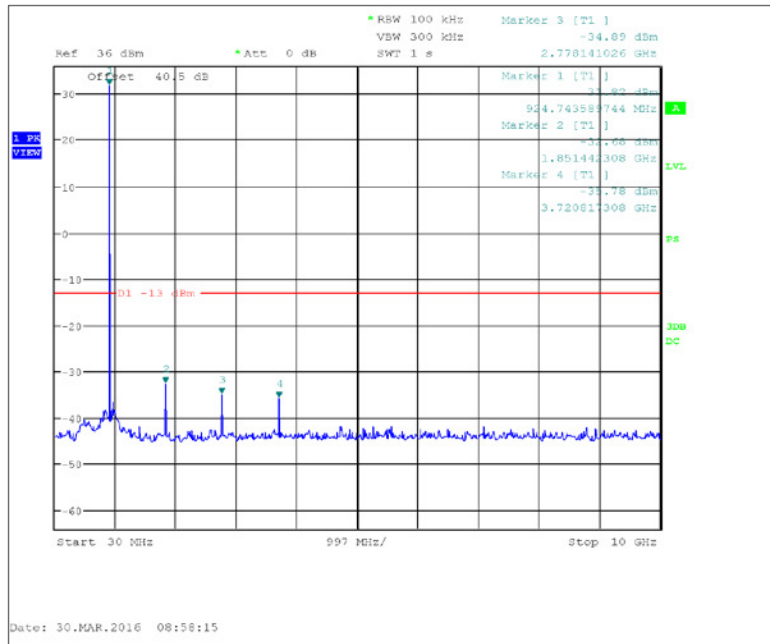
Figure 7.3.2-14: 928.925 MHz – 30 MHz to 10 GHz – 2SFSK
