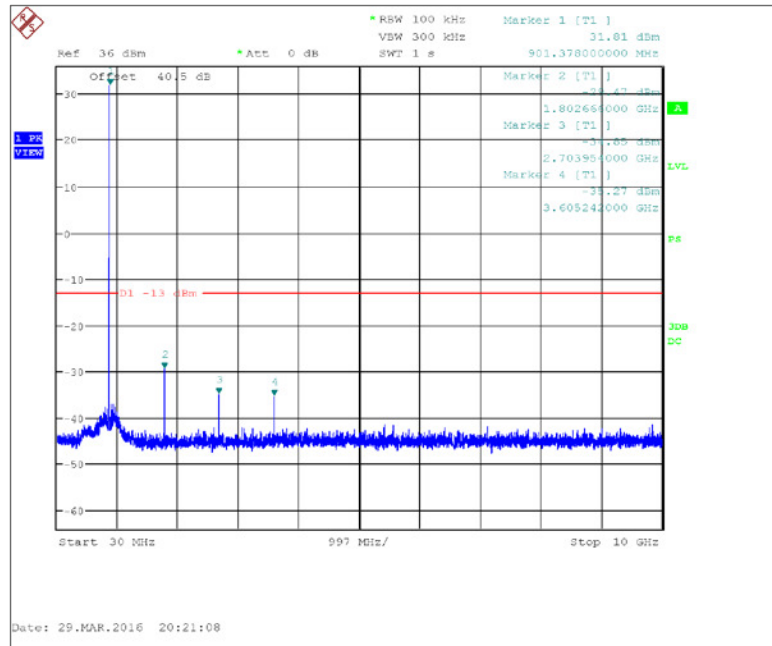
Figure 7.3.2-4: 901.5 MHz – 30 MHz to 10 GHz – 2SFSK
