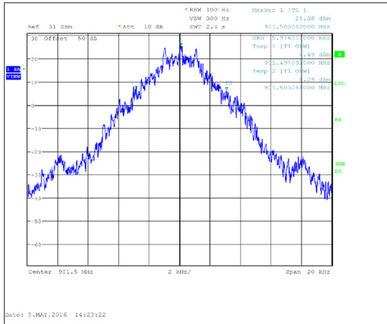
Figure 7.2.3-7: 901.5 MHz – C&amp;I
