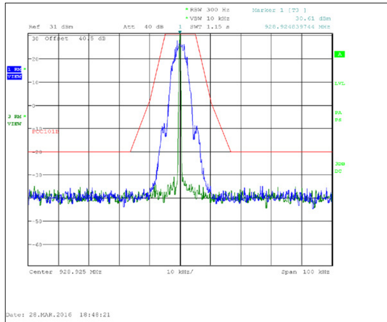
Figure 7.2.2-17: 928.925 MHz – 25 kHz Channel Spacing – 2SFSK (Half Baud)
