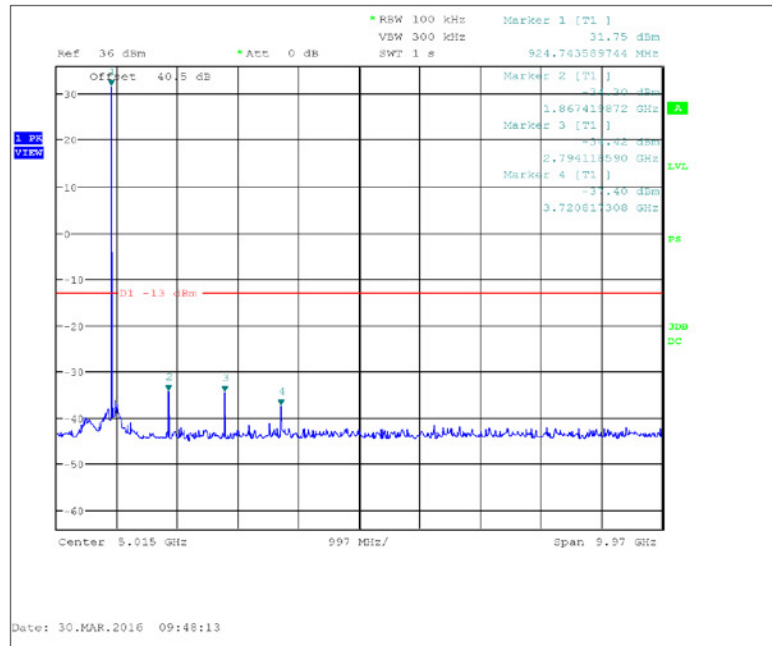
Figure 7.3.2-20: 932.25 MHz – 30 MHz to 10 GHz – 2SFSK
