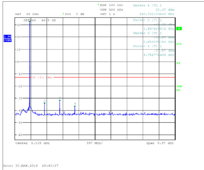
Figure 7.3.2-10: 940.0125 MHz – 30 MHz to 10 GHz – m4Pass 20k
