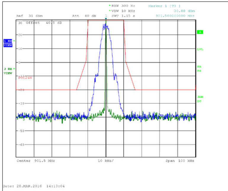
Figure 7.2.2-2: 901.5 MHz – 25 kHz Channel Spacing – 2SFSK (Half Baud)
