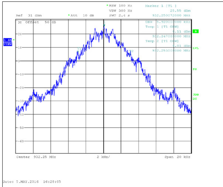
Figure 7.2.3-35: 932.25 MHz — C&amp;I
