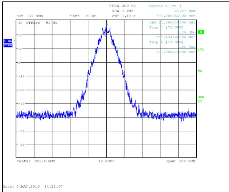
Figure 7.2.3-9: 901.5 MHz – Normal
