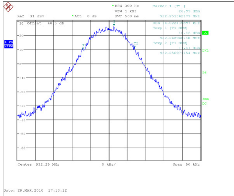
Figure 7.2.3-33: 932.25 MHz — 4FSK
