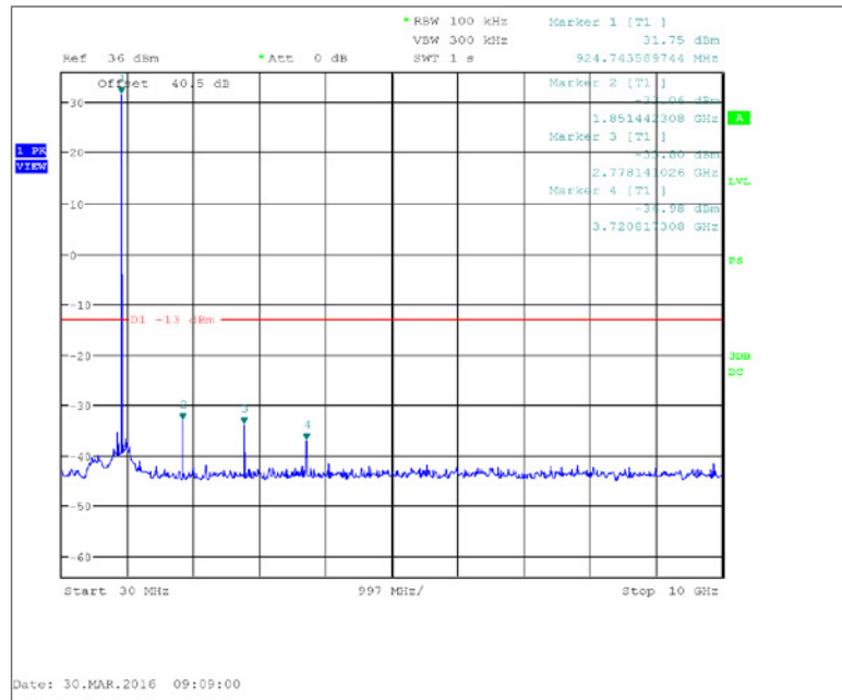
Figure 7.3.2-11: 928.925 MHz – 30 MHz to 10 GHz – 2FSK (Half Baud)
