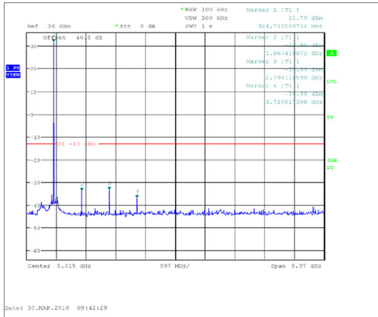
Figure 7.3.2-22: 932.25 MHz – 30 MHz to 10 GHz – 8SFSK
