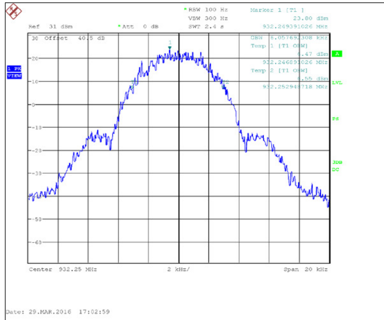
Figure 7.2.3-29: 932.25 MHz – 2FSK (Half Baud)
