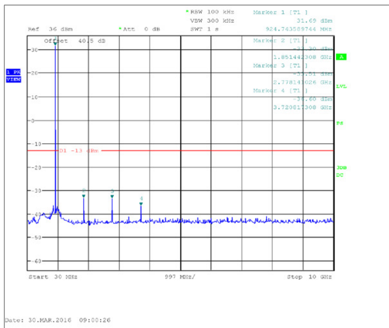
Figure 7.3.2-15: 928.925 MHz – 30 MHz to 10 GHz – 4SFSK
