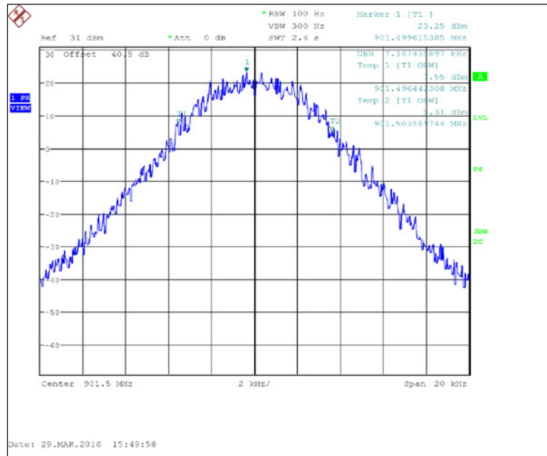
Figure 7.2.3-2: 901.5 MHz – 4FSK (Half Baud)
