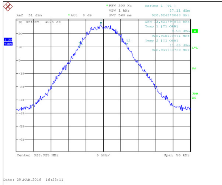
Figure 7.2.3-23: 928.925 MHz — 4FSK
