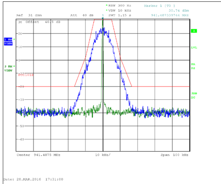
Figure 7.2.2-36: 941.4875 MHz – 25 kHz Channel Spacing - m4Pass 20k Mode
