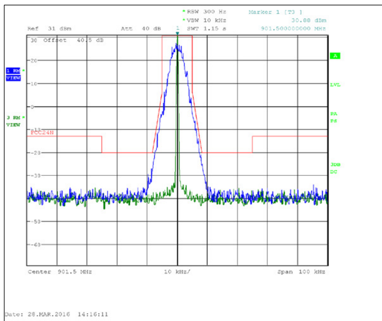
Figure 7.2.2-3: 901.5 MHz – 12.5 kHz Channel Spacing – 4SFSK (Half Baud)
