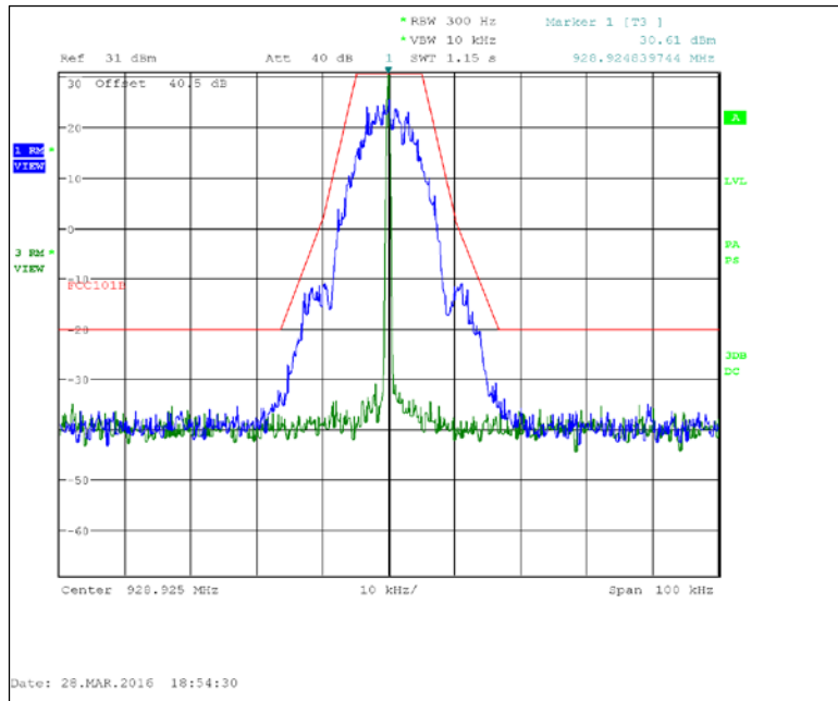
Figure 7.2.2-22: 928.925 MHz – 25 kHz Channel Spacing – 2SFSK
