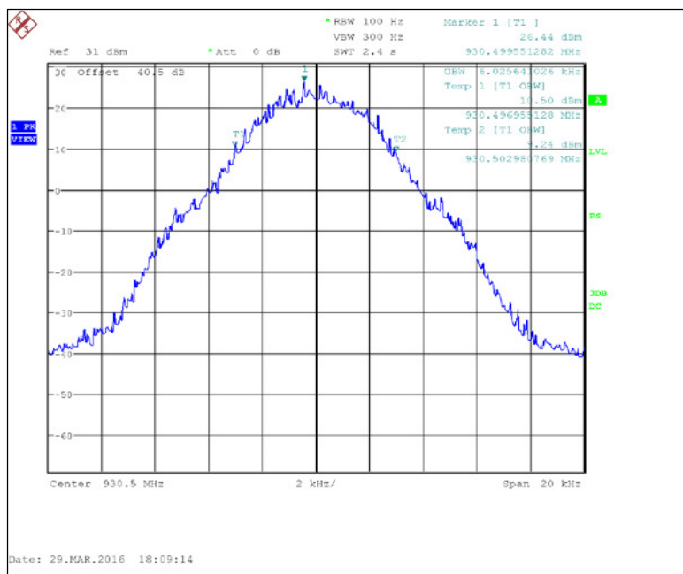
Figure 7.2.3-11: 930.5 MHz – m4Pass 10k Mode
