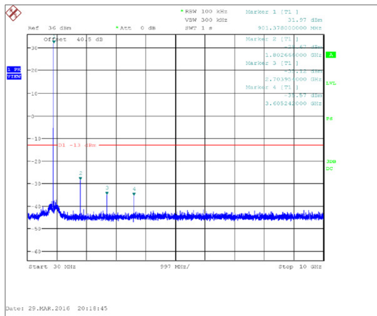
Figure 7.3.2-5: 901.5 MHz – 30 MHz to 10 GHz – 4SFSK
