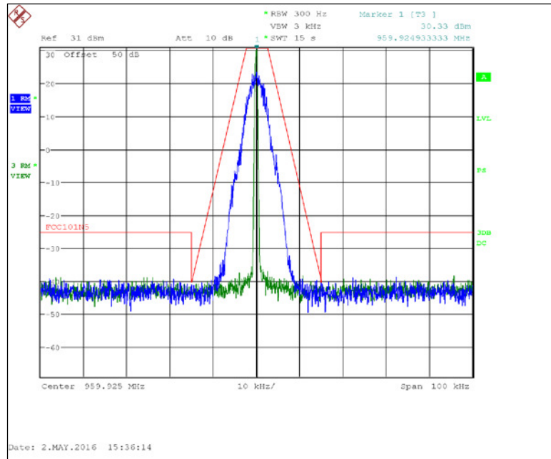
Figure 7.2.2-40: 959.925 MHz – 12.5 kHz Channel Spacing - m4Pass 10k Mode
