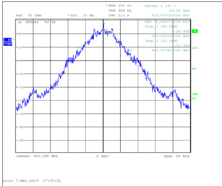
Figure 7.2.3-25: 928.925 MHz — C&amp;I
