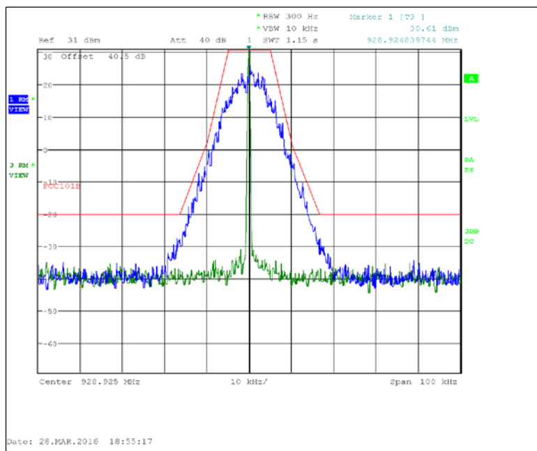
Figure 7.2.2-23: 928.925 MHz – 25 kHz Channel Spacing – 4SFSK
