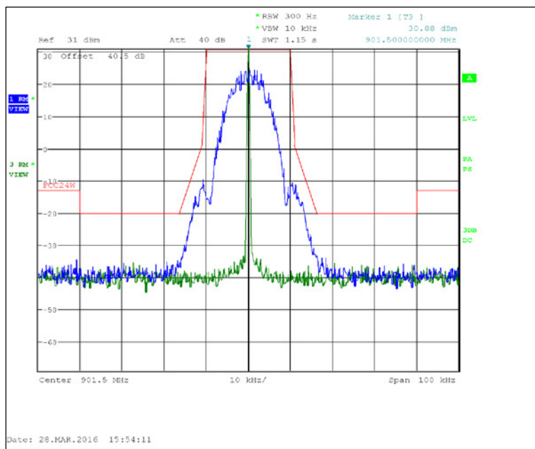
Figure 7.2.2-7: 901.5 MHz – 25 kHz Channel Spacing – 2SFSK
