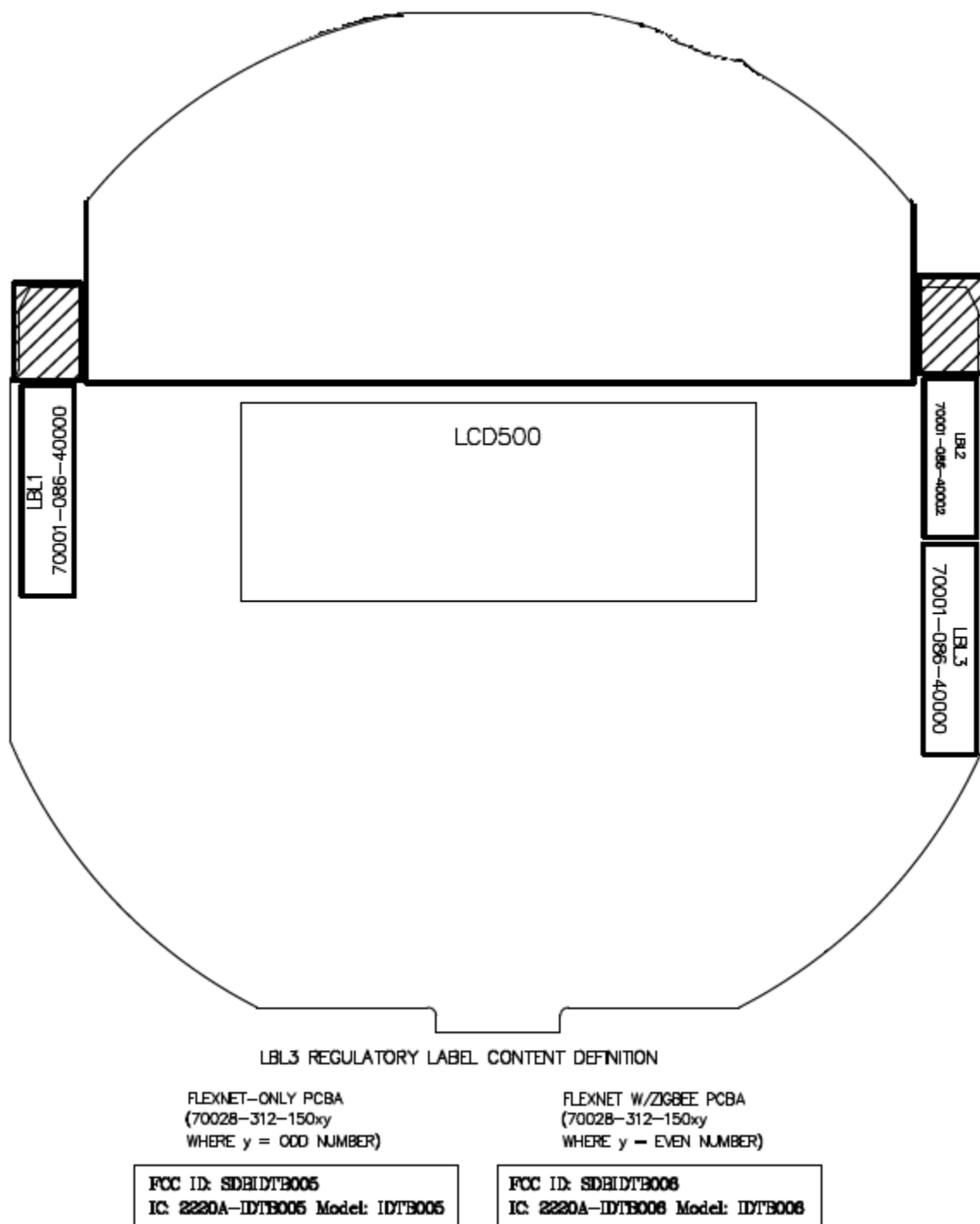
Figure 2: Top of Primary PCBA
