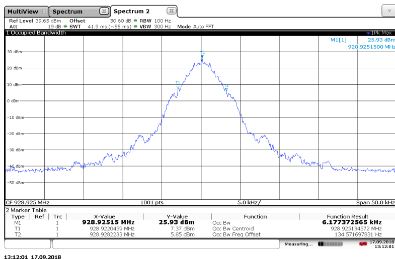
Figure 7.3.2-21: 928.925 MHz – C&I (Half Baud) Mode
