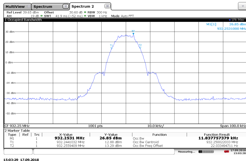
Figure 7.3.2-36: 932.25 MHz – 2SFSK Mode
