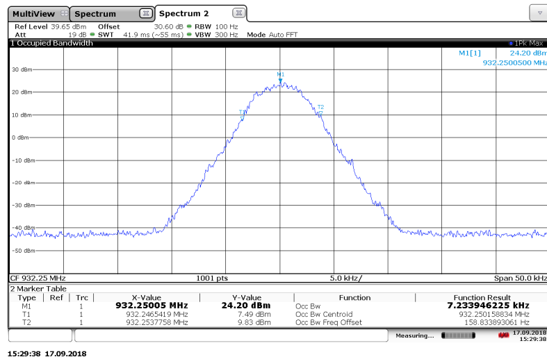
Figure 7.3.2-35: 932.25 MHz – 8SFSK (Half Baud) Mode
