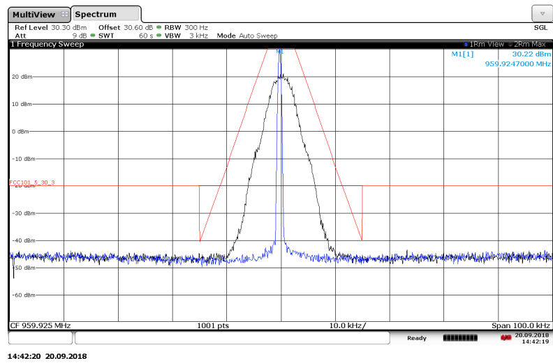
Figure 7.2.2-49: 959.925 MHz – 12.5 kHz Channel Spacing – m4Pass 10k Mode
