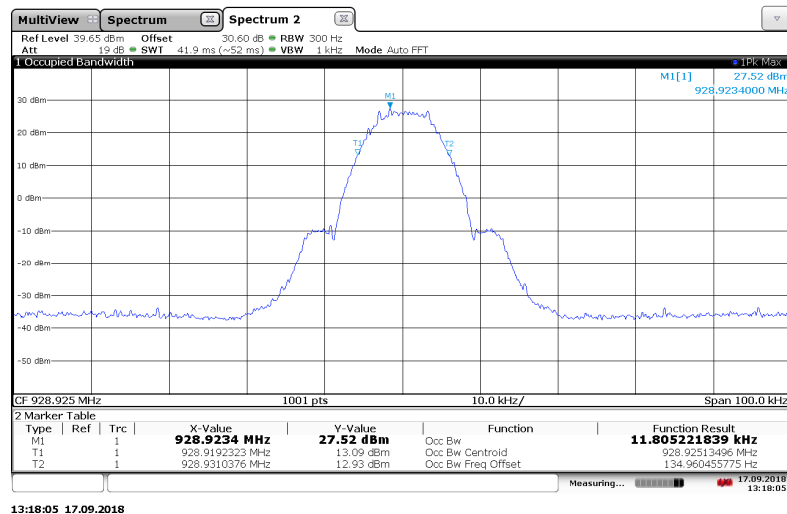
Figure 7.3.2-26: 928.925 MHz – 2FSK Mode
