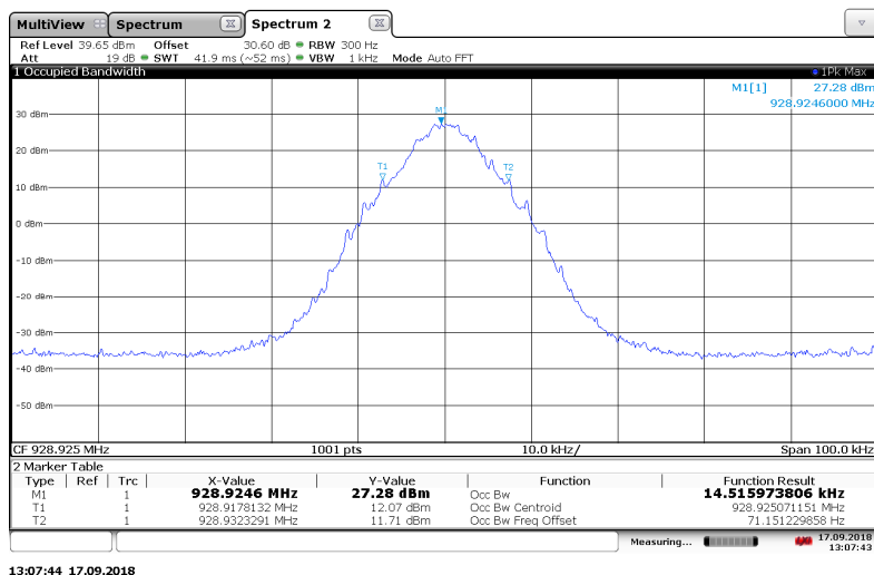
Figure 7.3.2-20: 928.925 MHz – Double Density Mode
