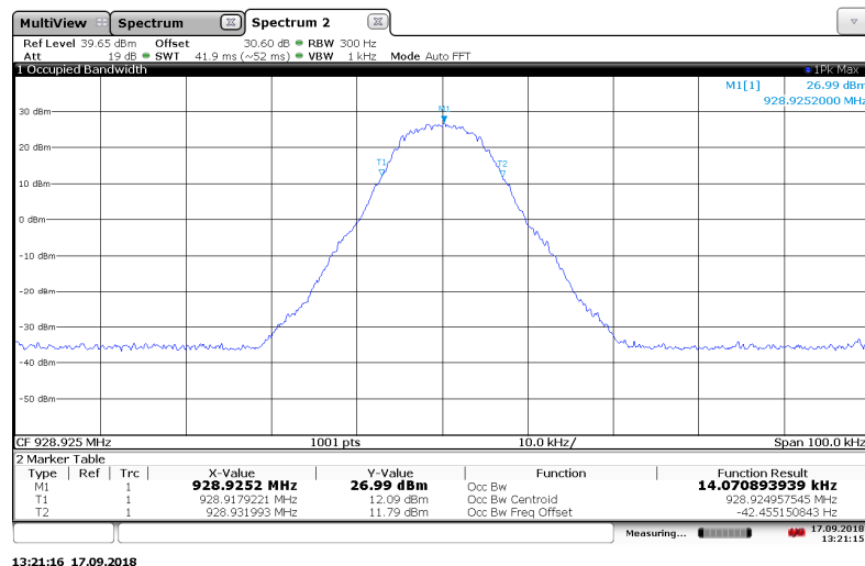
Figure 7.3.2-27: 928.925 MHz – 4FSK Mode
