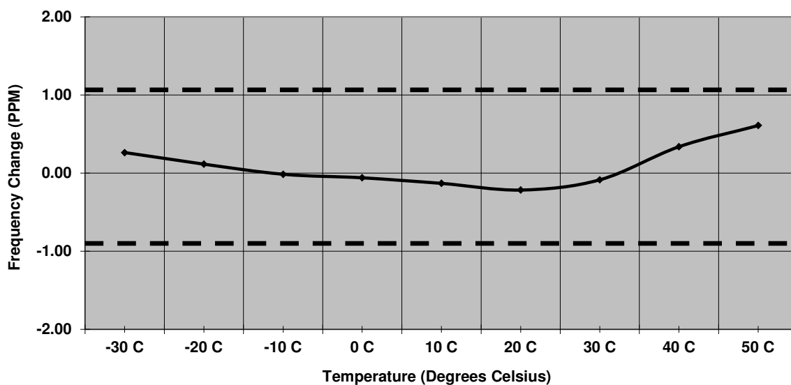
Figure 7.6.2-6: Frequency Stability – 930.5 MHz – EPSON
