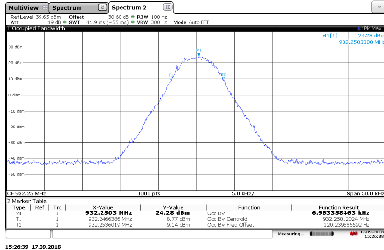
Figure 7.3.2-34: 932.25 MHz – 4SFSK (Half Baud) Mode
