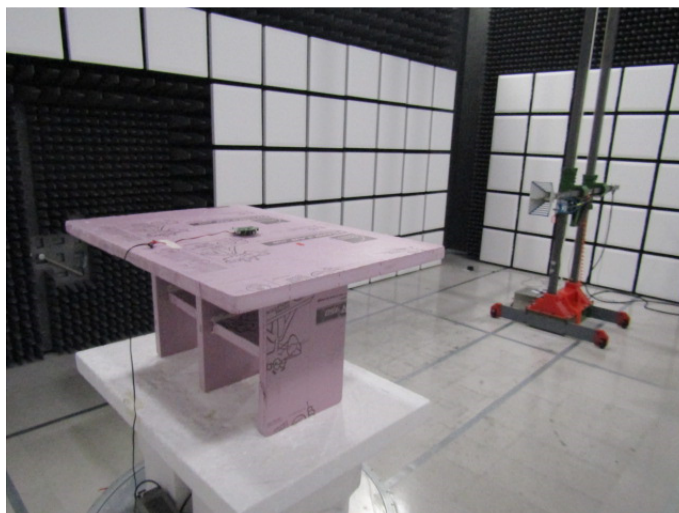
Figure 4: Radiated Emissions – Back – Above 1GHz – XPOS
