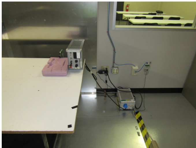
Figure 8: Conducted Emissions
