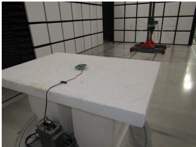
Figure 2: Radiated Emissions – Back – Below 1GHz
