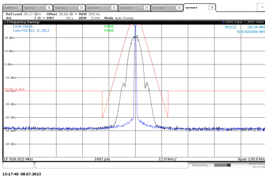
Figure 2.2.6-22 - Emissions Mask – KDS TCXO – 928.925 MHz - 12.5 kHz Channel Spacing - 2FSK (Half Baud) Mode
