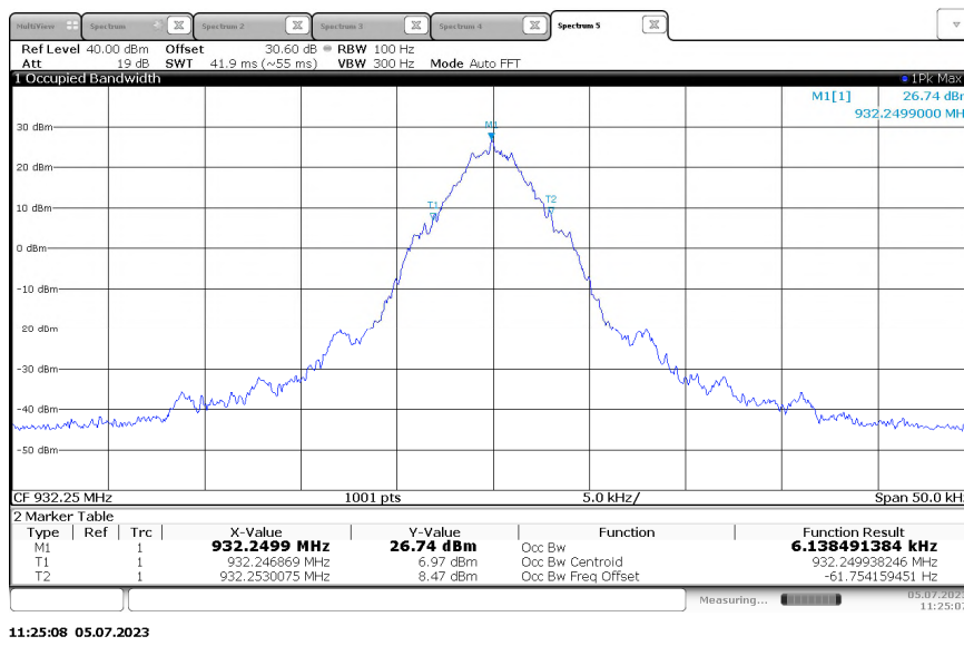
Figure 2.3.6-27 - 99% Bandwidth – KDS TCXO – 932.25 MHz - C&amp;I Mode
