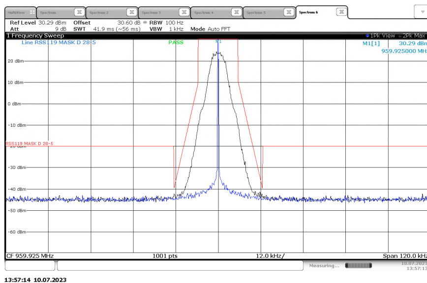
Figure 2.2.6-42 - Emissions Mask – KDS TCXO – 959.925 MHz - 12.5 kHz Channel Spacing - m4Pass10 Mode
