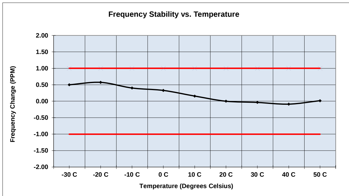
Figure 2.6.6-6 - Frequency Stability – KDS TCXO – 959.925 MHz
