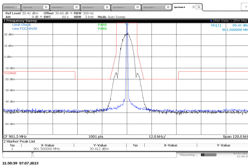
Figure 2.2.6-7 - Emissions Mask – KDS TCXO – 901.5 MHz - 12.5 kHz Channel Spacing - 2SFSK (Half Baud) Mode
