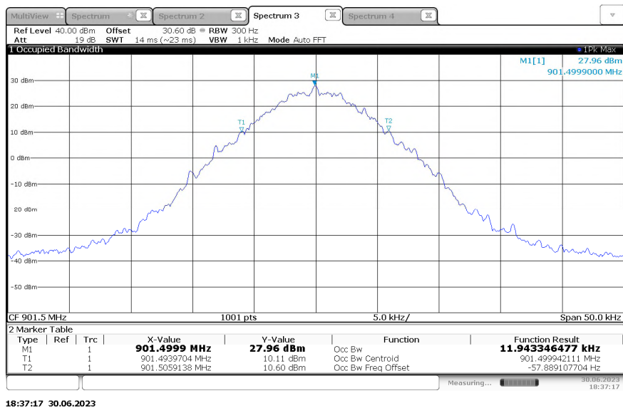
Figure 2.3.6-1 - 99% Bandwidth – KDS TCXO – 901.5 MHz - Normal Mode
