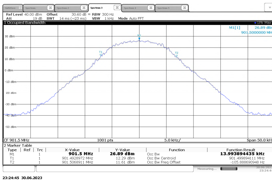
Figure 2.3.6-9 - 99% Bandwidth – KDS TCXO – 901.5 MHz - 4FSK Mode
