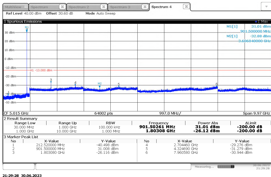
Figure 2.4.6-2 - Transmitter Conducted Spurious Emissions – KDS TCXO – 901.5 MHz - Normal Mode
