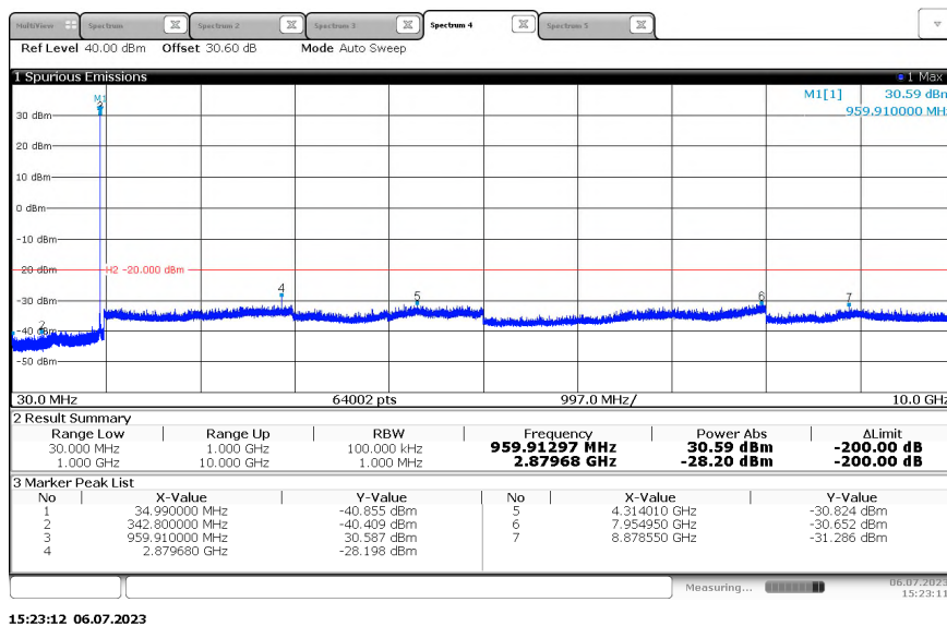
Figure 2.4.6-9 - Transmitter Conducted Spurious Emissions – KDS TCXO – 959.925 MHz - mPass5k Mode
