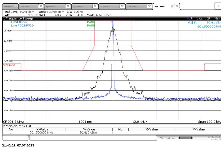
Figure 2.2.6-4 - Emissions Mask – KDS TCXO – 901.5 MHz - 25 kHz Channel Spacing- C&amp;I Mode
