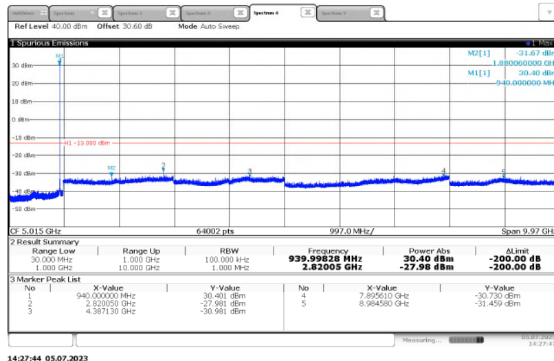
Figure 2.4.6-4 - Transmitter Conducted Spurious Emissions – KDS TCXO – 940.0125 MHz - mPass5k Mode
