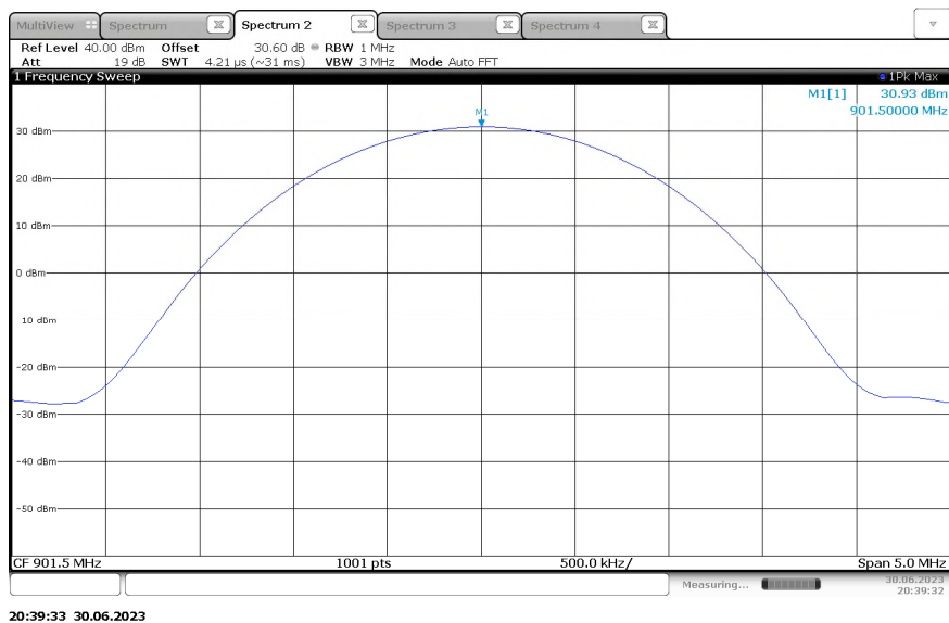
Figure 2.1.6-2 - RF Output Power – KDS TCXO – 901.5 MHz
