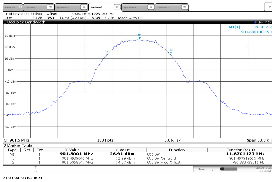
Figure 2.3.6-8 - 99% Bandwidth – KDS TCXO – 901.5 MHz - 2FSK Mode
