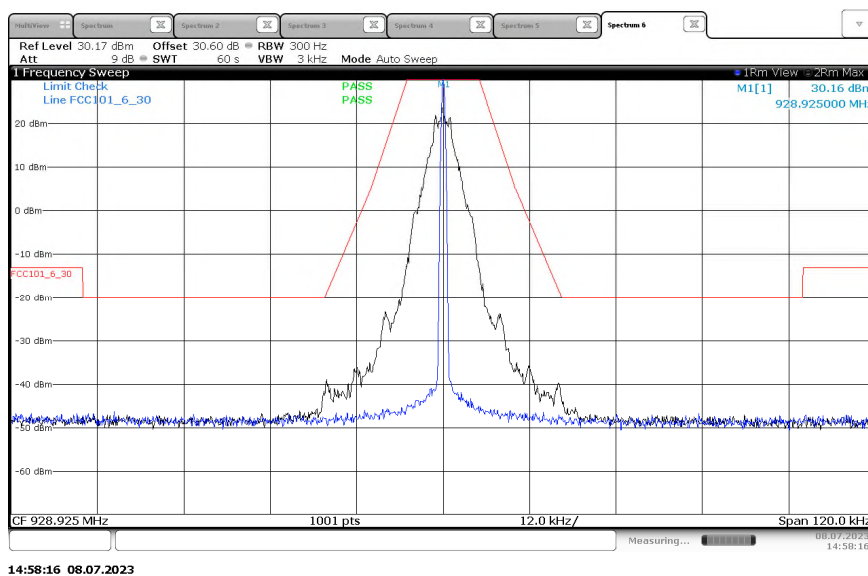
Figure 2.2.6-19 - Emissions Mask – KDS TCXO – 928.925 MHz - 25 kHz Channel Spacing- C&I Mode
