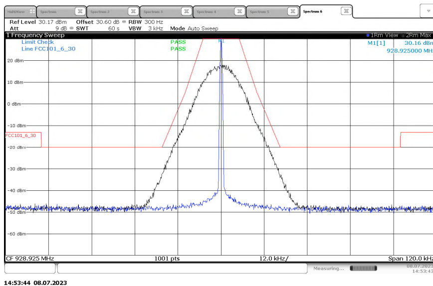
Figure 2.2.6-30 - Emissions Mask – KDS TCXO – 928.925 MHz - 25 kHz Channel Spacing- 8SFSK Mode
