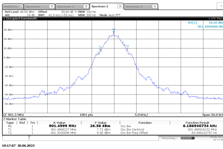
Figure 2.3.6-3 - 99% Bandwidth – KDS TCXO – 901.5 MHz - C&amp;I Mode
