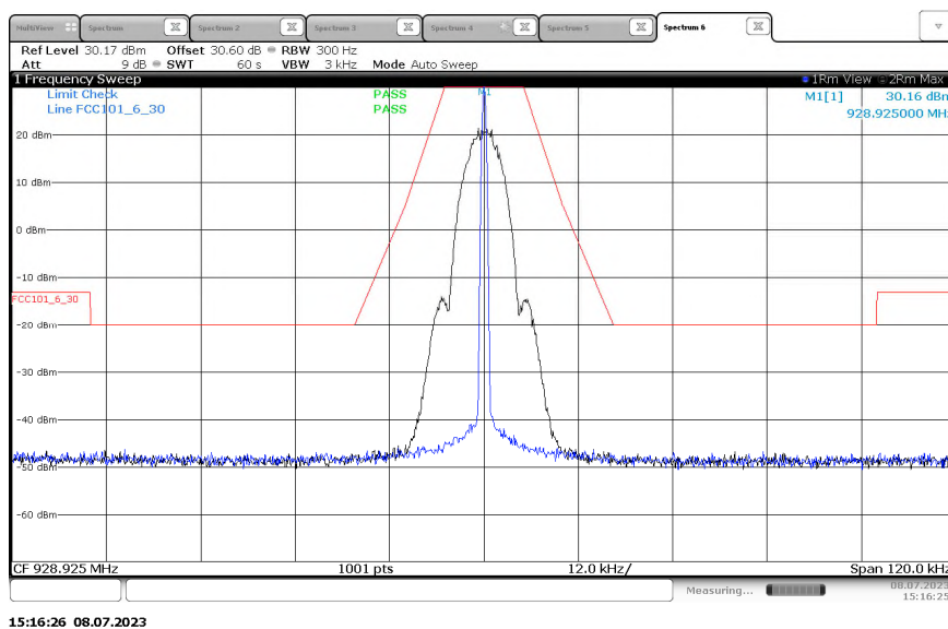
Figure 2.2.6-23 - Emissions Mask – KDS TCXO – 928.925 MHz - 25 kHz Channel Spacing- 2FSK (Half Baud) Mode
