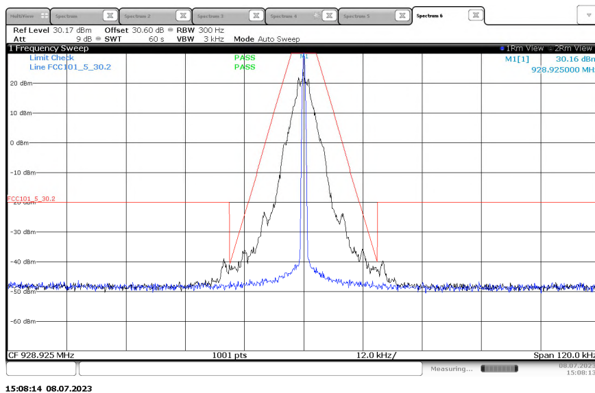
Figure 2.2.6-18 - Emissions Mask – KDS TCXO – 928.925 MHz - 12.5 kHz Channel Spacing - C&I Mode
