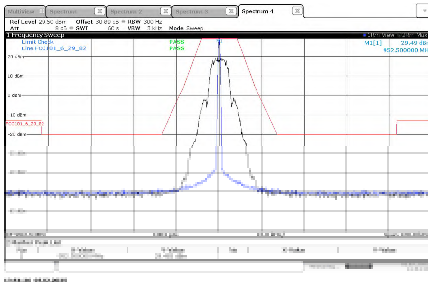
Figure 2.2.6-61 - Emissions Mask – TXC TCXO – 952.5 MHz - 25 kHz Channel Spacing- mPass5k Mode
