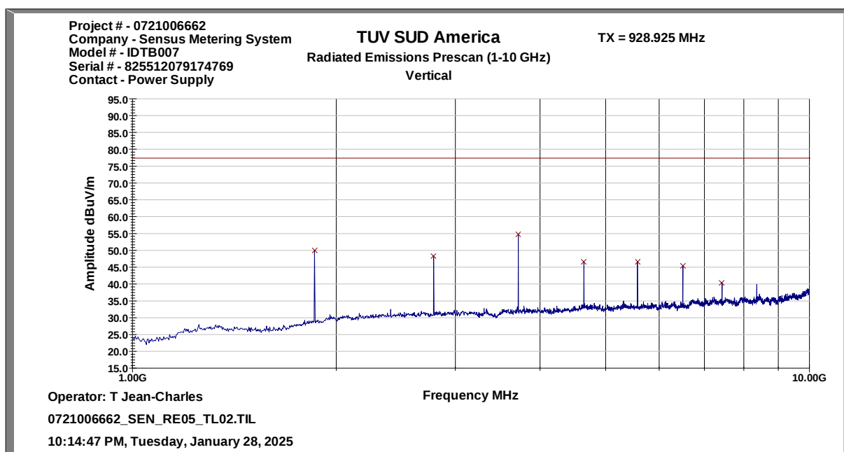
Figure 2.5.6-5 - Transmitter Radiated Spurious Emissions – TXC TCXO – 928.925 MHz - Normal Mode – 1 GHz – 10 GHz – Vertical Polarization
