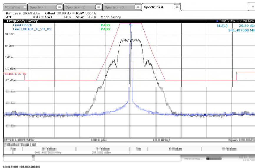
Figure 2.2.6-56 - Emissions Mask – TXC TCXO – 941.4875 MHz - 25 kHz Channel Spacing - mPass10k Mode
