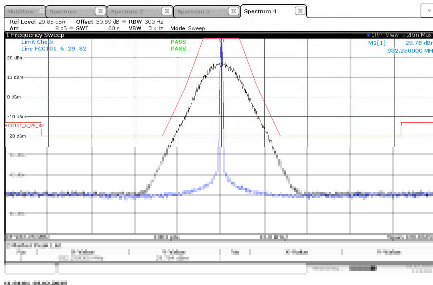
Figure 2.2.6-53 - Emissions Mask – TXC TCXO – 932.25 MHz - 25 kHz Channel Spacing- 8FSK Mode
