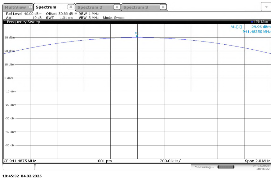
Figure 2.1.6-7 - RF Output Power – TXC TCXO – 941.4875 MHz
