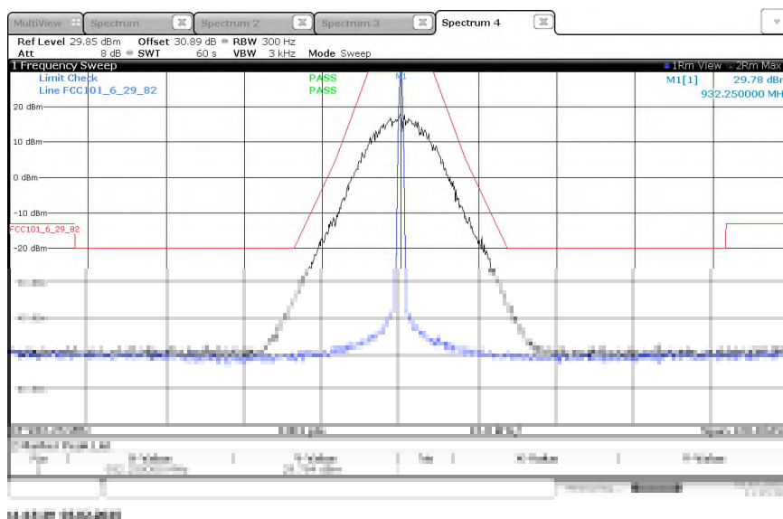
Figure 2.2.6-52 - Emissions Mask – TXC TCXO – 932.25 MHz - 25 kHz Channel Spacing- 4FSK Mode
