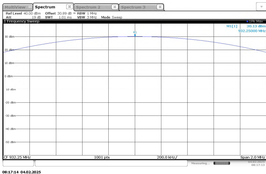
Figure 2.1.6-6 - RF Output Power – TXC TCXO – 932.25 MHz
