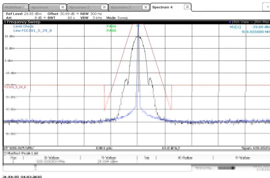
Figure 2.2.6-32 - Emissions Mask – TxC TCXO – 928.925 MHz - 12.5 kHz Channel Spacing - 2FSK (Half Baud) Mode
