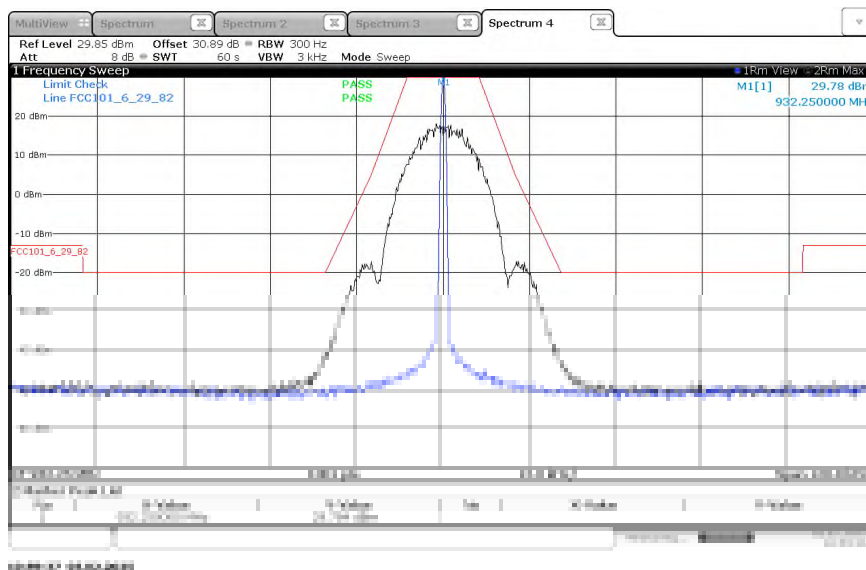
Figure 2.2.6-51 - Emissions Mask – TXC TCXO – 932.25 MHz - 25 kHz Channel Spacing- 2SFSK Mode
