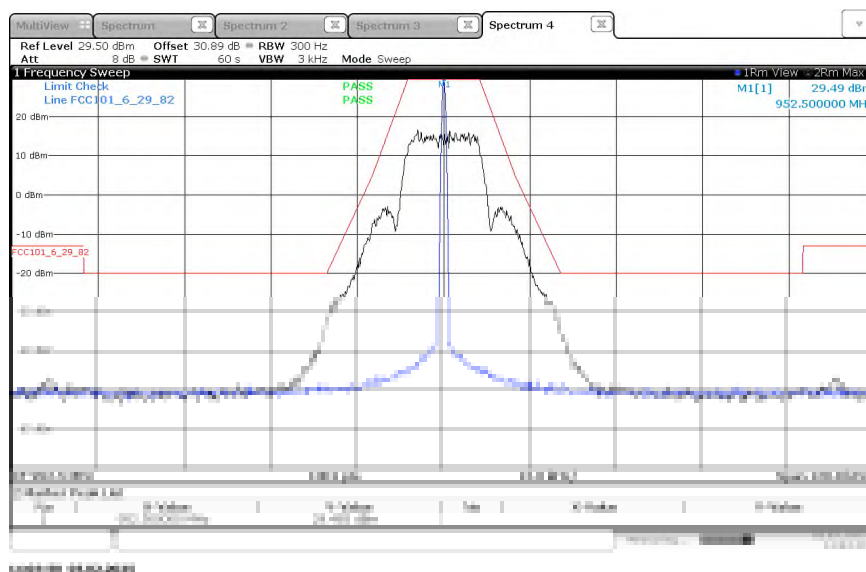
Figure 2.2.6-62 - Emissions Mask – TXC TCXO – 952.5 MHz - 25 kHz Channel Spacing - mPass10k Mode
