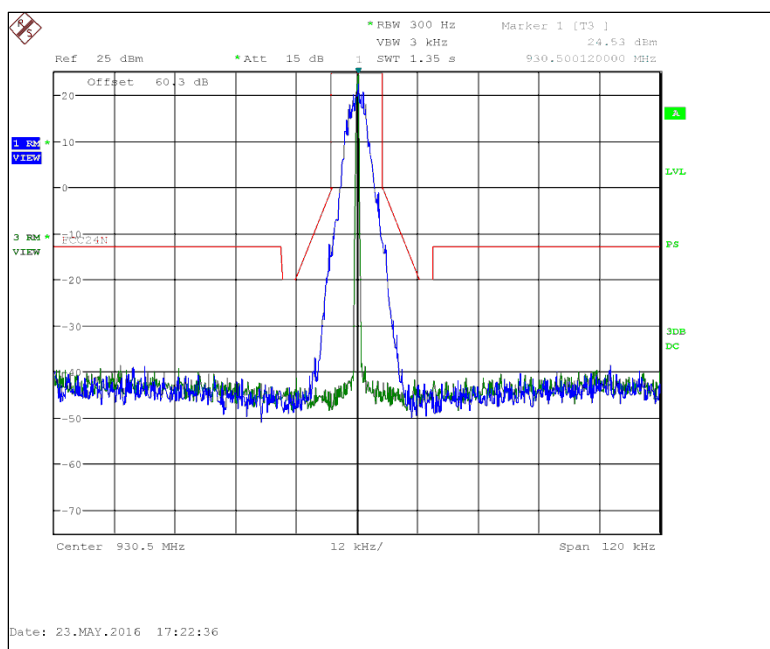
Figure 7.2.2-4: 930.5 MHz – 12.5 kHz Channel Spacing – mPass4 10k Mode
