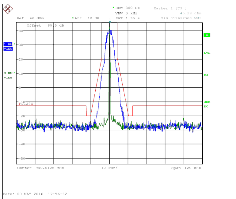
Figure 7.2.2-22: 940.0125 MHz – 12.5 kHz Channel Spacing – mPass4 10k Mode
