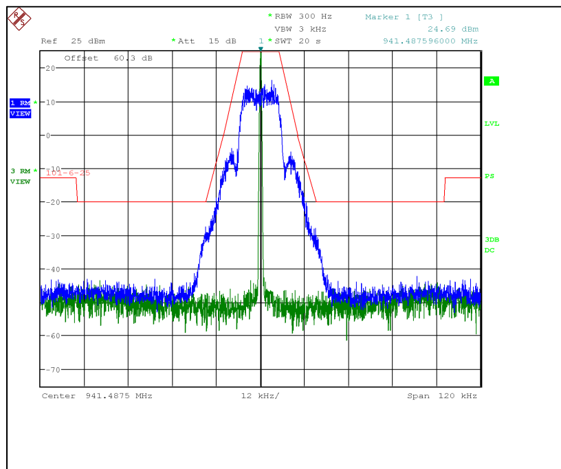
Figure 7.2.2-26: 941.4875 MHz – 25 kHz Channel Spacing – mPass2 10k Mode
