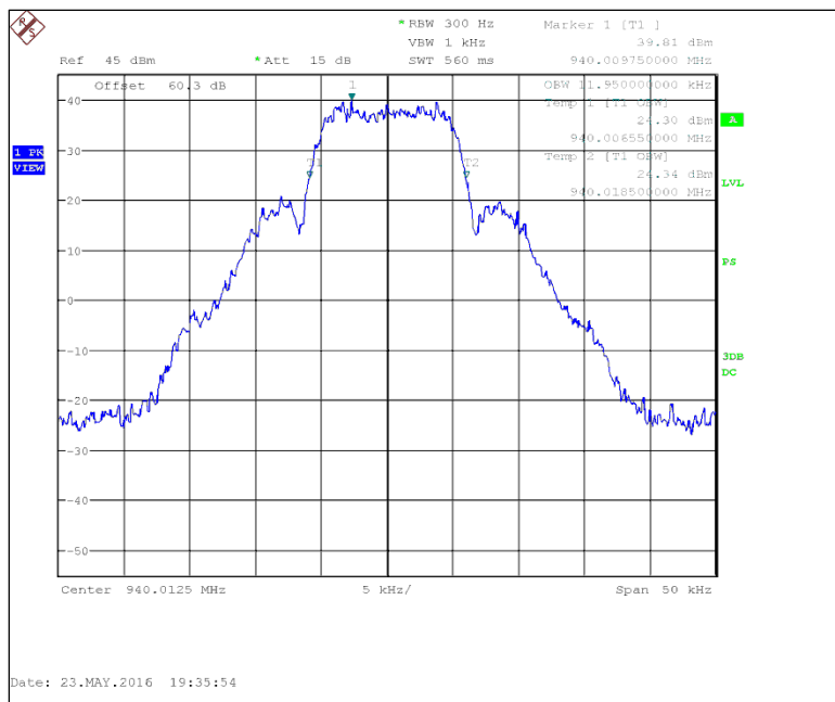
Figure 7.2.3-6: 940.0125 MHz – mPass2 10k
