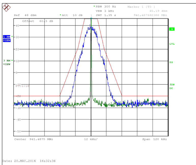
Figure 7.2.2-32: 941.4875 MHz – 25 kHz Channel Spacing – mPass4 20k Mode
