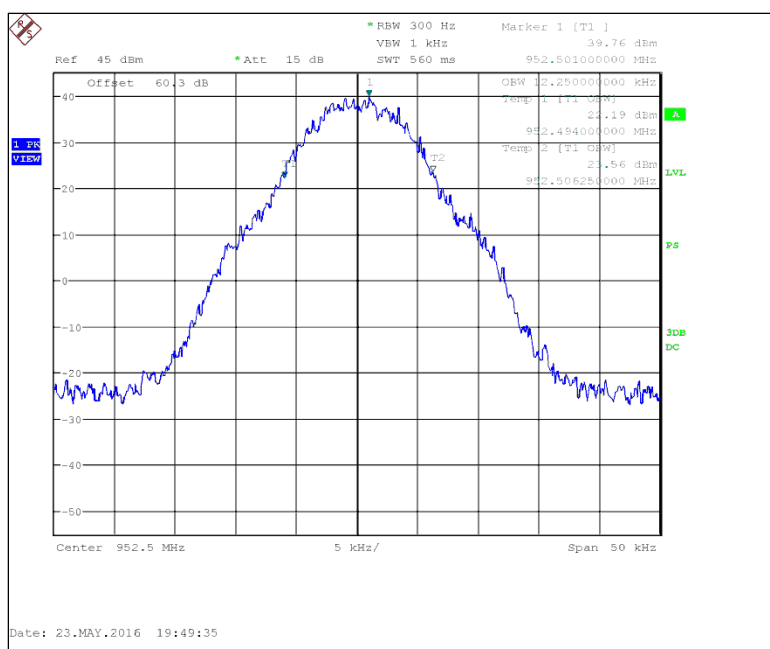
Figure 7.2.3-16: 952.5 MHz – mPass4 20k
