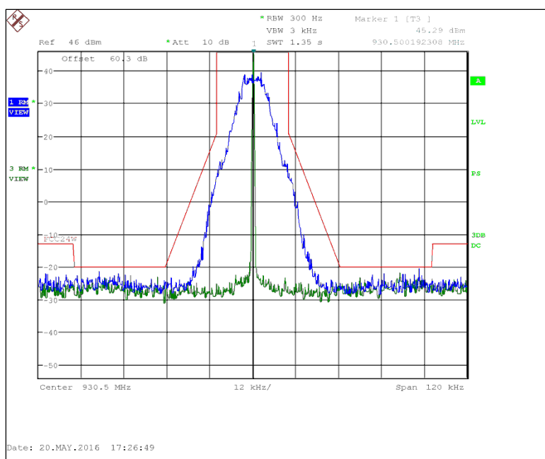
Figure 7.2.2-12: 930.5 MHz – 25 kHz Channel Spacing – mPass4 20k Mode
