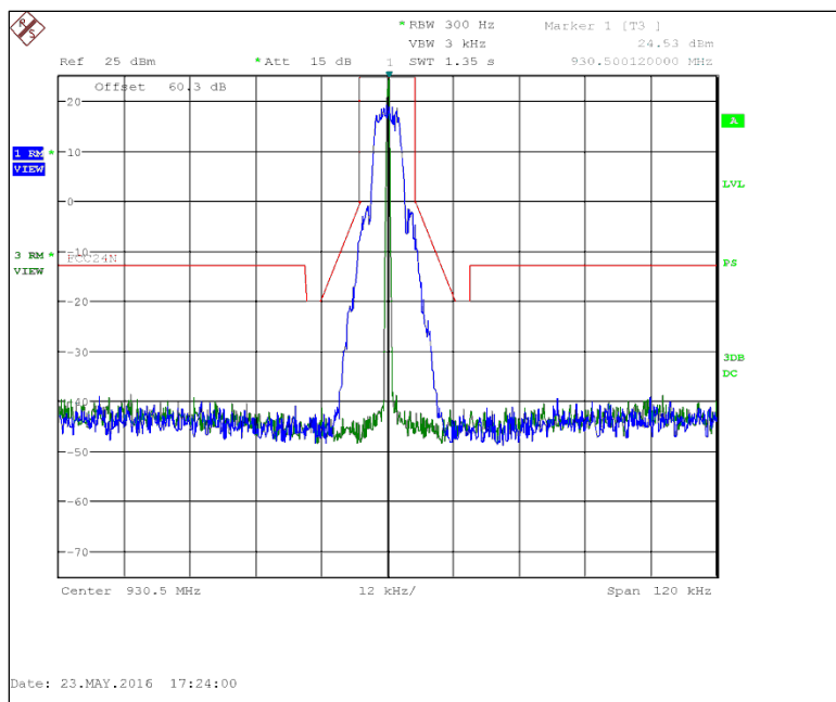
Figure 7.2.2-1: 930.5 MHz – 12.5 kHz Channel Spacing – mPass 5k Mode
