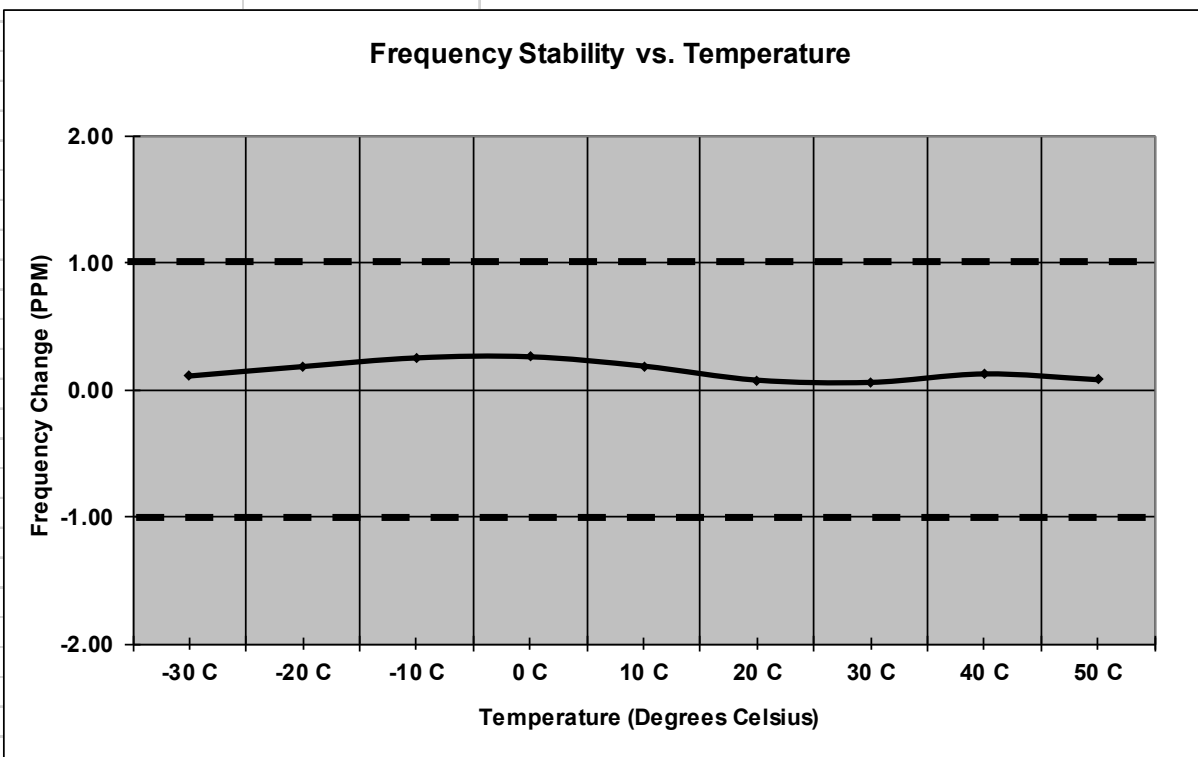
Figure 7.5.2-1: Frequency Stability – 930.5 MHz
