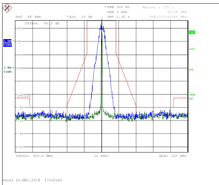
Figure 7.2.2-11: 930.5 MHz – 25 kHz Channel Spacing – mPass4 10k Mode
