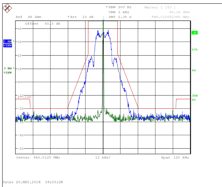
Figure 7.2.2-21: 940.0125 MHz – 25 kHz Channel Spacing – mPass2 10k Mode
