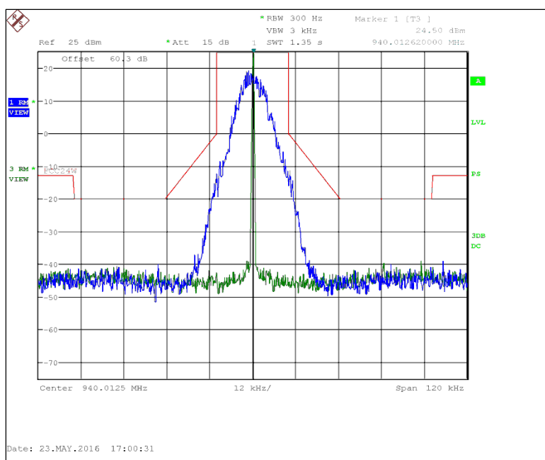
Figure 7.2.2-18: 940.0125 MHz – 25 kHz Channel Spacing – mPass4 20k Mode
