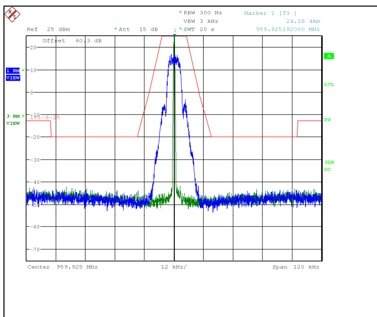
Figure 7.2.2-41: 959.925 MHz – 25 kHz Channel Spacing – mPass 5k Mode
