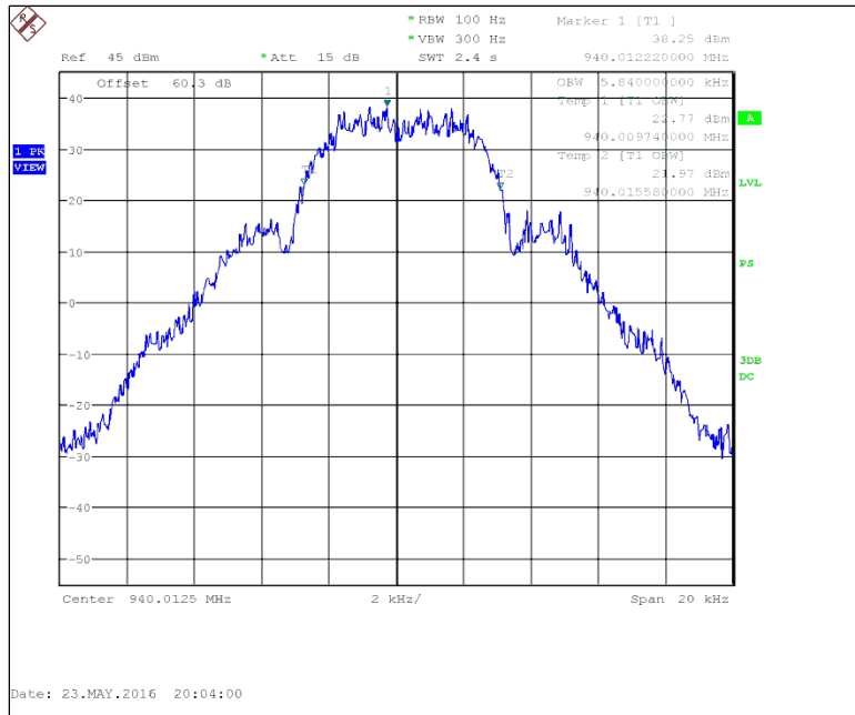
Figure 7.2.3-5: 940.0125 MHz – mPass 5k
