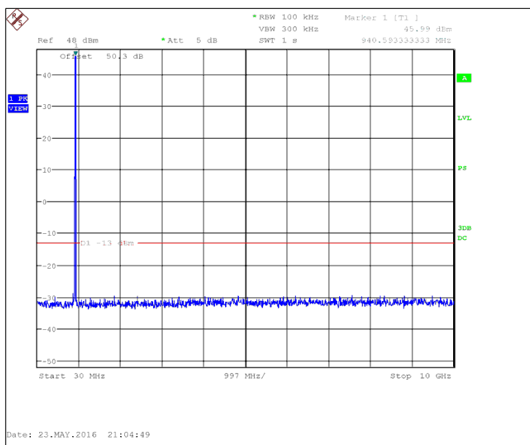
Figure 7.3.2-4: 940.0125 MHz – 30 MHz to 10 GHz – mPass 5k
