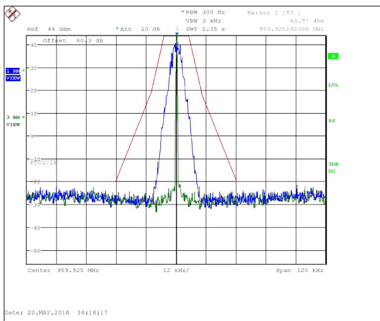
Figure 7.2.2-47: 959.925 MHz – 25 kHz Channel Spacing – mPass4 10k Mode
