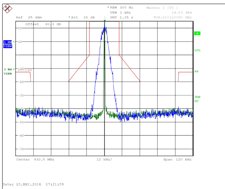
Figure 7.2.2-5: 930.5 MHz – 25 kHz Channel Spacing – mPass4 10k Mode
