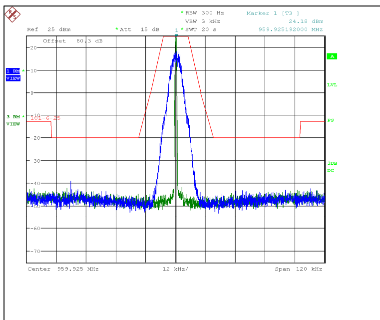
Figure 7.2.2-43: 959.925 MHz – 25 kHz Channel Spacing – mPass4 10k Mode
