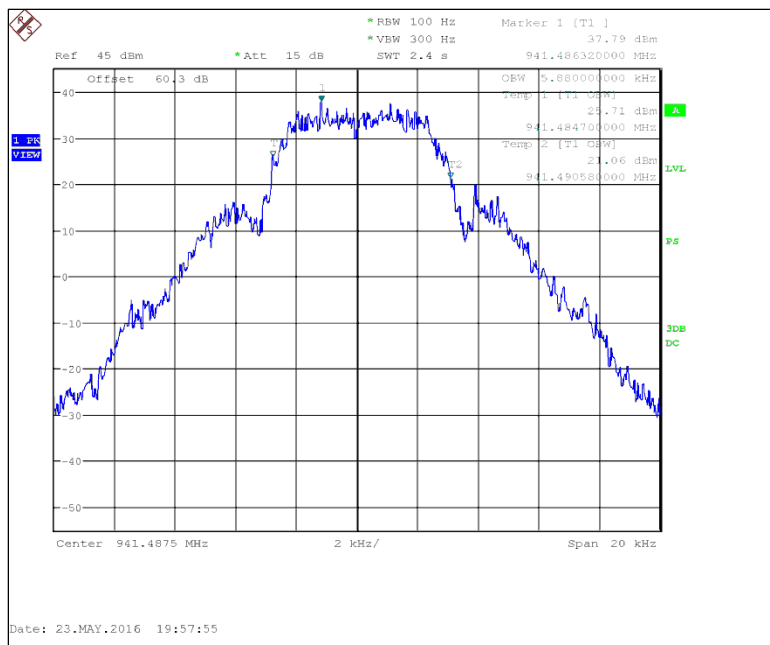
Figure 7.2.3-9: 941.4875 MHz – mPass 5k
