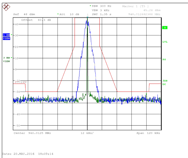
Figure 7.2.2-23: 940.0125 MHz – 25 kHz Channel Spacing – mPass4 10k Mode
