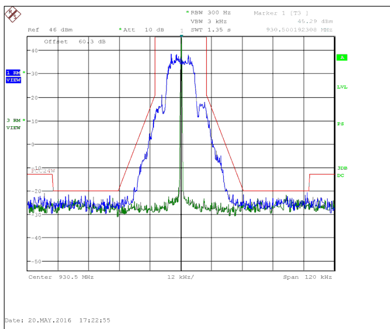
Figure 7.2.2-9: 930.5 MHz – 25 kHz Channel Spacing – mPass2 10k Mode
