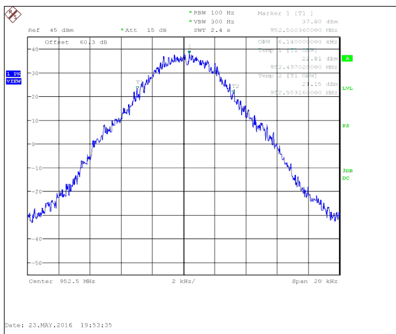
Figure 7.2.3-15: 952.5 MHz – mPass4 10k
