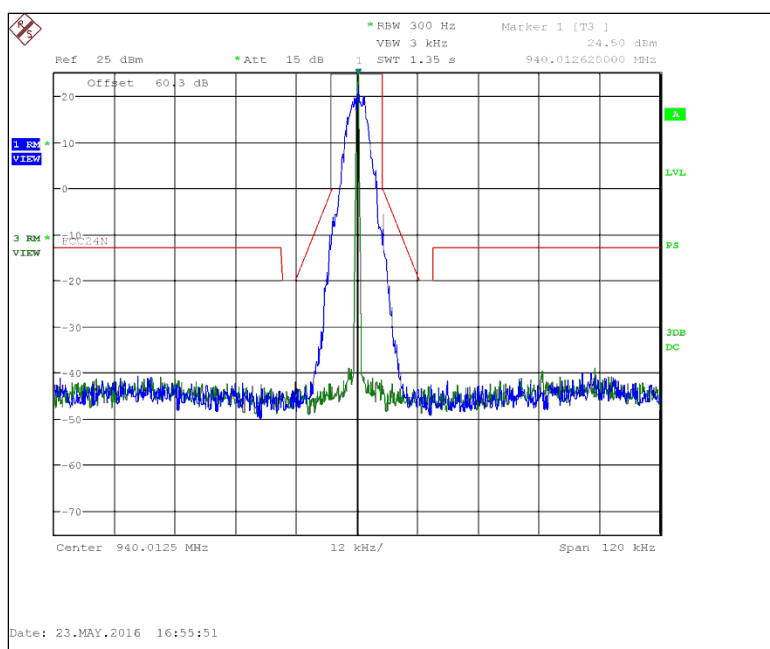
Figure 7.2.2-16: 940.0125 MHz – 12.5 kHz Channel Spacing – mPass4 10k Mode
