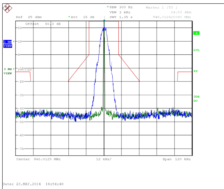
Figure 7.2.2-17: 940.0125 MHz – 25 kHz Channel Spacing – mPass4 10k Mode
