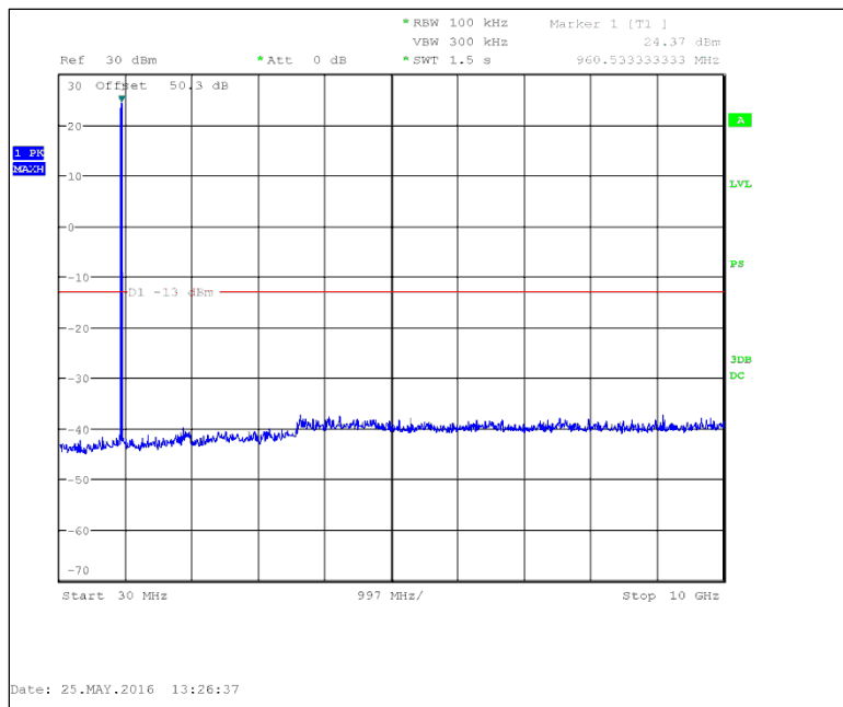
Figure 7.3.2-7: 959.925 MHz – 30 MHz to 10 GHz – mPass 5k
