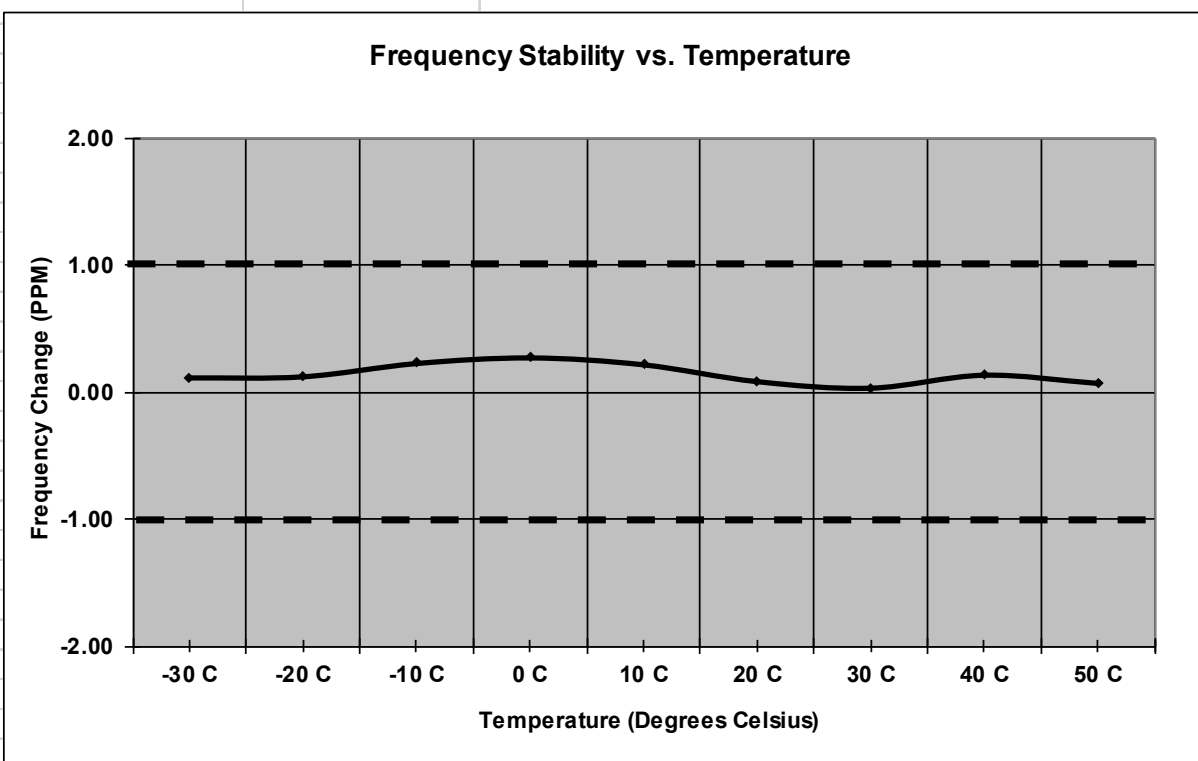
Figure 7.5.2-3: Frequency Stability – 959.925 MHz
