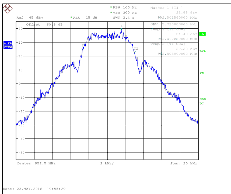
Figure 7.2.3-13: 952.5 MHz – mPass 5k
