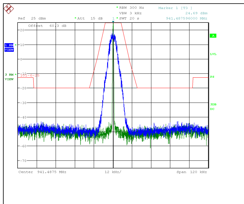
Figure 7.2.2-27: 941.4875 MHz – 25 kHz Channel Spacing – mPass4 10k Mode
