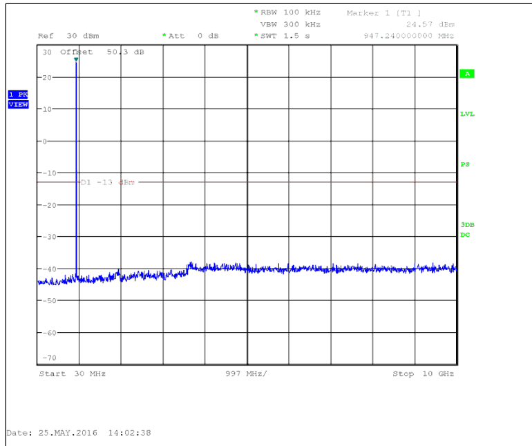
Figure 7.3.2-6: 952.5 MHz – 30 MHz to 10 GHz – mPass 5k
