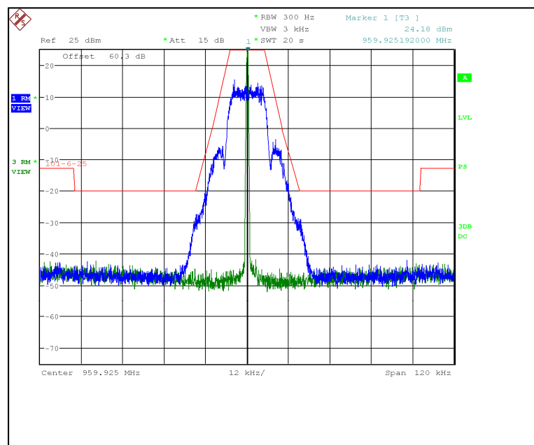
Figure 7.2.2-42: 959.925 MHz – 25 kHz Channel Spacing – mPass2 10k Mode
