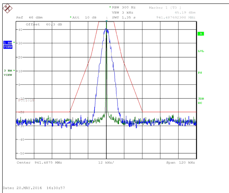
Figure 7.2.2-31: 941.4875 MHz – 25 kHz Channel Spacing – mPass4 10k Mode
