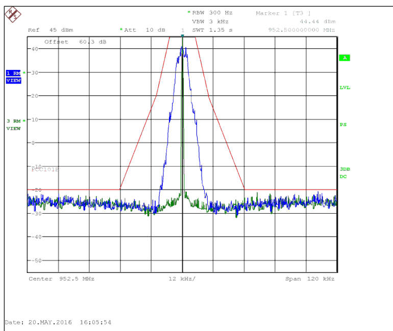
Figure 7.2.2-39: 952.5 MHz – 25 kHz Channel Spacing – mPass4 10k Mode
