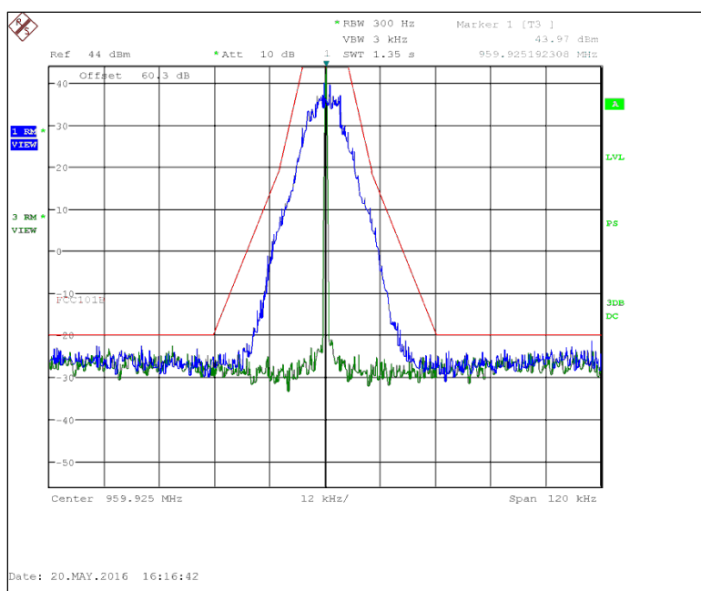
Figure 7.2.2-48: 959.925 MHz – 25 kHz Channel Spacing – mPass4 20k Mode
