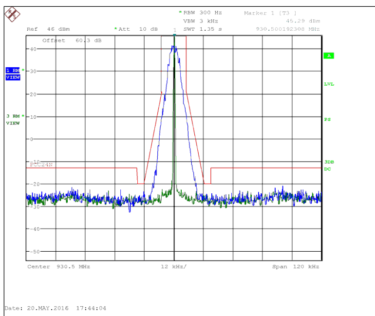
Figure 7.2.2-10: 930.5 MHz – 12.5 kHz Channel Spacing – mPass4 10k Mode
