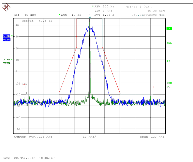
Figure 7.2.2-24: 940.0125 MHz – 25 kHz Channel Spacing – mPass4 20k Mode
