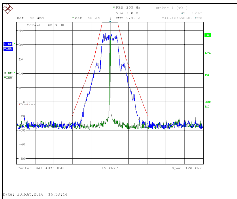
Figure 7.2.2-30: 941.4875 MHz – 25 kHz Channel Spacing – mPass2 10k Mode
