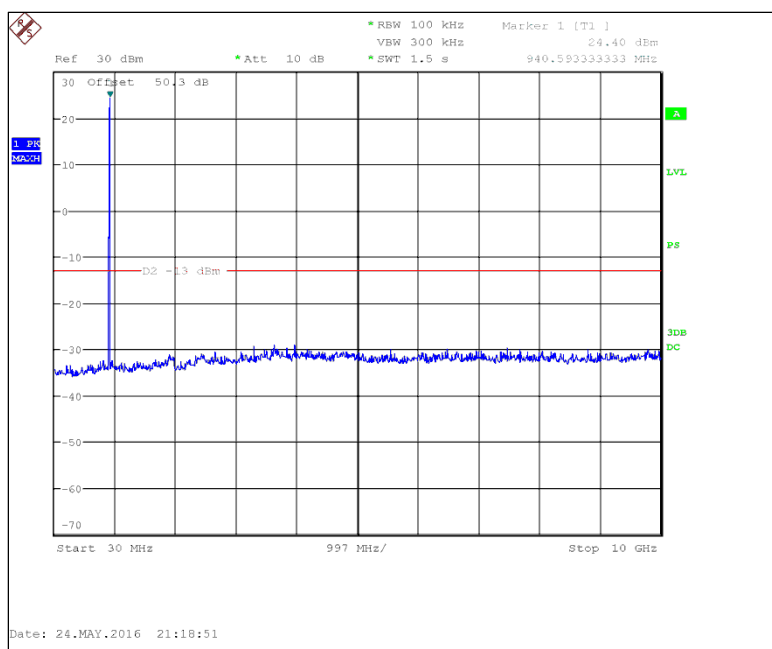
Figure 7.3.2-2: 940.0125 MHz – 30 MHz to 10 GHz – mPass 5k
