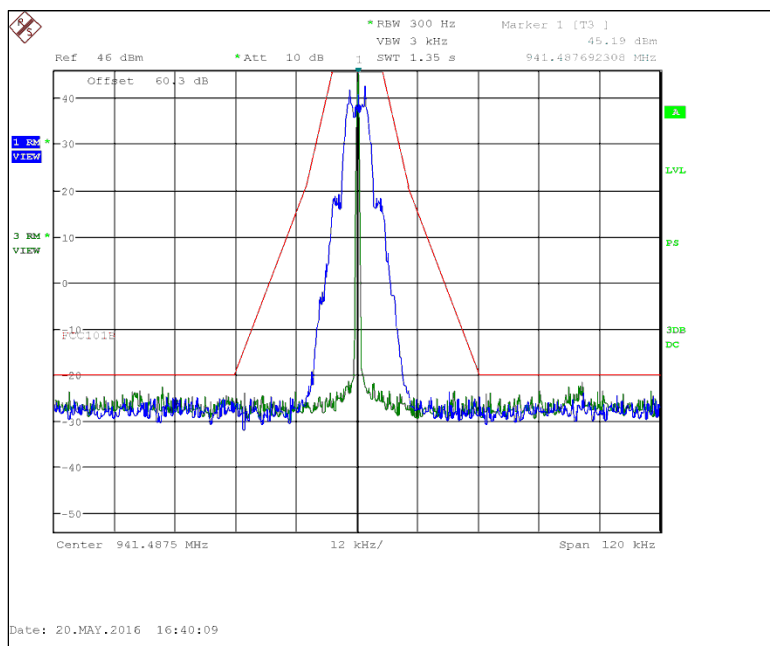
Figure 7.2.2-29: 941.4875 MHz – 25 kHz Channel Spacing – mPass 5k Mode
