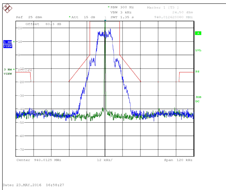
Figure 7.2.2-15: 940.0125 MHz – 25 kHz Channel Spacing – mPass2 10k Mode
