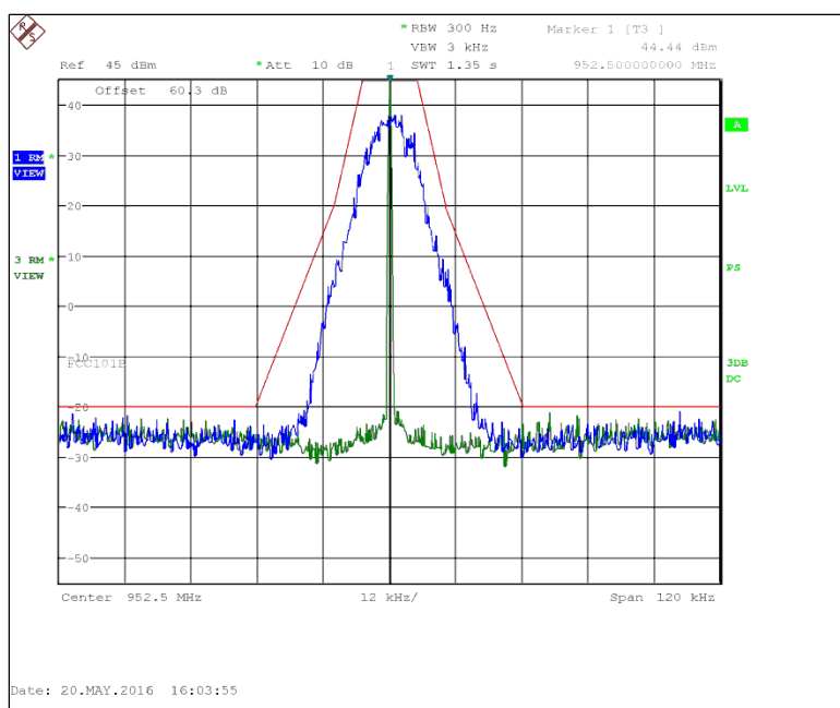
Figure 7.2.2-40: 952.5 MHz – 25 kHz Channel Spacing – mPass4 20k Mode
