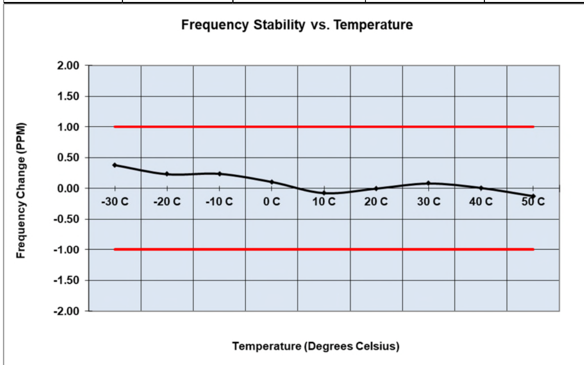
Figure 2.6.6-5: Frequency Stability – 941.4875 MHz – High Power
