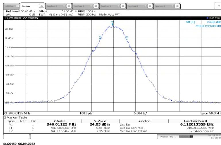
Figure 2.3.6-27: 99% Bandwidth – 940.0125 MHz - m4Pass – Low Power
