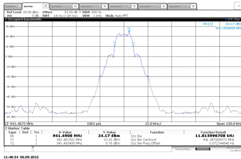
Figure 2.3.6-30: 99% Bandwidth – 941.4875 MHz - mPass2 – Low Power
