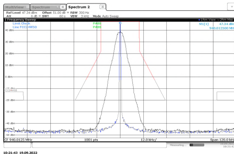
Figure 2.2.6-11: Emissions Mask – 940.0125 MHz - 25 kHz Channel Spacing- m4Pass Mode – High Power
