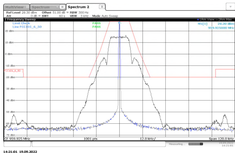
Figure 2.2.6-46: Emissions Mask – 959.925 MHz - 25 kHz Channel Spacing- mPass2 Mode – Low Power
