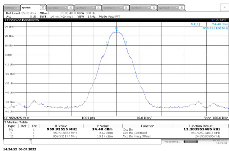
Figure 2.3.6-40: 99% Bandwidth – 959.925 MHz - m4Pass2 – Low Power
