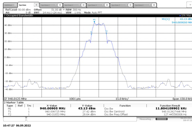
Figure 2.3.6-6: 99% Bandwidth – 940.0125 MHz - mPass2 – High Power
