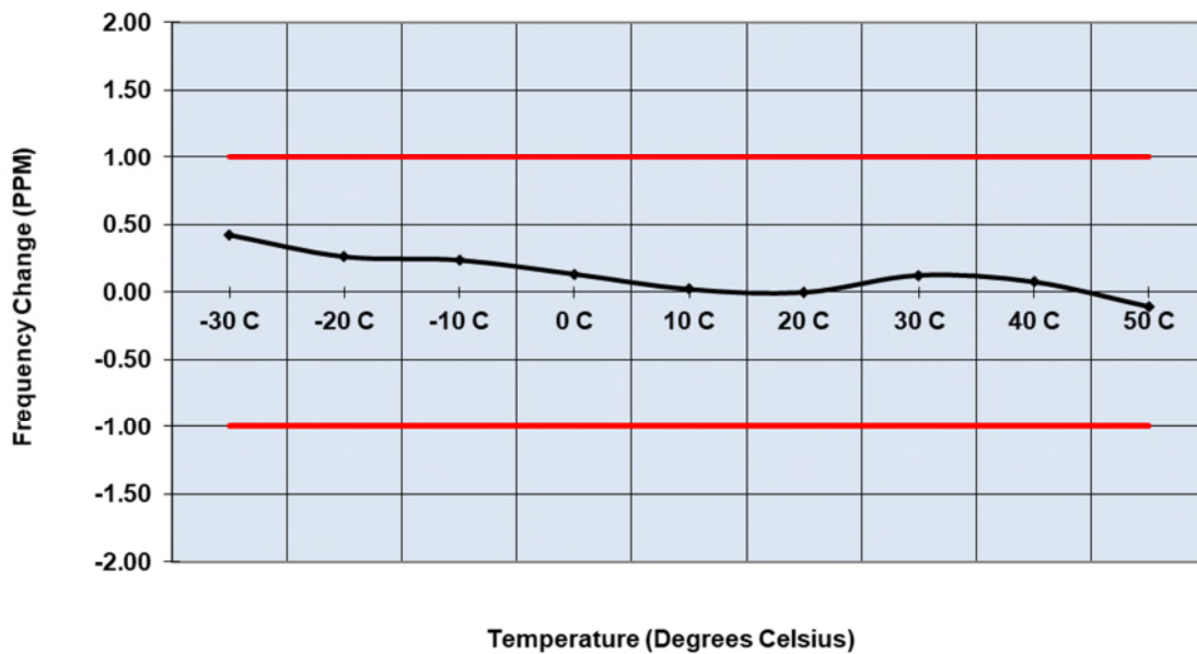
Figure 2.6.6-6: Frequency Stability – 952.5 MHz – High Power
