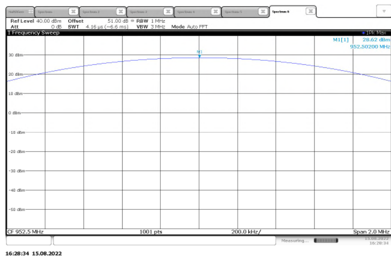
Figure 2.1.6-9: RF Output Power – 952.5 MHz – Low Power
