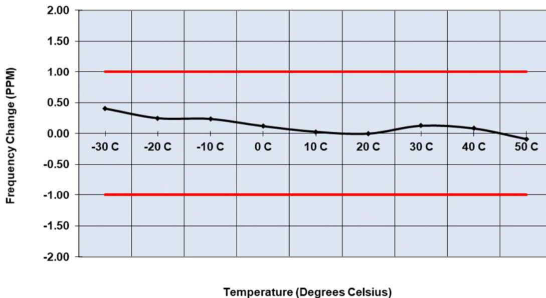
Figure 2.6.6-7: Frequency Stability – 959.925 MHz – High Power
