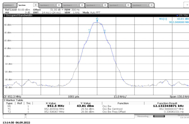
Figure 2.3.6-16: 99% Bandwidth – 952.5 MHz - m4Pass2 – High Power
