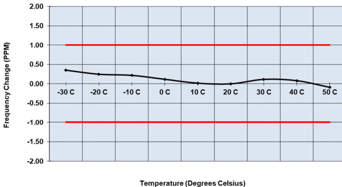
Figure 2.6.6-10: Frequency Stability – 959.925 MHz – Low Power
