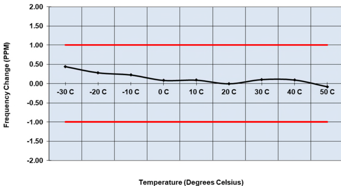
Figure 2.6.6-1: Frequency Stability – 930.5 MHz – High Power
