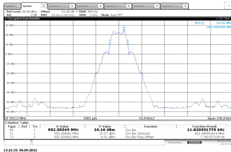
Figure 2.3.6-34: 99% Bandwidth – 952.5 MHz - mPass2 – Low Power
