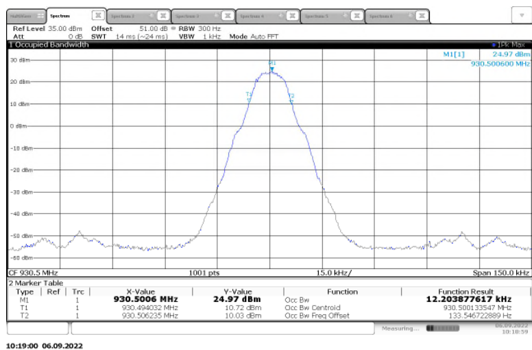
Figure 2.3.6-24: 99% Bandwidth – 930.5 MHz - m4Pass2 – Low Power
