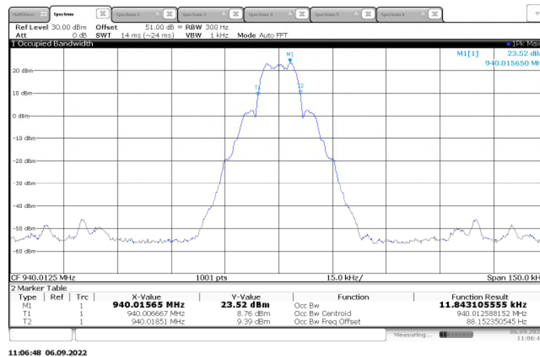
Figure 2.3.6-26: 99% Bandwidth – 940.0125 MHz - mPass2 – Low Power
