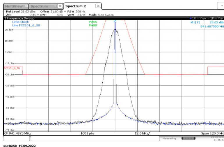
Figure 2.2.6-39: Emissions Mask – 941.4875 MHz - 25 kHz Channel Spacing- m4Pass Mode – Low Power
