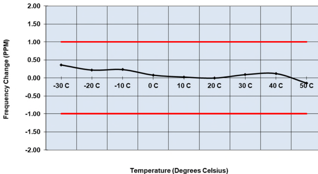
Figure 2.6.6-4: Frequency Stability – 940.0125 MHz – Low Power
