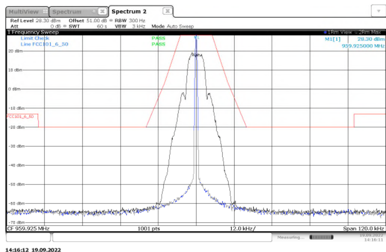
Figure 2.2.6-45: Emissions Mask – 959.925 MHz - 25 kHz Channel Spacing- mPass Mode – Low Power
