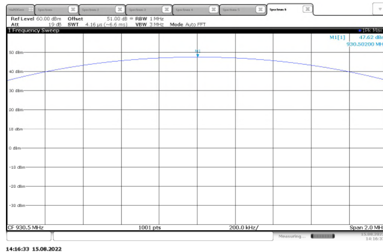
Figure 2.1.6-1: RF Output Power – 930.5 MHz – High Power
