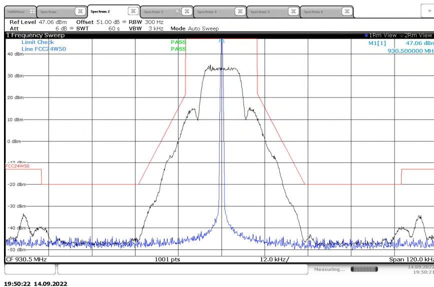
Figure 2.2.6-3: Emissions Mask – 930.5 MHz - 25 kHz Channel Spacing- mPass2 Mode – High Power
