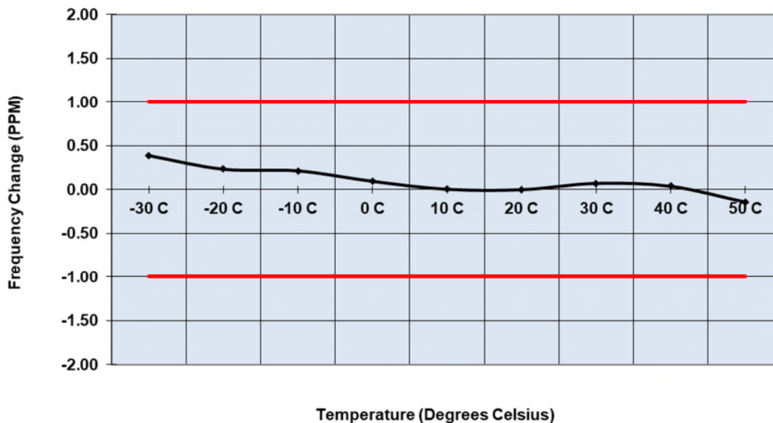
Figure 2.6.6-8: Frequency Stability – 941.4875 MHz – Low Power
