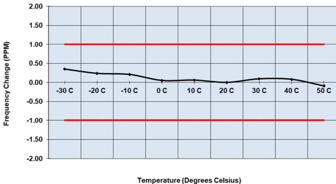
Figure 2.6.6-3: Frequency Stability – 930.5 MHz – Low Power
