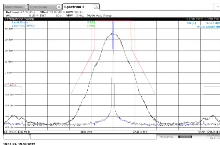
Figure 2.2.6-12: Emissions Mask – 940.0125 MHz - 25 kHz Channel Spacing- m4Pass2 Mode – High Power
