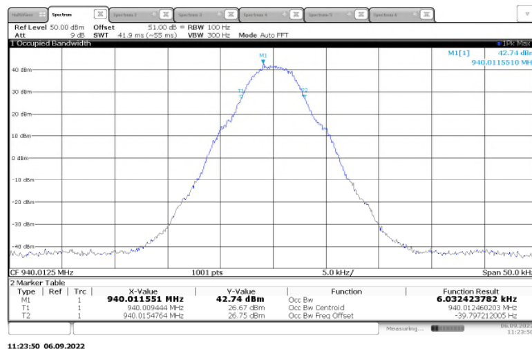
Figure 2.3.6-7: 99% Bandwidth – 940.0125 MHz - m4Pass – High Power
