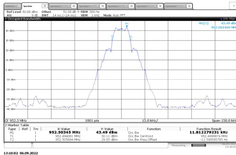
Figure 2.3.6-14: 99% Bandwidth – 952.5 MHz - mPass2 – High Power
