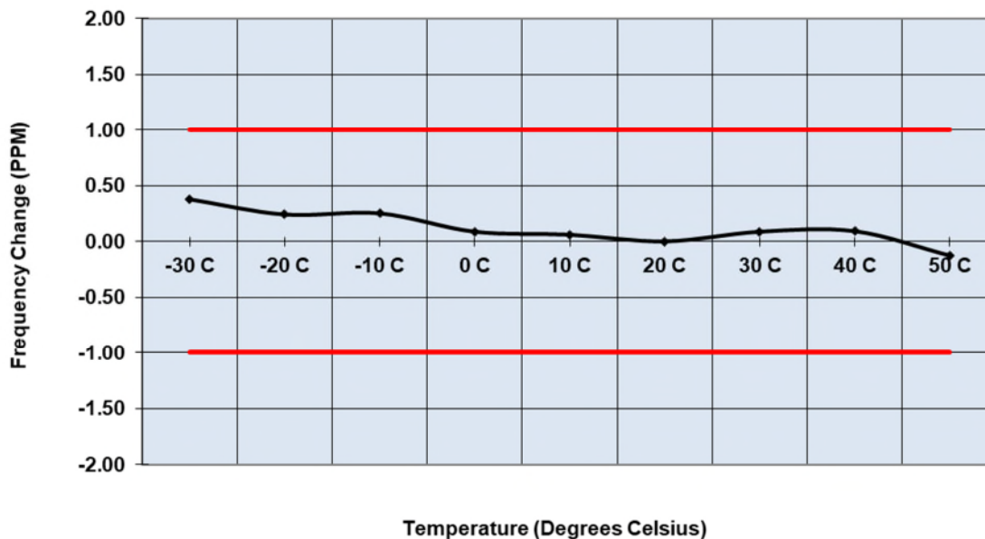
Figure 2.6.6-2: Frequency Stability – 940.0125 MHz – High Power
