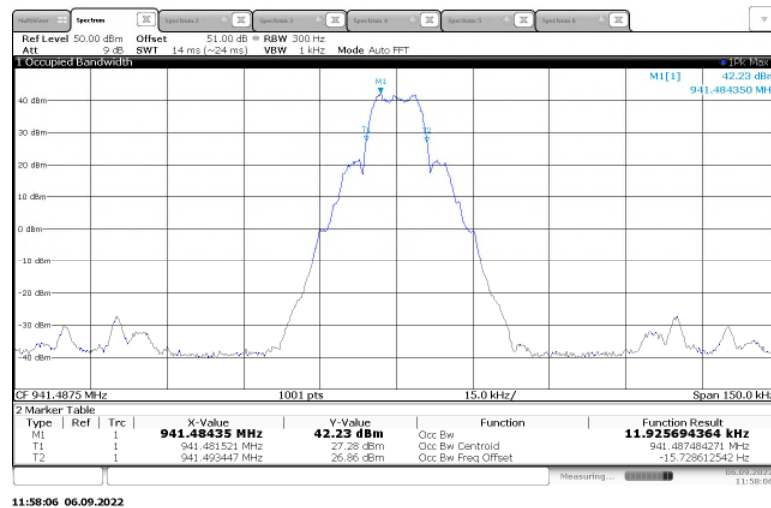
Figure 2.3.6-10: 99% Bandwidth – 941.4875 MHz - mPass2 – High Power
