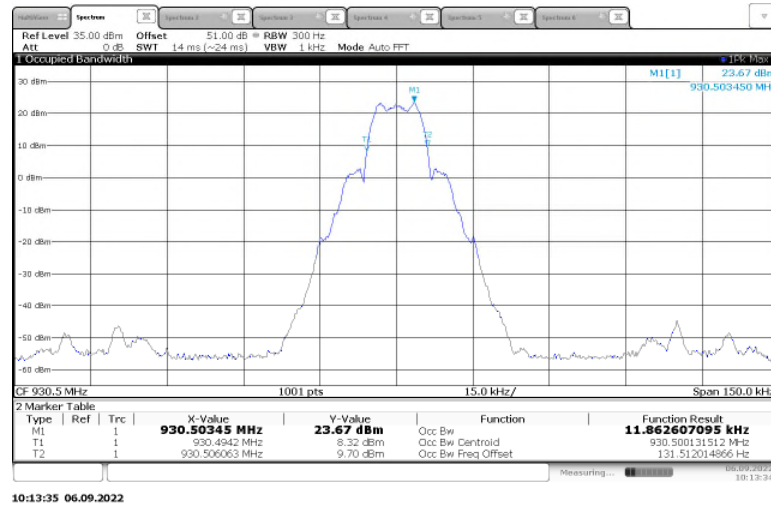
Figure 2.3.6-22: 99% Bandwidth – 930.5 MHz - mPass2 – Low Power
