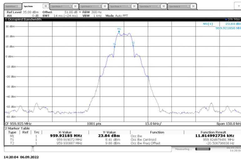
Figure 2.3.6-38: 99% Bandwidth – 959.925 MHz - mPass2 – Low Power
