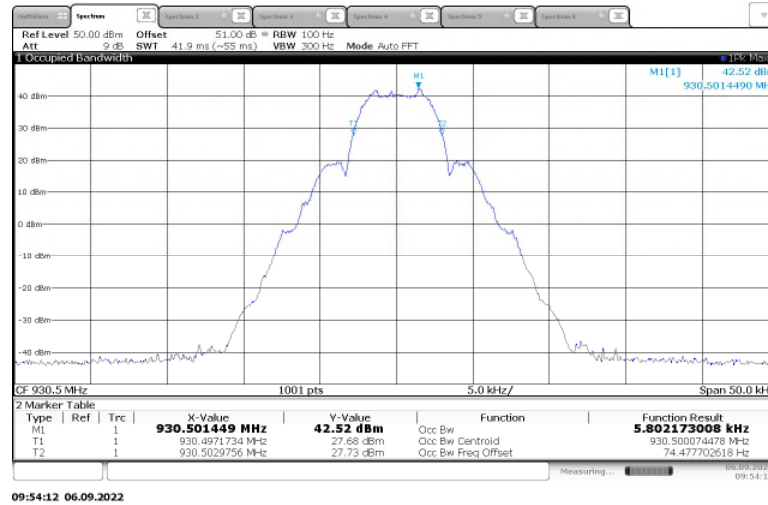
Figure 2.3.6-1: 99% Bandwidth – 930.5 MHz - mPass – High Power
