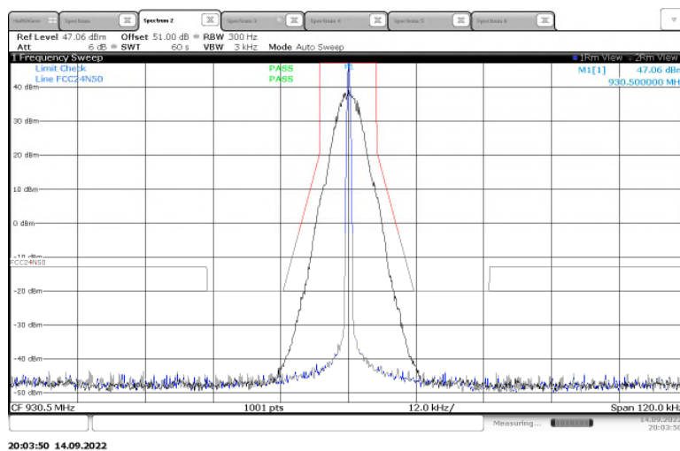
Figure 2.2.6-4: Emissions Mask – 930.5 MHz - 12.5 kHz Channel Spacing - m4Pass Mode – High Power
