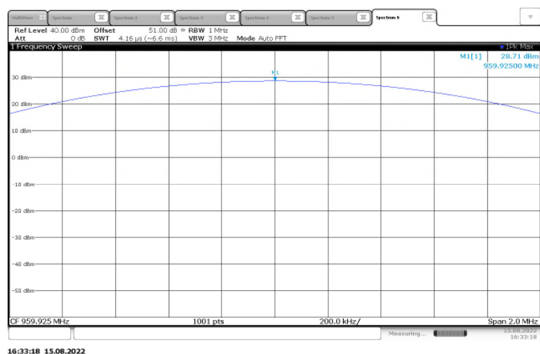
Figure 2.1.6-10: RF Output Power – 959.925 MHz – Low Power
