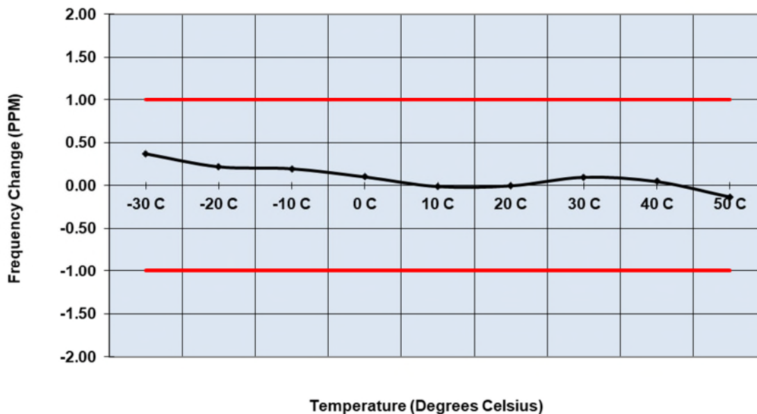
Figure 2.6.6-9: Frequency Stability – 952.5 MHz – Low Power
