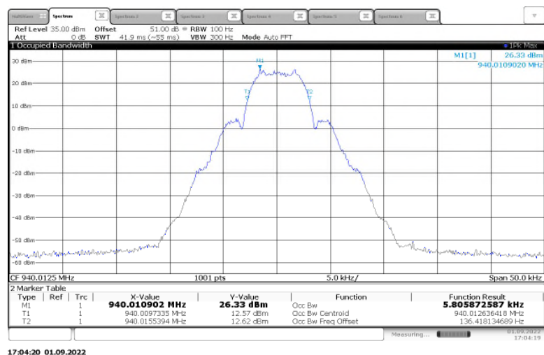
Figure 2.3.6-25: 99% Bandwidth – 940.0125 MHz - mPass – Low Power
