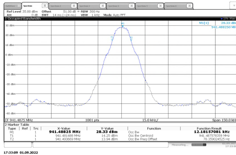
Figure 2.3.6-32: 99% Bandwidth – 941.4875 MHz - m4Pass2 – Low Power
