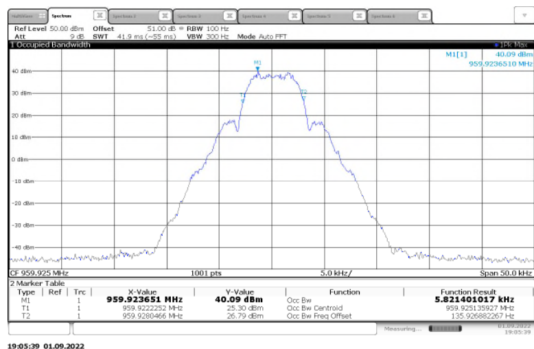
Figure 2.3.6-17: 99% Bandwidth – 959.925 MHz - mPass – High Power
