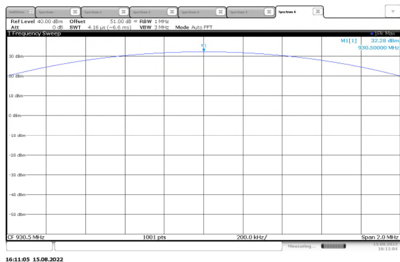
Figure 2.1.6-3: RF Output Power – 930.5 MHz – Low Power
