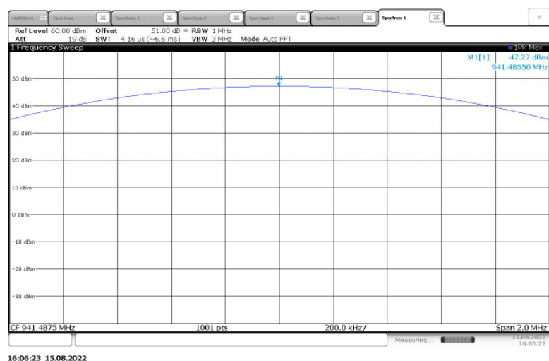
Figure 2.1.6-5: RF Output Power – 941.4875 MHz – High Power
