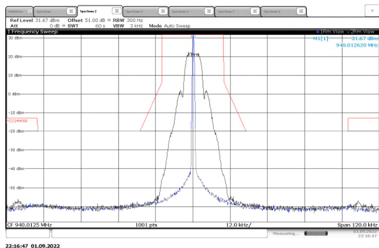
Figure 2.2.6-20: Emissions Mask – 940.0125 MHz - 25 kHz Channel Spacing- mPass Mode – Low Power
