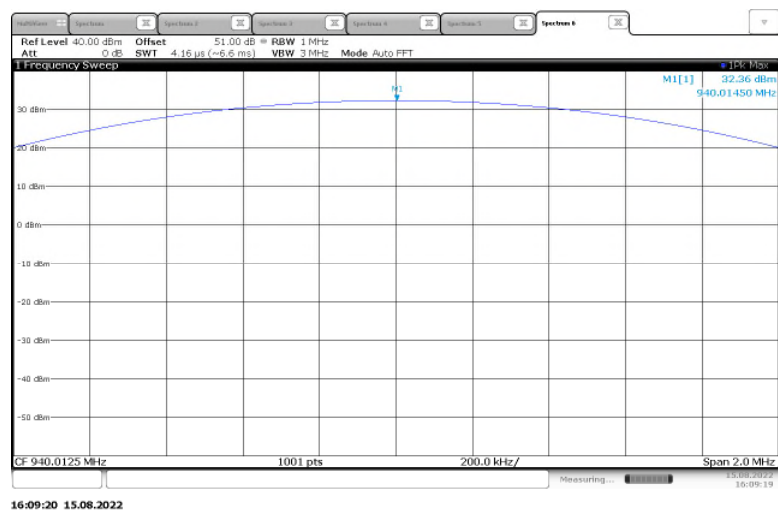
Figure 2.1.6-4: RF Output Power – 940.0125 MHz – Low Power
