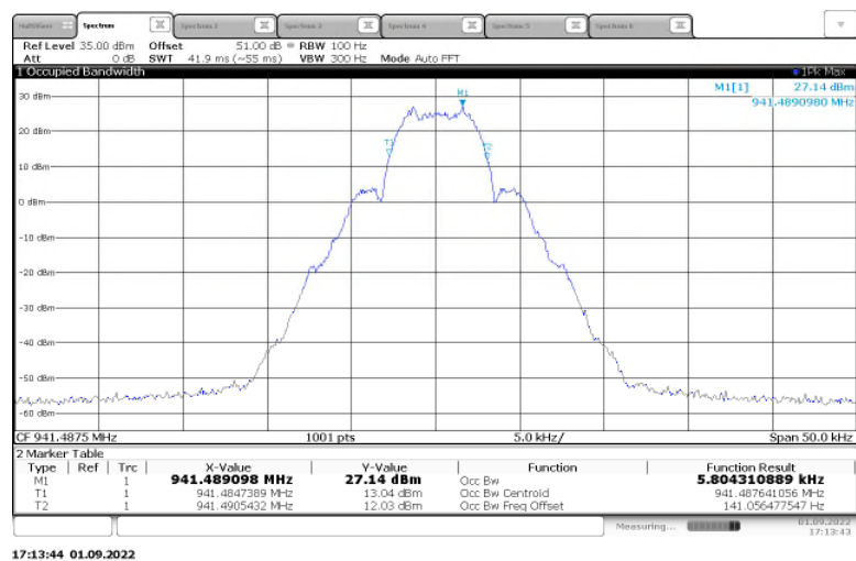
Figure 2.3.6-29: 99% Bandwidth – 941.4875 MHz - mPass – Low Power
