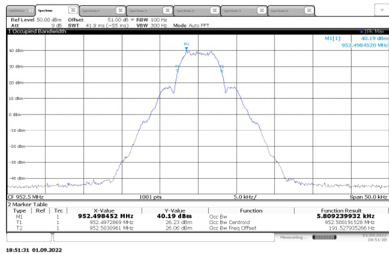
Figure 2.3.6-13: 99% Bandwidth – 952.5 MHz - mPass – High Power
