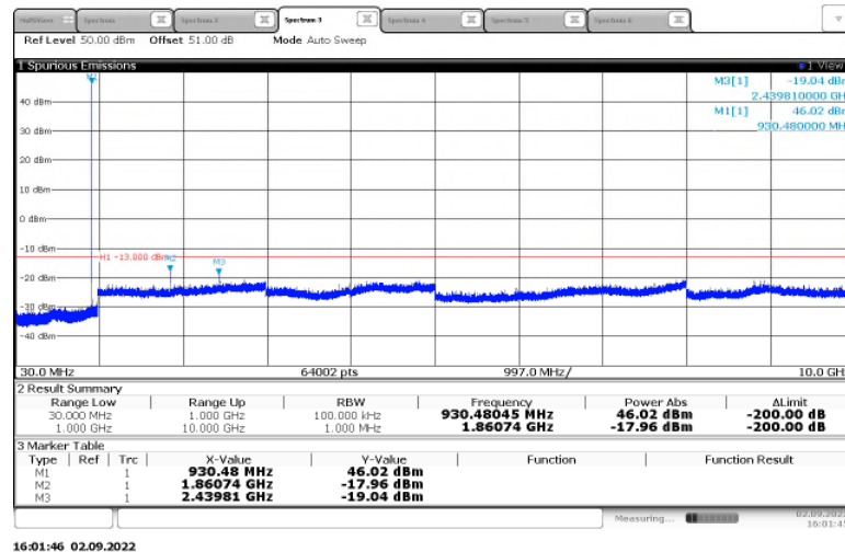
Figure 2.4.6-1: Transmitter Conducted Spurious Emissions – 930.5 MHz - mPass5k Mode – High Power
