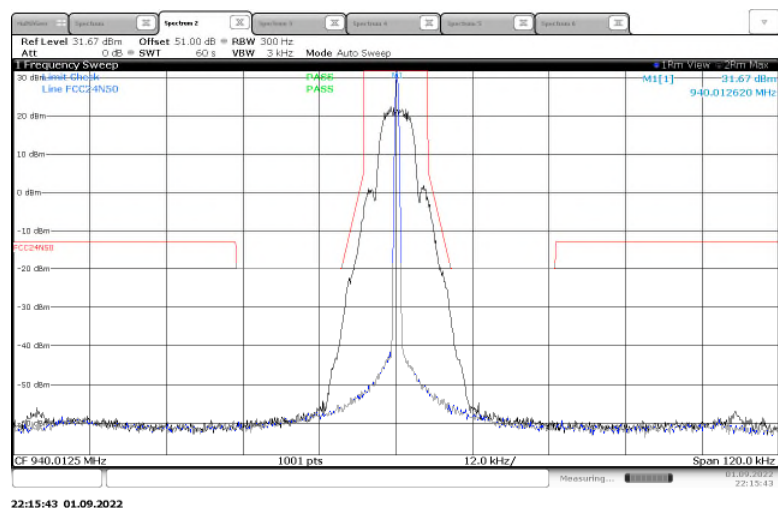
Figure 2.2.6-19: Emissions Mask – 940.0125 MHz - 12.5 kHz Channel Spacing - mPass Mode – Low Power
