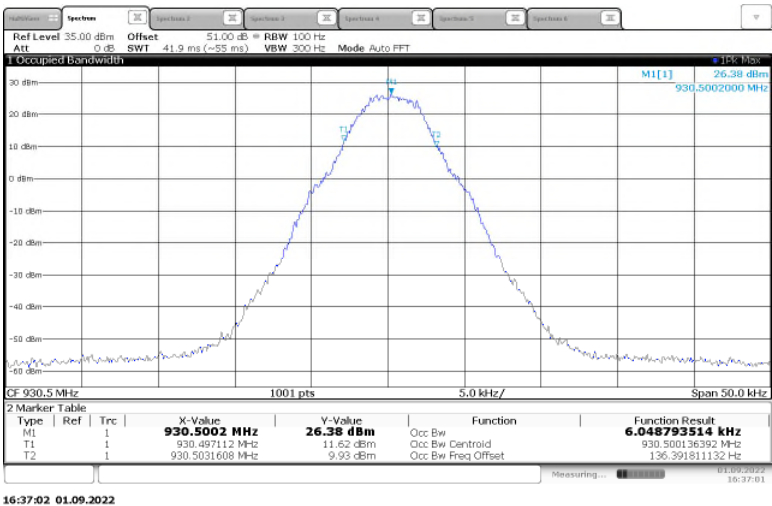
Figure 2.3.6-23: 99% Bandwidth – 930.5 MHz - m4Pass – Low Power
