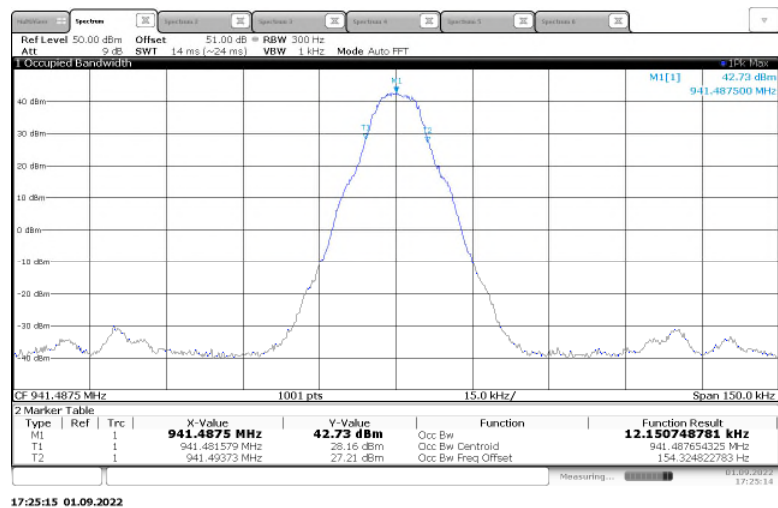
Figure 2.3.6-12: 99% Bandwidth – 941.4875 MHz - m4Pass2 – High Power
