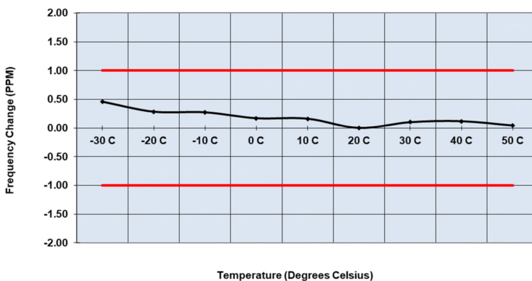
Figure 2.6.6-6: Frequency Stability – 952.5 MHz – High Power
