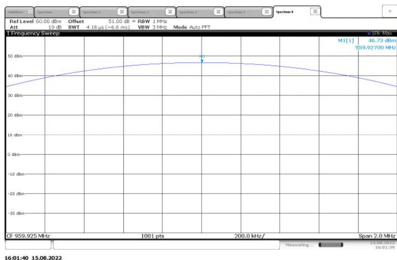
Figure 2.1.6-7: RF Output Power – 959.925 MHz – High Power
