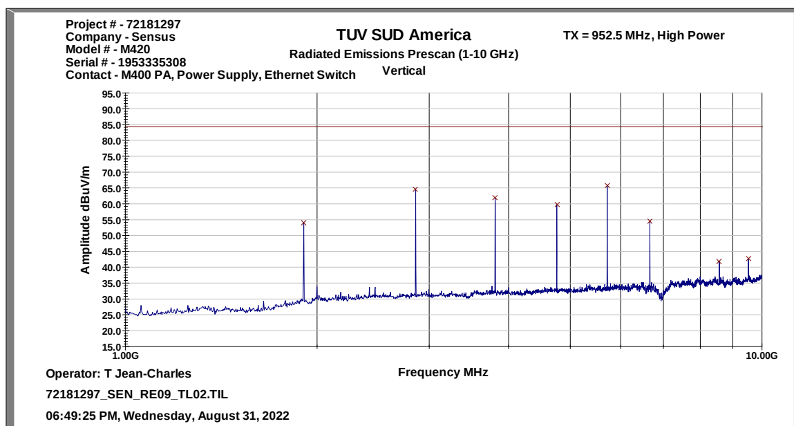
Figure 2.5.6-4: Transmitter Radiated Spurious Emissions – 952.5 MHz - mPass5k Mode – 1 GHz – 10 GHz – Vertical Polarization
