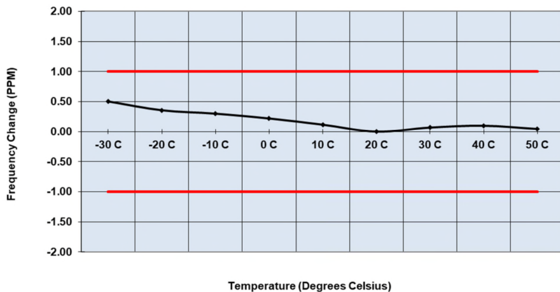
Figure 2.6.6-1: Frequency Stability – 930.5 MHz – High Power
