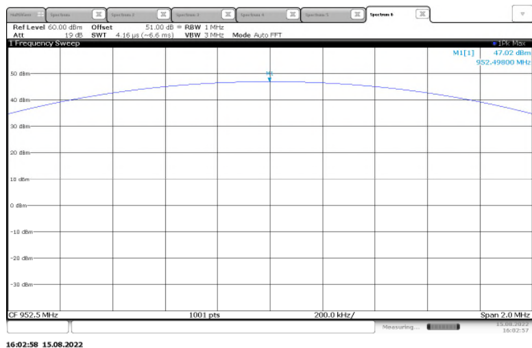
Figure 2.1.6-6: RF Output Power – 952.5 MHz – High Power
