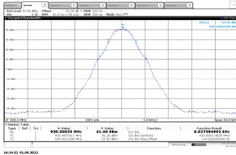
Figure 2.3.6-3: 99% Bandwidth – 930.5 MHz - m4Pass – High Power
