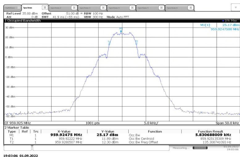
Figure 2.3.6-37: 99% Bandwidth – 959.925 MHz - mPass – Low Power
