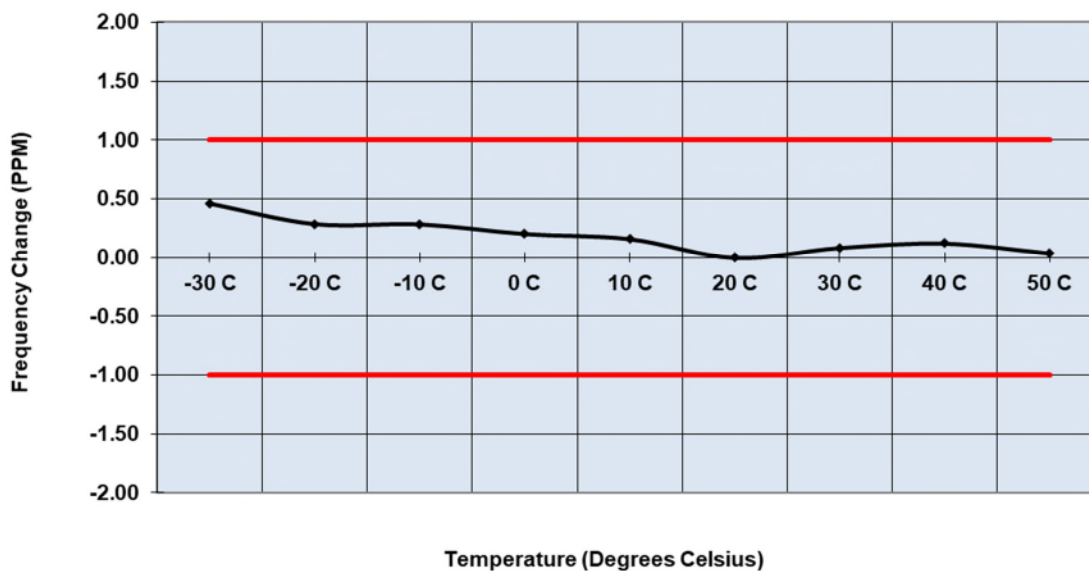
Figure 2.6.6-9: Frequency Stability – 952.5 MHz – Low Power
