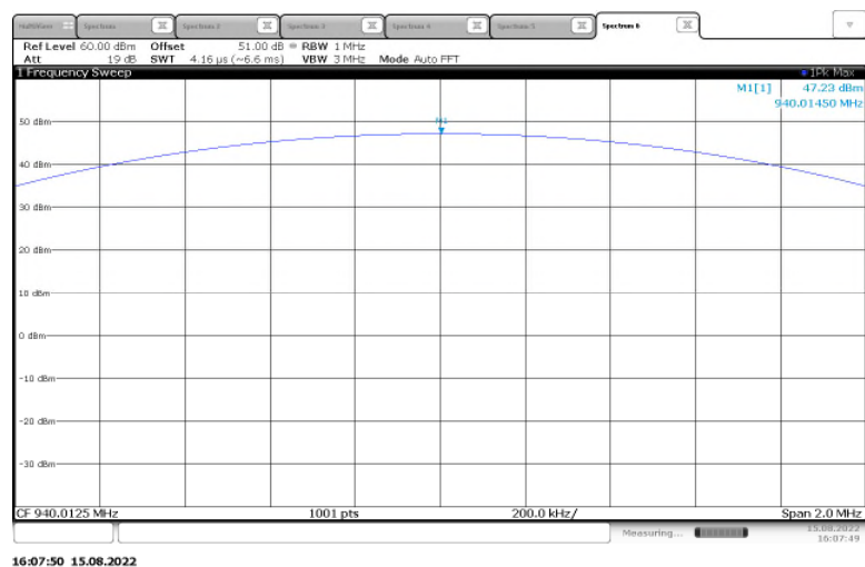
Figure 2.1.6-2: RF Output Power – 940.0125 MHz – High Power
