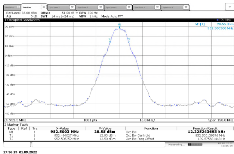
Figure 2.3.6-36: 99% Bandwidth – 952.5 MHz - m4Pass2 – Low Power
