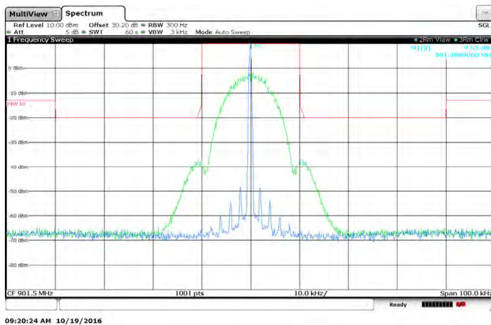
Figure 7.2.2-56: 901.5 MHz – 25 kHz Channel Spacing – 2FSK Mode
