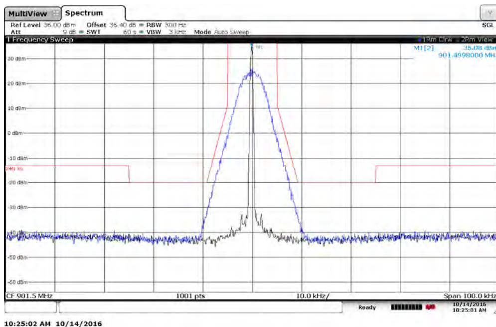
Figure 7.2.2-5: 901.5 MHz – 12.5 kHz Channel Spacing – 8FSK (Half Baud) Mode
