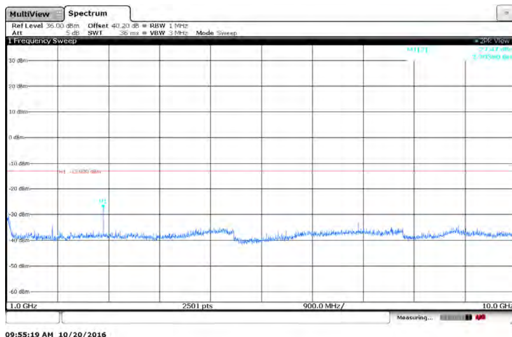
Figure 7.4.2-2: 901.5 MHz – 1GHz to 10GHz – Normal mode
