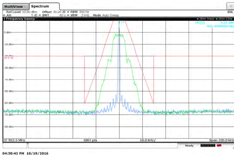
Figure 7.2.2-101: 952.5 MHz - 12.5 kHz Channel Spacing – mPass 5k Mode
