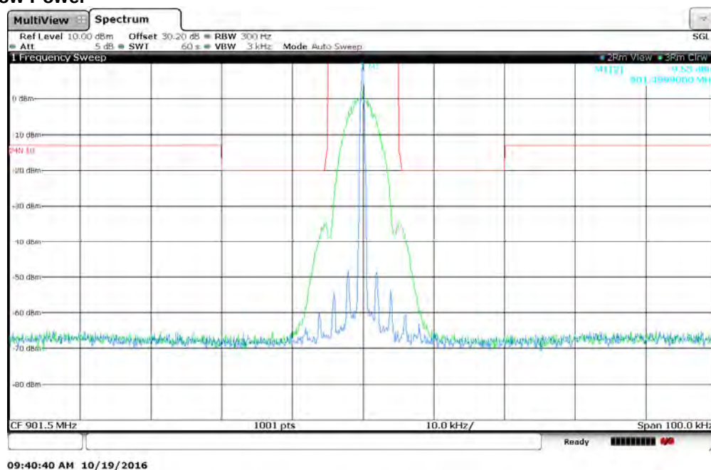
Figure 7.2.2-55: 901.5 MHz – 12.5 kHz Channel Spacing – 2FSK (Half Baud) Mode
