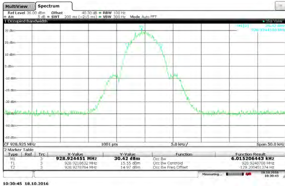
Figure 7.3.2-23: 928.925 MHz – 2FSK (Half Baud) Mode
