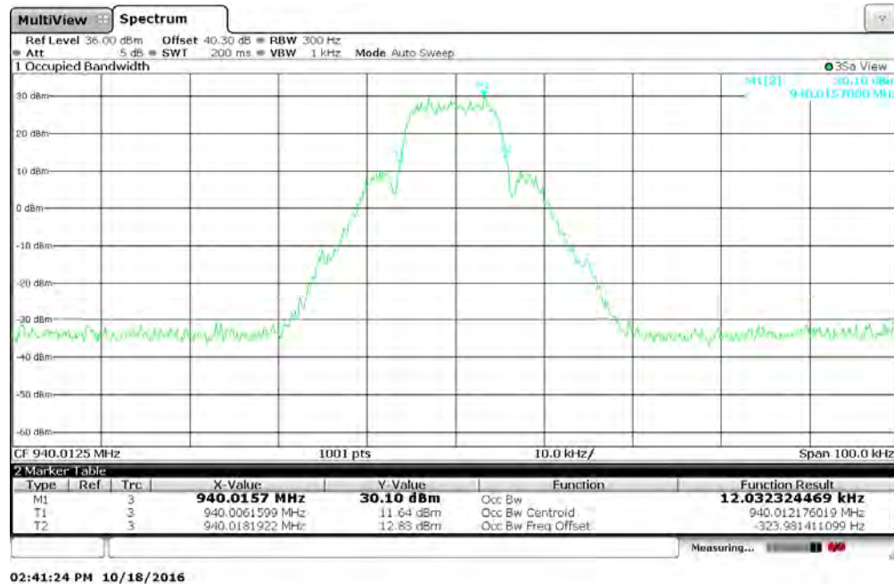
Figure 7.3.2-19: 940.0125 MHz – MPass 10k Mode
