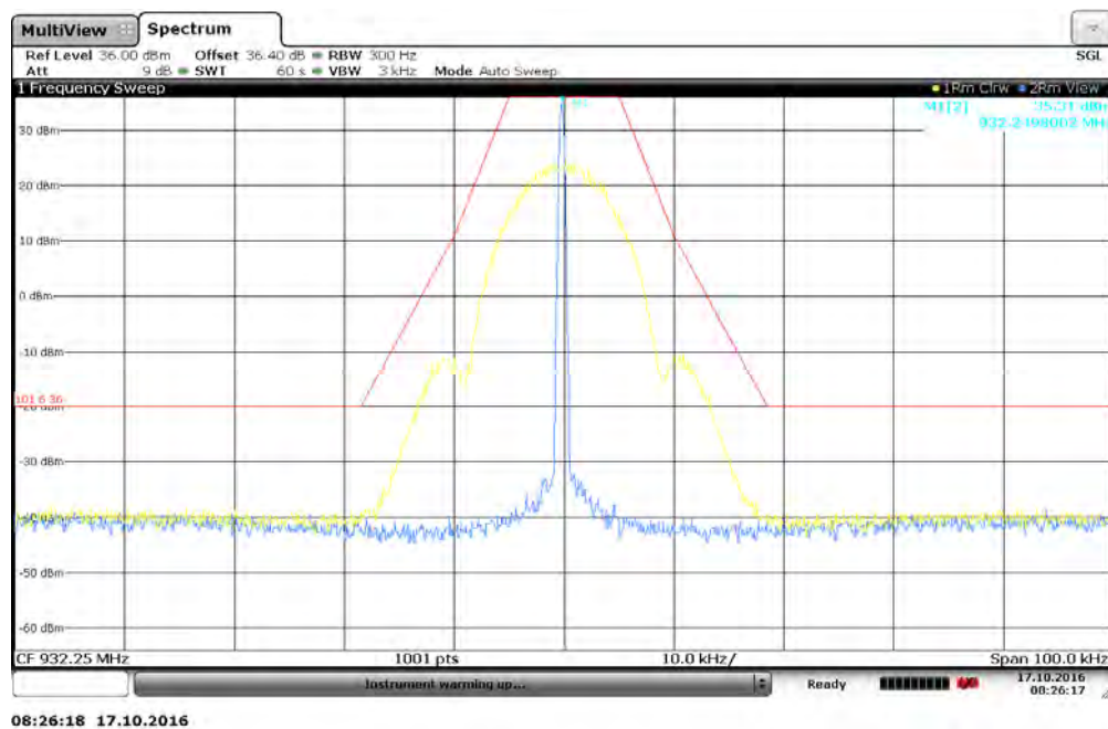
Figure 7.2.2-37: 932.25 MHz –25 kHz Channel Spacing - 2FSK Mode
