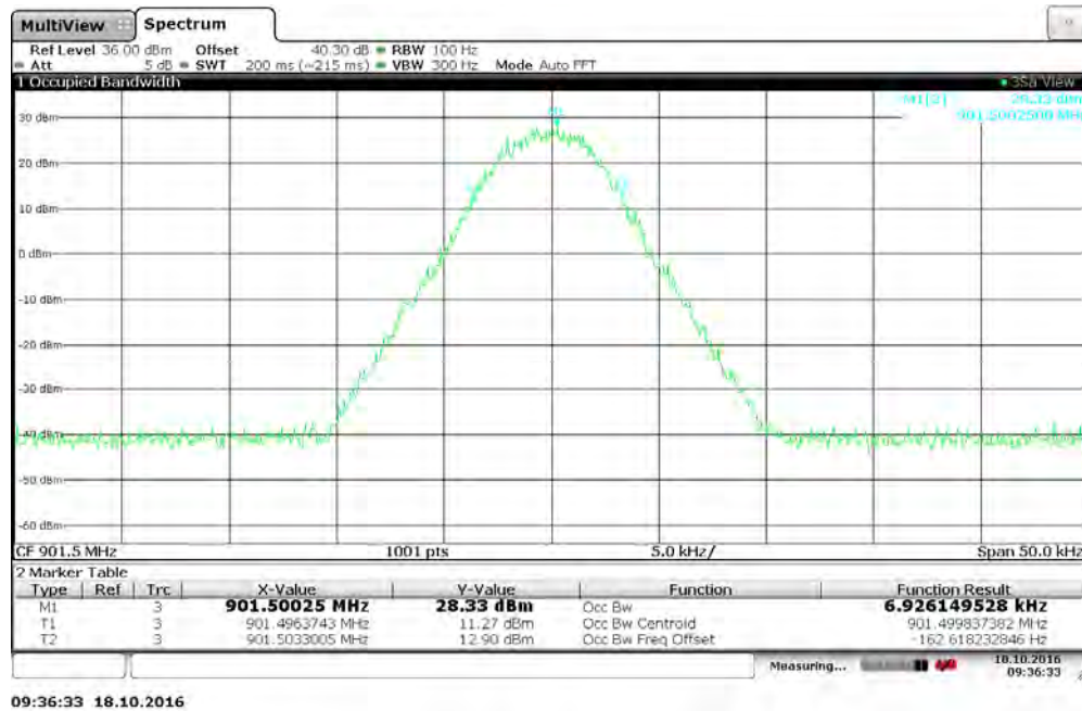
Figure 7.3.2-5: 901.5 MHz – 4SFSK (Half Baud) Mode
