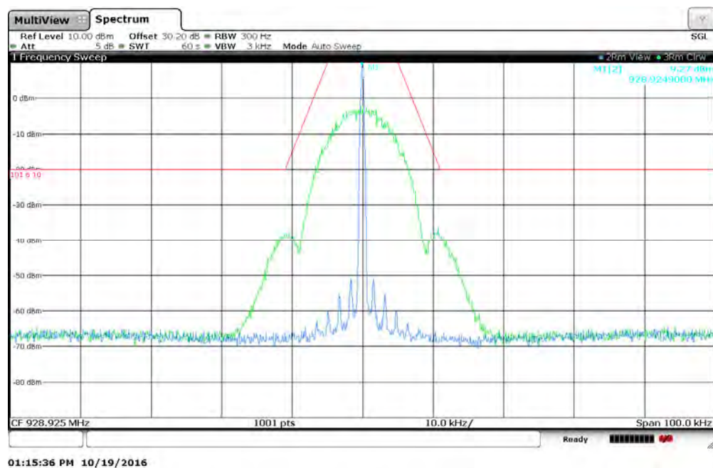
Figure 7.2.2-77: 928.925 MHz – 25 kHz Channel Spacing - 2FSK Mode
