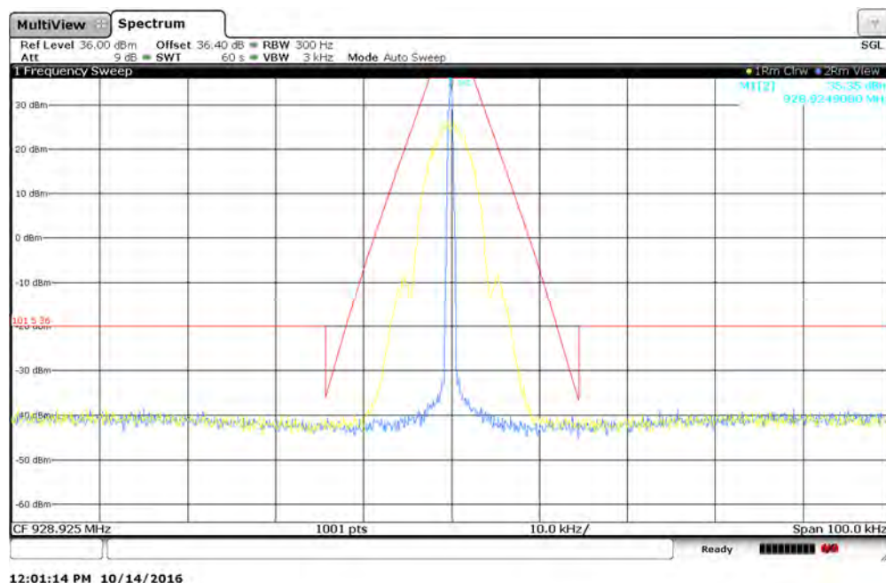
Figure 7.2.2-29: 928.925 MHz — 12.5 kHz Channel Spacing - 2FSK (Half Baud) Mode
