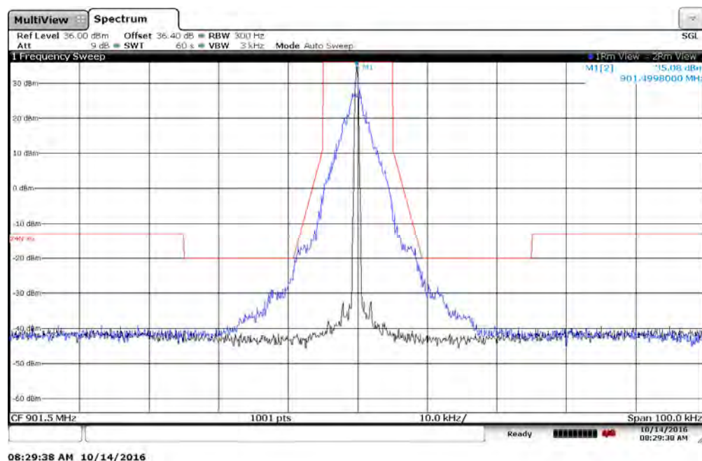
Figure 7.2.2-10: 901.5 MHz – 12.5 kHz Channel Spacing – Priority Mode
