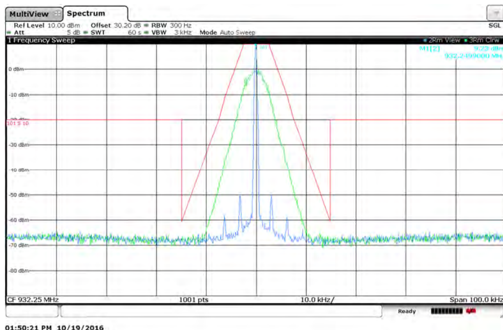
Figure 7.2.2-95: 932.25 MHz – 12.5 kHz Channel Spacing - 4FSK (Half Baud) Mode
