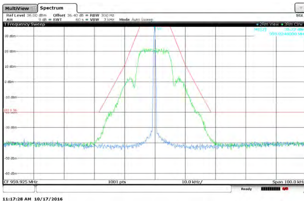
Figure 7.2.2-52: 959.925 MHz – 25 kHz Channel Spacing – mPass 10k Mode
