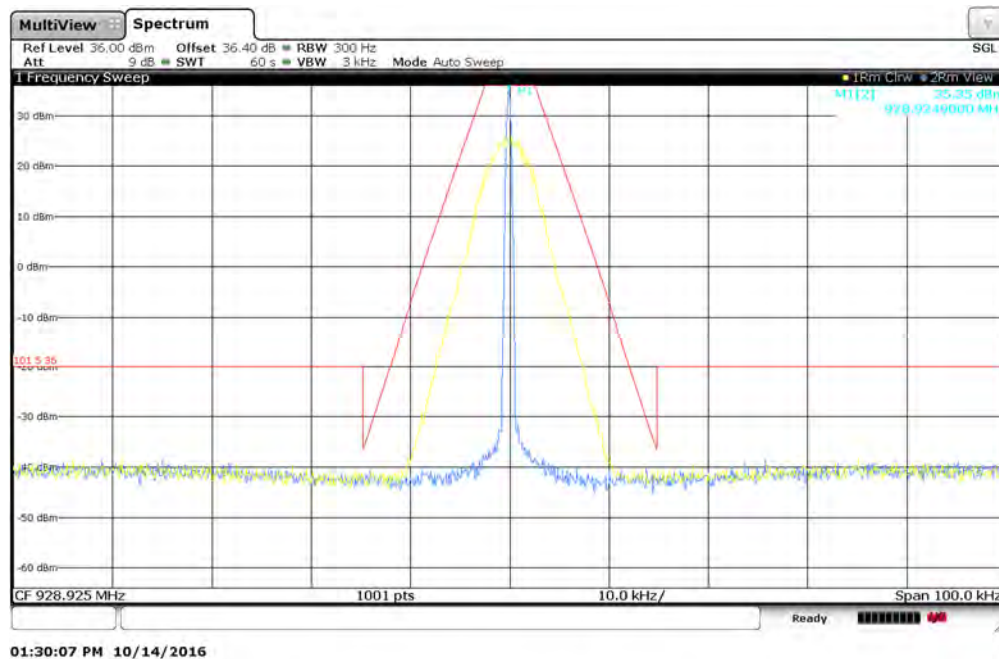
Figure 7.2.2-30: 928.925 MHz — 12.5 kHz Channel Spacing - 4SFSK (Half Baud) Mode
