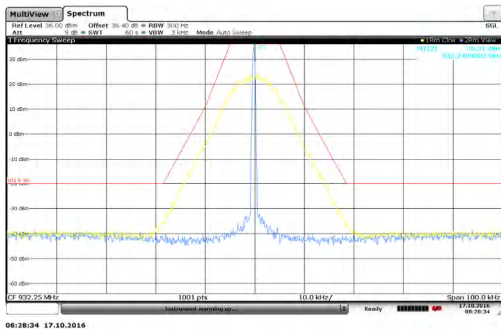
Figure 7.2.2-38: 932.25 MHz – 25 kHz Channel Spacing - 4FSK Mode
