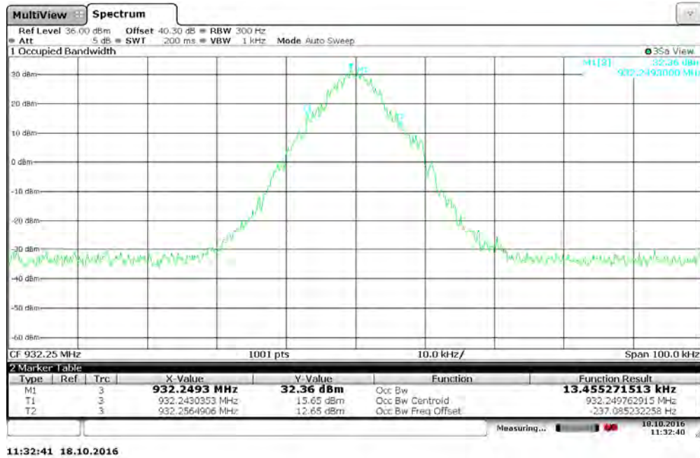
Figure 7.3.2-39: 932.25 MHz – Double Density Mode
