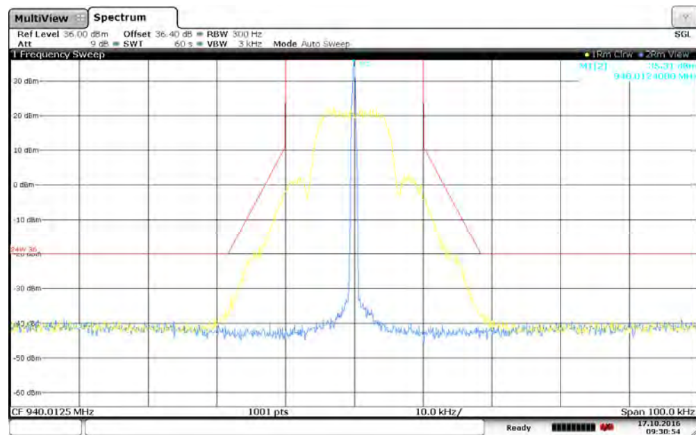
Figure 7.2.2-18: 940.0125 MHz – 25 kHz Channel Spacing – mPass 10k Mode
