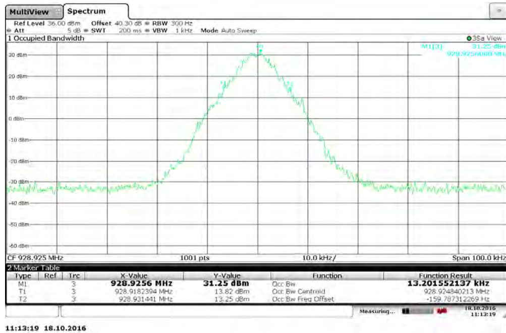
Figure 7.3.2-28: 928.925 MHz – Double Density Mode
