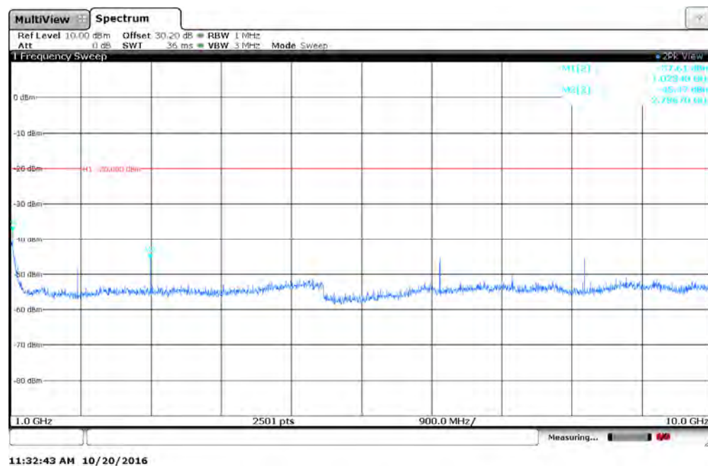
Figure 7.4.2-24: 928.925 MHz – 1GHz to 10GHz
