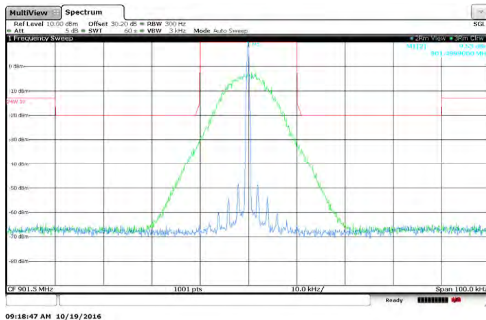
Figure 7.2.2-58: 901.5 MHz – 25 kHz Channel Spacing – 4FSK Mode
