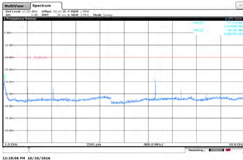
Figure 7.4.2-30: 952.5 MHz – 1GHz to 10GHz
