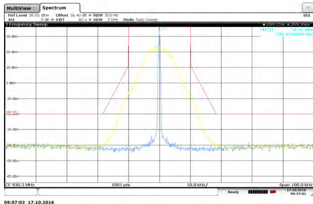
Figure 7.2.2-14: 930.5 MHz – 25 kHz Channel Spacing – m4Pass 20k Mode
