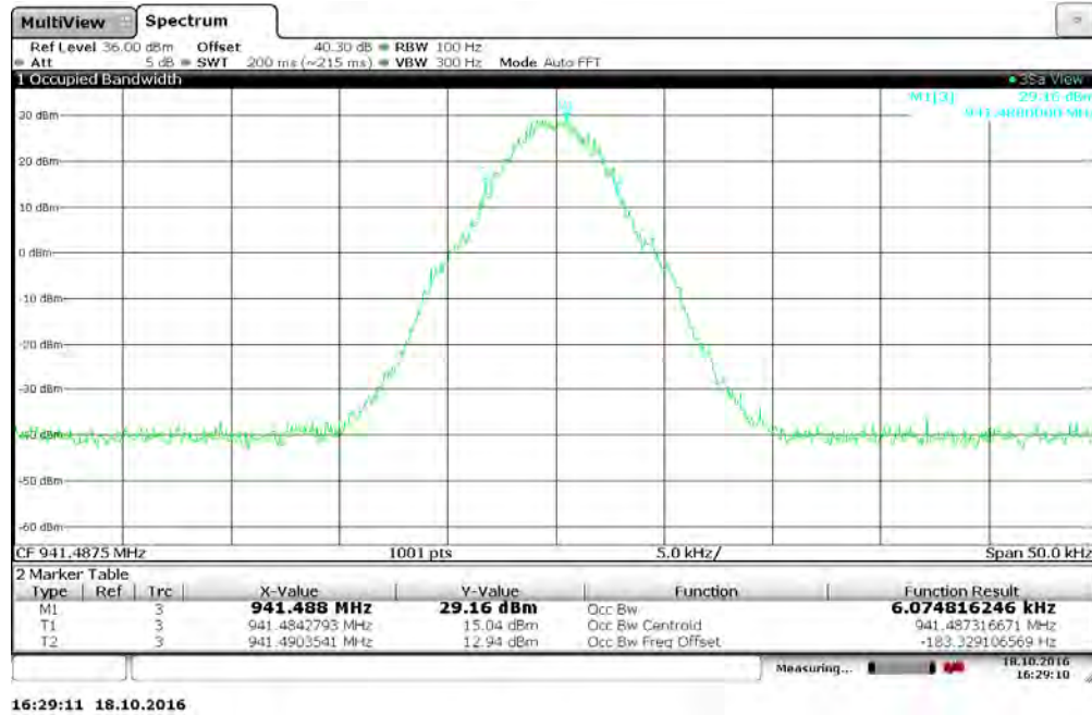
Figure 7.3.2-42: 941.4875 MHz – m4Pass 10k Mode
