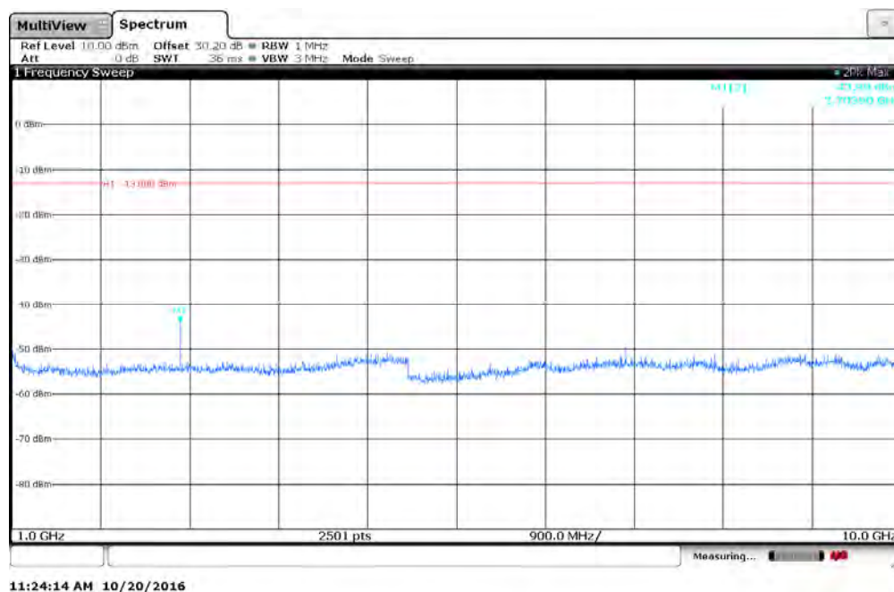
Figure 7.4.2-18: 901.5 MHz – 1GHz to 10GHz
