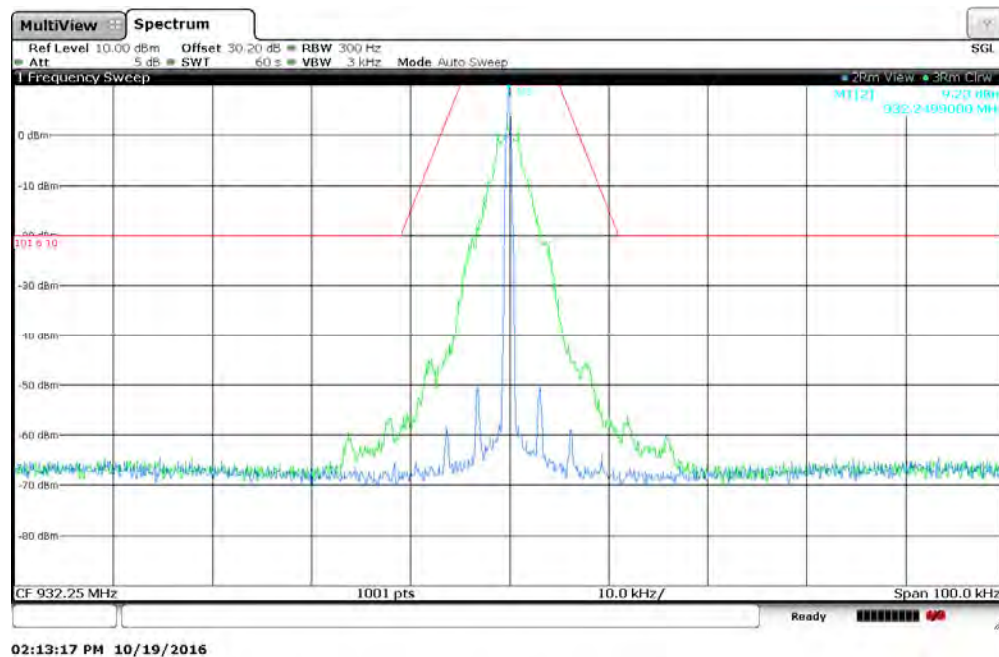
Figure 7.2.2-86: 932.25 MHz – 25 kHz Channel Spacing - C&I Mode
