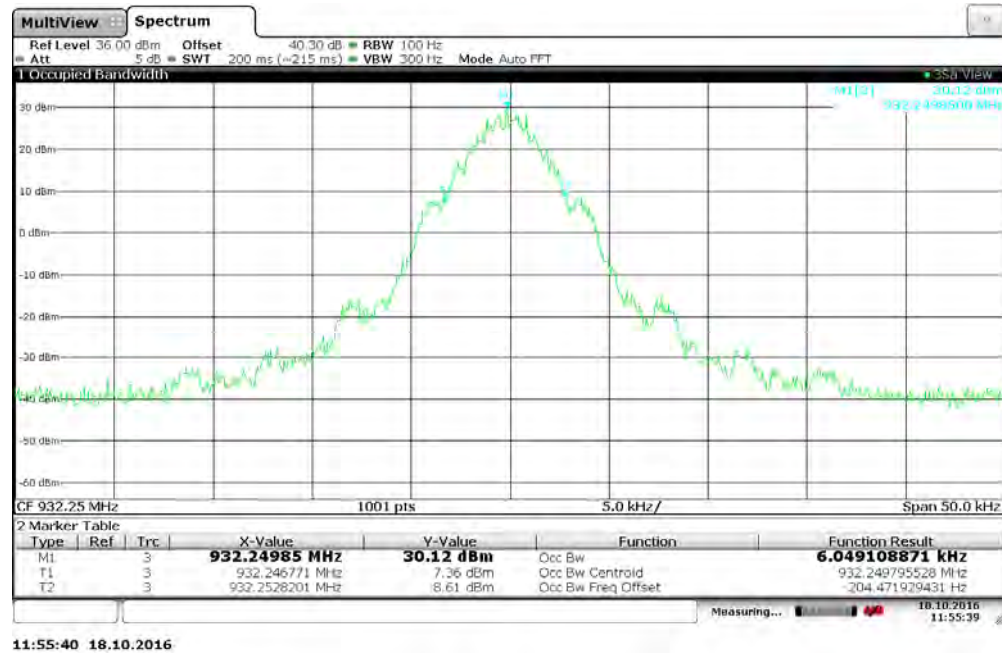
Figure 7.3.2-38: 932.25 MHz – C&amp;I (Half Baud) Mode
