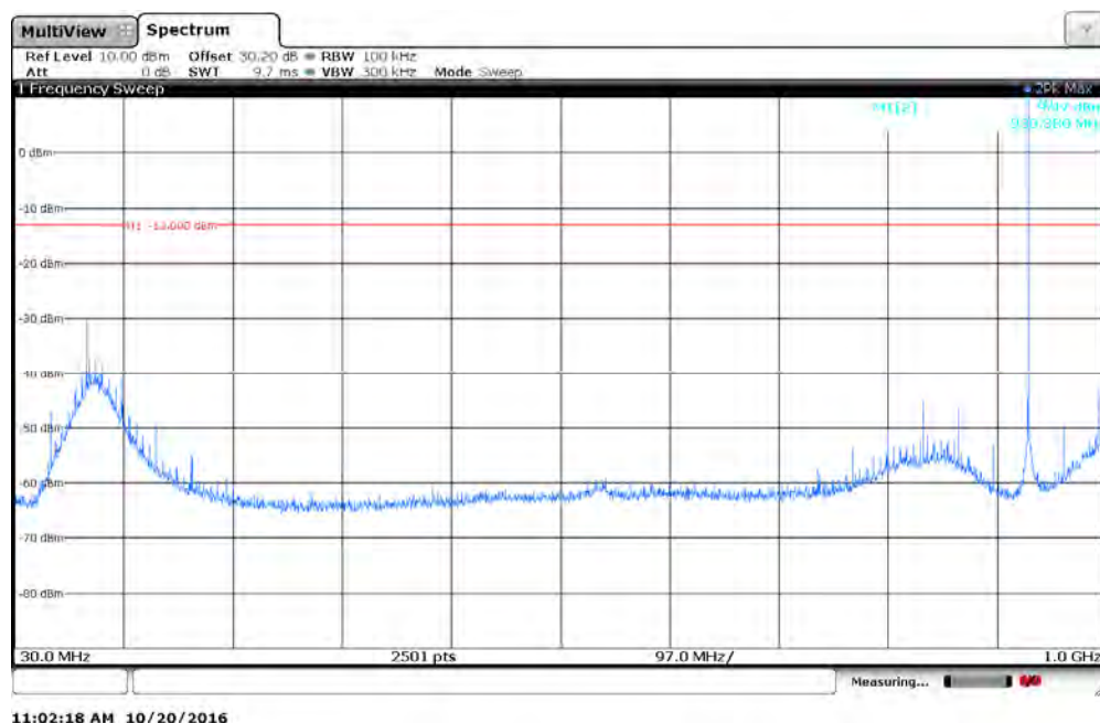
Figure 7.4.2-19: 930.5 MHz – 30MHz to 1GHz
