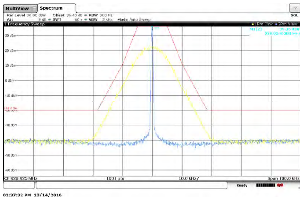
Figure 7.2.2-25: 928.925 MHz – 25 kHz Channel Spacing - 8FSK Mode
