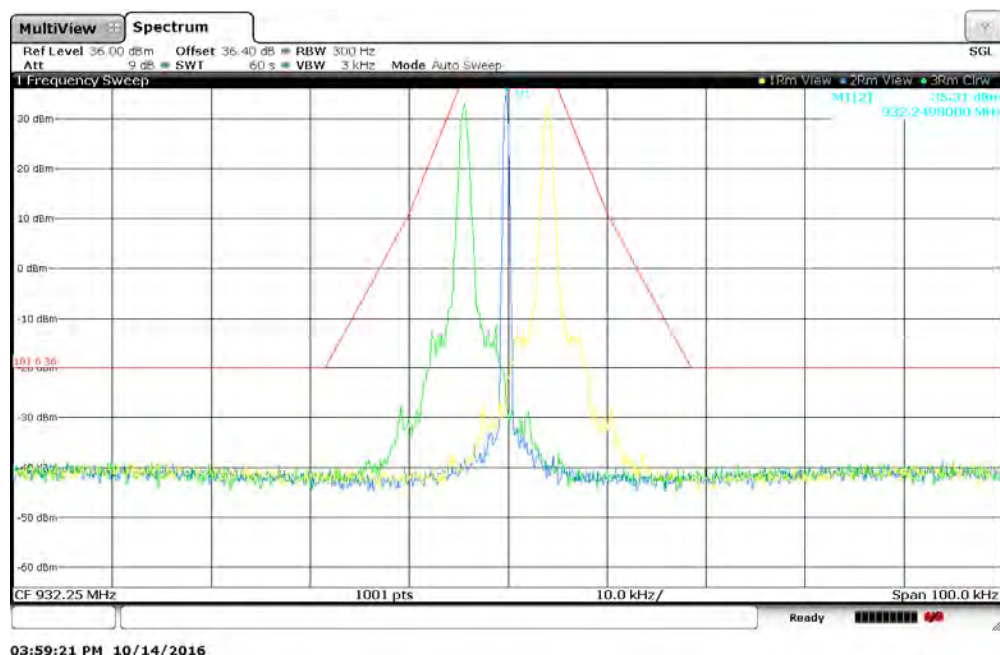
Figure 7.2.2-36: 932.25 MHz – 25 kHz Channel Spacing - Boost Mode
