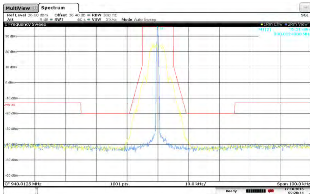
Figure 7.2.2-17: 940.0125 MHz – 12.5 kHz Channel Spacing – mPass 5k Mode
