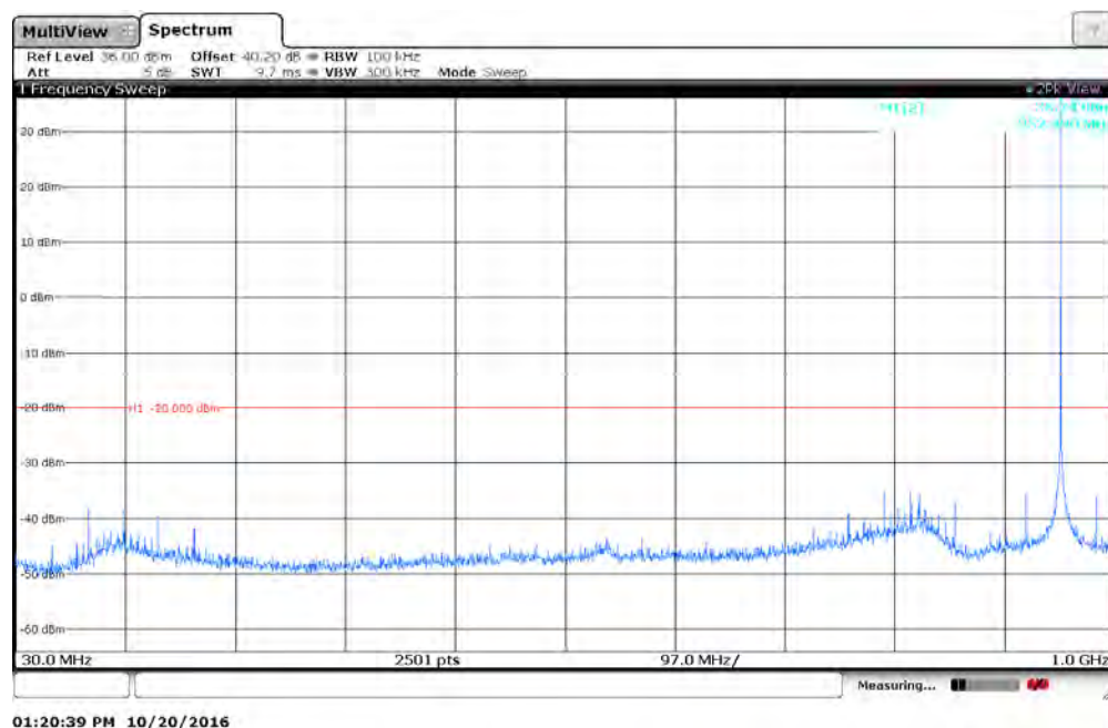
Figure 7.4.2-13: 952.5 MHz – 30MHz to 1GHz – Mpass5k mode
