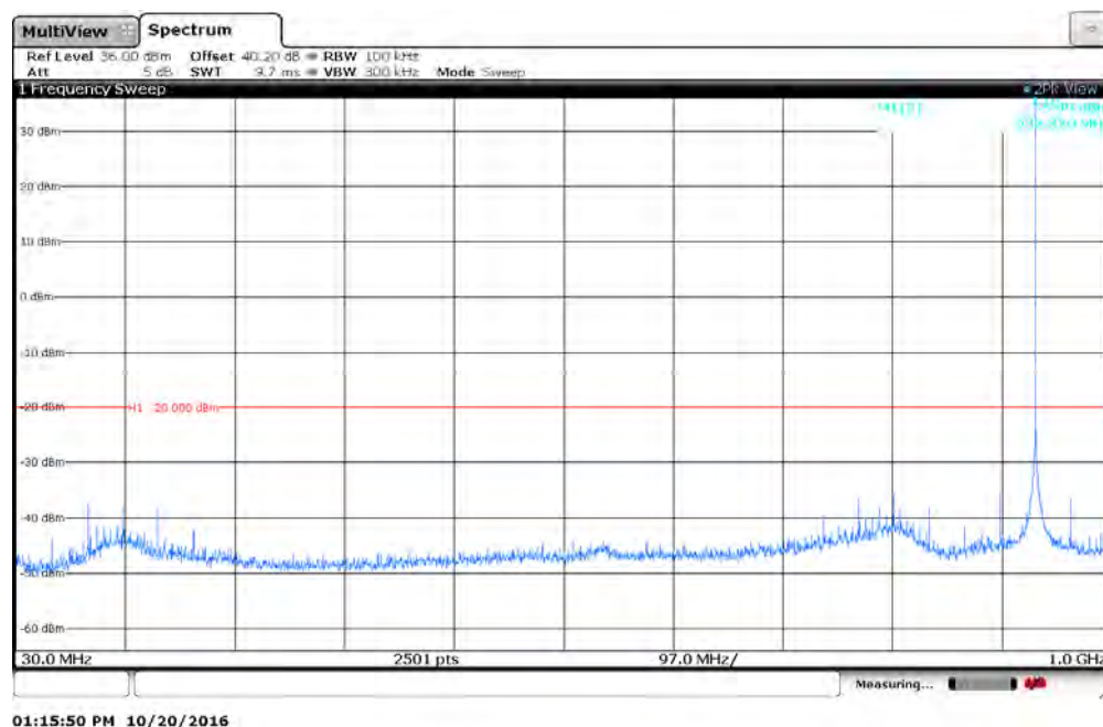
Figure 7.4.2-9: 932.25 MHz – 30MHz to 1GHz – Normal mode
