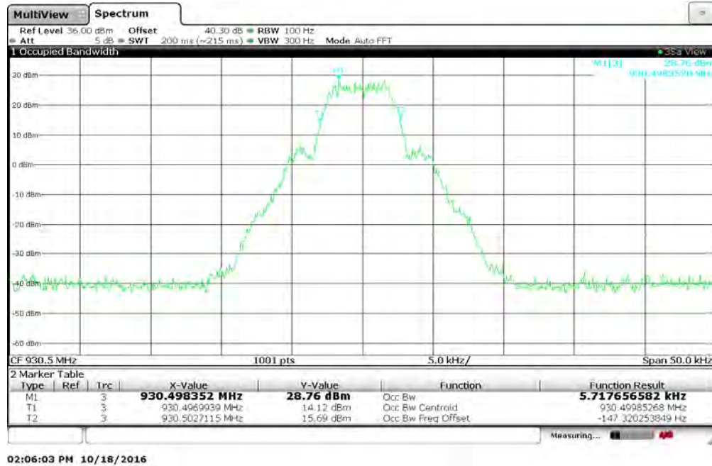
Figure 7.3.2-14: 930.5 MHz – MPass 5k Mode
