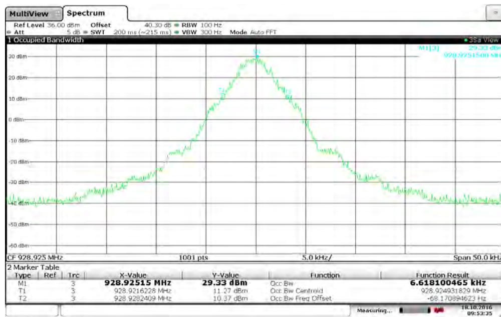
Figure 7.3.2-30: 928.925 MHz – Priority Mode
