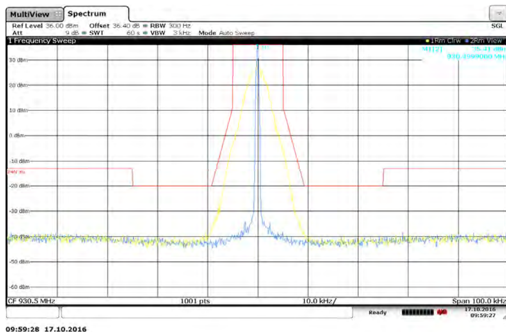
Figure 7.2.2-13: 930.5 MHz - 12.5 kHz Channel Spacing – m4Pass 10k Mode
