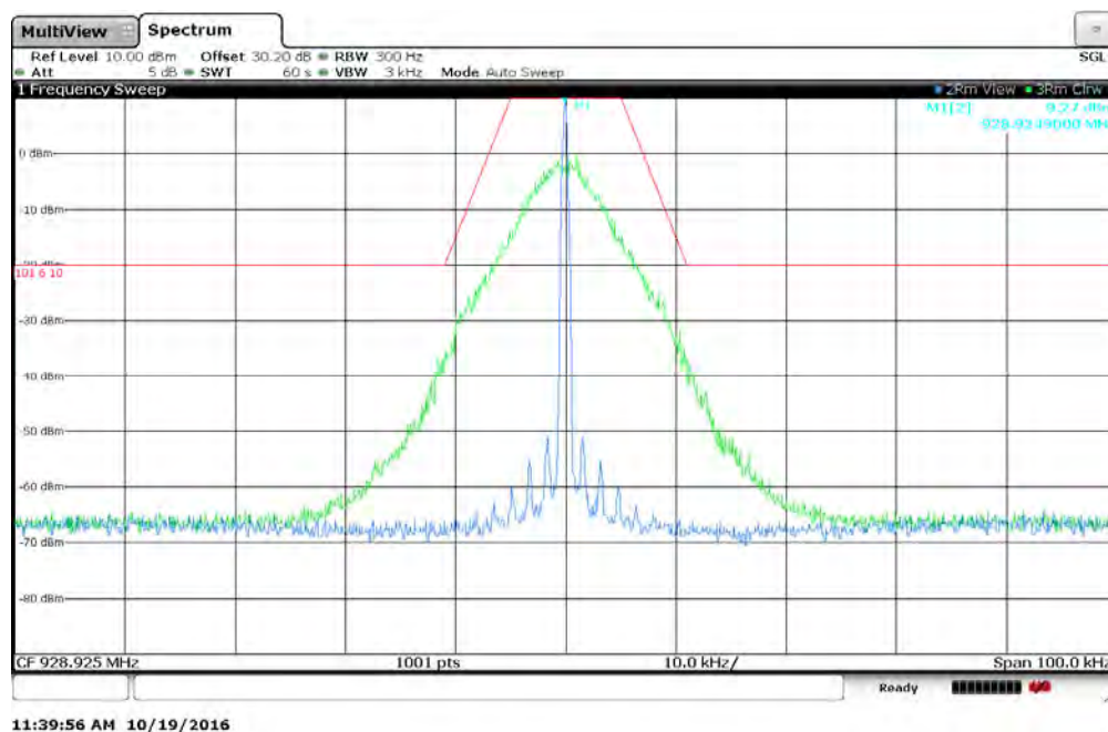
Figure 7.2.2-76: 928.925 MHz – 25 kHz Channel Spacing - Double Density Mode
