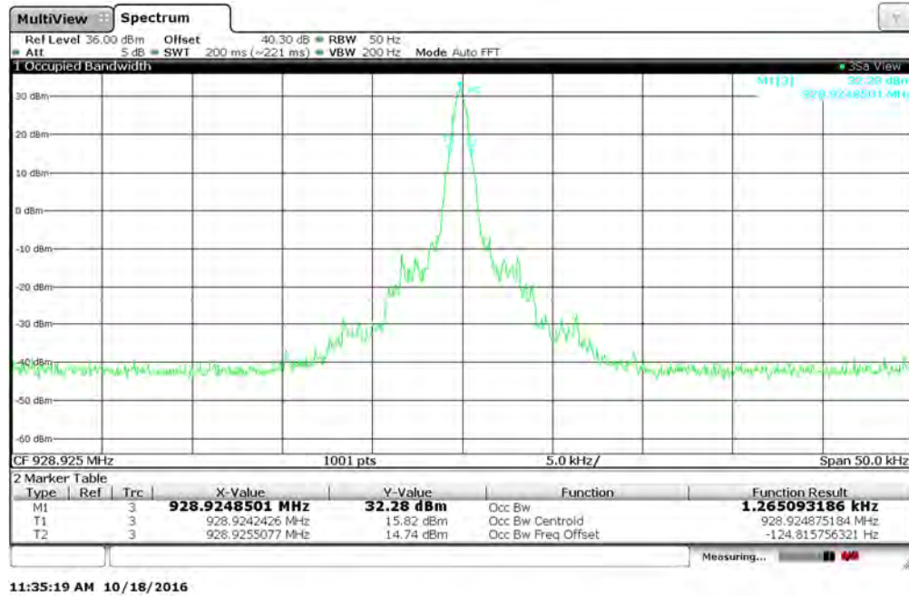
Figure 7.3.2-26: 928.925 MHz – Boost Mode
