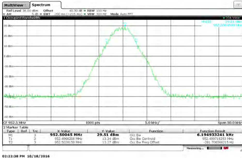
Figure 7.3.2-46: 952.5 MHz – m4Pass 10k Mode
