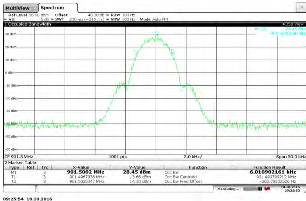
Figure 7.3.2-4: 901.5 MHz – 2SFSK (Half Baud) Mode
