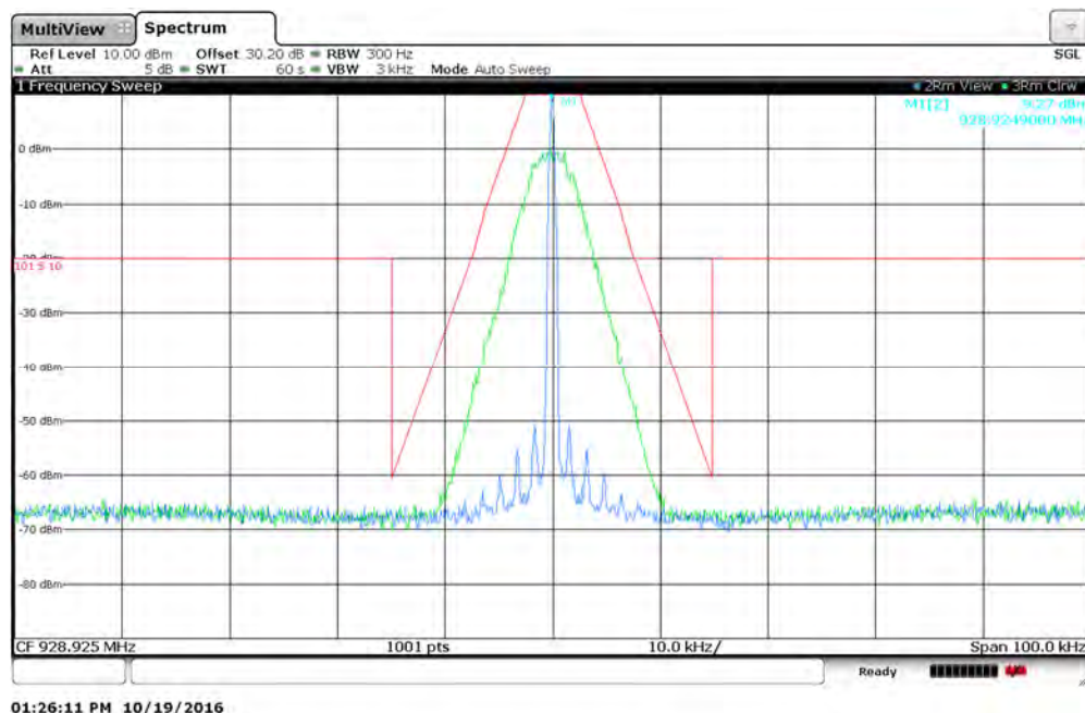
Figure 7.2.2-84: 928.925 MHz -- 12.5 kHz Channel Spacing - 4FSK (Half Baud) Mode
