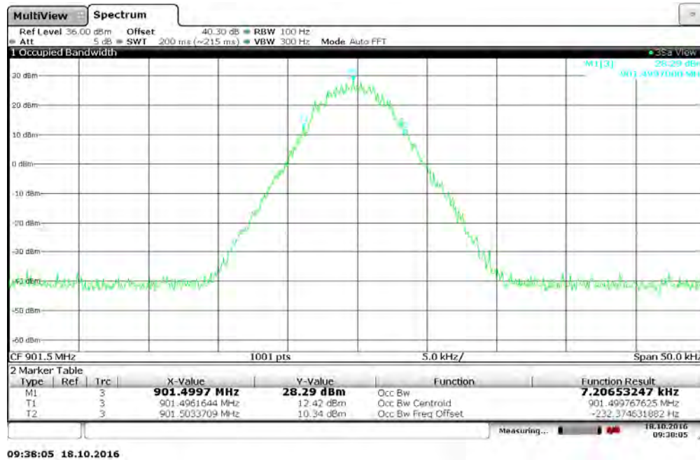
Figure 7.3.2-6: 901.5 MHz – 8 SFSK (Half Baud) Mode
