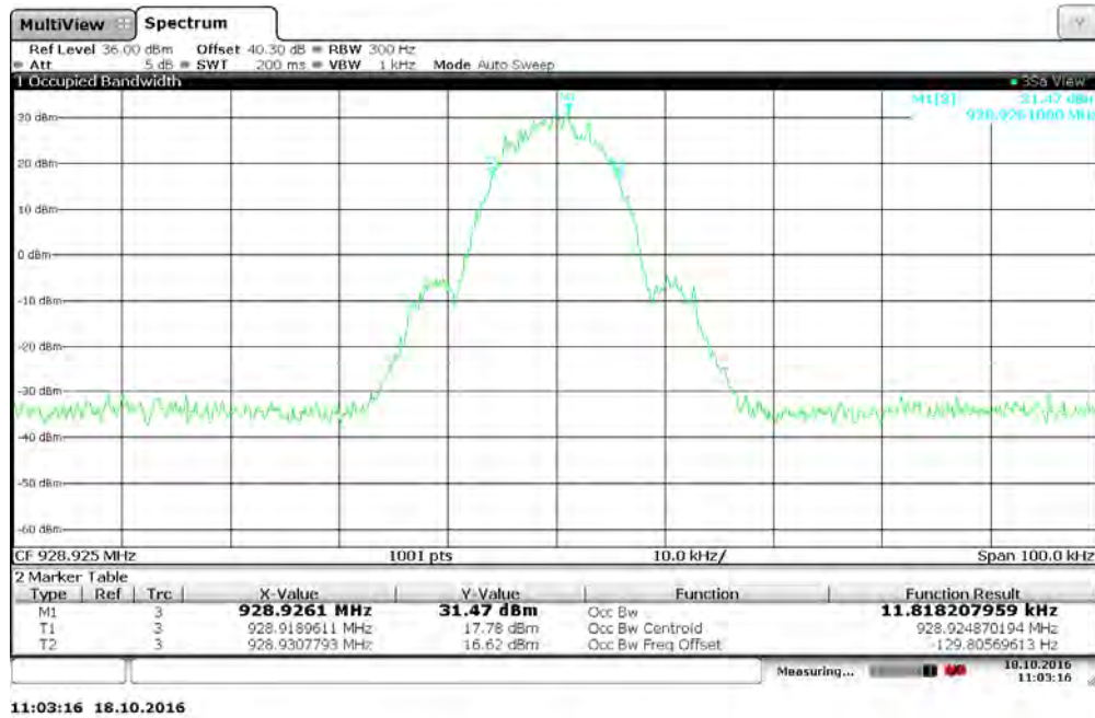
Figure 7.3.2-20: 928.925 MHz – 2FSK Mode
