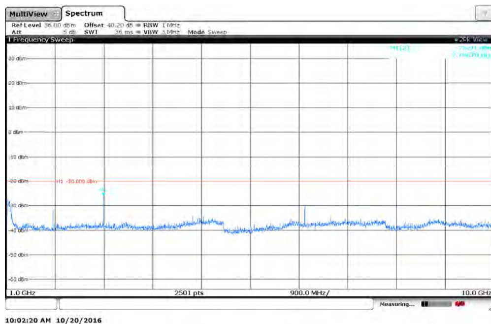
Figure 7.4.2-8: 928.925 MHz – 1GHz to 10GHz – Normal mode
