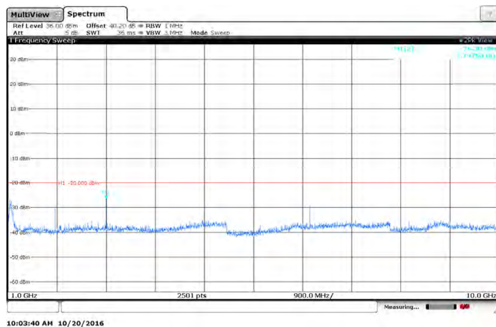
Figure 7.4.2-10: 932.25 MHz – 1GHz to 10GHz – Normal mode
