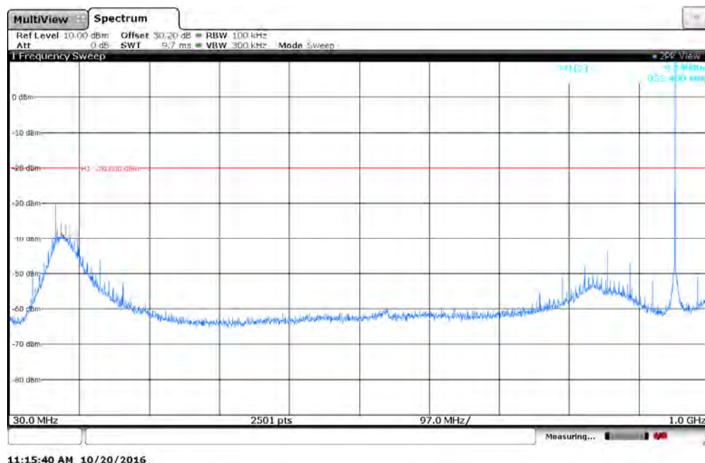
Figure 7.4.2-29: 952.5 MHz – 30MHz to 1GHz
