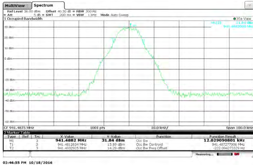
Figure 7.3.2-43: 941.4875 MHz – m4Pass 20k Mode
