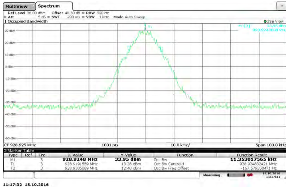
Figure 7.3.2-29: 928.925 MHz – Normal Mode
