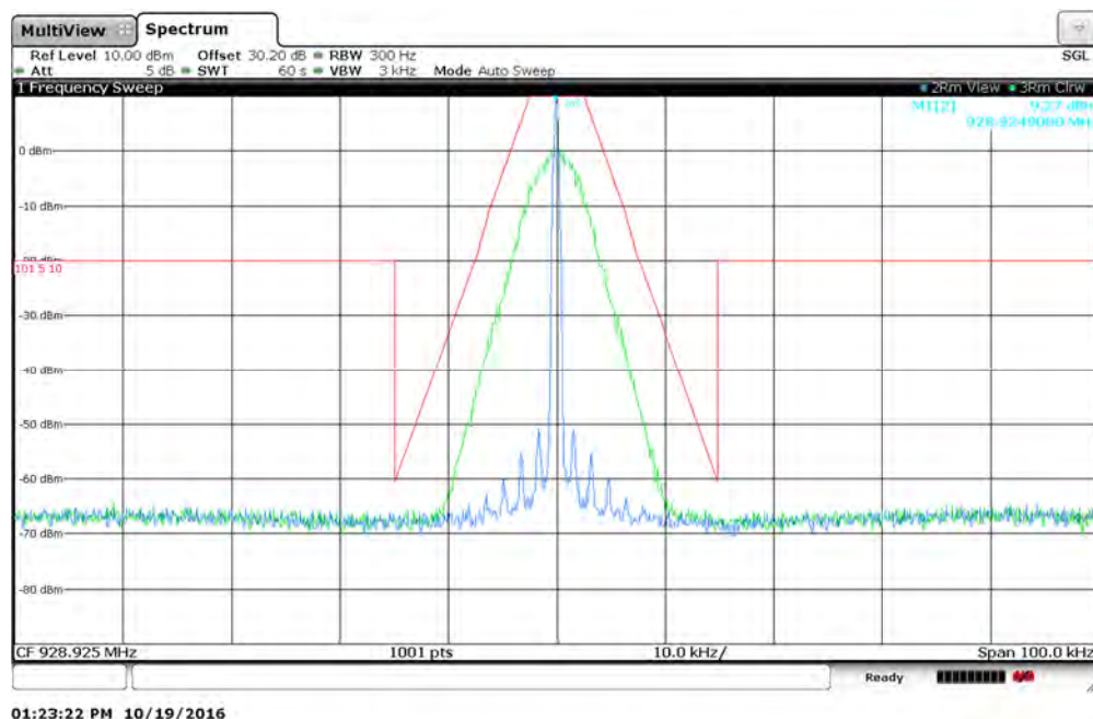
Figure 7.2.2-85: 928.925 MHz -- 12.5 kHz Channel Spacing - 8FSK (Half Baud) Mode
