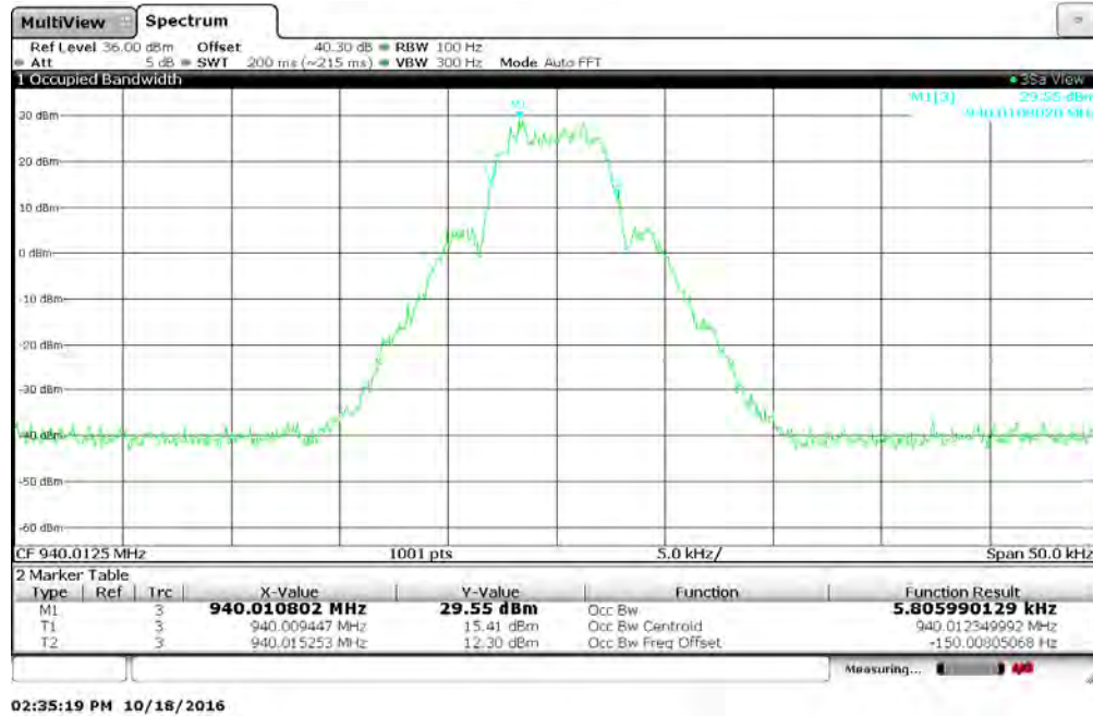
Figure 7.3.2-18: 940.0125 MHz – MPass 5k Mode
