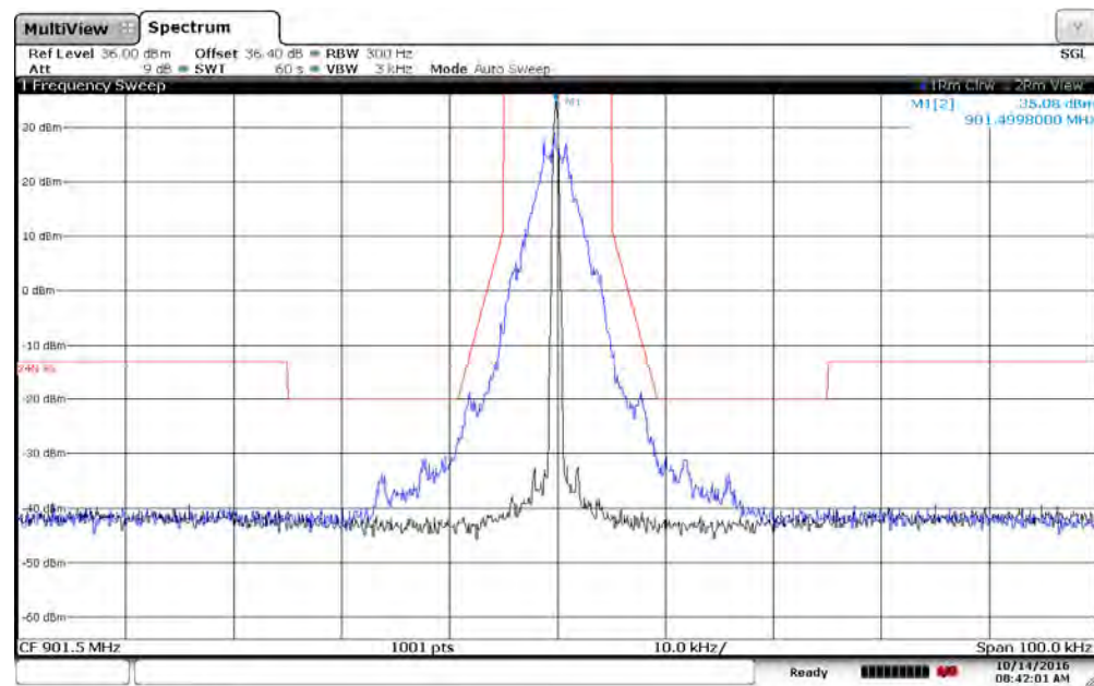
Figure 7.2.2-9: 901.5 MHz – 12.5 kHz Channel Spacing – C&amp;I (Half Baud) Mode
