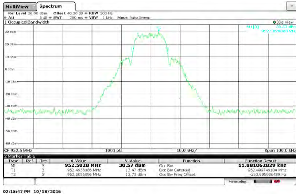
Figure 7.3.2-49: 952.5 MHz – MPass 10k Mode
