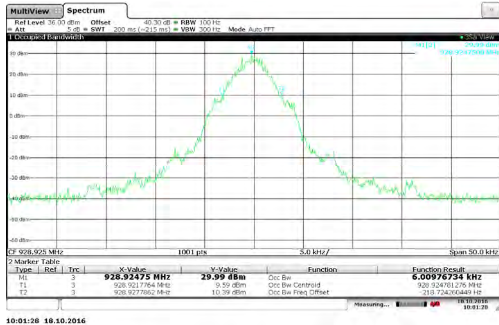
Figure 7.3.2-27: 928.925 MHz – C&amp;I (Half Baud) Mode
