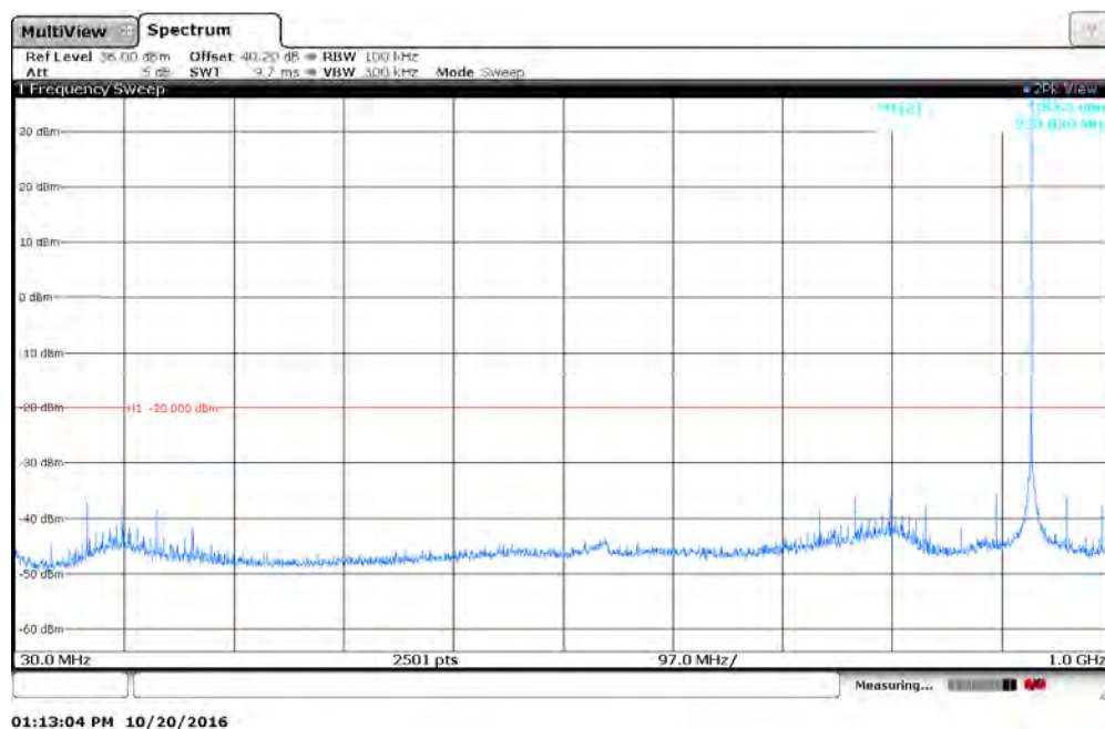
Figure 7.4.2-7: 928.925 MHz – 30MHz to 1GHz – Normal mode
