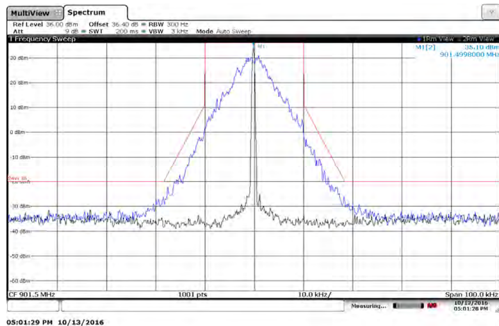
Figure 7.2.2-11: 901.5 MHz – 25 kHz Channel Spacing – Double Density Mode
