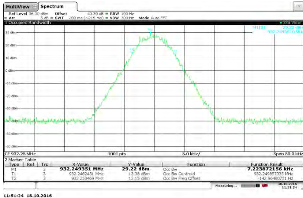
Figure 7.3.2-36: 932.25 MHz – 8SFSK (Half Baud) Mode
