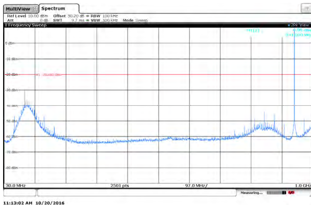
Figure 7.4.2-27: 941.4875 MHz – 30MHz to 1GHz
