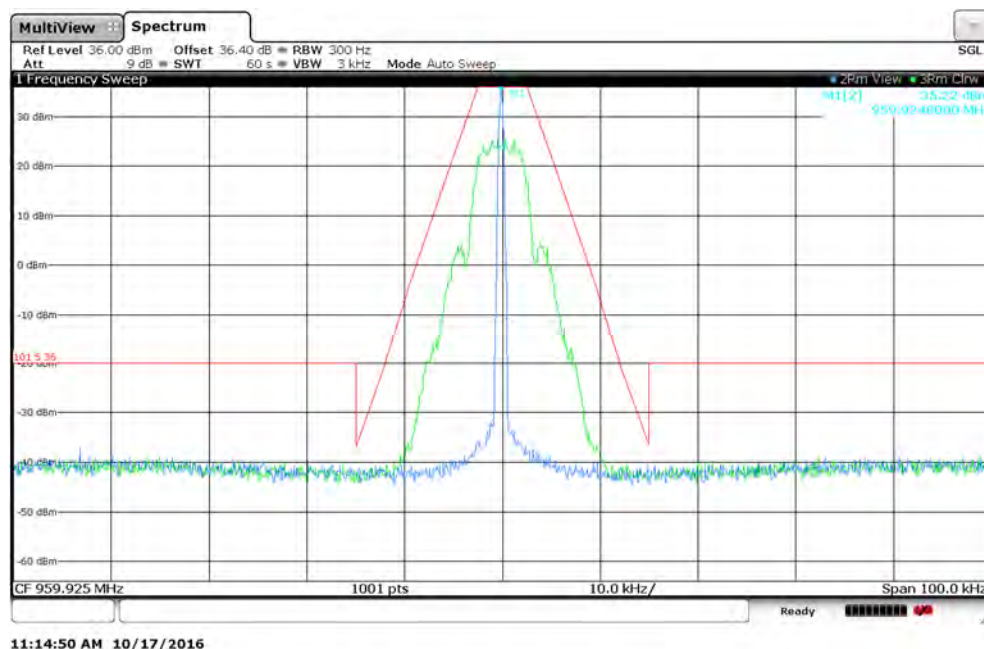
Figure 7.2.2-51: 959.925 MHz - 12.5 kHz Channel Spacing – mPass 5k Mode
