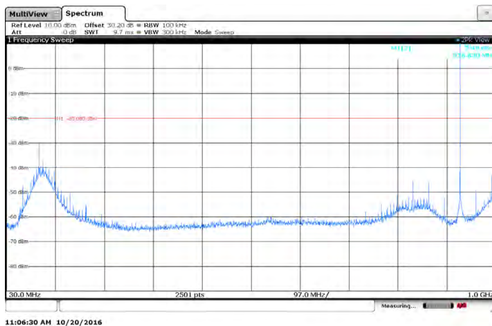
Figure 7.4.2-23: 928.925 MHz – 30MHz to 1GHz
