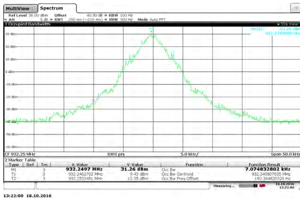
Figure 7.3.2-41: 932.25 MHz — Priority Mode
