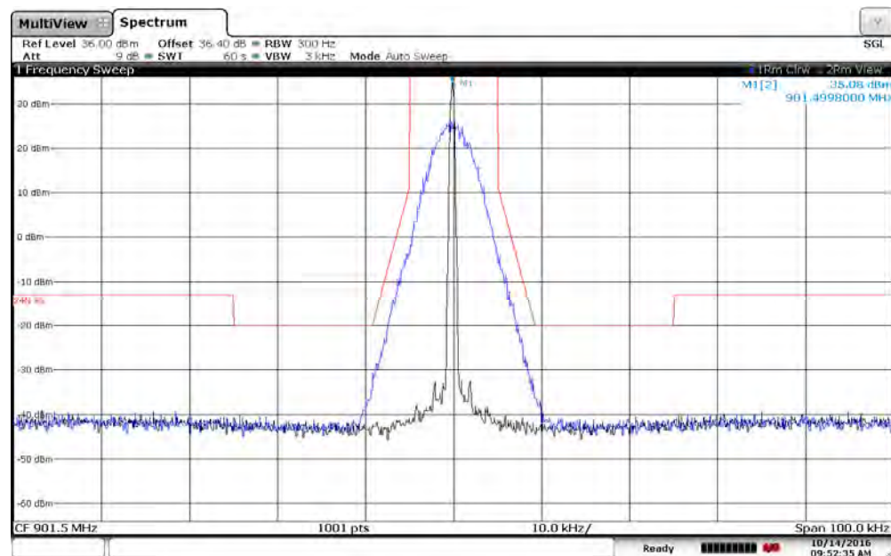
Figure 7.2.2-3: 901.5 MHz – 12.5 kHz Channel Spacing – 4FSK (Half Baud) Mode
