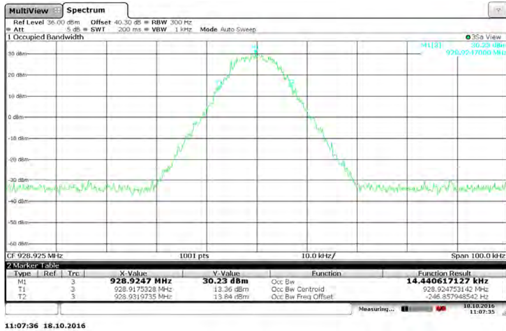
Figure 7.3.2-22: 928.925 MHz – 8FSK Mode
