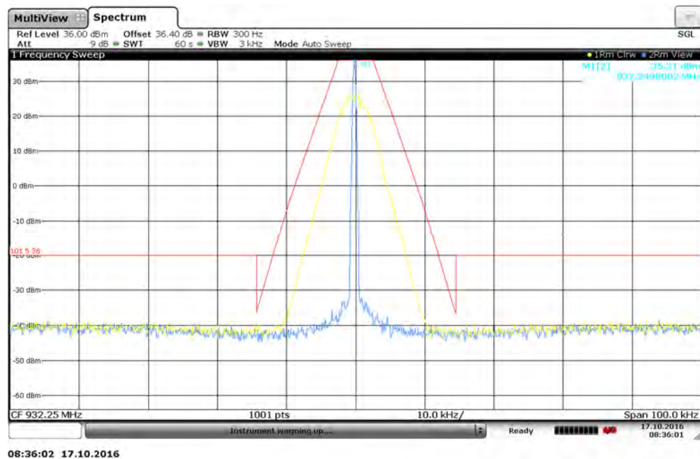
Figure 7.2.2-41: 932.25 MHz – 12.5 kHz Channel Spacing - 4SFSK (Half Baud) Mode
