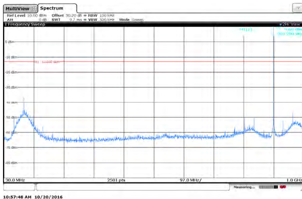
Figure 7.4.2-17: 901.5 MHz – 30MHz to 1GHz
