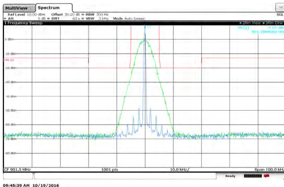
Figure 7.2.2-59: 901.5 MHz – 12.5 kHz Channel Spacing – 8FSK (Half Baud) Mode
