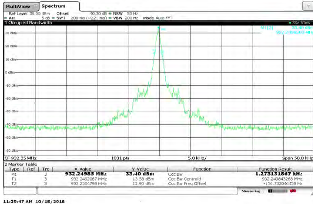
Figure 7.3.2-37: 932.25 MHz – Boost Mode
