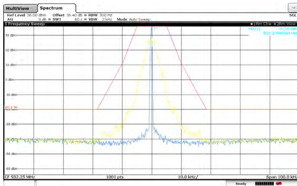
Figure 7.2.2-32: 932.25 MHz – 25 kHz Channel Spacing - C&amp;I Mode
