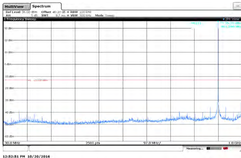
Figure 7.4.2-1: 901.5 MHz – 30MHz to 1GHz – Normal mode
