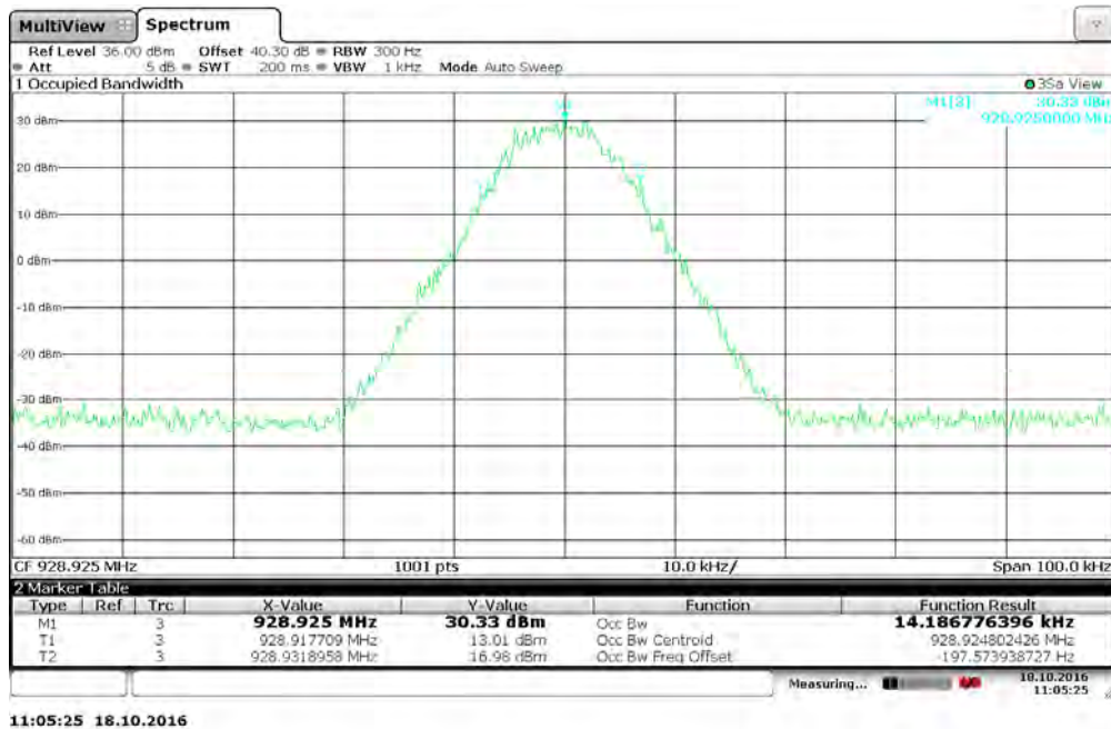
Figure 7.3.2-21: 928.925 MHz – 4FSK Mode
