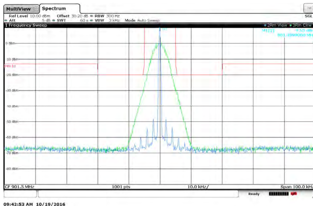
Figure 7.2.2-57: 901.5 MHz – 12.5 kHz Channel Spacing – 4FSK (Half Baud) Mode
