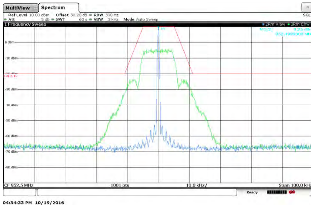
Figure 7.2.2-102: 952.5 MHz – 25 kHz Channel Spacing – mPass 10k Mode
