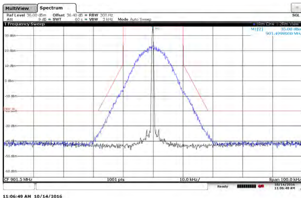
Figure 7.2.2-4: 901.5 MHz – 25 kHz Channel Spacing – 4FSK Mode
