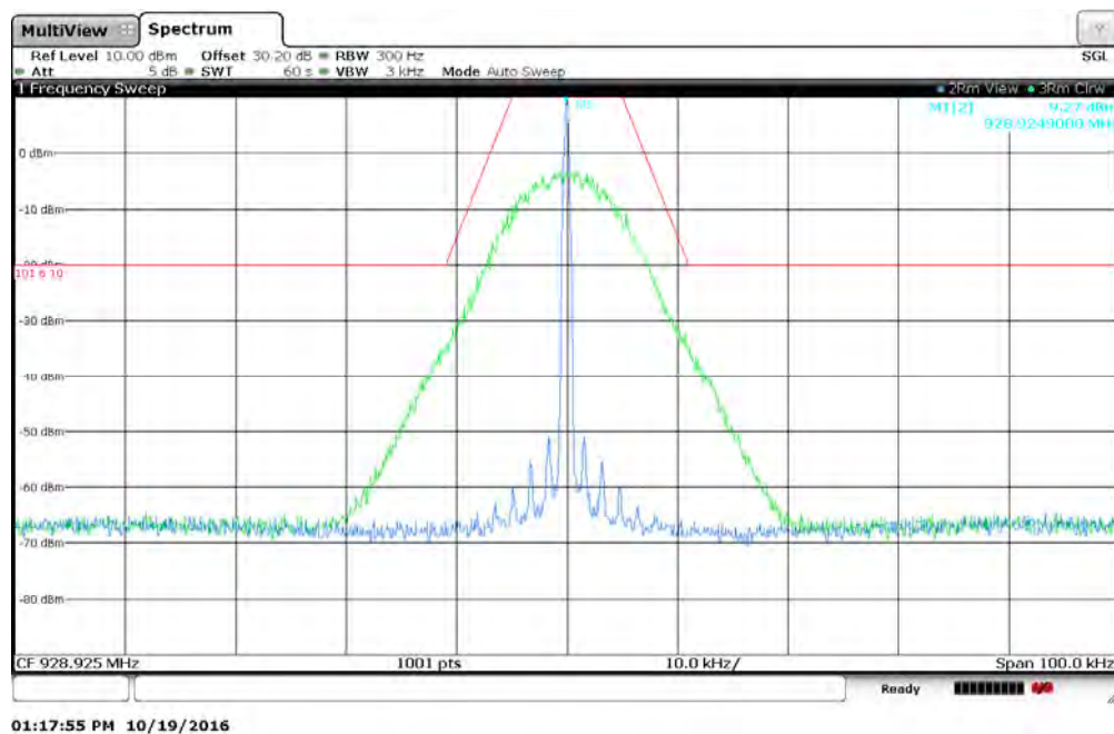
Figure 7.2.2-78: 928.925 MHz – 25 kHz Channel Spacing - 4FSK Mode
