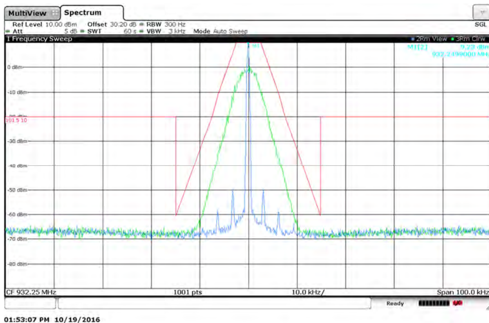
Figure 7.2.2-96: 932.25 MHz – 12.5 kHz Channel Spacing - 8FSK (Half Baud) Mode
