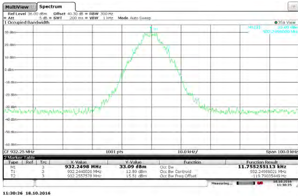
Figure 7.3.2-40: 932.25 MHz – Normal Mode
