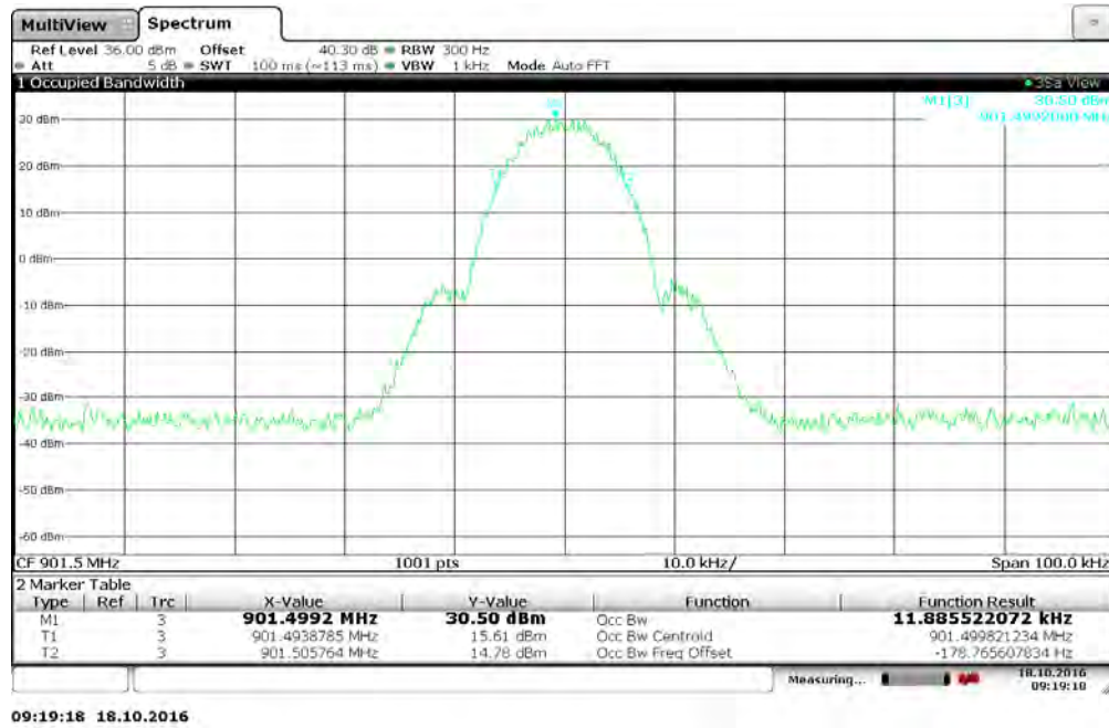
Figure 7.3.2-1: 901.5 MHz – 2FSK Mode
