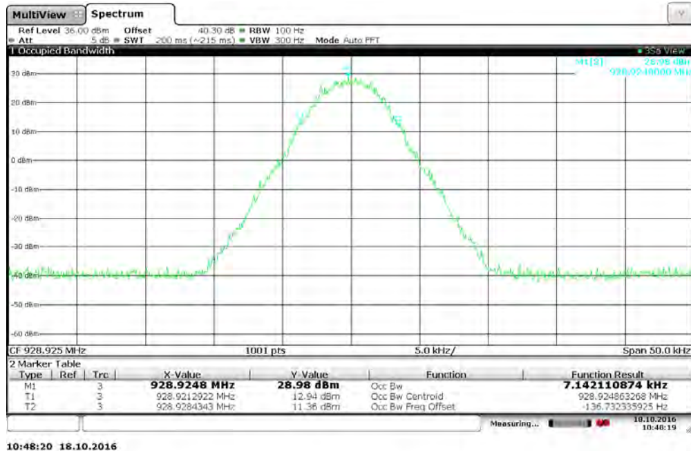
Figure 7.3.2-24: 928.925 MHz – 4FSK (Half Baud) Mode
