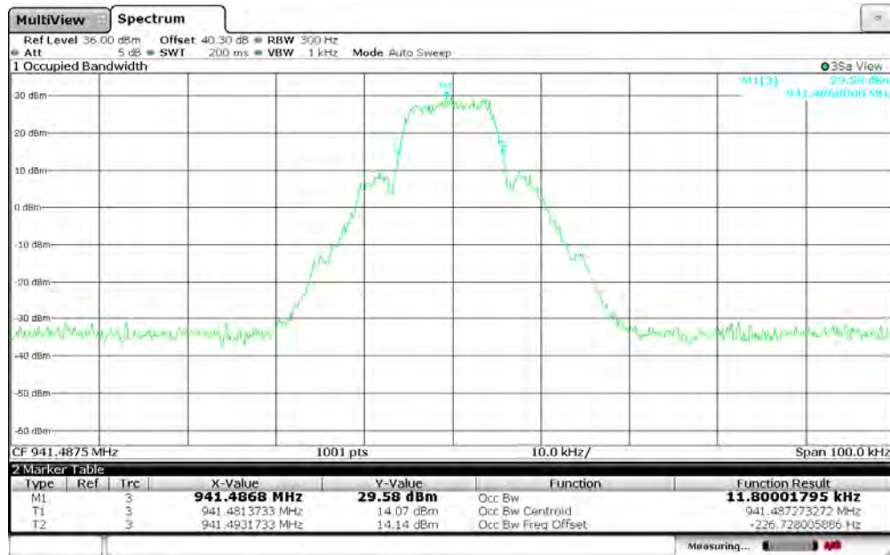
Figure 7.3.2-45: 941.4875 MHz – MPass 10k Mode
