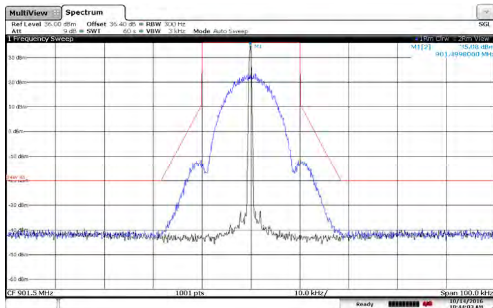
Figure 7.2.2-2: 901.5 MHz – 25 kHz Channel Spacing – 2FSK Mode
