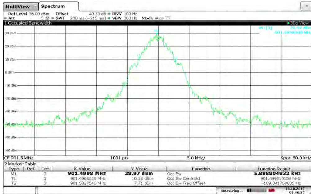
Figure 7.3.2-8: 901.5 MHz – C&amp;I (Half Baud) Mode
