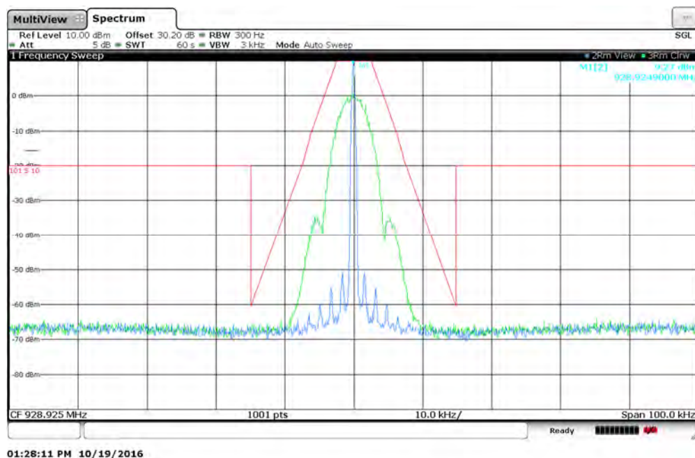
Figure 7.2.2-83: 928.925 MHz -- 12.5 kHz Channel Spacing - 2FSK (Half Baud) Mode
