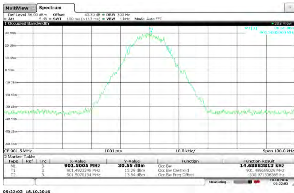
Figure 7.3.2-3: 901.5 MHz – 8FSK Mode
