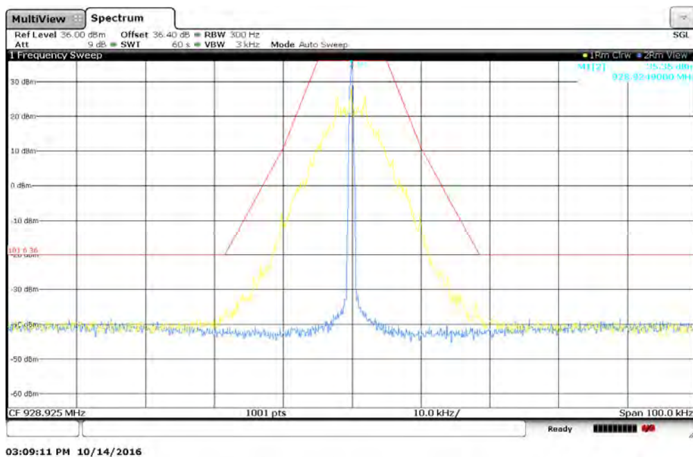
Figure 7.2.2-26: 928.925 MHz – 25 kHz Channel Spacing - Normal Mode
