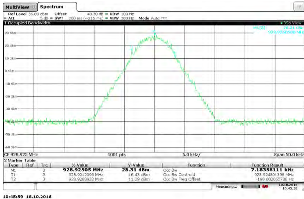
Figure 7.3.2-25: 928.925 MHz – 8FSK (Half Baud) Mode
