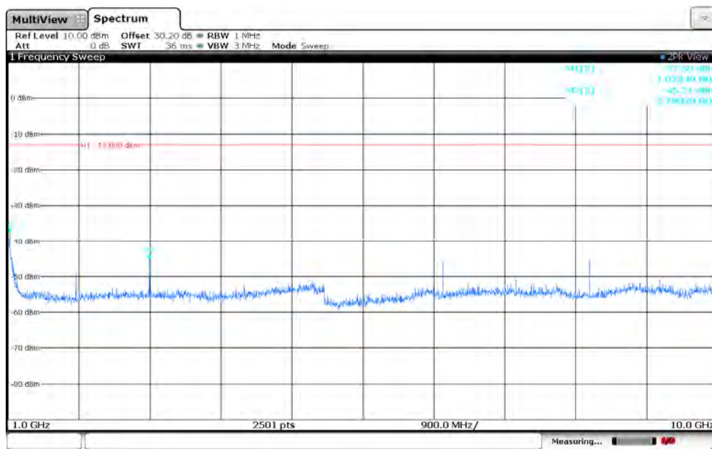
Figure 7.4.2-20: 930.5 MHz – 1GHz to 10GHz
