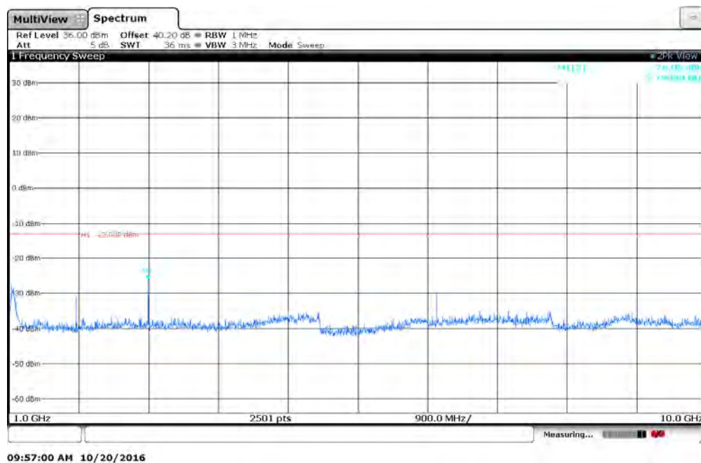
Figure 7.4.2-4: 930.5 MHz – 1GHz to 10GHz – Mpass 5k mode
