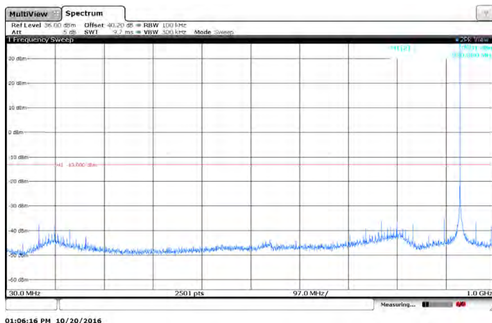
Figure 7.4.2-3: 930.5 MHz – 30MHz to 1GHz – Mpass5k mode
