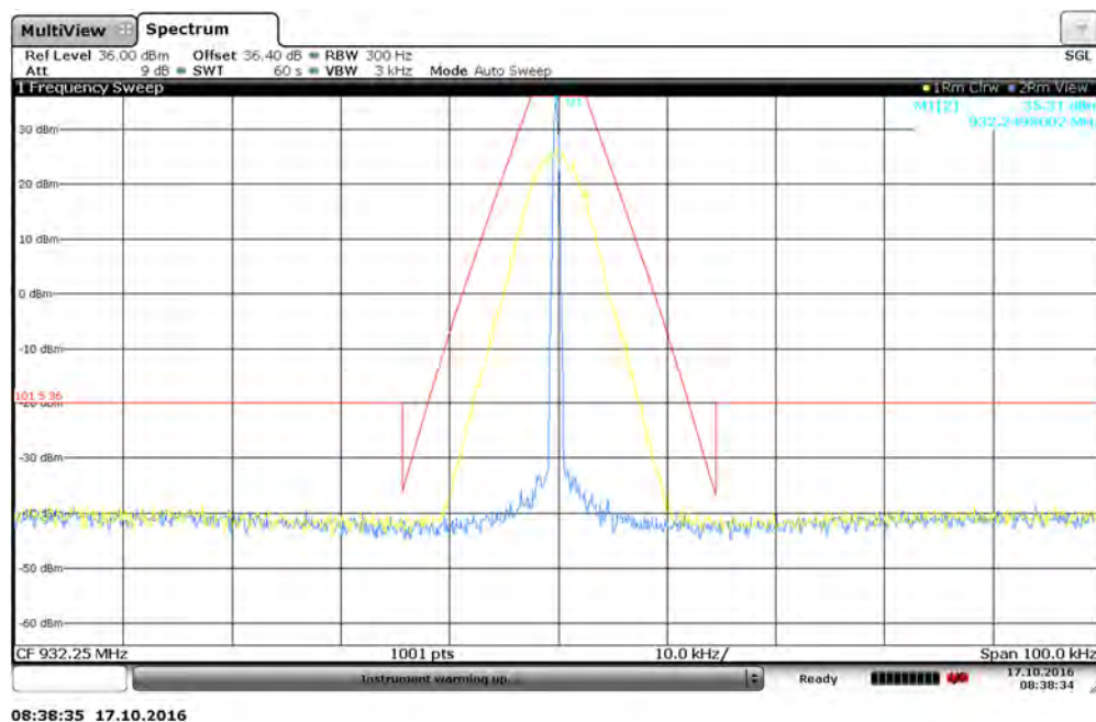
Figure 7.2.2-42: 932.25 MHz – 12.5 kHz Channel Spacing - 8SFSK (Half Baud) Mode
