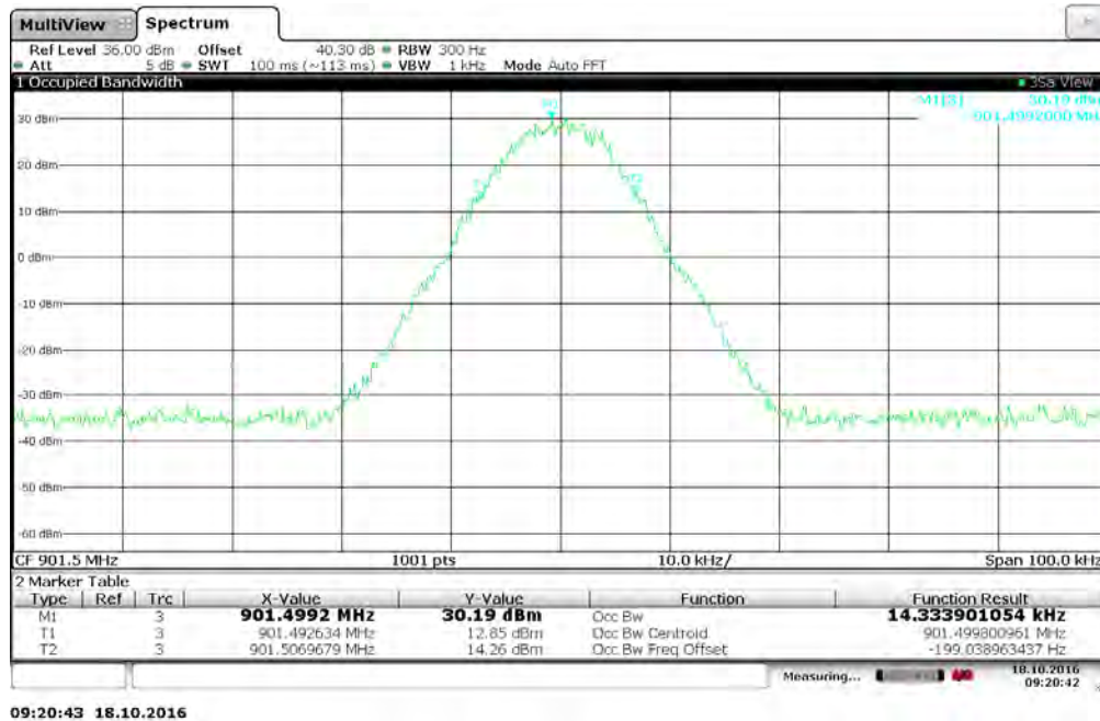
Figure 7.3.2-2: 901.5 MHz – 4FSK Mode
