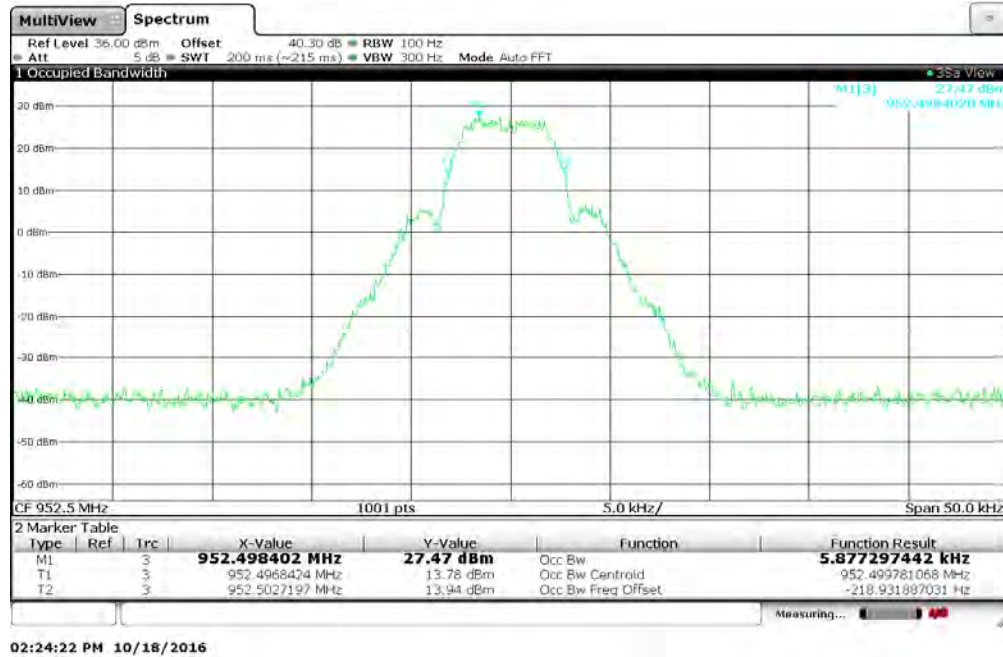
Figure 7.3.2-48: 952.5 MHz – MPass 5k Mode
