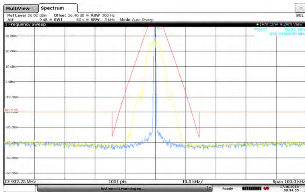
Figure 7.2.2-40: 932.25 MHz –12.5 kHz Channel Spacing - 2SFSK (Half Baud) Mode
