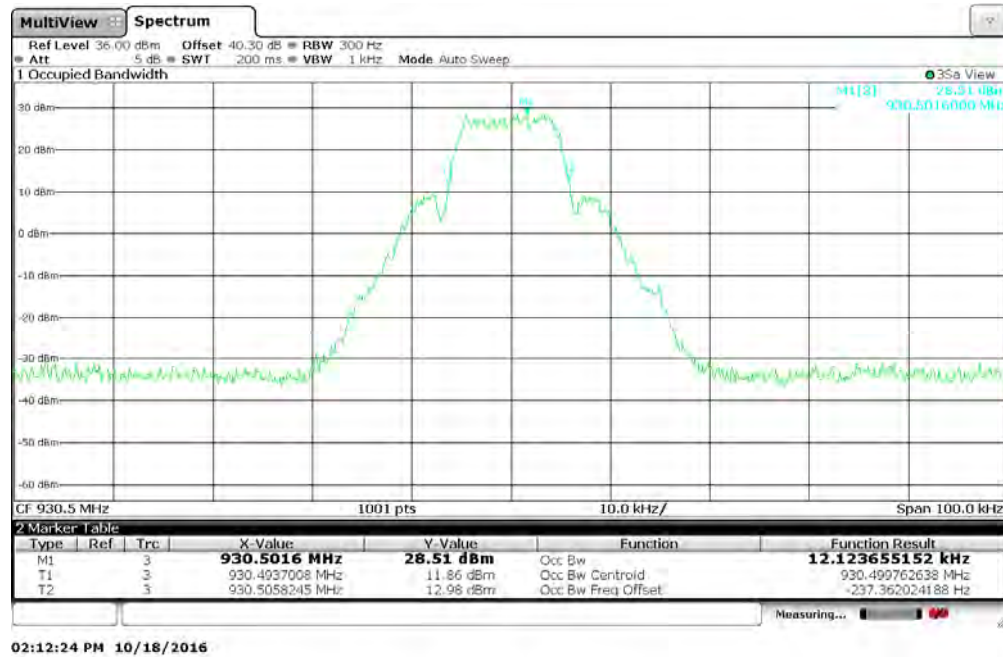
Figure 7.3.2-15: 930.5 MHz – MPass 10k Mode
