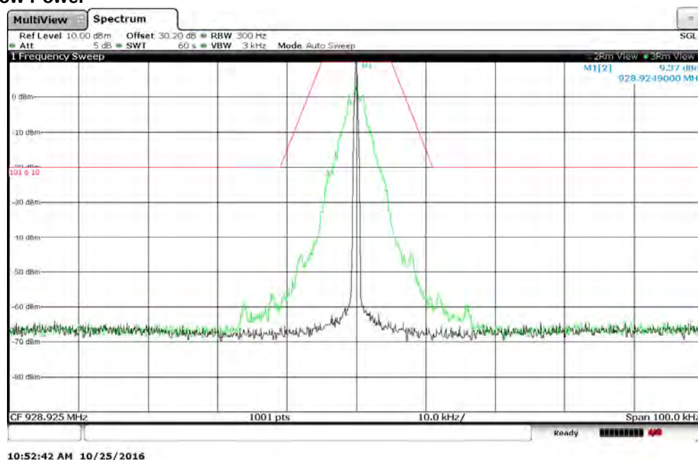
Figure 7.2.2-75: 928.925 MHz – 25 kHz Channel Spacing - C&amp;I Mode
