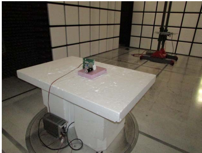
Figure 4: Below 1 GHz
