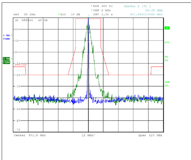
Figure 7.2.2-2: 901.5 MHz – 25 kHz Channel Spacing – C&amp;I Mode
