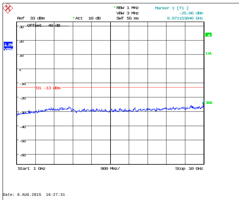
Figure 7.3.2-36: 952.5 MHz – 1GHz to 10GHz (KDS TCXO)
