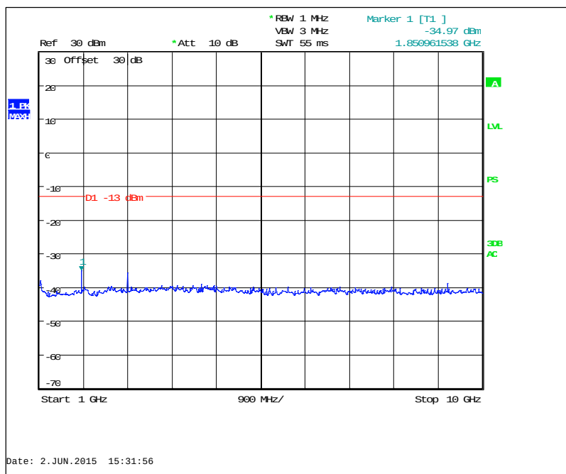
Figure 7.3.2-16: 930.5 MHz – 1GHz to 10GHz (Taitien TCXO)
