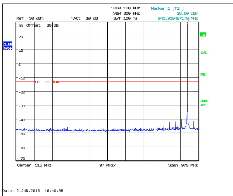
Figure 7.3.2-17: 940.0125 MHz – 30MHz to 1GHz (Taitien TCXO)
