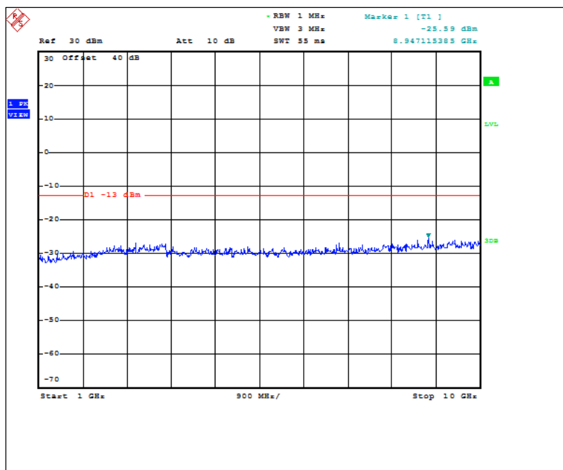
Figure 7.3.2-26: 952.5 MHz – 1GHz to 10GHz (ILSI TCXO)
