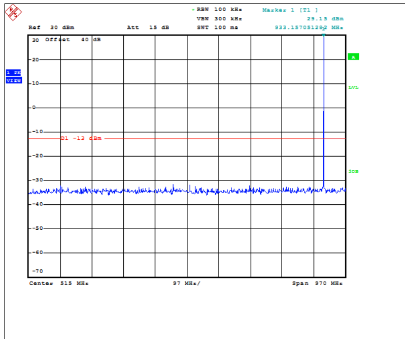
Figure 7.3.2-21: 932.25 MHz – 30MHz to 1GHz (ILSI TCXO)
