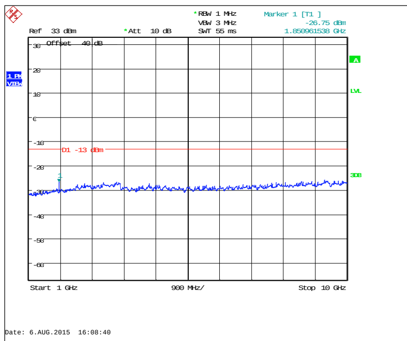
Figure 7.3.2-10: 930.5 MHz – 1GHz to 10GHz (KDS TCXO)
