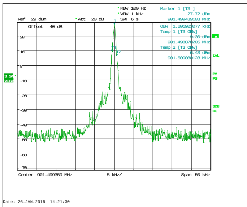
Figure 7.2.3-4: 901.5 MHz – Boost Mode
