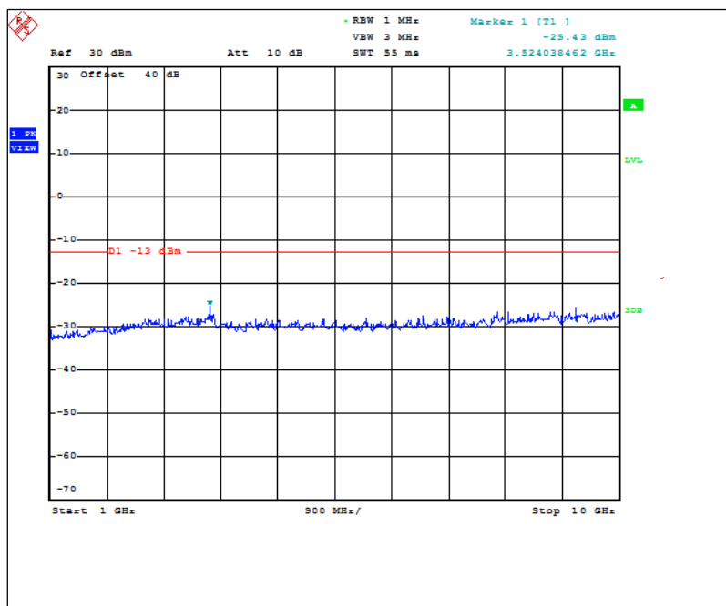
Figure 7.3.2-4: 930.5 MHz – 1GHz to 10GHz (ILSI TCXO)
