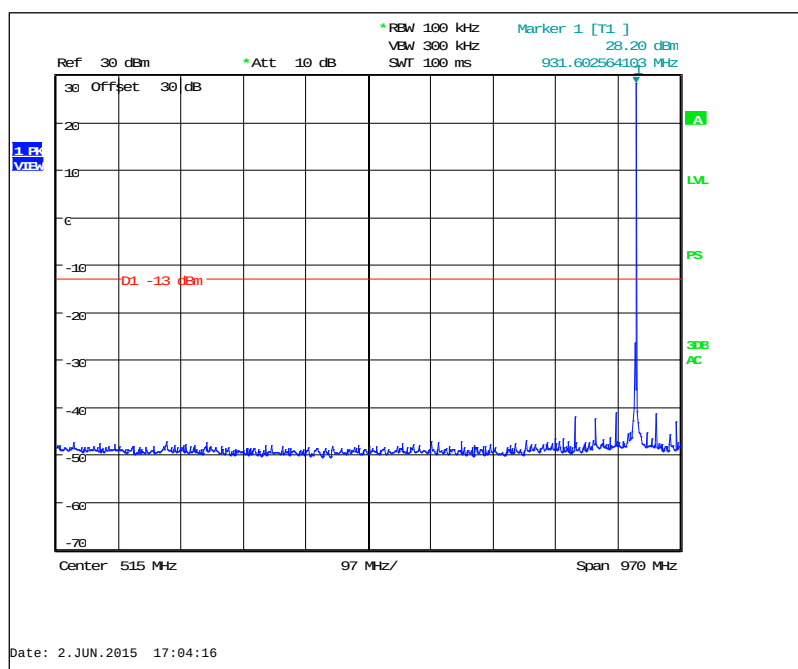
Figure 7.3.2-15: 930.5 MHz – 30MHz to 1GHz (Taitien TCXO)
