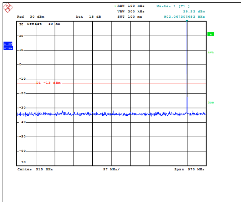
Figure 7.3.2-1: 901.5 MHz – 30MHz to 1GHz (ILSI TCXO)
