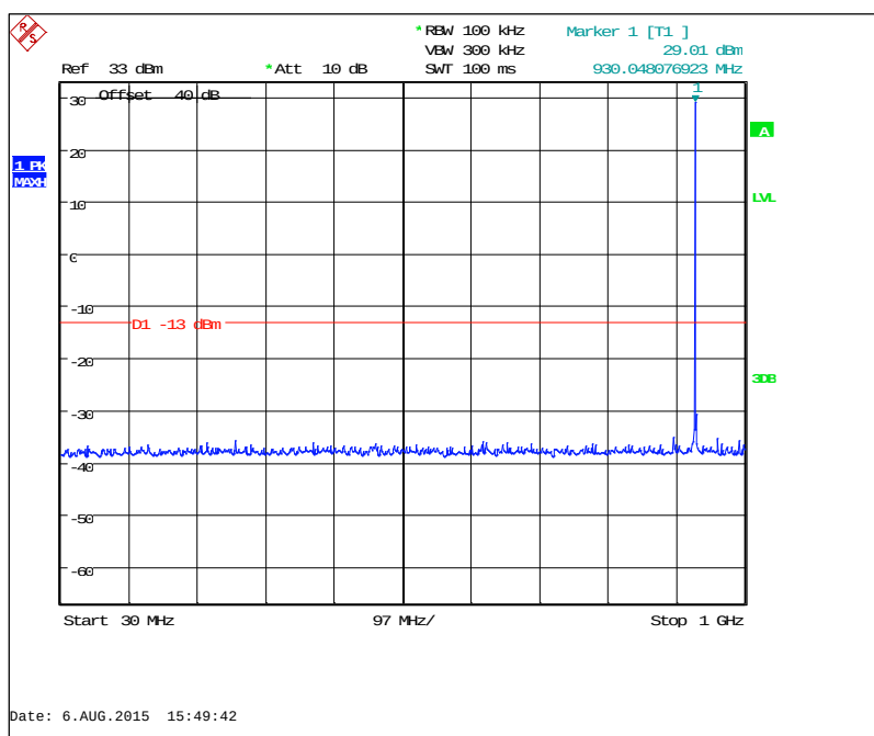
Figure 7.3.2-29: 928.925 MHz – 30MHz to 1GHz (KDS TCXO)
