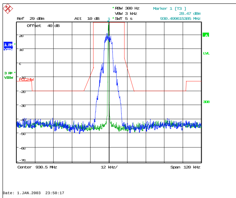
Figure 7.2.2-11: 930.5 MHz – 25 kHz Channel Spacing – mPass 5k Mode
