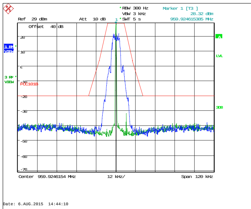
Figure 7.2.2-32: 959.925 MHz – mPass 5k Mode
