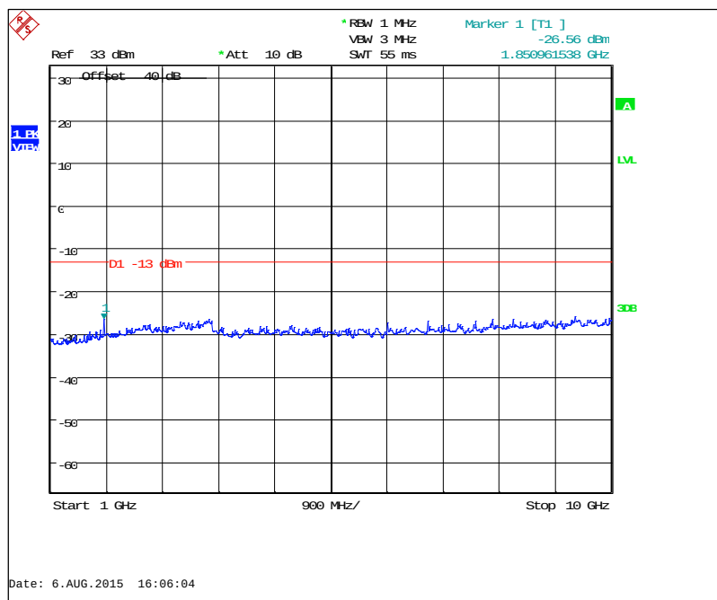
Figure 7.3.2-30: 928.925 MHz – 1GHz to 10GHz (KDS TCXO)
