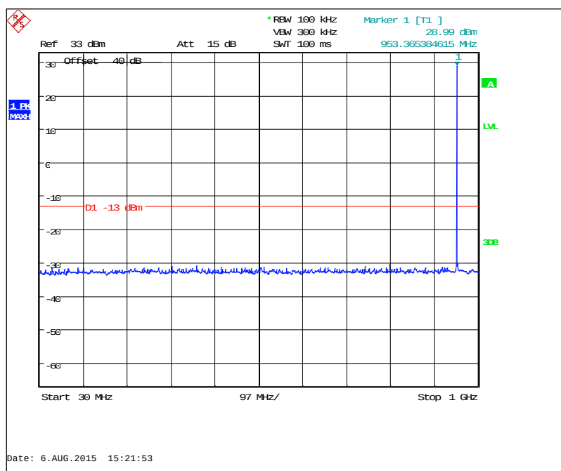
Figure 7.3.2-35 952.5 MHz – 30MHz to 1GHz (KDS TCXO)
