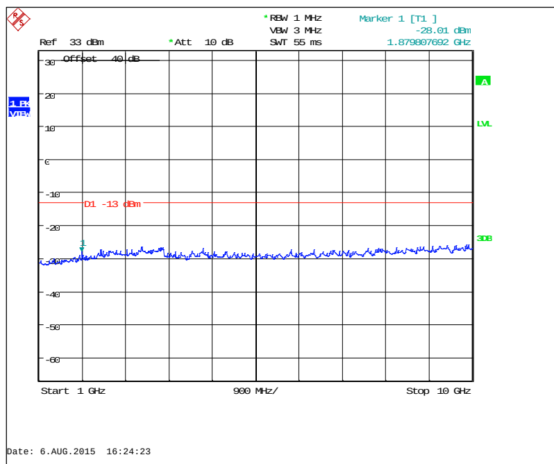
Figure 7.3.2-34: 941.4875 MHz – 1GHz to 10GHz (KDS TCXO)
