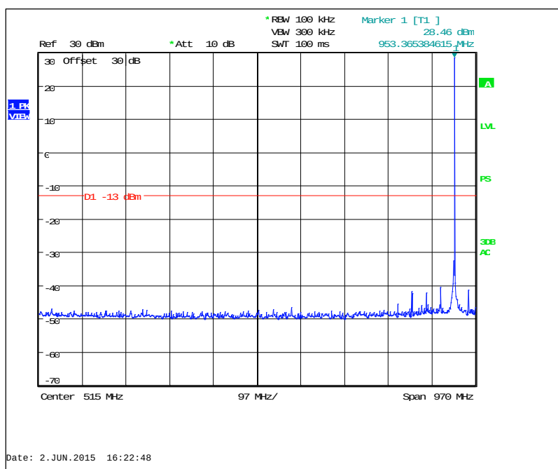
Figure 7.3.2-45 952.5 MHz – 30MHz to 1GHz (Taitien TCXO)
