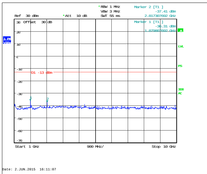
Figure 7.3.2-44: 941.4875 MHz – 1GHz to 10GHz (Taitien TCXO)
