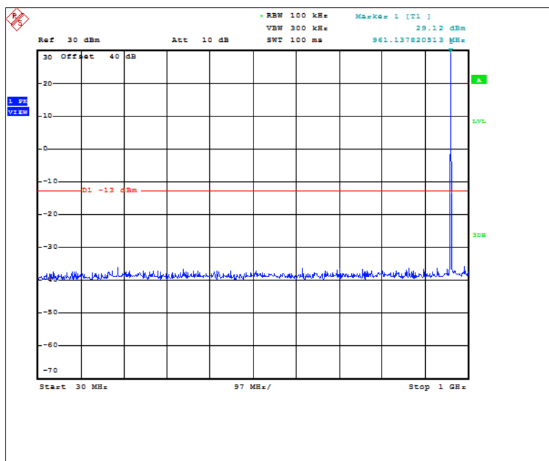
Figure 7.3.2-27: 959.925 MHz – 30MHz to 1GHz (ILSI TCXO)
