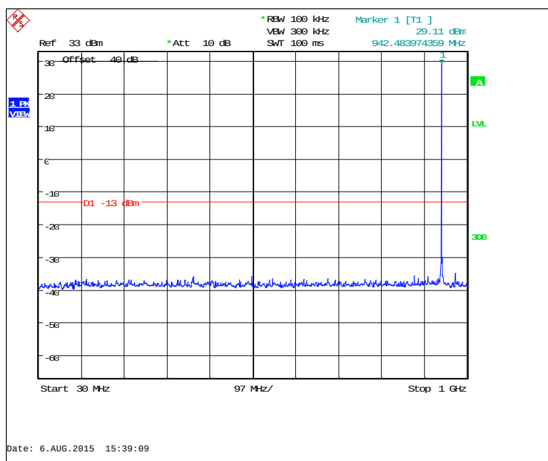
Figure 7.3.2-33: 941.4875 MHz – 30MHz to 1GHz (KDS TCXO)
