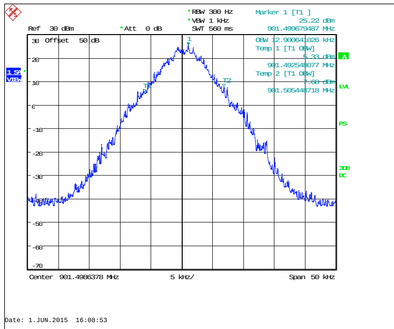
Figure 7.2.3-2: 901.5 MHz – Double Density Mode
