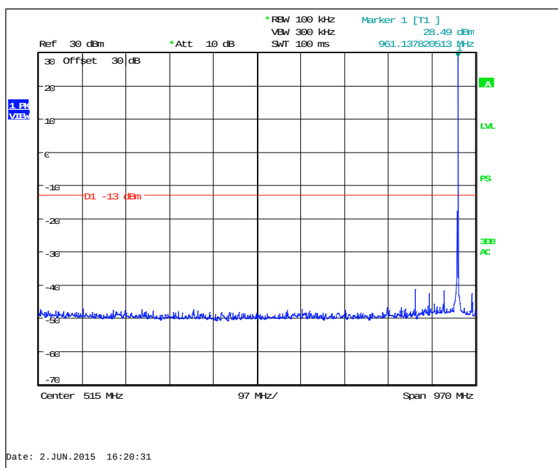
Figure 7.3.2-47: 959.925 MHz – 30MHz to 1GHz (Taitien TCXO)
