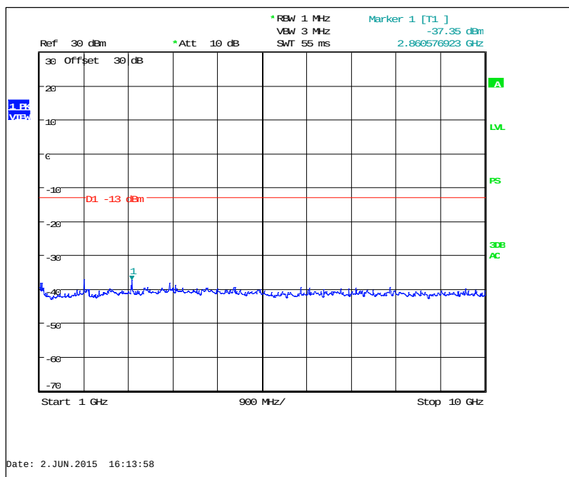
Figure 7.3.2-46: 952.5 MHz – 1GHz to 10GHz (Taitien TCXO)
