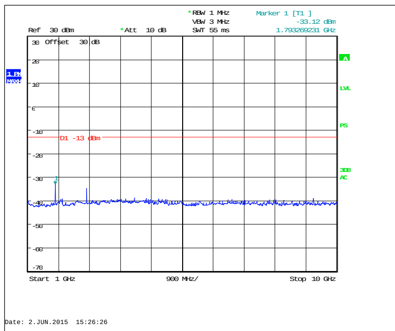
Figure 7.3.2-14: 901.5 MHz – 1GHz to 10GHz (Taitien TCXO)
