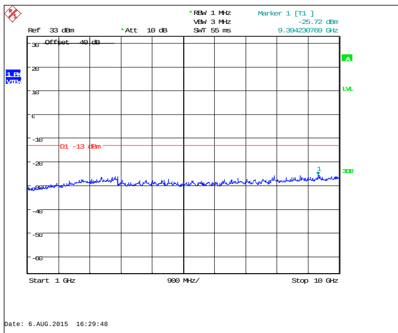
Figure 7.3.2-38: 959.925 MHz – 1GHz to 10GHz (KDS TCXO)
