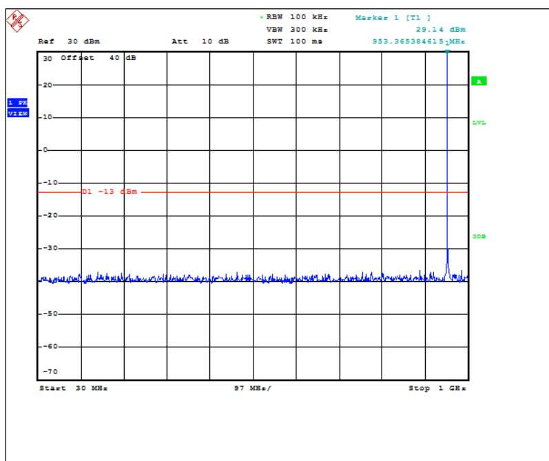
Figure 7.3.2-25: 952.5 MHz – 30MHz to 1GHz (ILSI TCXO)
