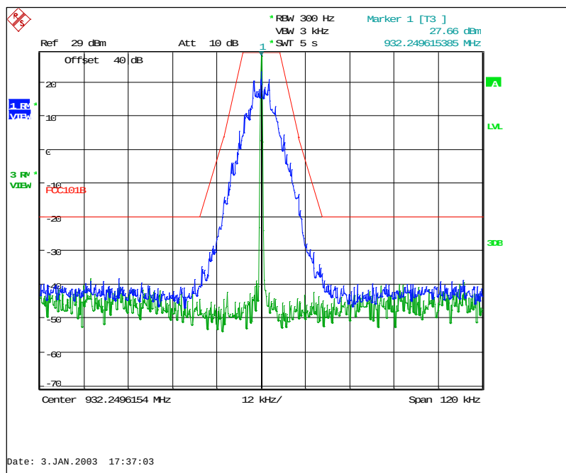
Figure 7.2.2-26: 932.25 MHz – Normal Mode
