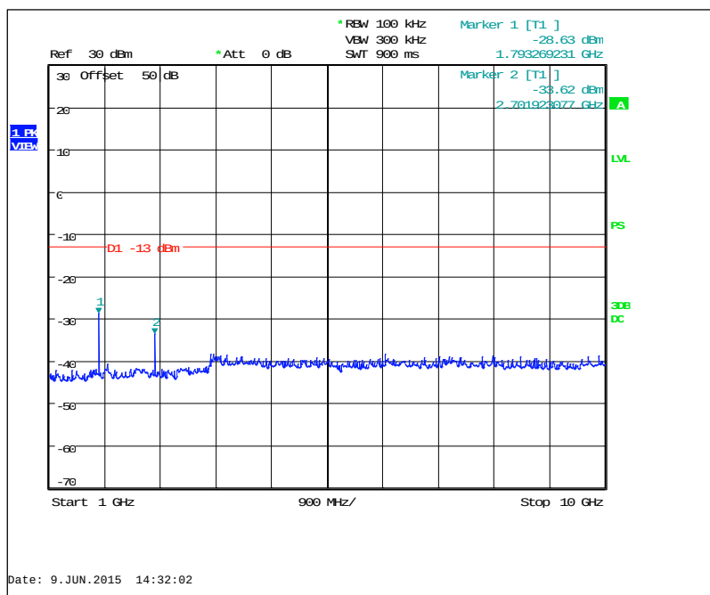
Figure 7.3.2-8: 901.5 MHz – 1GHz to 10GHz (KDS TCXO)
