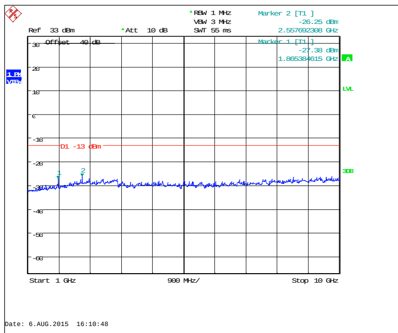
Figure 7.3.2-32: 932.25 MHz – 1GHz to 10GHz (KDS TCXO)
