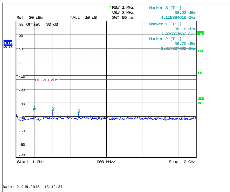
Figure 7.3.2-18: 940.0125 MHz – 1GHz to 10GHz (Taitien TCXO)
