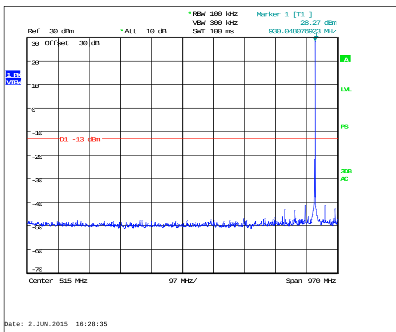
Figure 7.3.2-39: 928.925 MHz – 30MHz to 1GHz (Taitien TCXO)
