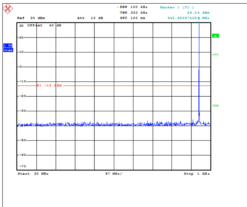
Figure 7.3.2-23: 941.4875 MHz – 30MHz to 1GHz (ILSI TCXO)
