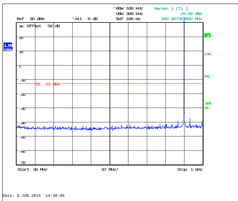
Figure 7.3.2-7: 901.5 MHz – 30MHz to 1GHz (KDS TCXO)
