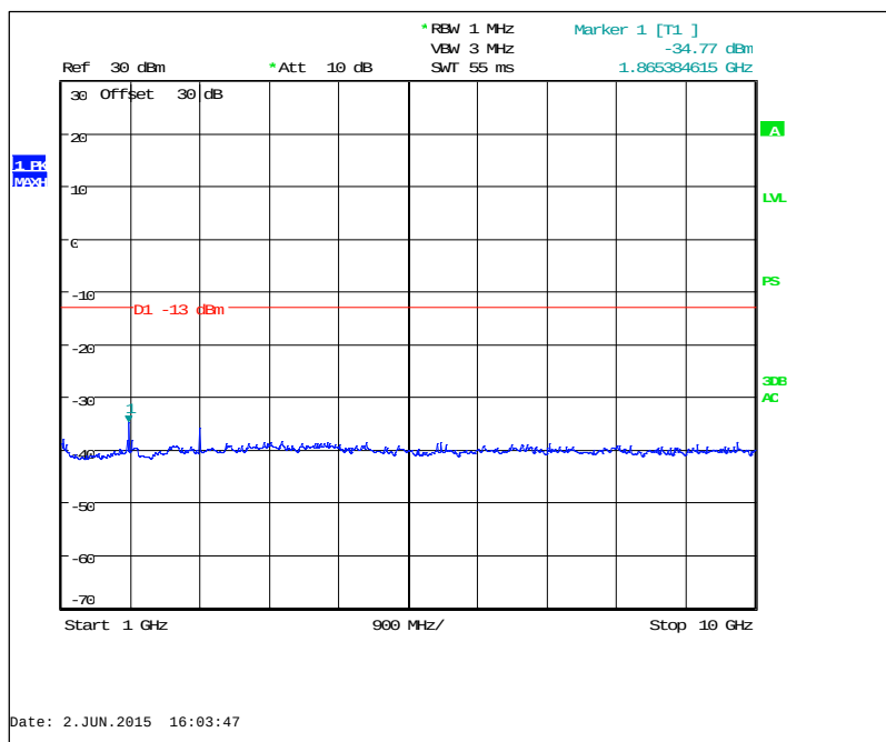
Figure 7.3.2-42: 932.25 MHz – 1GHz to 10GHz (Taitien TCXO)
