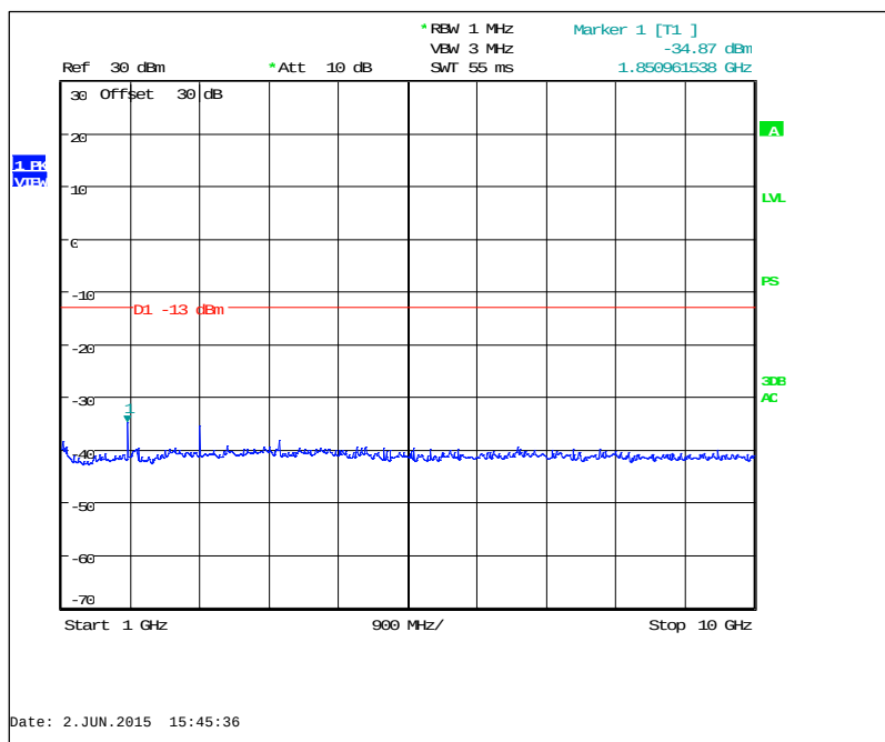
Figure 7.3.2-40: 928.925 MHz – 1GHz to 10GHz (Taitien TCXO)
