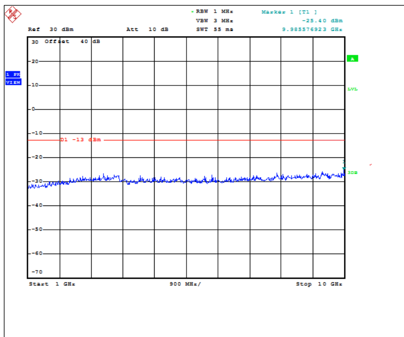
Figure 7.3.2-22: 932.25 MHz – 1GHz to 10GHz (ILSI TCXO)
