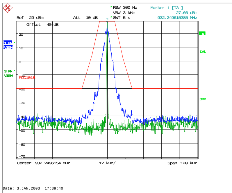
Figure 7.2.2-22: 932.25 MHz – C&amp;I Mode
