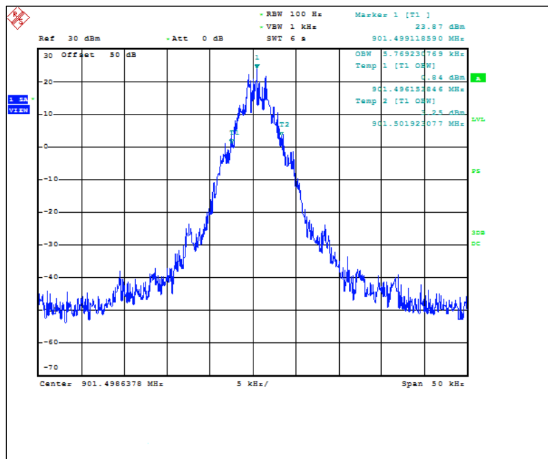
Figure 7.2.3-1: 901.5 MHz – C&amp;I Mode
