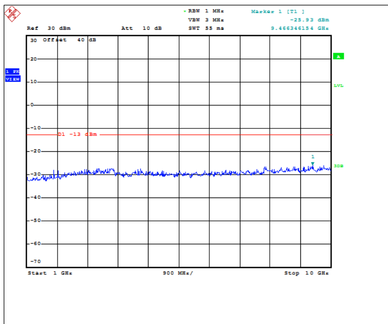
Figure 7.3.2-2: 901.5 MHz – 1GHz to 10GHz (ILSI TCXO)
