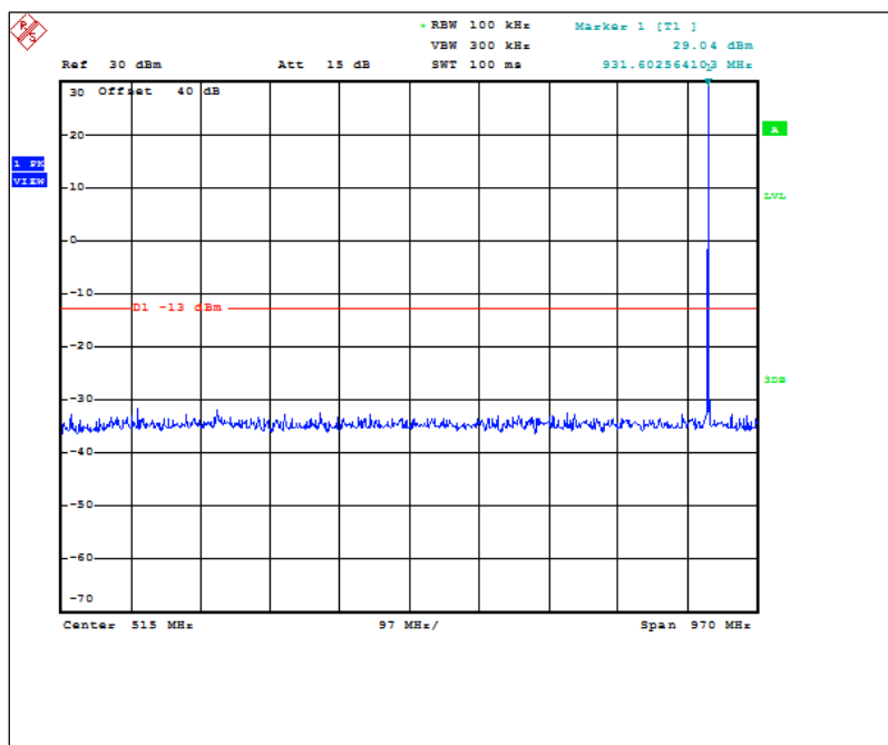
Figure 7.3.2-3: 930.5 MHz – 30MHz to 1GHz (ILSI TCXO)
