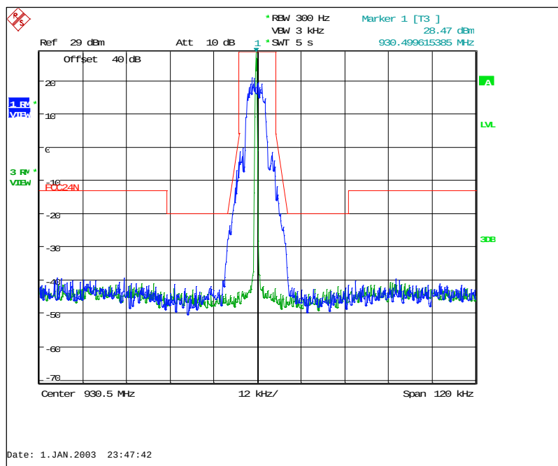
Figure 7.2.2-10: 930.5 MHz - 12.5 kHz Channel Spacing – mPass 5k Mode
