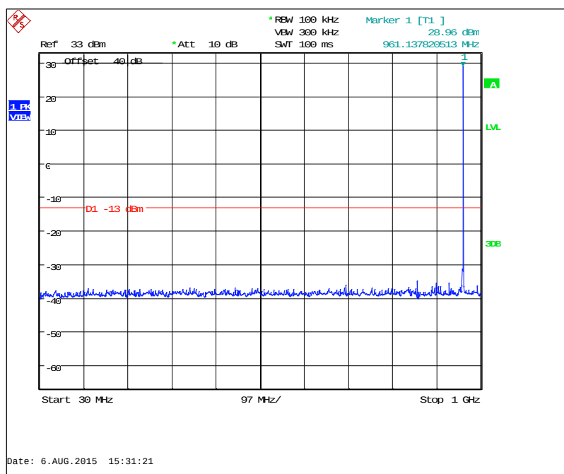
Figure 7.3.2-37: 959.925 MHz – 30MHz to 1GHz (KDS TCXO)
