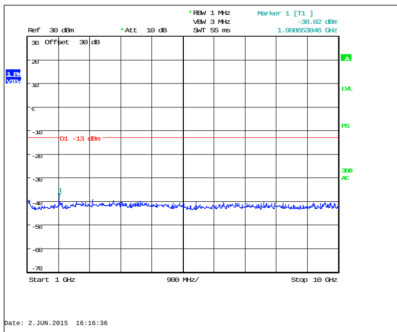
Figure 7.3.2-48: 959.925 MHz – 1GHz to 10GHz (Taitien TCXO)
