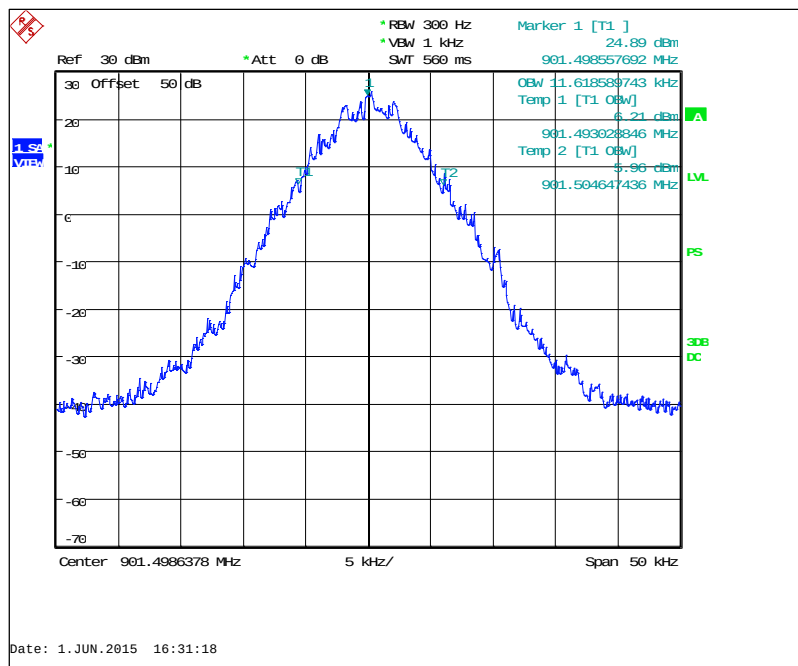
Figure 7.2.3-3: 901.5 MHz – Normal Mode
