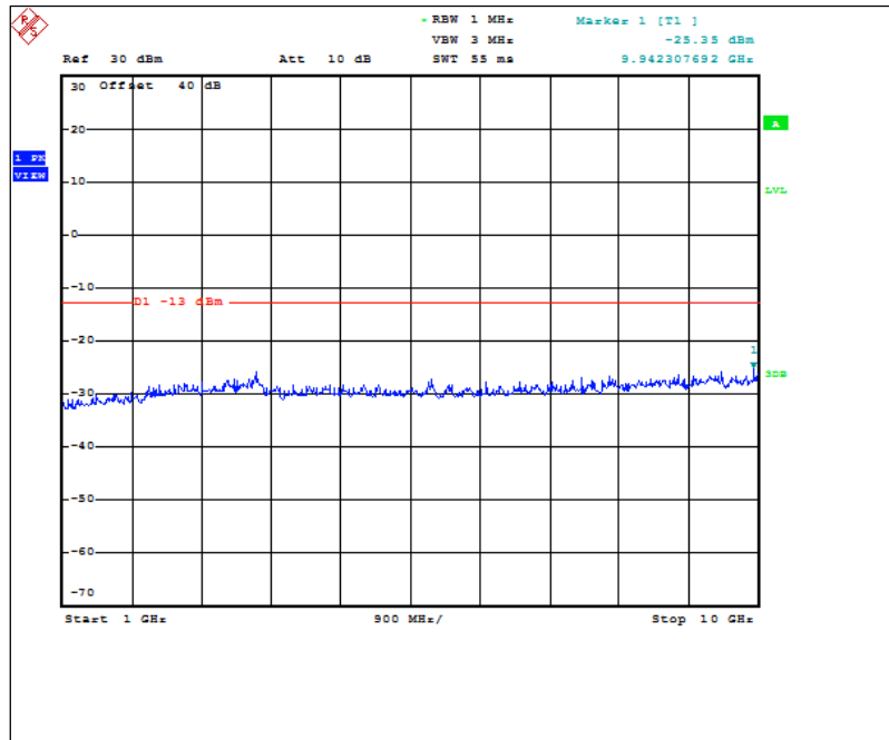
Figure 7.3.2-20: 928.925 MHz – 1GHz to 10GHz (ILSI TCXO)
