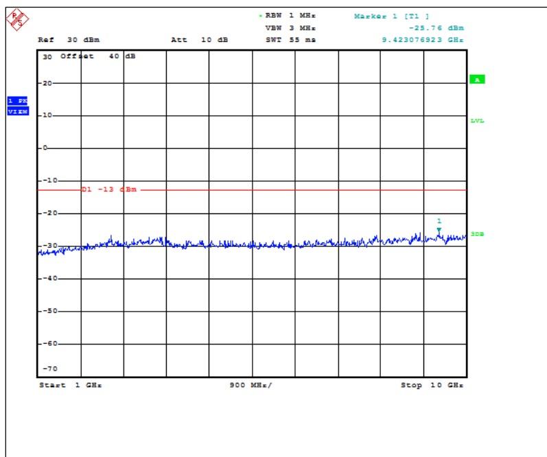
Figure 7.3.2-24: 941.4875 MHz – 1GHz to 10GHz (ILSI TCXO)
