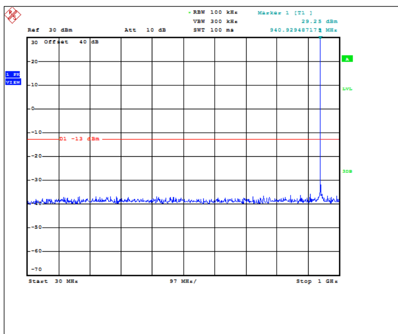
Figure 7.3.2-5: 940.0125 MHz – 30MHz to 1GHz (ILSI TCXO)
