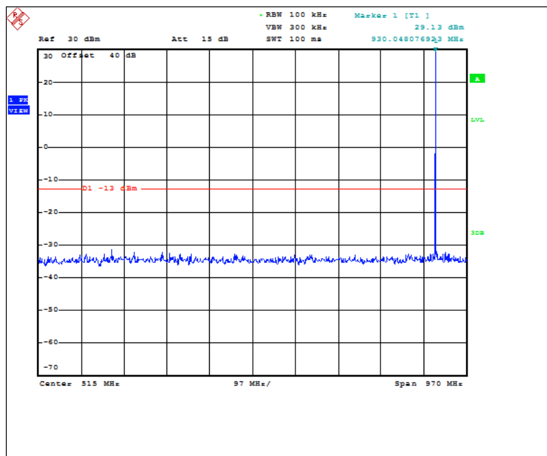
Figure 7.3.2-19: 928.925 MHz – 30MHz to 1GHz (ILSI TCXO)
