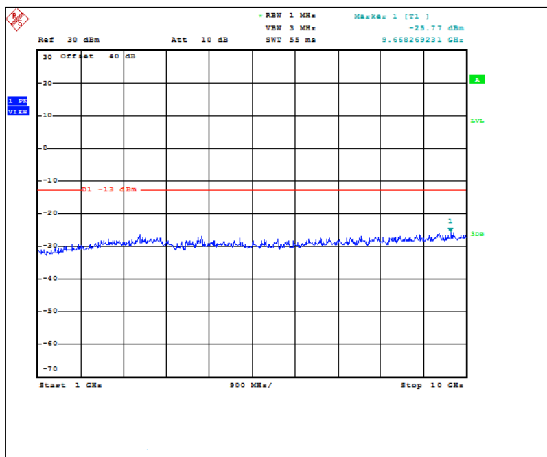
Figure 7.3.2-28: 959.925 MHz – 1GHz to 10GHz (ILSI TCXO)
