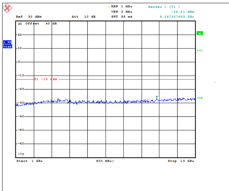
Figure 7.3.2-6: 940.0125 MHz – 1GHz to 10GHz (ILSI TCXO)
