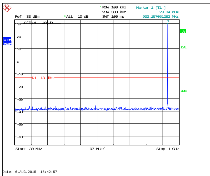
Figure 7.3.2-31: 932.25 MHz – 30MHz to 1GHz (KDS TCXO)
