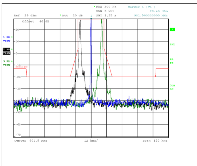
Figure 7.2.2-9: 901.5 MHz – 25 kHz Channel Spacing – Boost Mode Offset Channel of +/- 14 (+/- 8400 Hz)
