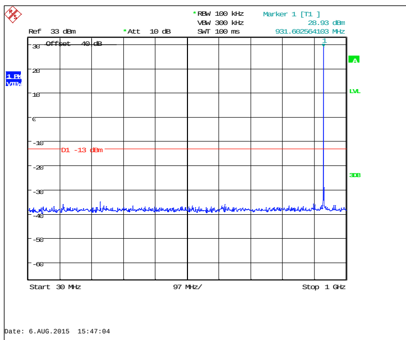
Figure 7.3.2-9: 930.5 MHz – 30MHz to 1GHz (KDS TCXO)
