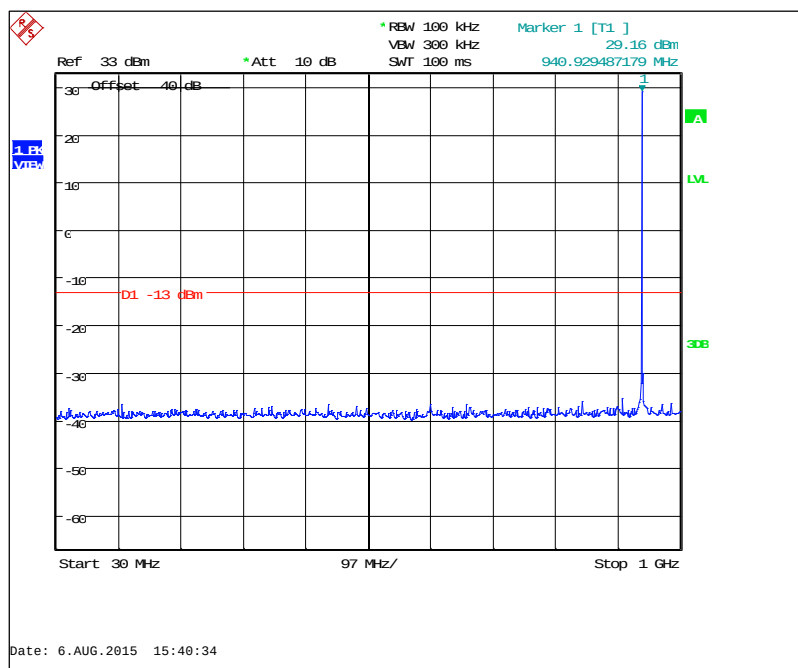
Figure 7.3.2-11: 940.0125 MHz – 30MHz to 1GHz (KDS TCXO)
