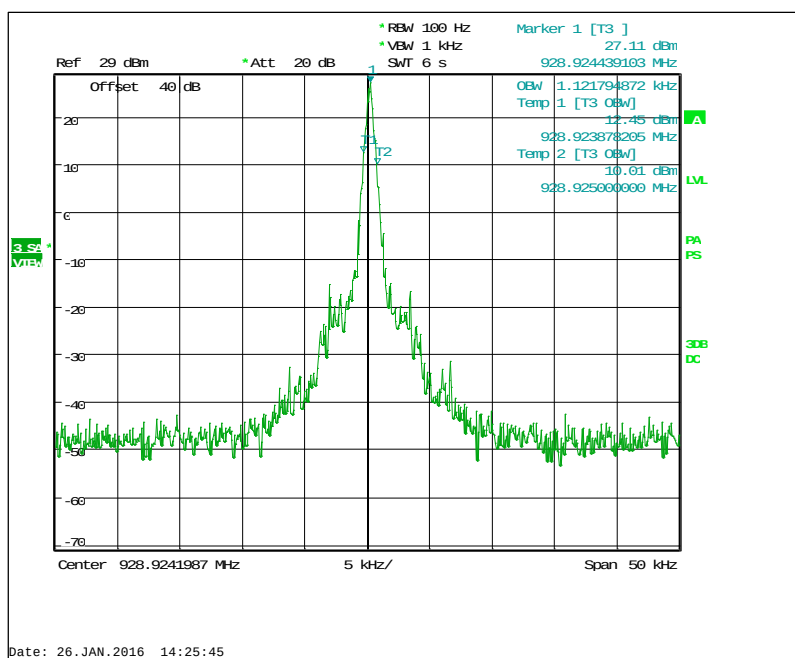
Figure 7.2.3-12: 928.925 MHz -- Boost Mode
