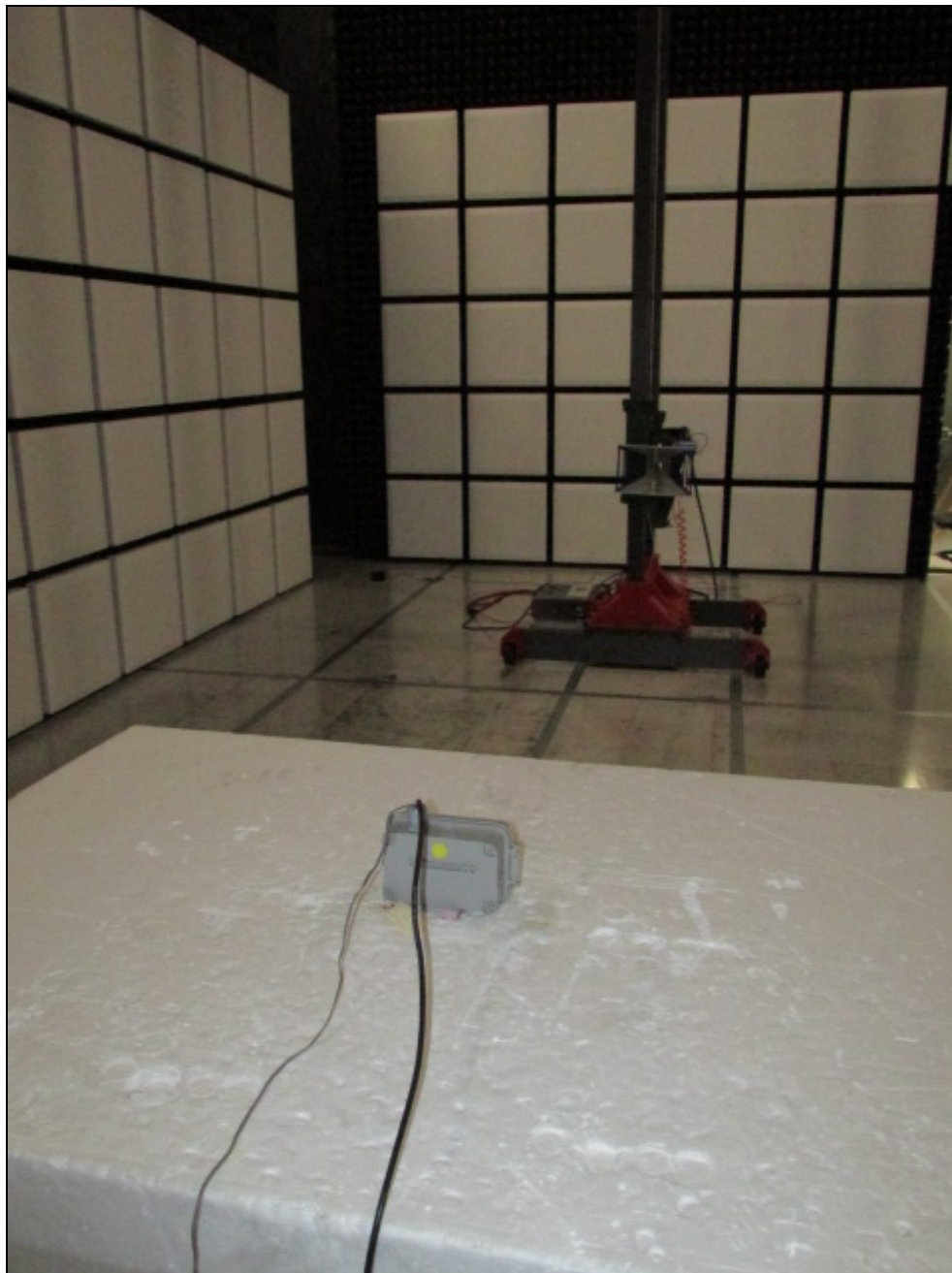
Figure 4: Radiated Emissions – Rear View – Above 1GHz
