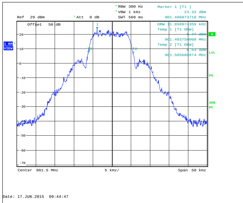
Figure 7.2.3-4: 901.5 MHz – mPass 10k Mode
