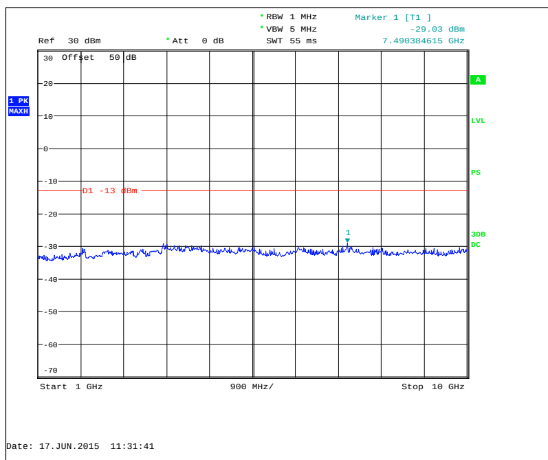
Figure 7.3.2-6: 940.0125 MHz – 1GHz to 10GHz
