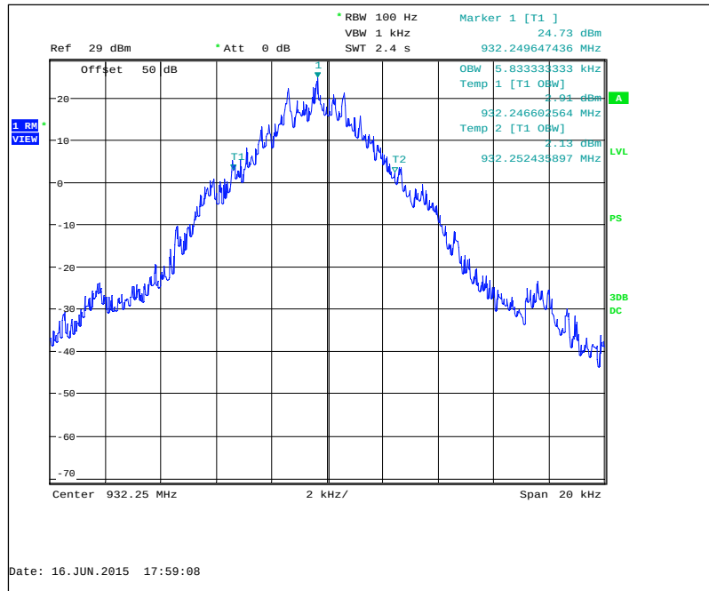
Figure 7.2.3-17: 932.25 MHz – C&amp;I Mode
