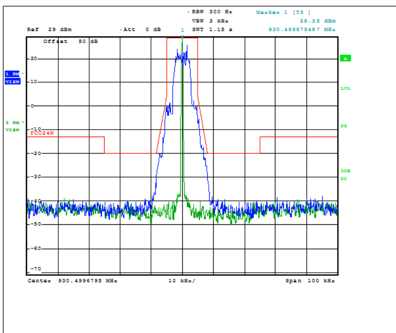
Figure 7.2.2-10: 930.5 MHz - 12.5 kHz Channel Spacing – mPass 5k Mode
