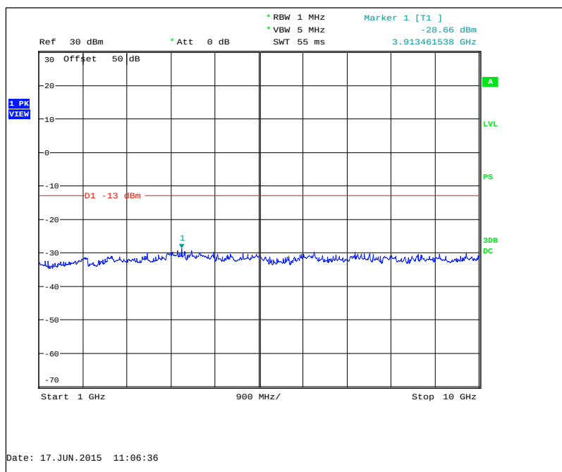
Figure 7.3.2-16: 959.925 MHz – 1GHz to 10GHz
