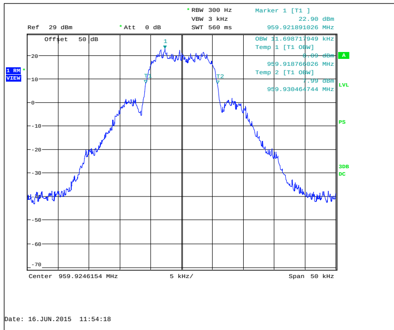
Figure 7.2.3-28: 959.925 MHz – mPass 10k Mode
