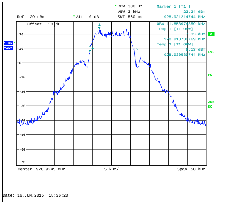
Figure 7.2.3-14: 928.925 MHz – mPass 10k Mode
