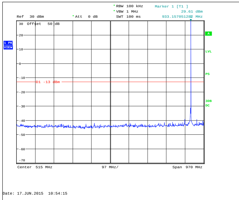
Figure 7.3.2-9: 932.25 MHz – 30MHz to 1GHz
