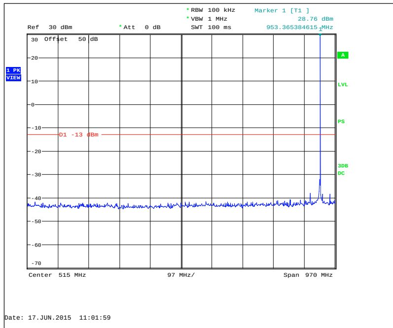
Figure 7.3.2-13: 952.5 MHz – 30MHz to 1GHz
