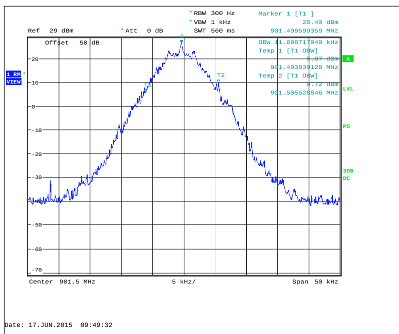
Figure 7.2.3-5: 901.5 MHz – Normal Mode
