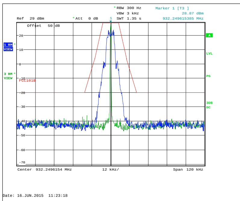
Figure 7.2.2-24: 932.25 MHz – mPass 5k Mode
