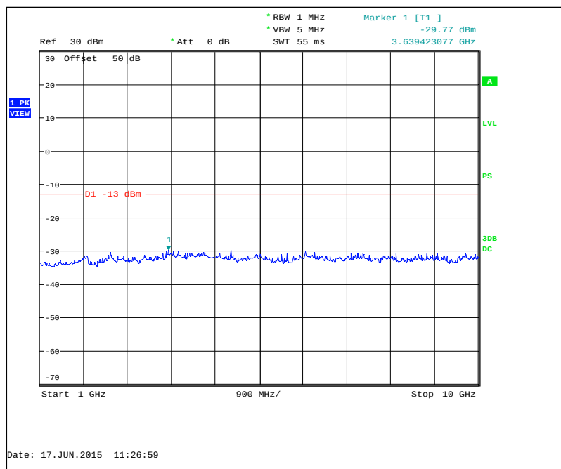
Figure 7.3.2-2: 901.5 MHz – 1GHz to 10GHz
