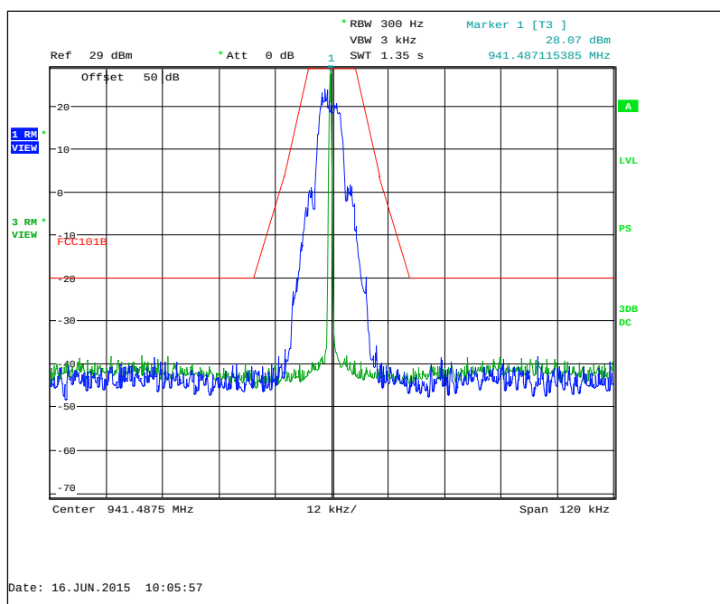
Figure 7.2.2-28: 941.4875 MHz – mPass 5k Mode
