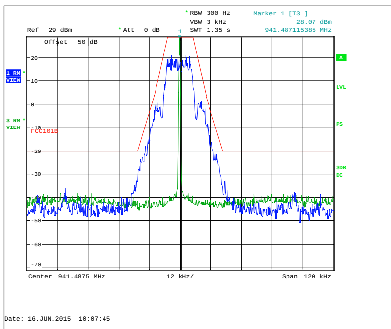
Figure 7.2.2-29: 941.4875 MHz – mPass 10k Mode
