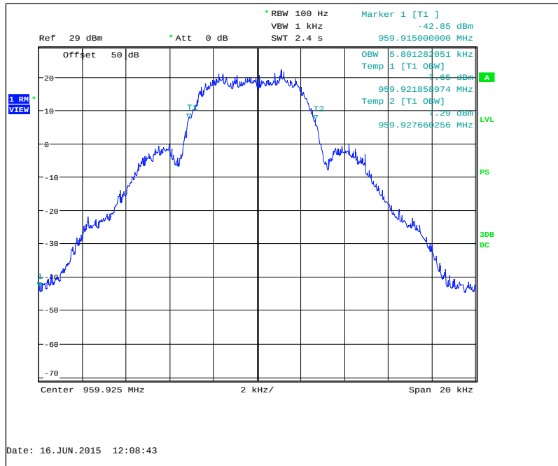
Figure 7.2.3-27: 959.925 MHz – mPass 5k Mode
