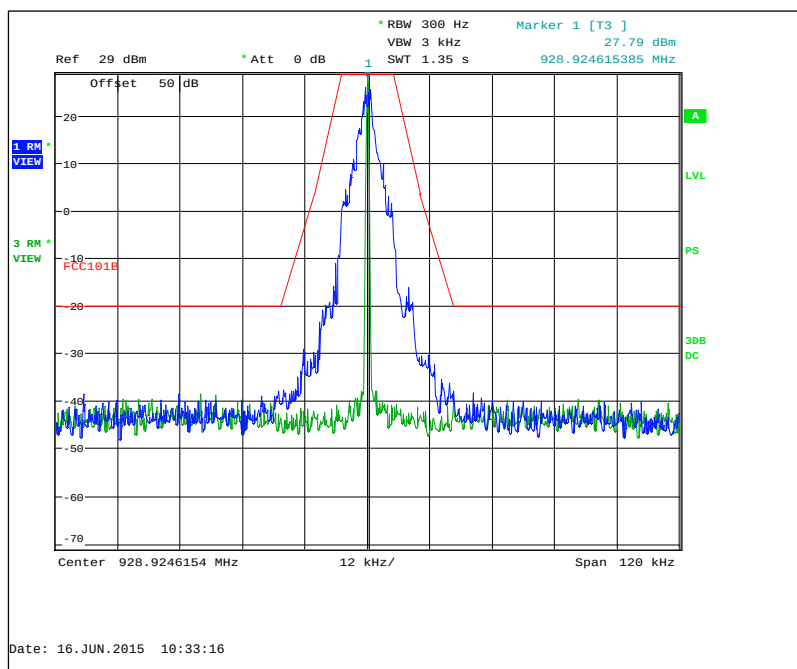
Figure 7.2.2-21: 928.925 MHz -- Priority Mode
