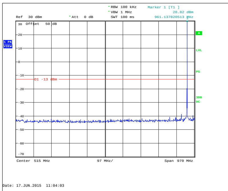
Figure 7.3.2-15: 959.925 MHz – 30MHz to 1GHz
