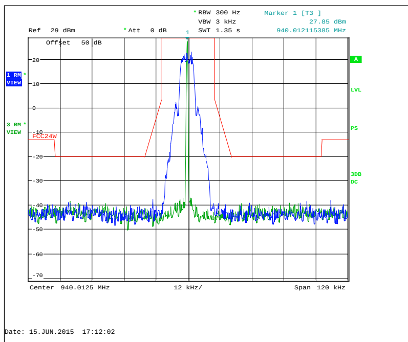
Figure 7.2.2-14: 940.0125 MHz – 25 kHz Channel Spacing – mPass 5k Mode
