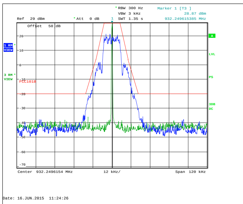
Figure 7.2.2-25: 932.25 MHz – mPass 10k Mode
