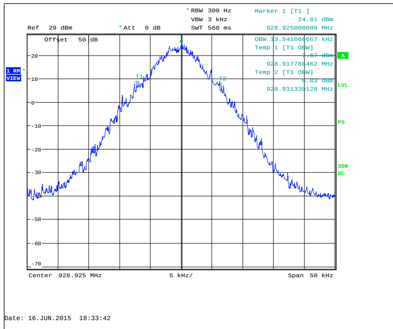
Figure 7.2.3-12: 928.925 MHz – Double Density Mode
