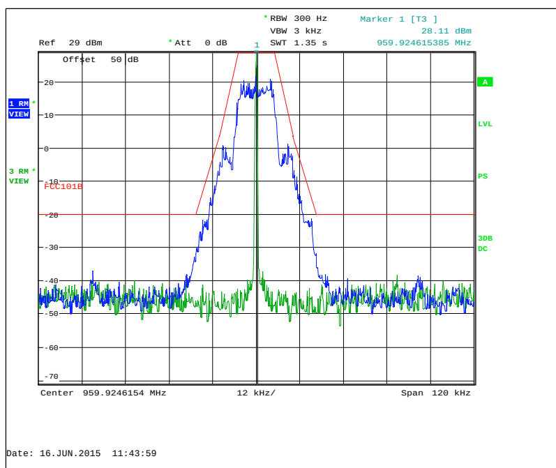
Figure 7.2.2-33: 959.925 MHz – mPass 10k Mode
