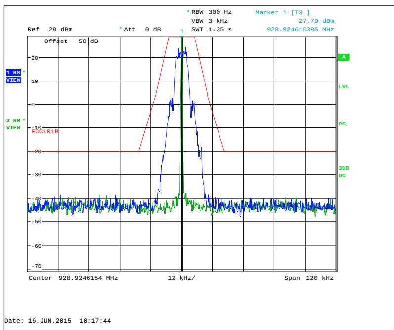
Figure 7.2.2-18: 928.925 MHz – mPass 5k Mode
