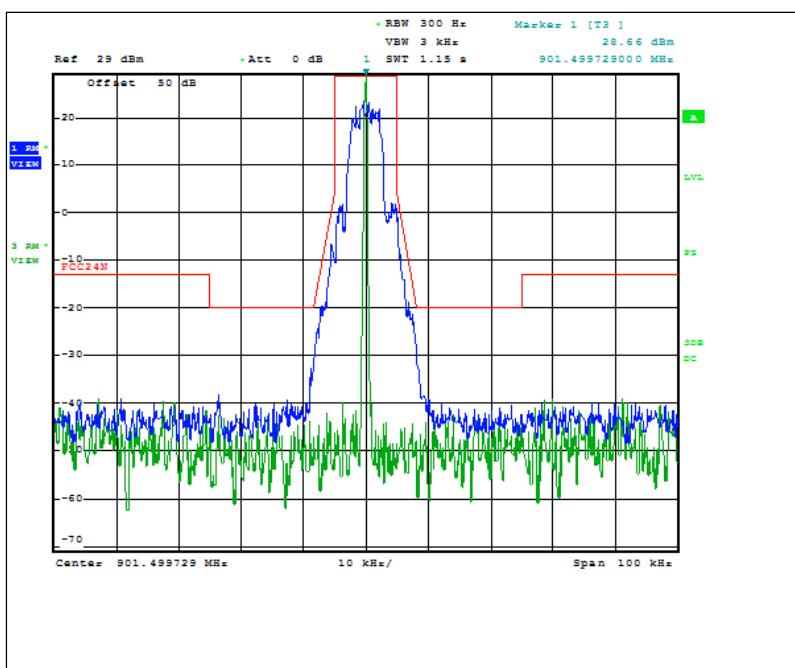
Figure 7.2.2-4: 901.5MHz – 12.5 kHz Channel Spacing – mPass 5k Mode
