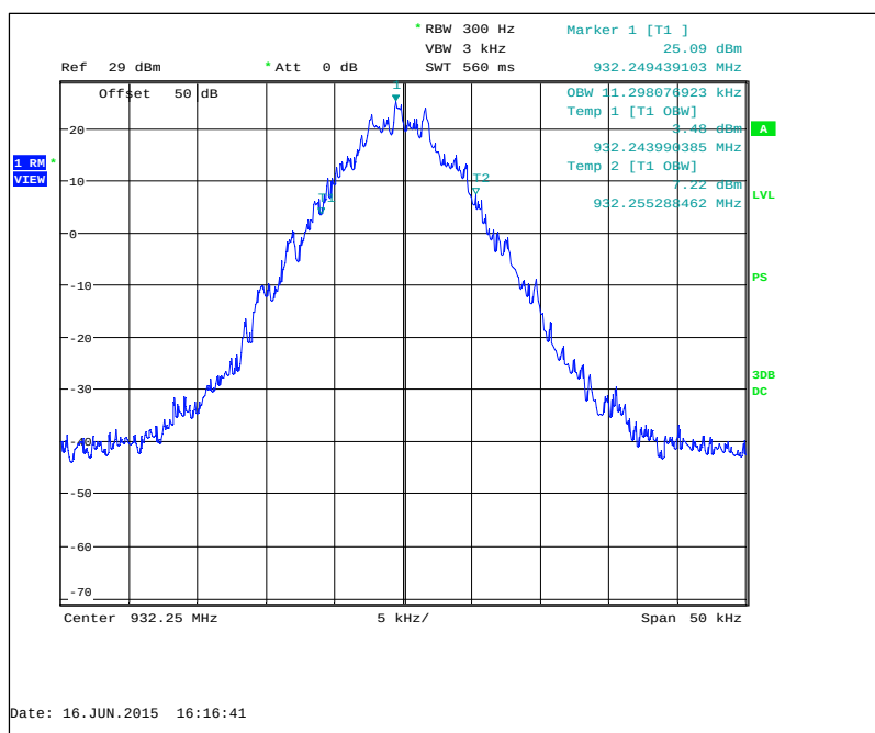
Figure 7.2.3-21: 932.25 MHz – Normal Mode
