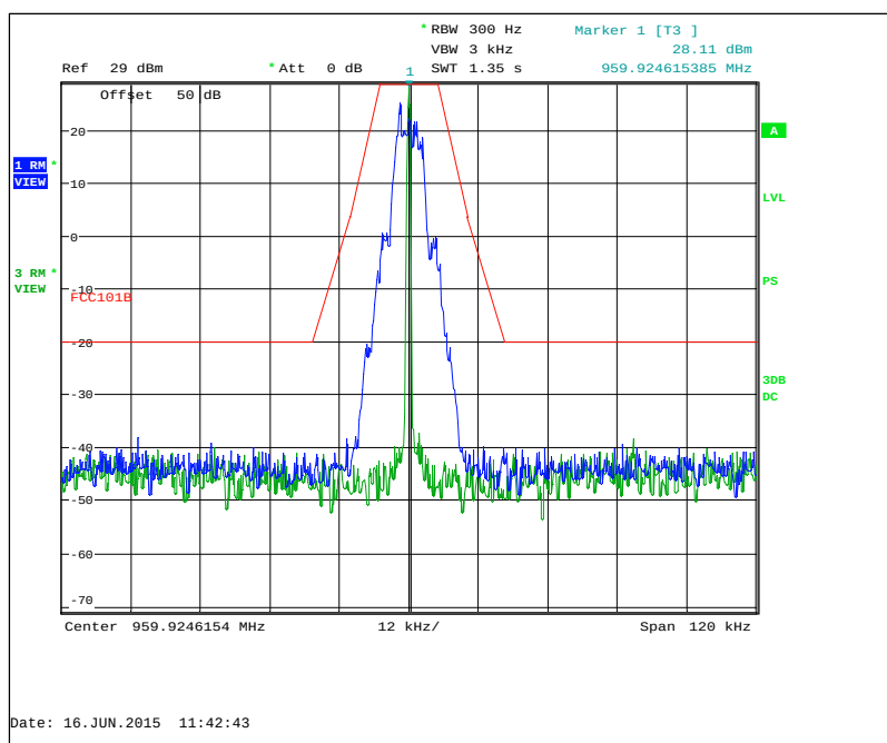
Figure 7.2.2-32: 959.925 MHz – mPass 5k Mode
