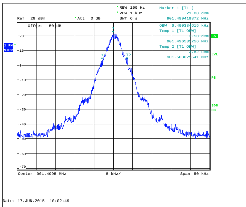
Figure 7.2.3-6: 901.5 MHz – Priority Mode
