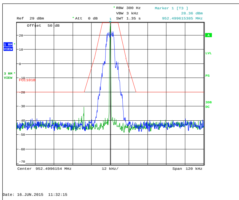
Figure 7.2.2-30: 952.5 MHz – mPass 5k Mode
