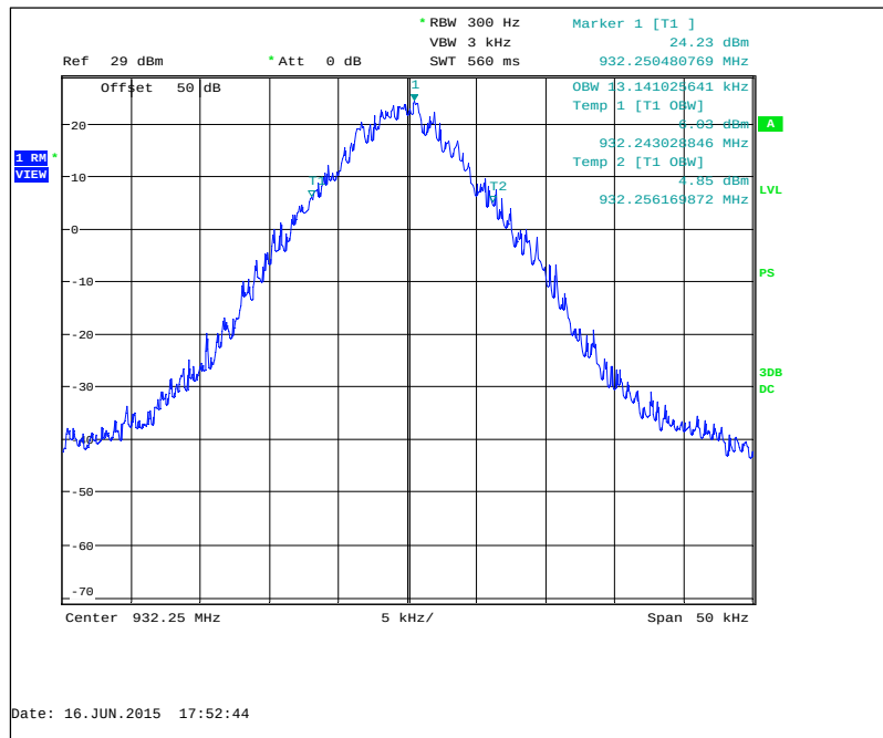
Figure 7.2.3-18: 932.25 MHz – Double Density Mode
