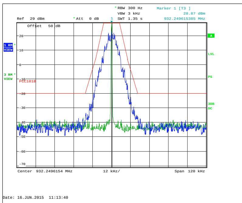
Figure 7.2.2-26: 932.25 MHz – Normal Mode
