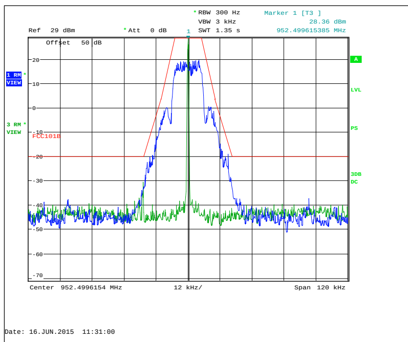
Figure 7.2.2-31: 952.5 MHz – mPass 10k Mode
