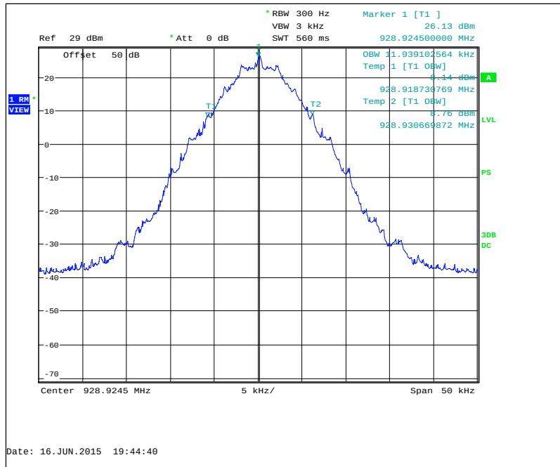
Figure 7.2.3-15: 928.925 MHz – Normal Mode
