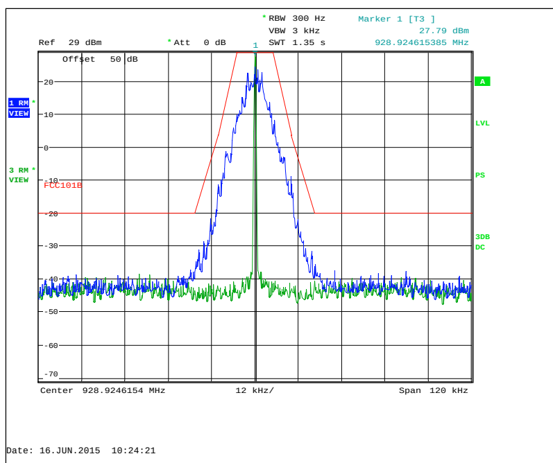
Figure 7.2.2-20: 928.925 MHz – Normal Mode
