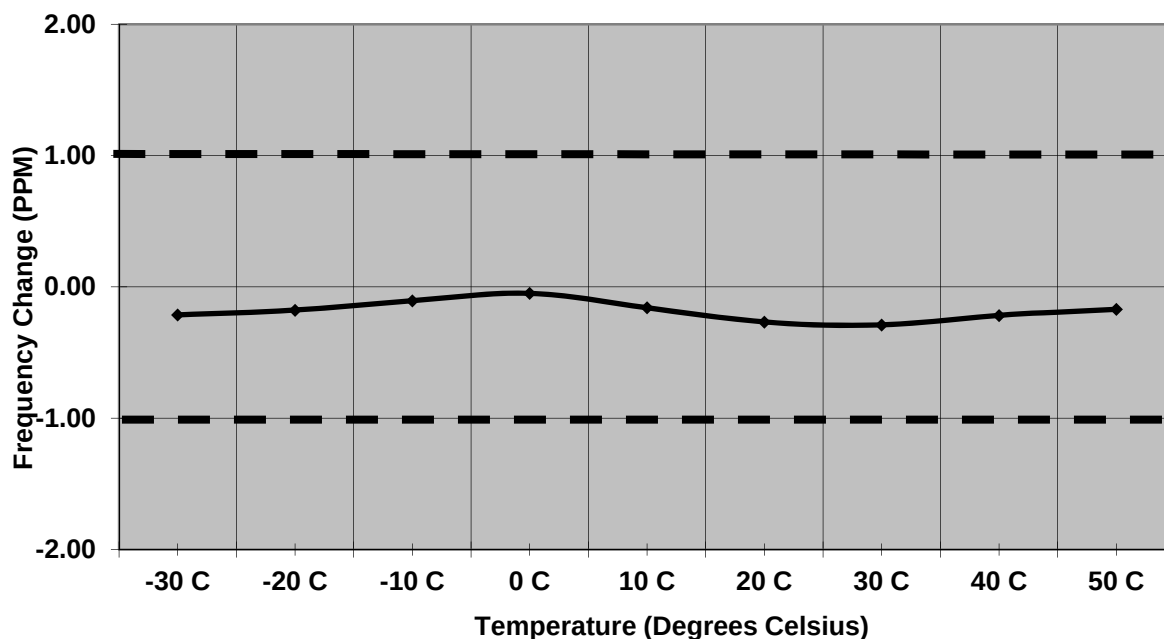
Figure 7.5.2-1: Frequency Stability – 901.5 MHz - KDS
