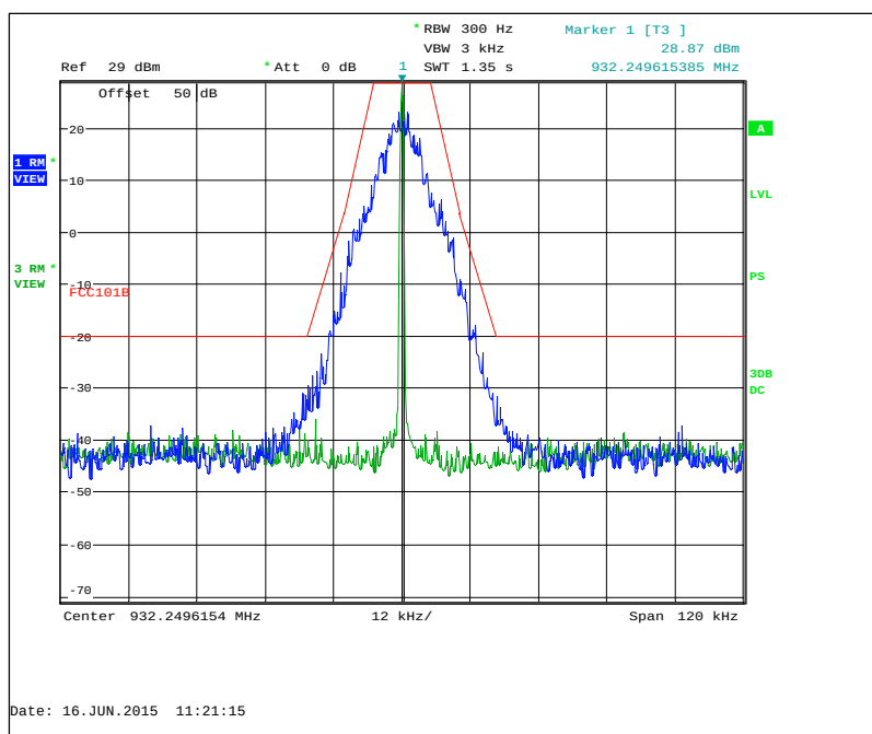
Figure 7.2.2-23: 932.25 MHz – Double Density Mode
