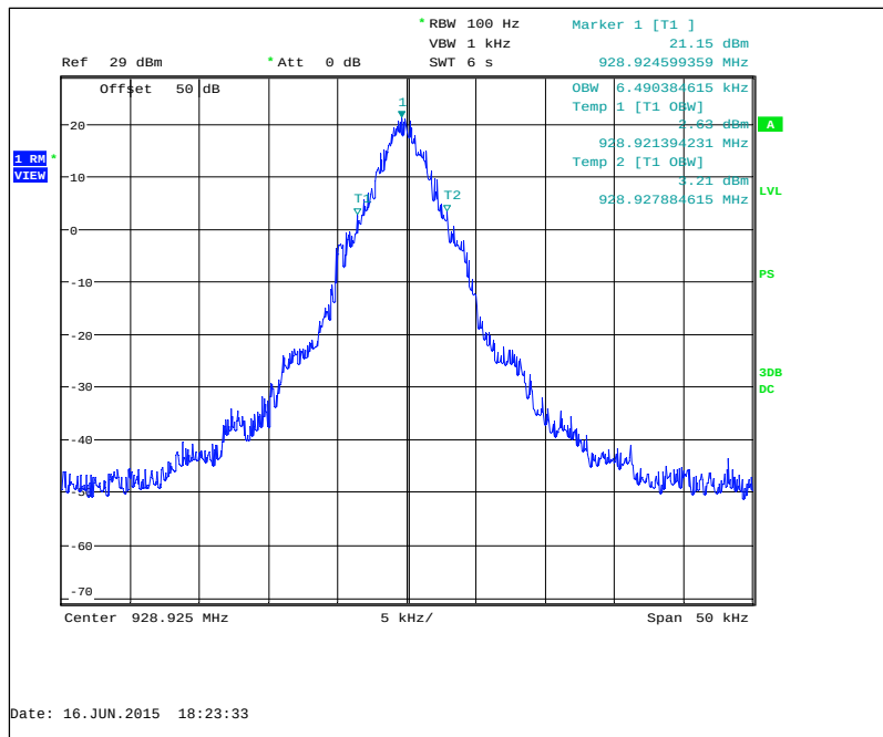
Figure 7.2.3-16: 928.925 MHz -- Priority Mode
