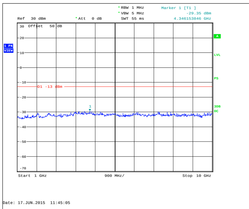
Figure 7.3.2-12: 941.4875 MHz – 1GHz to 10GHz
