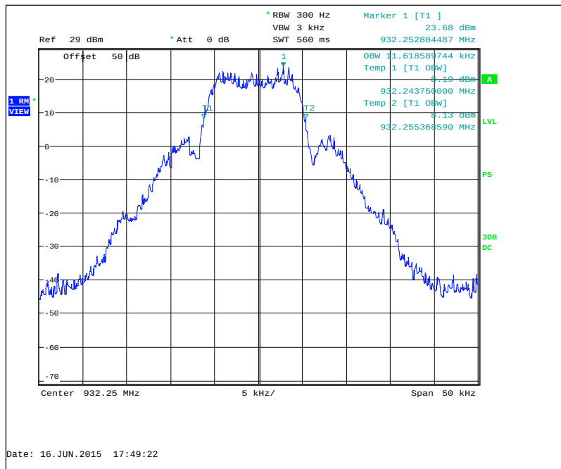
Figure 7.2.3-20: 932.25 MHz – mPass 10k Mode
