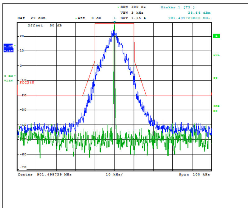
Figure 7.2.2-3: 901.5 MHz – 25 kHz Channel Spacing – Double Density Mode
