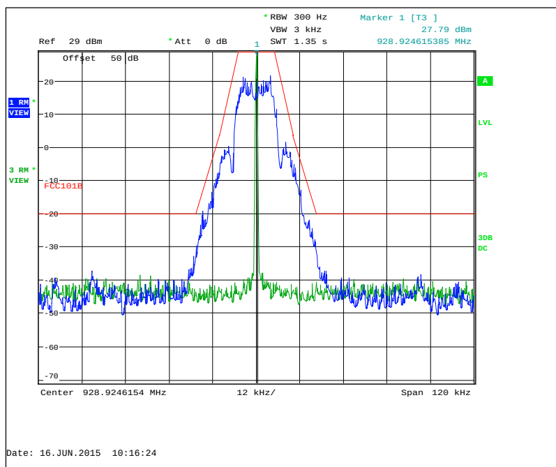
Figure 7.2.2-19: 928.925 MHz – mPass 10k Mode
