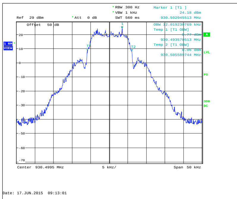
Figure 7.2.3-8: 930.5 MHz – mPass 10k Mode
