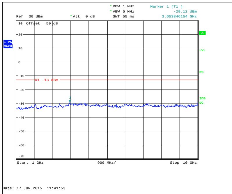
Figure 7.3.2-10: 932.25 MHz – 1GHz to 10GHz
