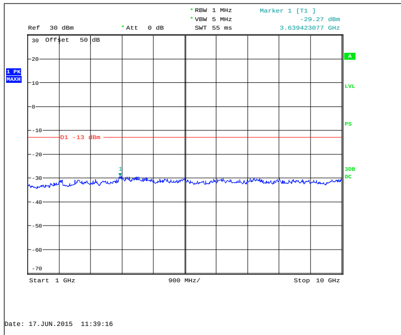
Figure 7.3.2-14: 952.5 MHz – 1GHz to 10GHz
