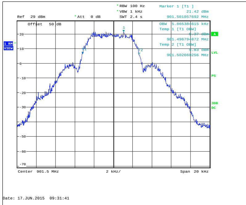
Figure 7.2.3-3: 901.5MHz – mPass 5k Mode
