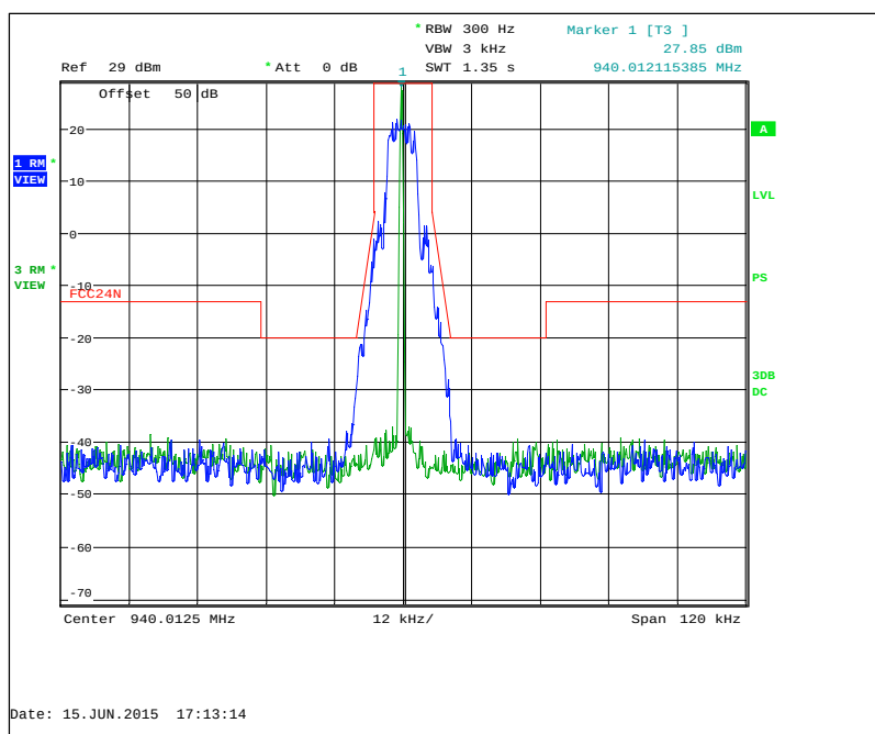
Figure 7.2.2-13: 940.0125 MHz – 12.5 kHz Channel Spacing – mPass 5k Mode
