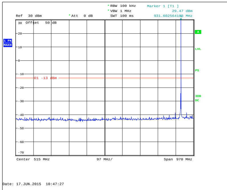
Figure 7.3.2-3: 930.5 MHz – 30MHz to 1GHz
