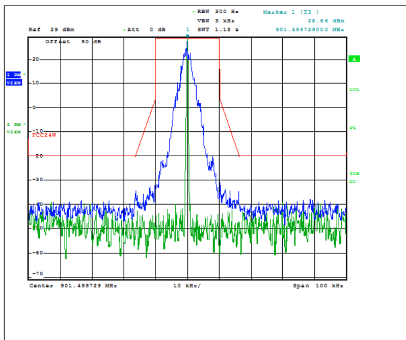
Figure 7.2.2-2: 901.5 MHz – 25 kHz Channel Spacing – C&amp;I Mode
