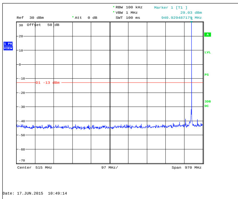
Figure 7.3.2-5: 940.0125 MHz – 30MHz to 1GHz
