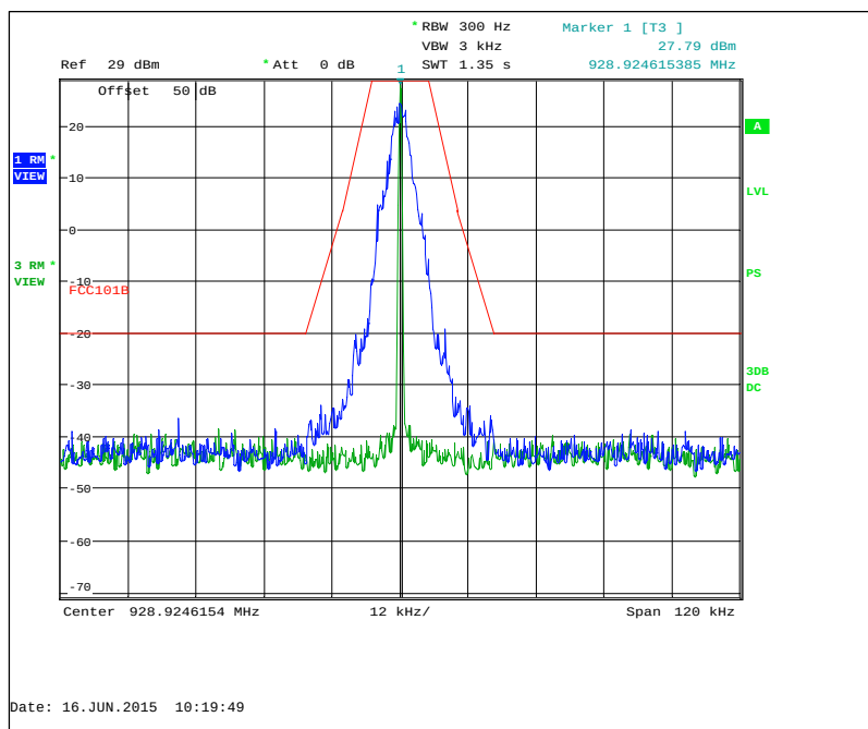
Figure 7.2.2-16: 928.925 MHz – C&I Mode
