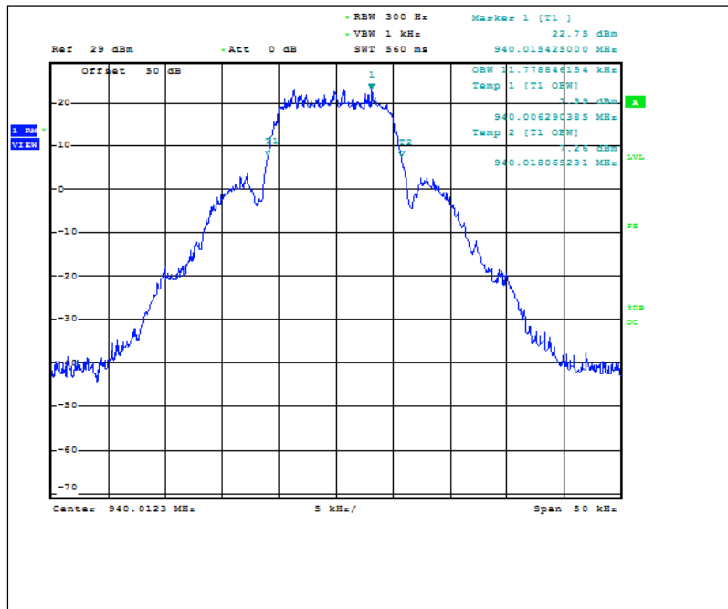
Figure 7.2.3-10: 940.0125 MHz – mPass 10k Mode
