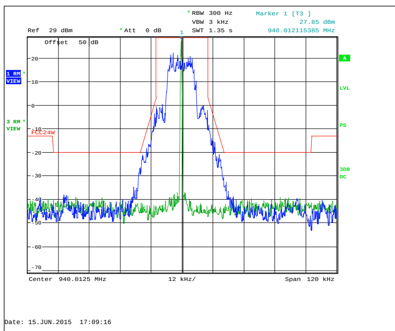
Figure 7.2.2-15: 940.0125 MHz – 25 kHz Channel Spacing – mPass 10k Mode
