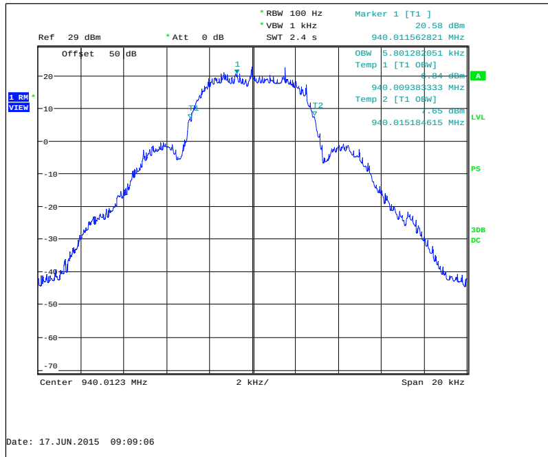
Figure 7.2.3-9: 940.0125 MHz – mPass 5k Mode
