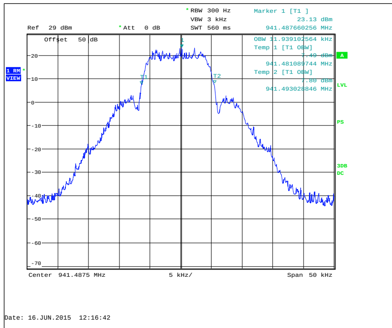
Figure 7.2.3-24: 941.4875 MHz – mPass 10k Mode
