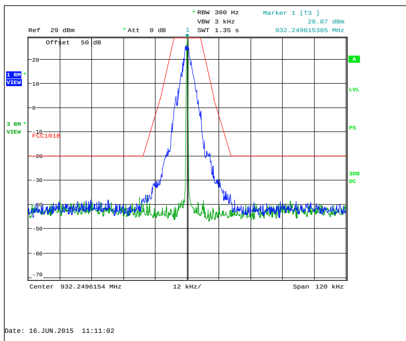
Figure 7.2.2-27: 932.25 MHz -- Priority Mode
