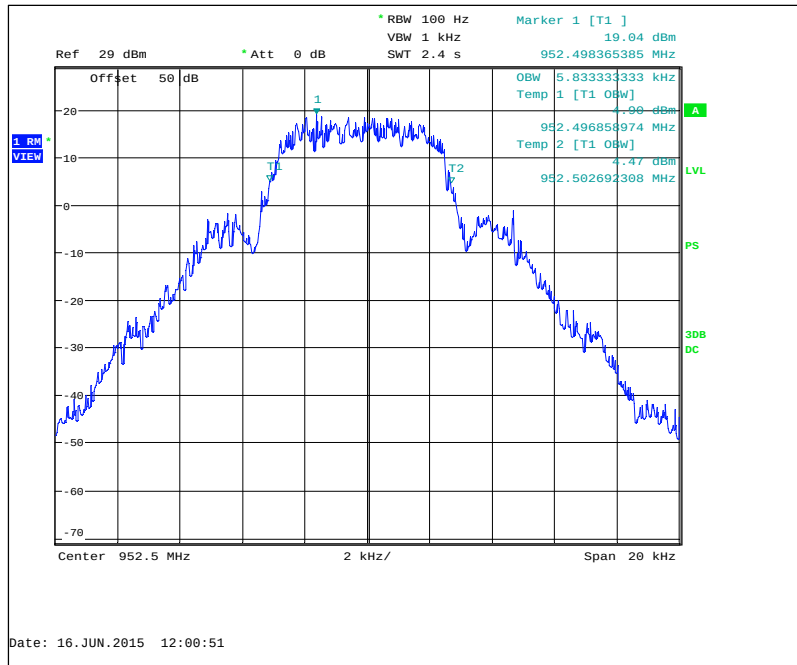
Figure 7.2.3-25: 952.5 MHz – mPass 5k Mode
