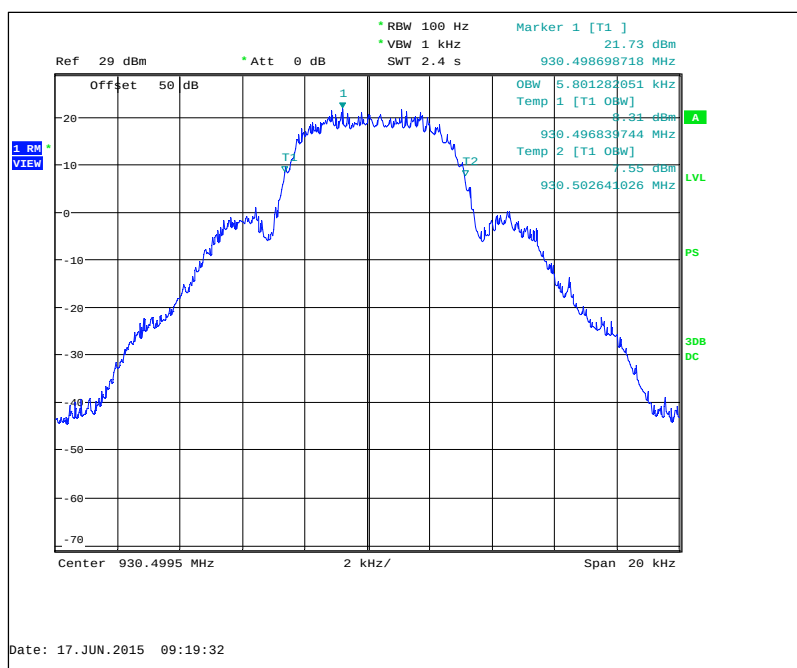
Figure 7.2.3-7: 930.5 MHz – mPass 5k Mode
