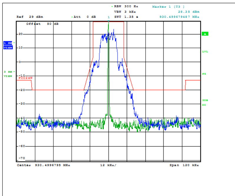
Figure 7.2.2-12: 930.5 MHz – 25 kHz Channel Spacing – mPass 10k Mode
