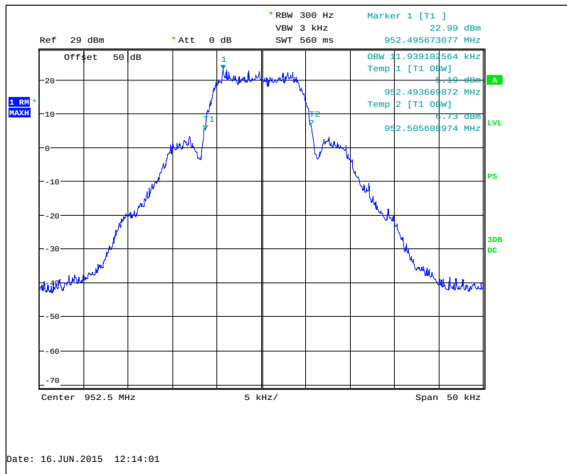
Figure 7.2.3-26: 952.5 MHz – mPass 10k Mode
