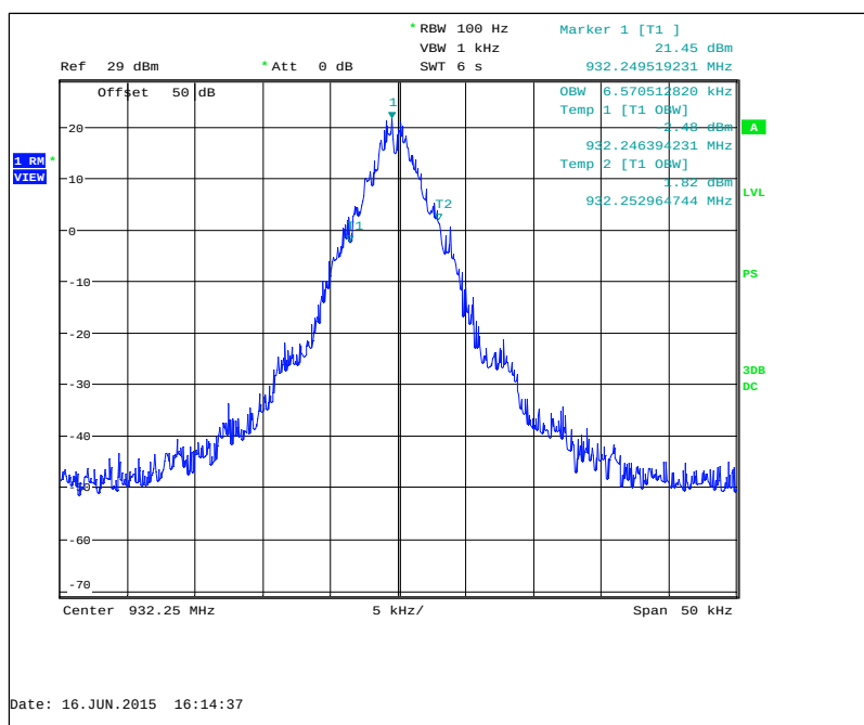
Figure 7.2.3-22: 932.25 MHz — Priority Mode
