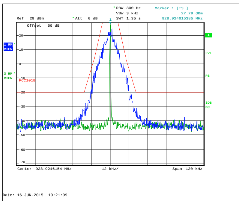
Figure 7.2.2-17: 928.925 MHz – Double Density Mode
