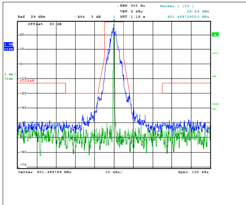
Figure 7.2.2-1: 901.5 MHz – 12.5 kHz Channel Spacing – C&I Mode
