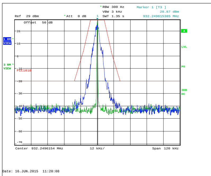
Figure 7.2.2-22: 932.25 MHz – C&amp;I Mode
