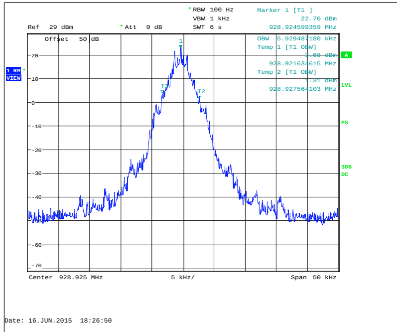
Figure 7.2.3-11: 928.925 MHz – C&I Mode
