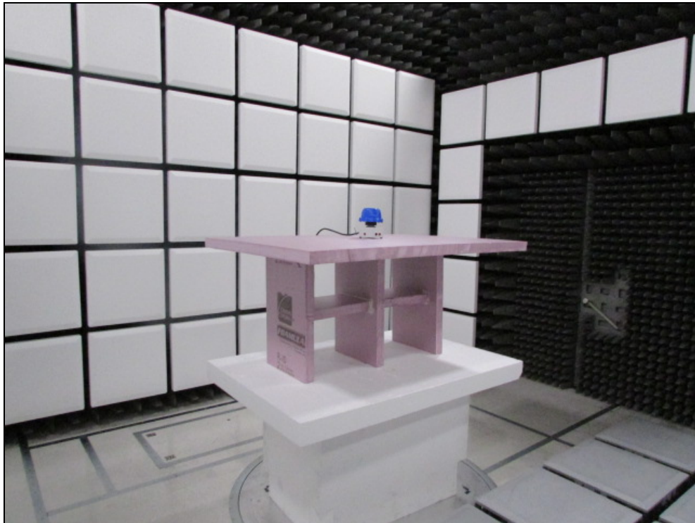
Figure 3: Radiated Emissions – Front View – Above 1GHz
