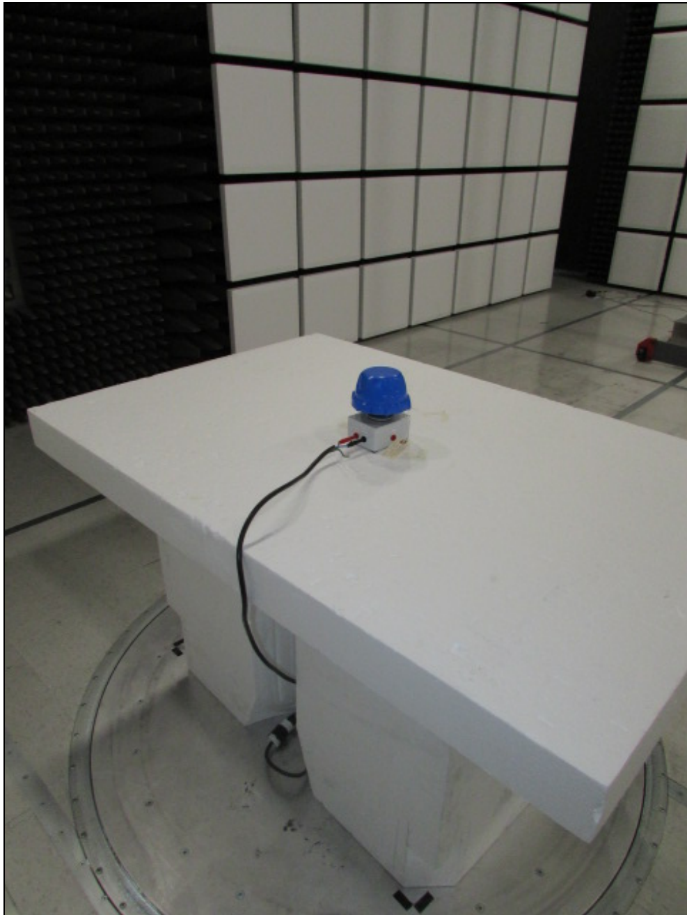
Figure 2: Radiated Emissions – Side View – Below 1GHz
