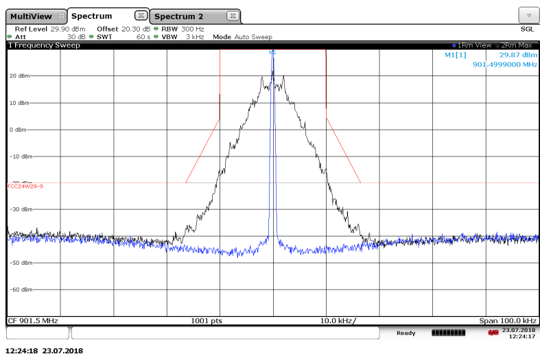
Figure 7.2.2-4: 901.5 MHz – 25 kHz Channel Spacing – Normal Mode
