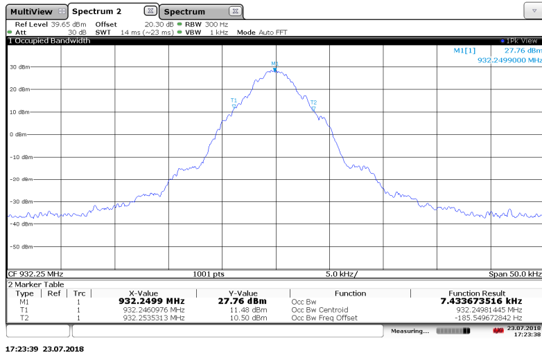
Figure 7.3.2-18: 932.25 MHz — Priority Mode
