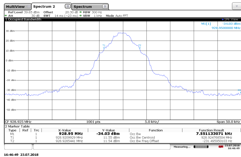
Figure 7.3.2-13: 928.925 MHz – Priority Mode
