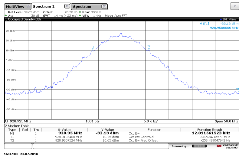
Figure 7.3.2-12: 928.925 MHz – Normal Mode
