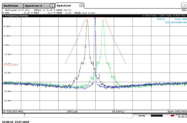
Figure 7.2.2-14: 928.925 MHz — 25 kHz Channel Spacing - Boost Mode
