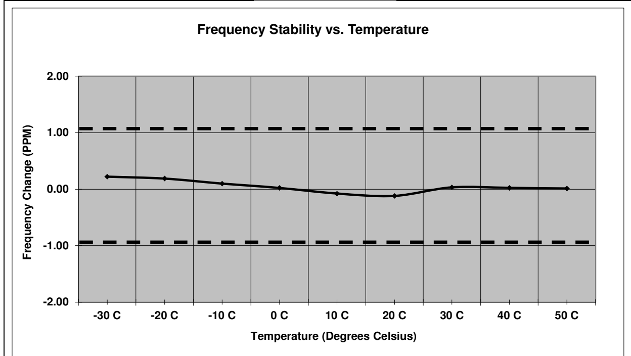
Figure 7.6.2-2: Frequency Stability – 901.5 MHz – TXC
