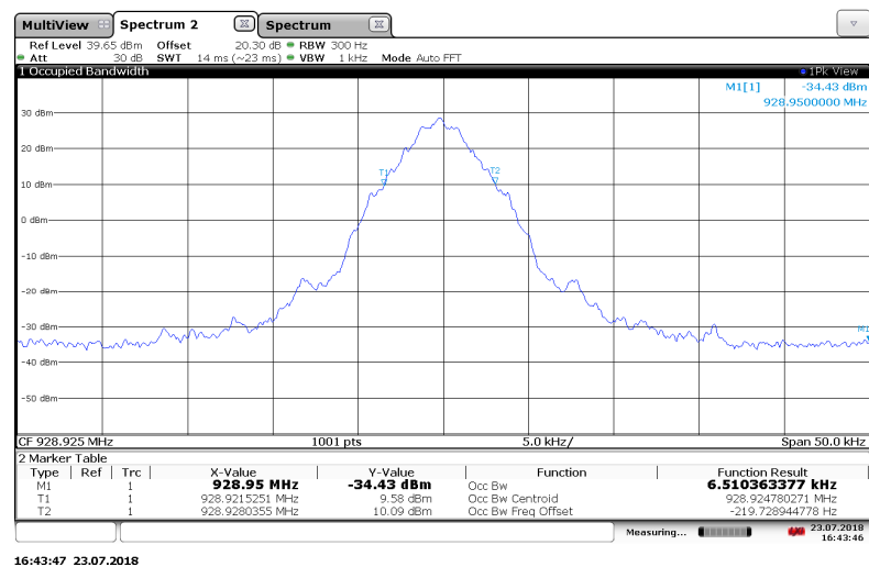
Figure 7.3.2-10: 928.925 MHz – C&I (Half Baud) Mode
