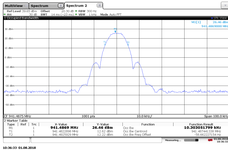
Figure 7.3.2-21: 941.4875 MHz – MPass 10k Mode
