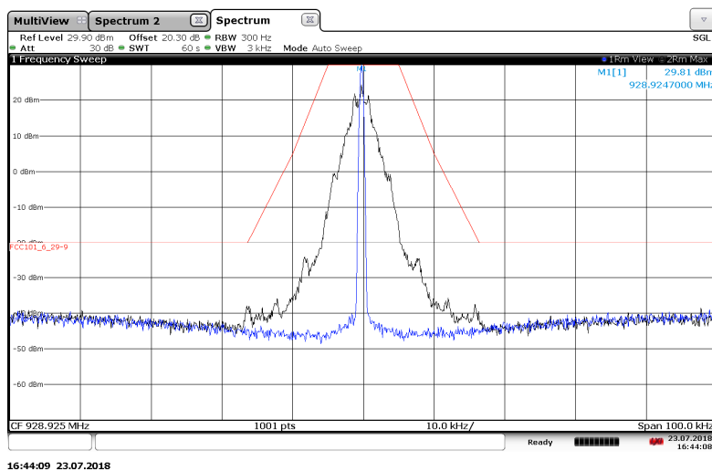
Figure 7.2.2-10: 928.925 MHz – 25 kHz Channel Spacing – C&I Mode
