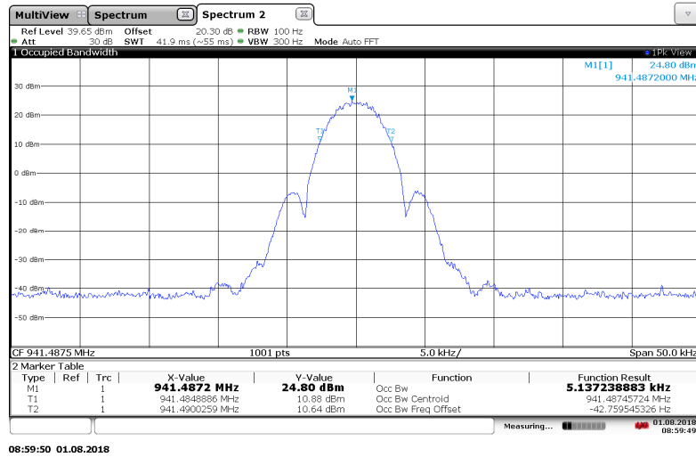
Figure 7.3.2-20: 941.4875 MHz – MPass 5k Mode
