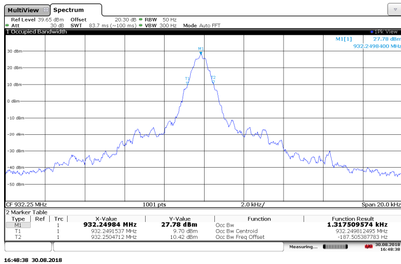
Figure 7.3.2-19: 932.25 MHz — Boost Mode
