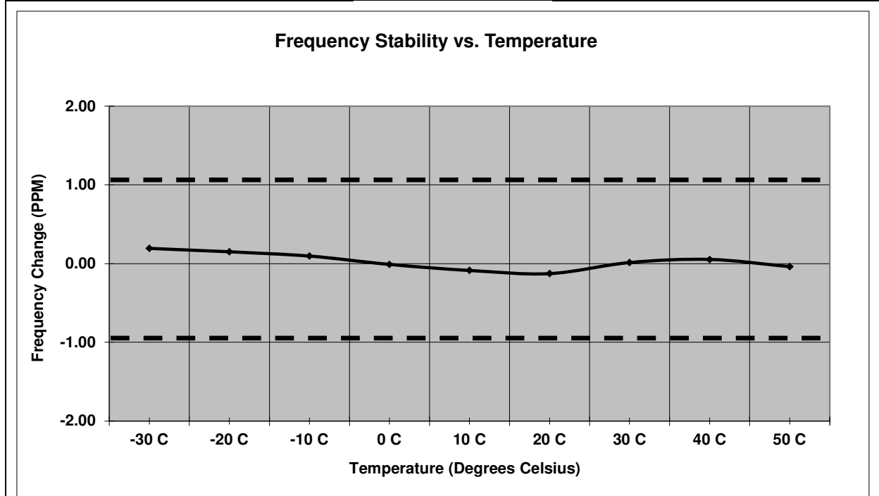
Figure 7.6.2-4: Frequency Stability – 930.5 MHz – TXC
