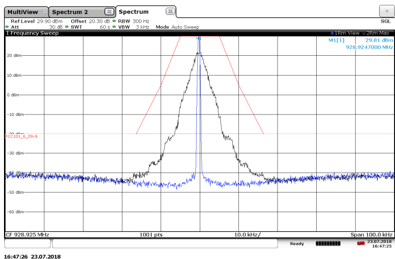
Figure 7.2.2-13: 928.925 MHz — 25 kHz Channel Spacing - Priority Mode
