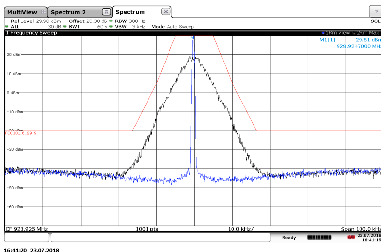
Figure 7.2.2-11: 928.925 MHz – 25 kHz Channel Spacing - Double Density Mode
