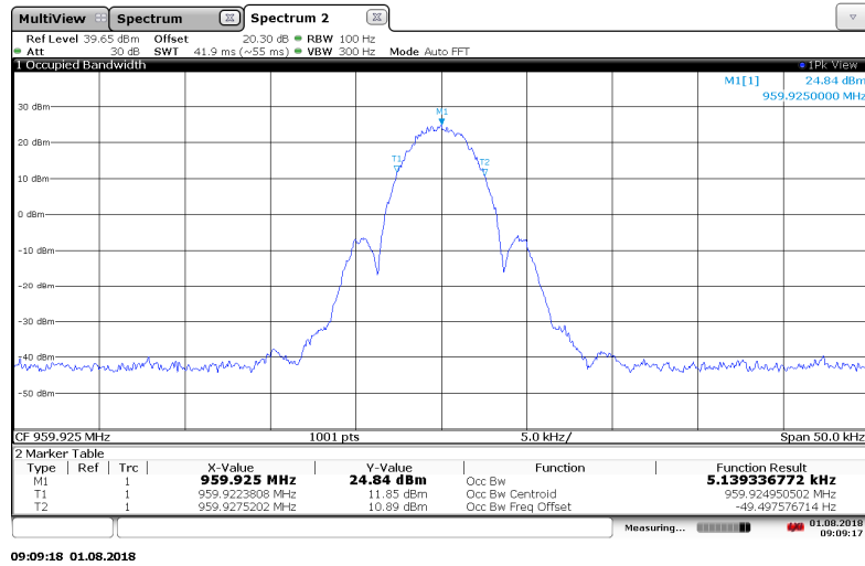
Figure 7.3.2-24: 959.925 MHz– mPass 5k Mode
