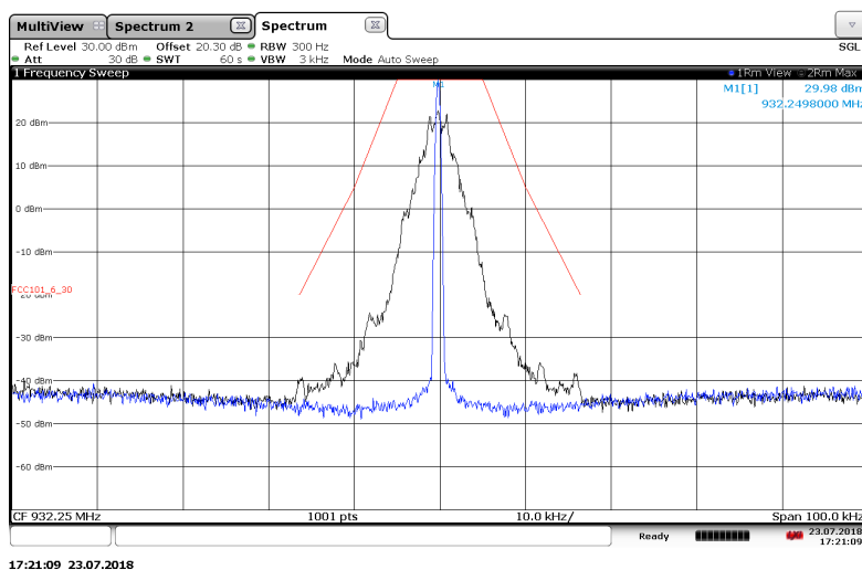
Figure 7.2.2-15: 932.25 MHz – 25 kHz Channel Spacing - C&amp;I Mode
