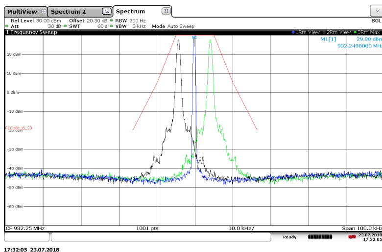
Figure 7.2.2-19: 932.25 MHz — 25 kHz Channel Spacing - Boost Mode
