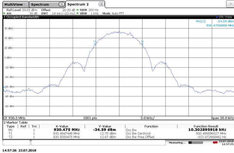
Figure 7.3.2-7: 930.5 MHz – MPass 10k Mode
