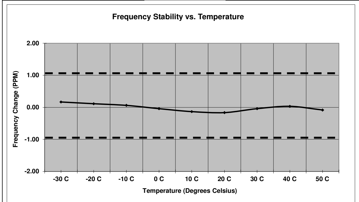
Figure 7.6.2-6: Frequency Stability – 959.925 MHz – TXC
