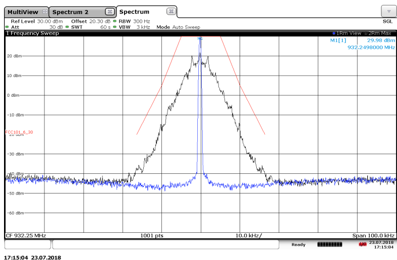
Figure 7.2.2-17: 932.25 MHz – 25 kHz Channel Spacing - Normal Mode
