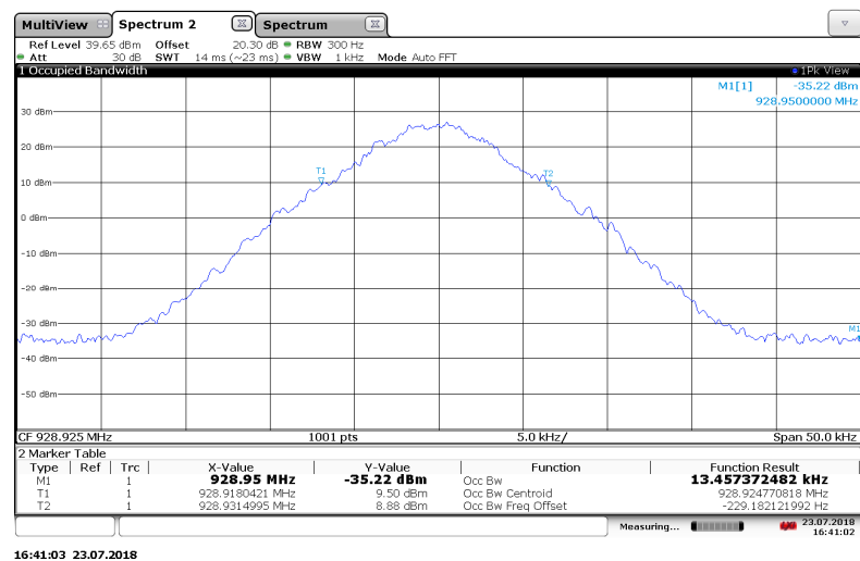
Figure 7.3.2-11: 928.925 MHz – Double Density Mode
