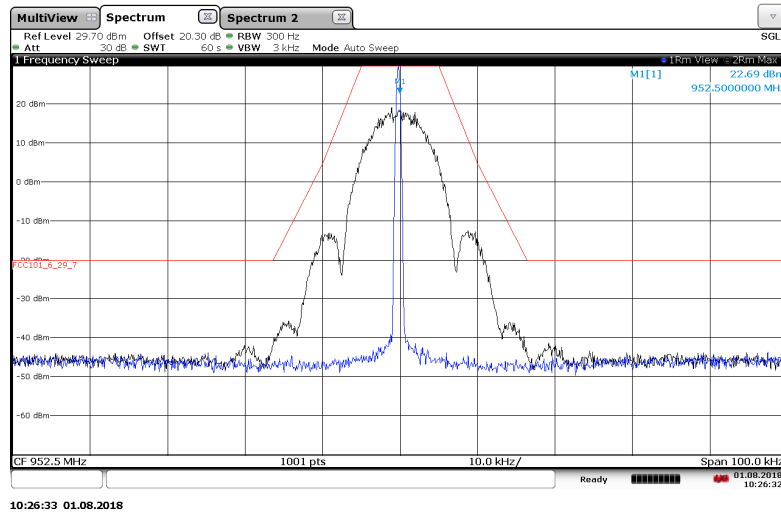
Figure 7.2.2-23: 952.5 MHz – 25 kHz Channel Spacing – mPass 10k Mode
