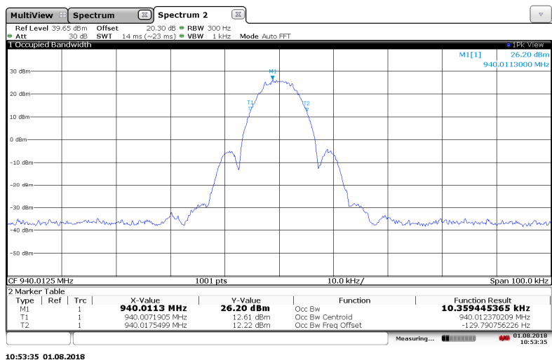
Figure 7.3.2-9: 940.0125 MHz – MPass 10k Mode
