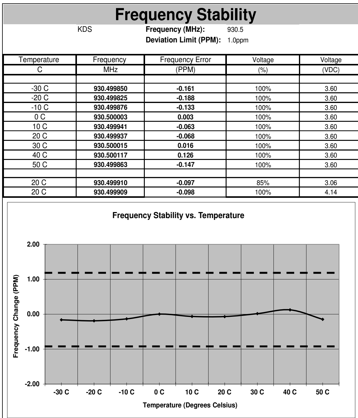
Figure 7.6.2-3: Frequency Stability – 930.5 MHz – KDS
