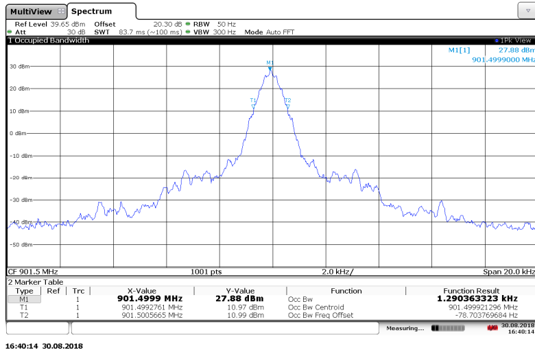
Figure 7.3.2-5: 901.5 MHz – Boost Mode
