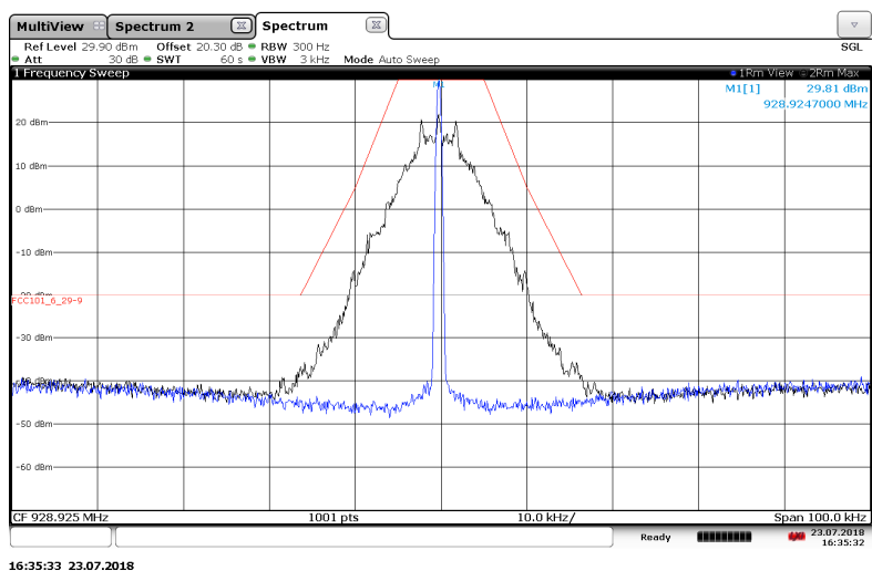
Figure 7.2.2-12: 928.925 MHz – 25 kHz Channel Spacing - Normal Mode
