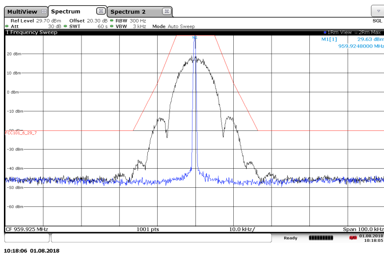
Figure 7.2.2-25: 959.925 MHz – 25 kHz Channel Spacing – mPass 10k Mode
