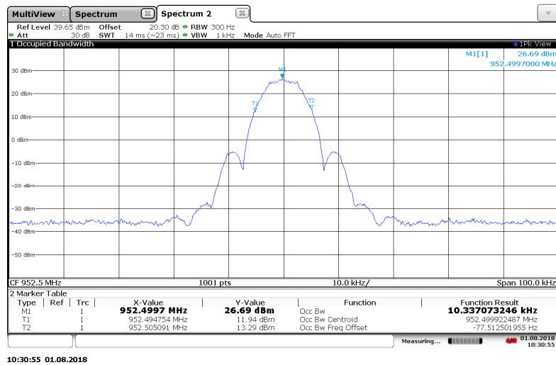
Figure 7.3.2-23: 952.5 MHz – MPass 10k Mode
