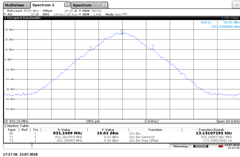
Figure 7.3.2-16: 932.25 MHz – Double Density Mode
