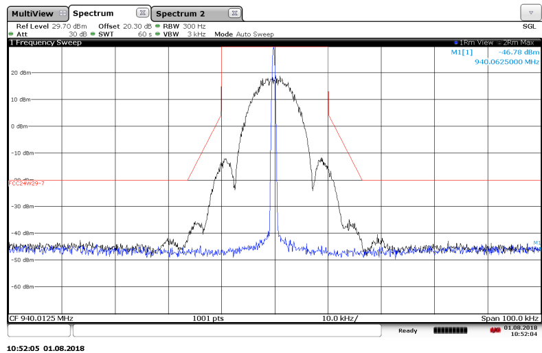
Figure 7.2.2-9: 940.0125 MHz – 25 kHz Channel Spacing – mPass 10k Mode
