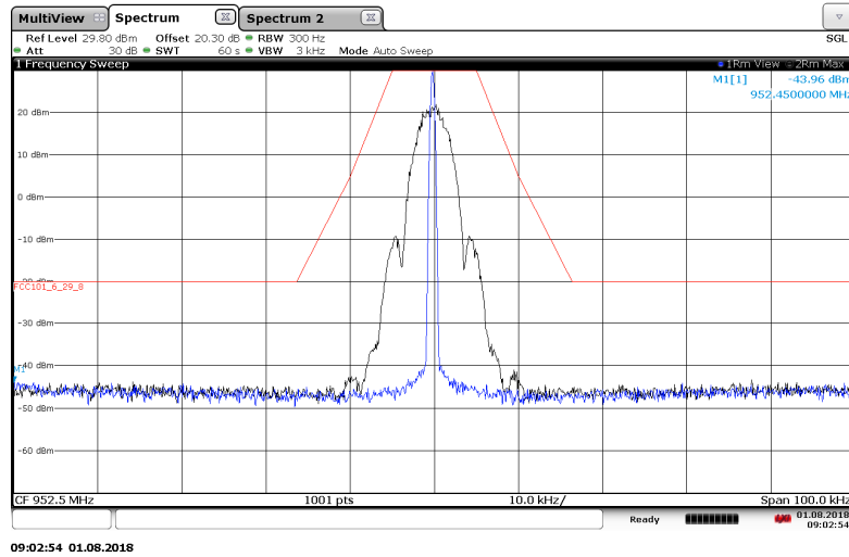
Figure 7.2.2-22: 952.5 MHz - 25 kHz Channel Spacing – mPass 5k Mode
