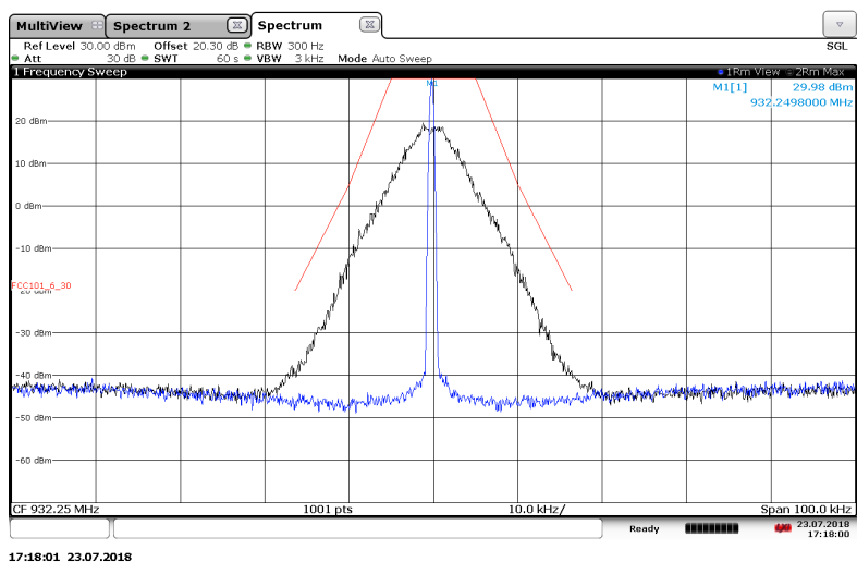
Figure 7.2.2-16: 932.25 MHz – 25 kHz Channel Spacing - Double Density Mode
