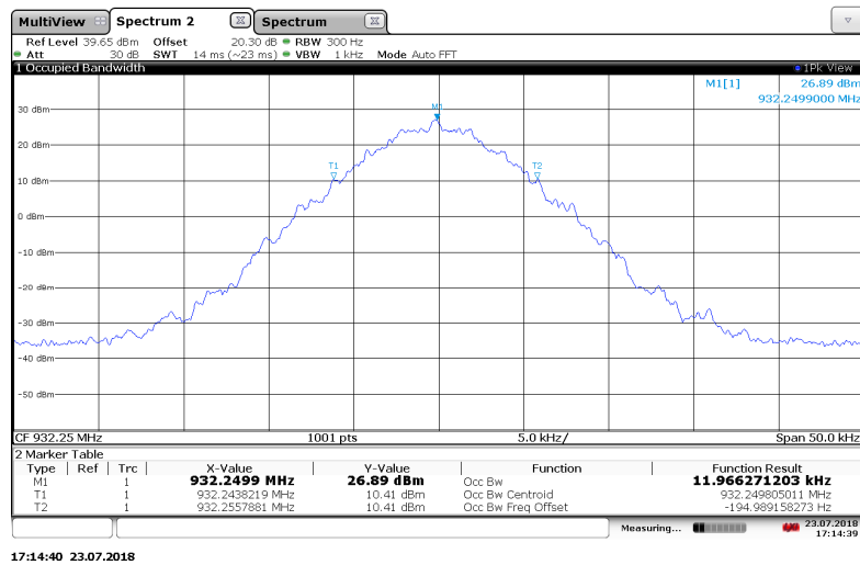
Figure 7.3.2-17: 932.25 MHz – Normal Mode
