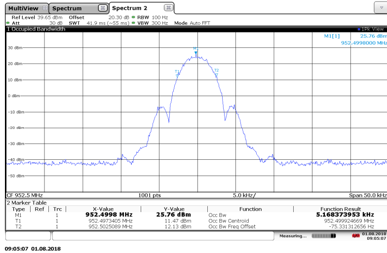
Figure 7.3.2-22: 952.5 MHz – MPass 5k Mode
