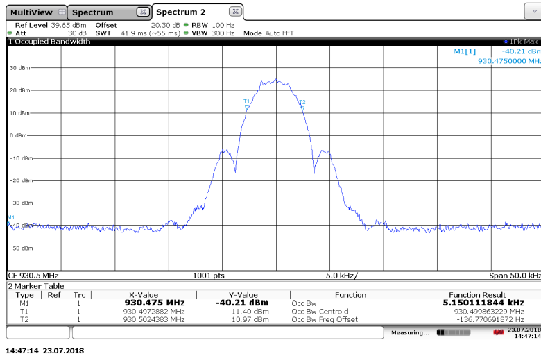
Figure 7.3.2-6: 930.5 MHz – MPass 5k Mode
