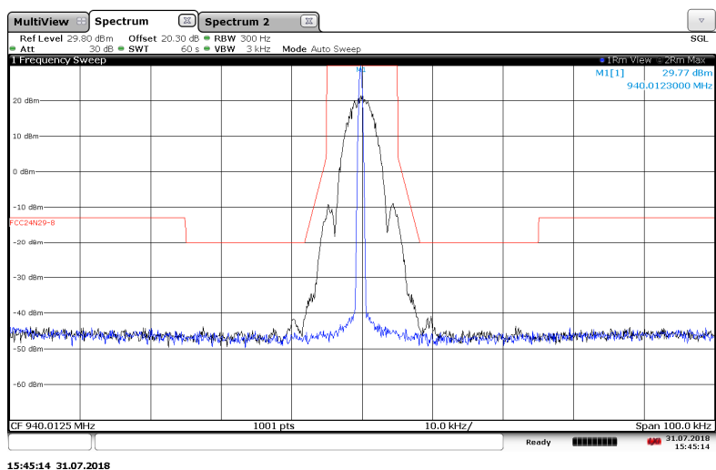
Figure 7.2.2-8: 940.0125 MHz – 12.5 kHz Channel Spacing – mPass 5k Mode
