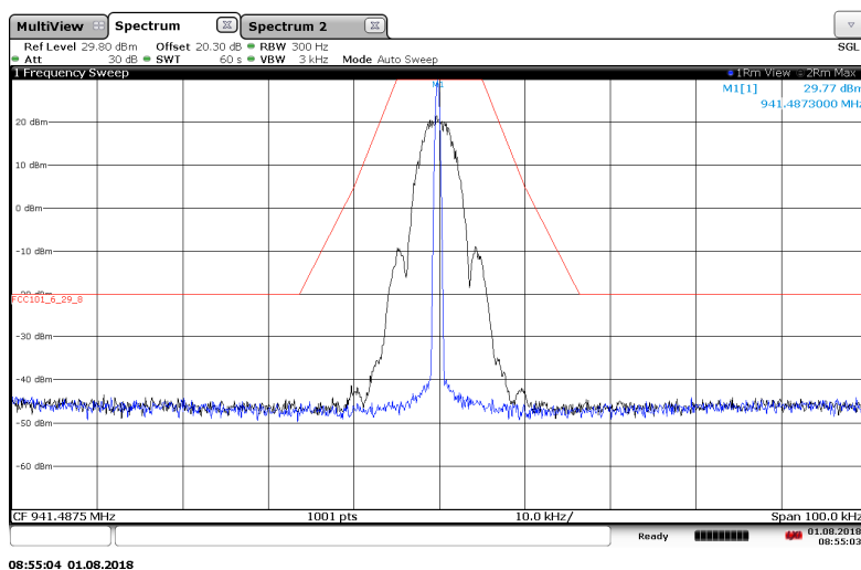
Figure 7.2.2-20: 941.4875 MHz - 25 kHz Channel Spacing – mPass 5k Mode
