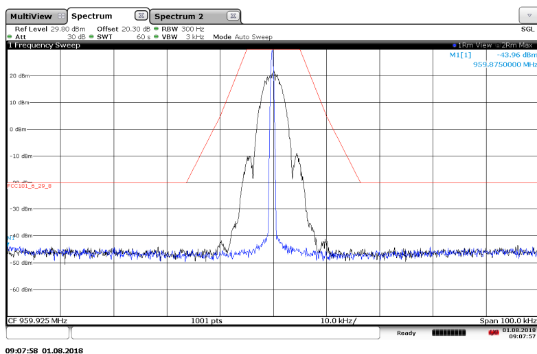
Figure 7.2.2-24: 959.925 MHz - 12.5 kHz Channel Spacing – mPass 5k Mode
