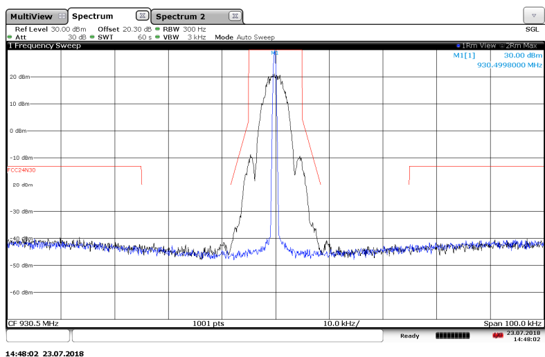
Figure 7.2.2-7: 930.5 MHz –25 kHz Channel Spacing – mPass 5k Mode
