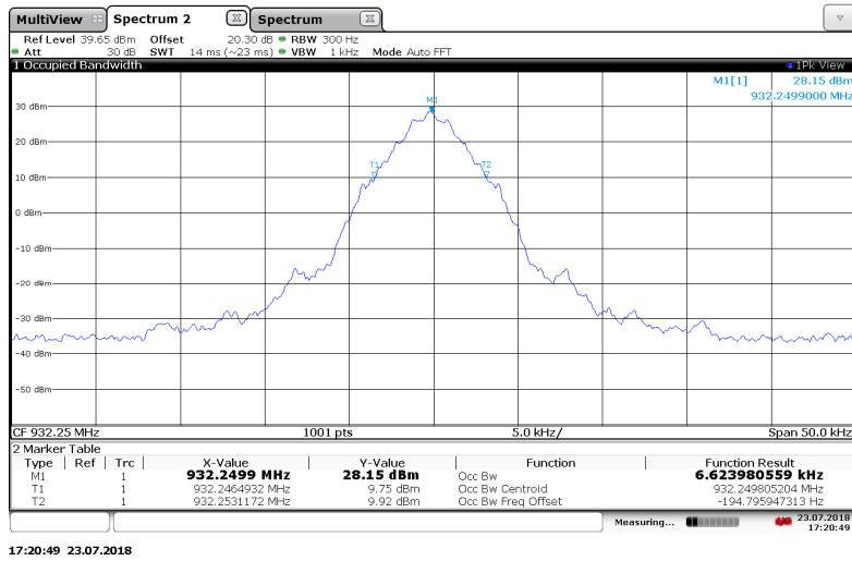
Figure 7.3.2-15: 932.25 MHz – C&amp;I (Half Baud) Mode
