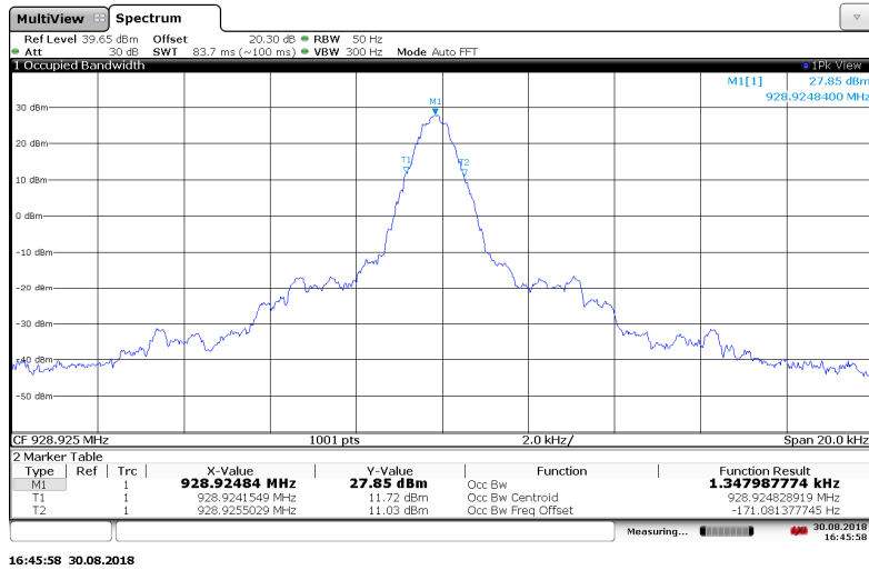
Figure 7.3.2-14: 928.925 MHz – Boost Mode
