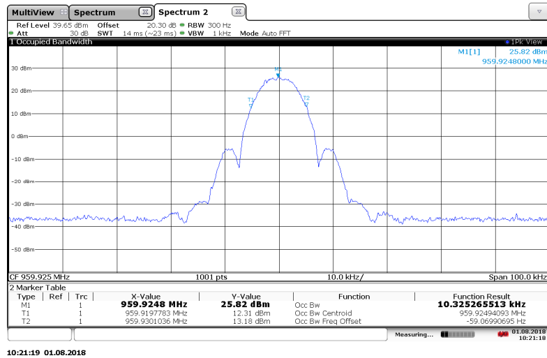
Figure 7.3.2-25: 959.925 MHz– mPass 10k Mode
