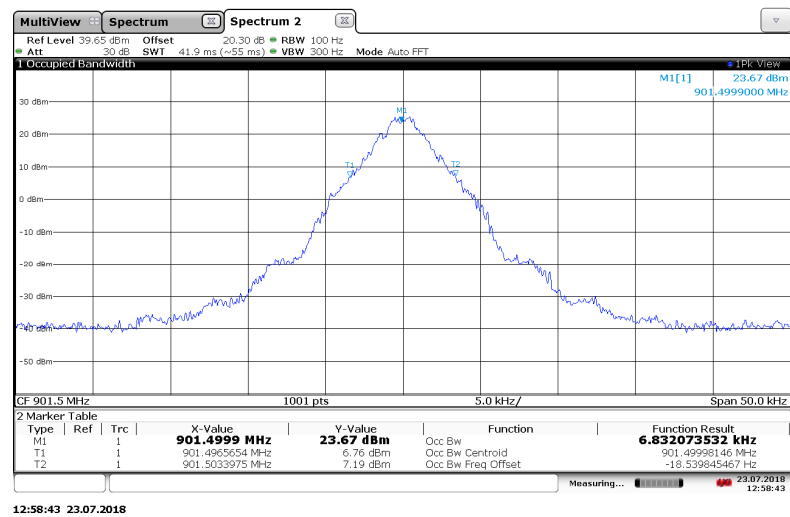
Figure 7.3.2-4: 901.5 MHz – Priority Mode
