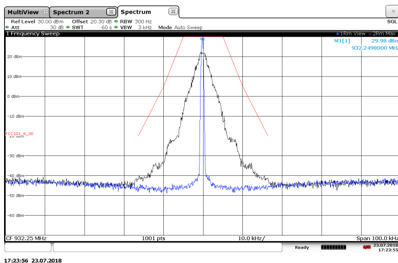
Figure 7.2.2-18: 932.25 MHz — 25 kHz Channel Spacing - Priority Mode
