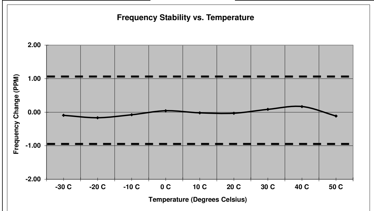
Figure 7.6.2-5: Frequency Stability – 959.925 MHz – KDS
