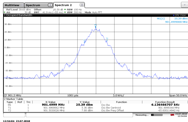
Figure 7.3.2-1: 901.5 MHz – C&I (Half Baud) Mode
