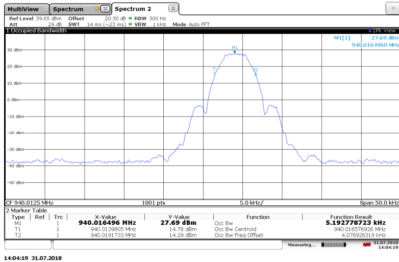
Figure 7.3.2-8: 940.0125 MHz – MPass 5k Mode
