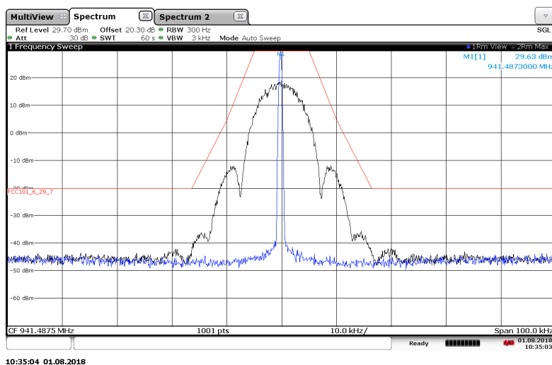
Figure 7.2.2-21: 941.4875 MHz – 25 kHz Channel Spacing – mPass 10k Mode
