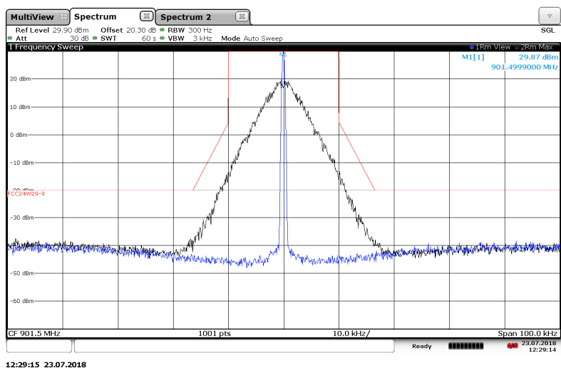
Figure 7.2.2-3: 901.5 MHz – 25 kHz Channel Spacing – Double Density Mode
