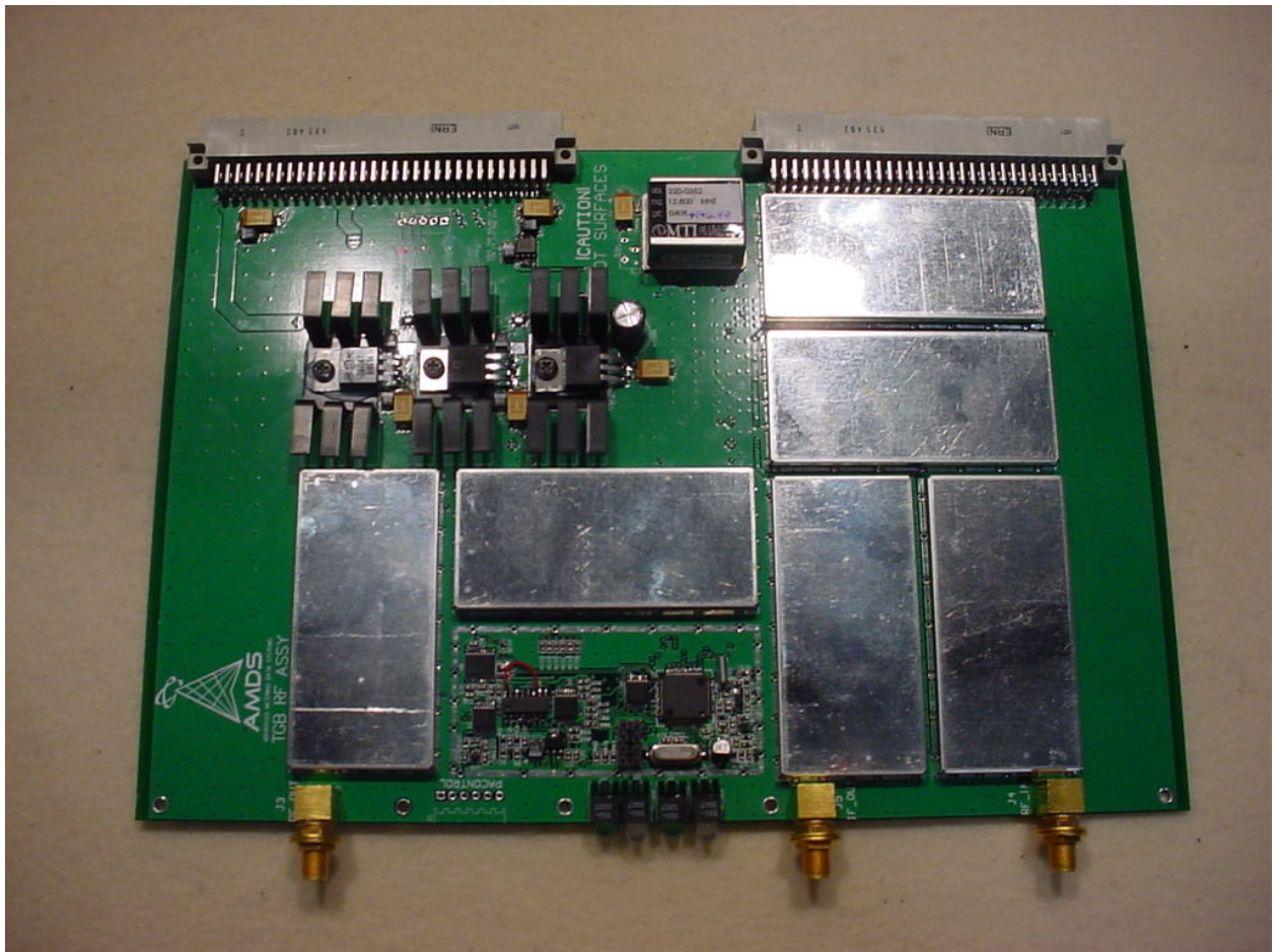
Figure 1. RF Board Front
