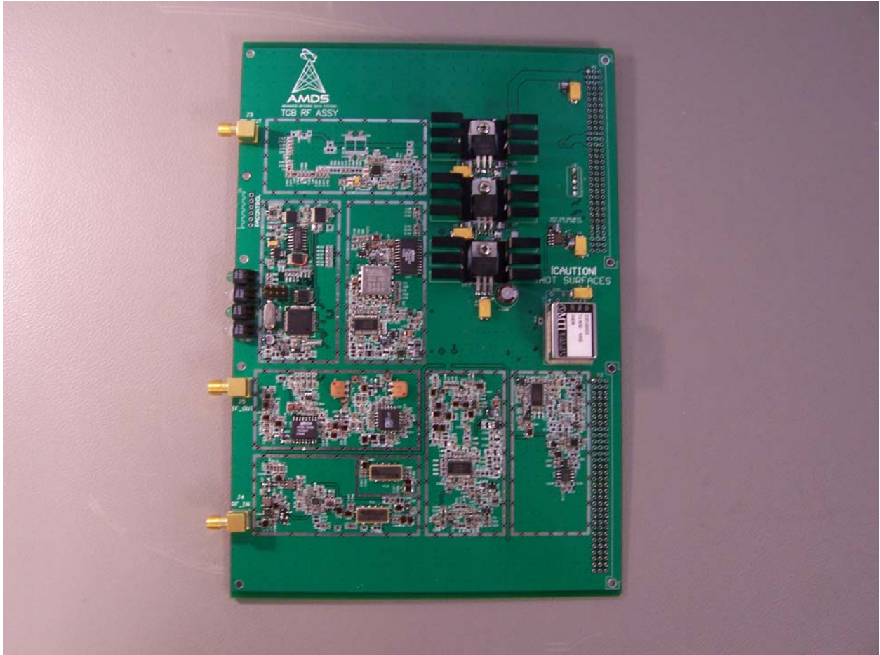
Figure 2. RF Board Front – No Shields
