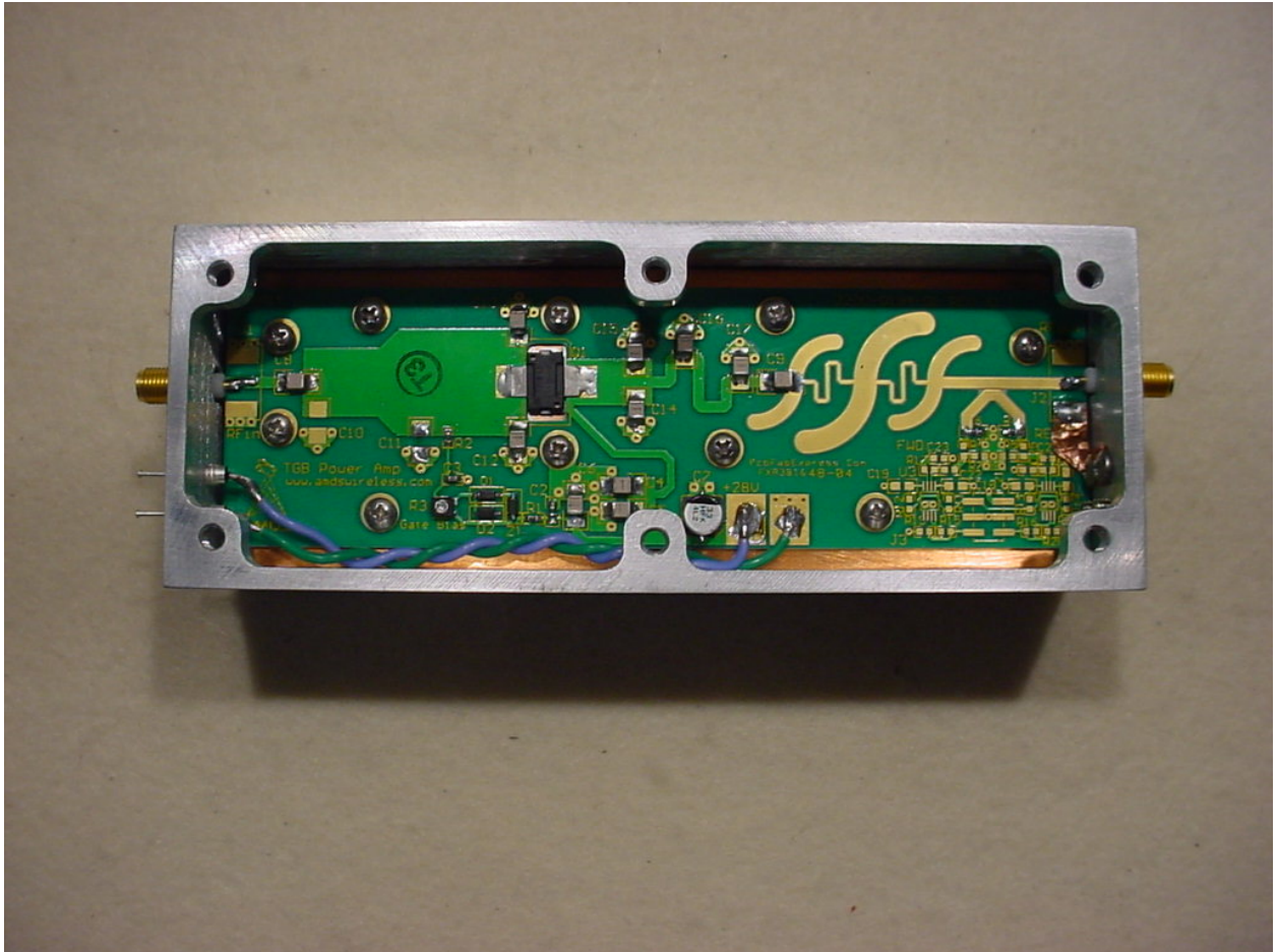
Figure 4. Power Amplifier (Only used in TGB001HP)
