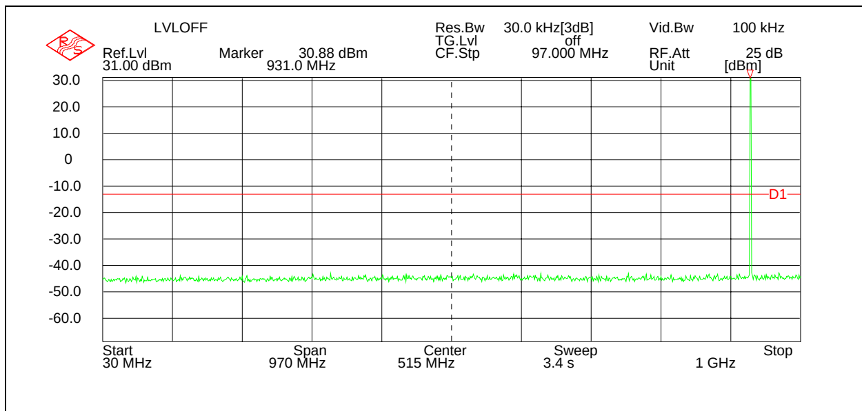
Figure 7.3.2-1: - 930.00625 MHz
