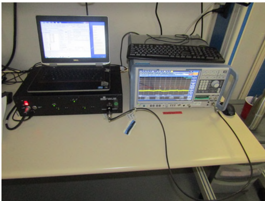
Figure 5: Conducted Emissions
