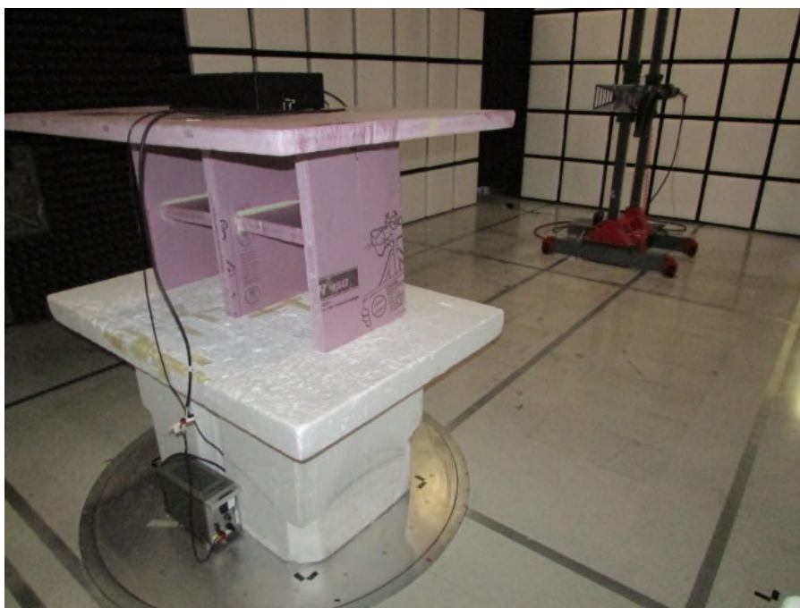
Figure 4: Radiated Emissions – Back – Above 1GHz
