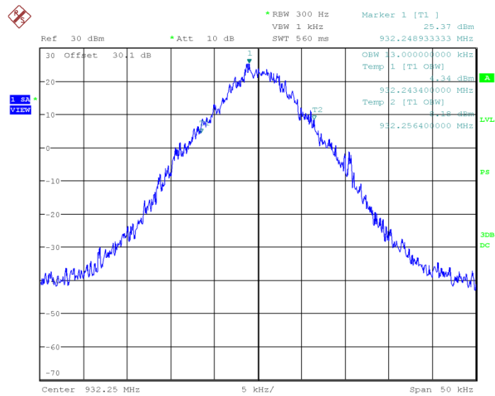
Figure 7.3.2-13: 932.25 MHz – C&amp;I Mode
