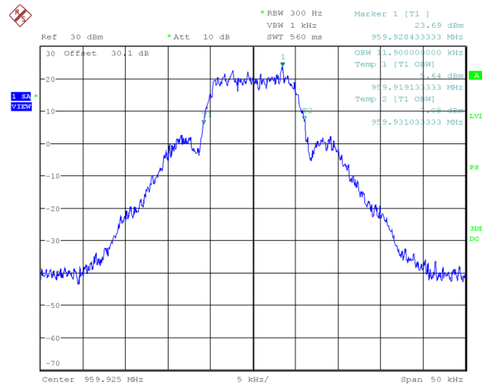
Figure 7.3.2-21: 959.925 MHz – mPass 5k Mode
