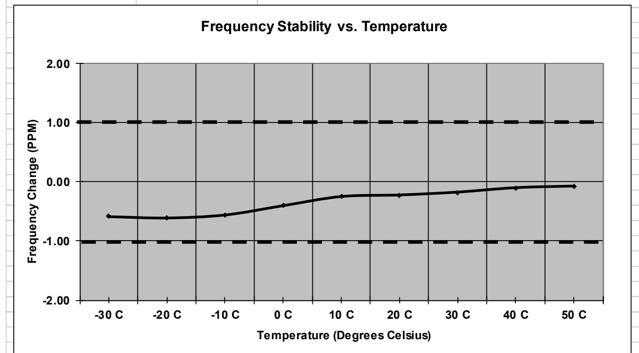
Figure 7.6.2-3: Frequency Stability – 959.925 MHz - KDS
