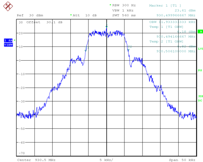
Figure 7.3.2-5: 930.5 MHz – mPass 5k Mode
