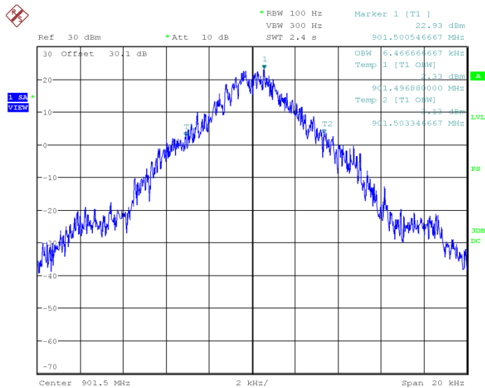
Figure 7.3.2-3: 901.5 MHz – Normal Mode
