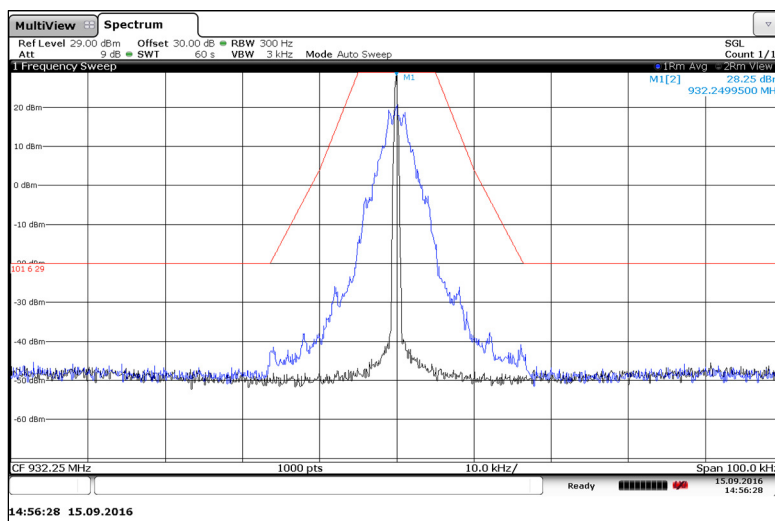
Figure 7.2.2-17: 932.25 MHz – C&amp;I Mode
