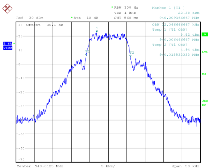
Figure 7.3.2-7: 940.0125 MHz – mPass 5k Mode
