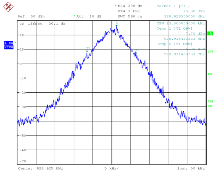
Figure 7.3.2-9: 928.925 MHz – C&I Mode
