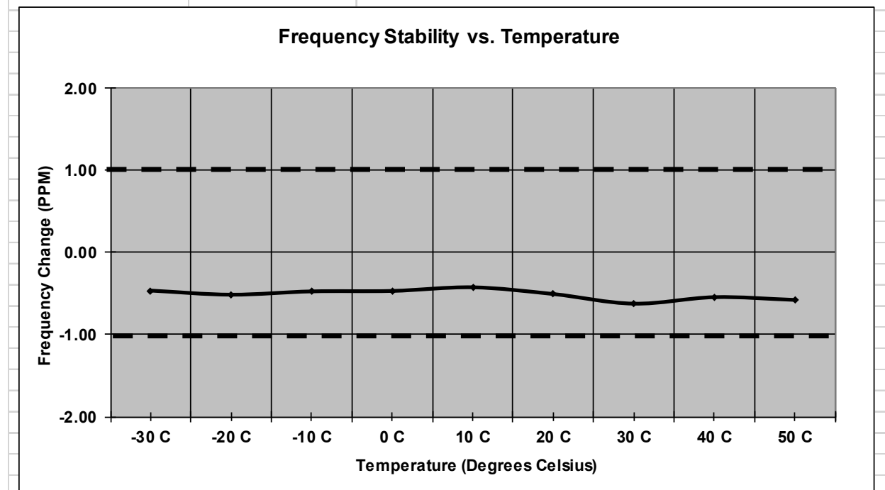
Figure 7.6.2-6: Frequency Stability – 959.925 MHz - ILSI
