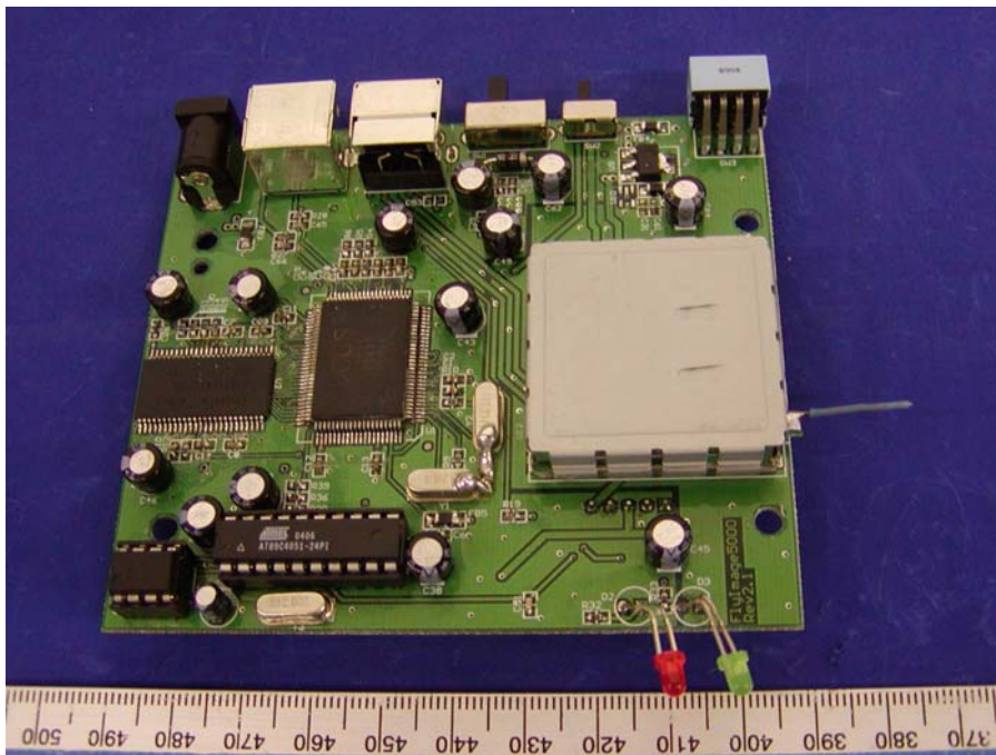
EUT – Component View with Shielding
