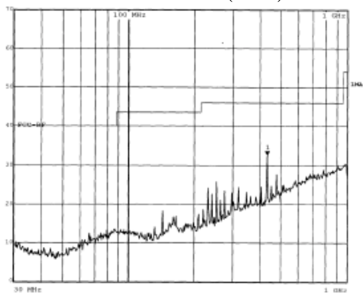
Bi-direction transmission (Vertical)
