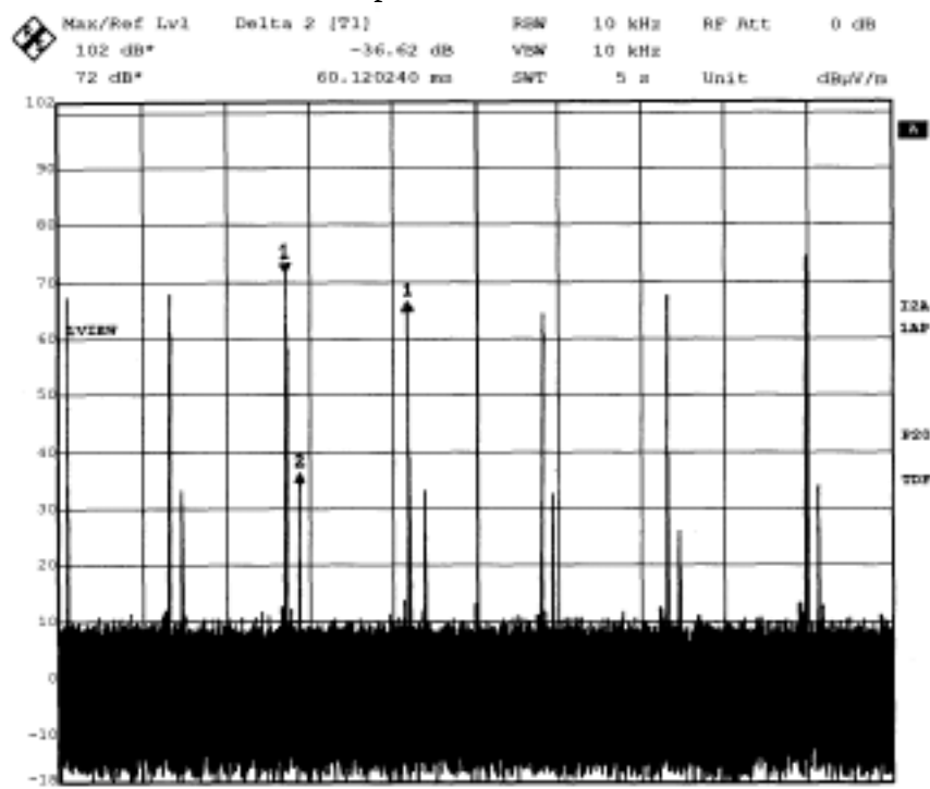
Graph A: Pulse Train
