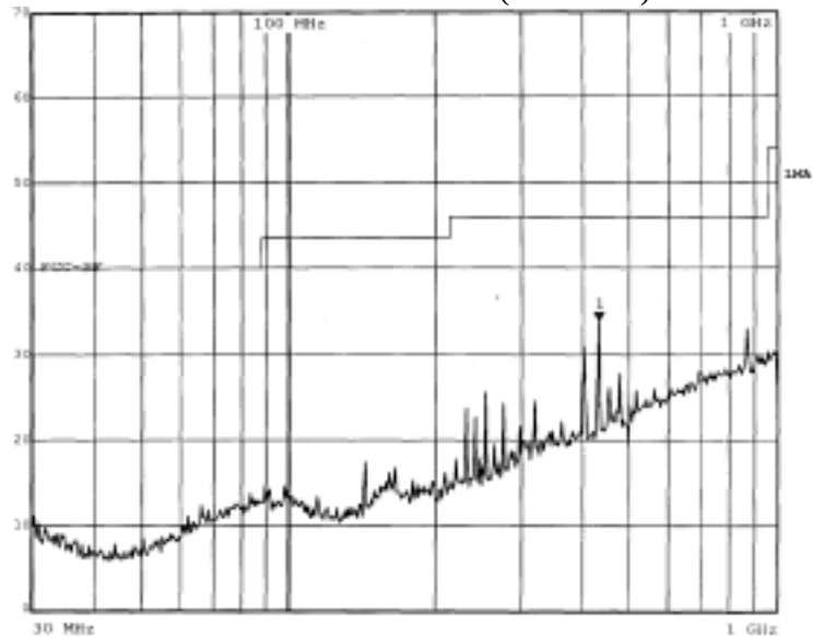
Bi-direction transmission (Horizontal)
