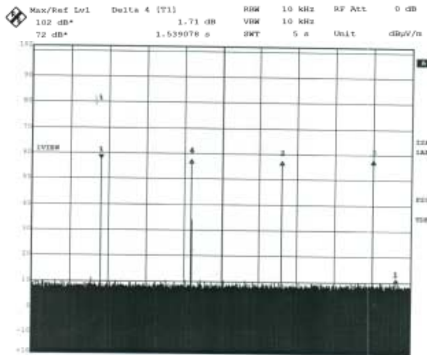
Graph A: Pulse Train (worst case)
