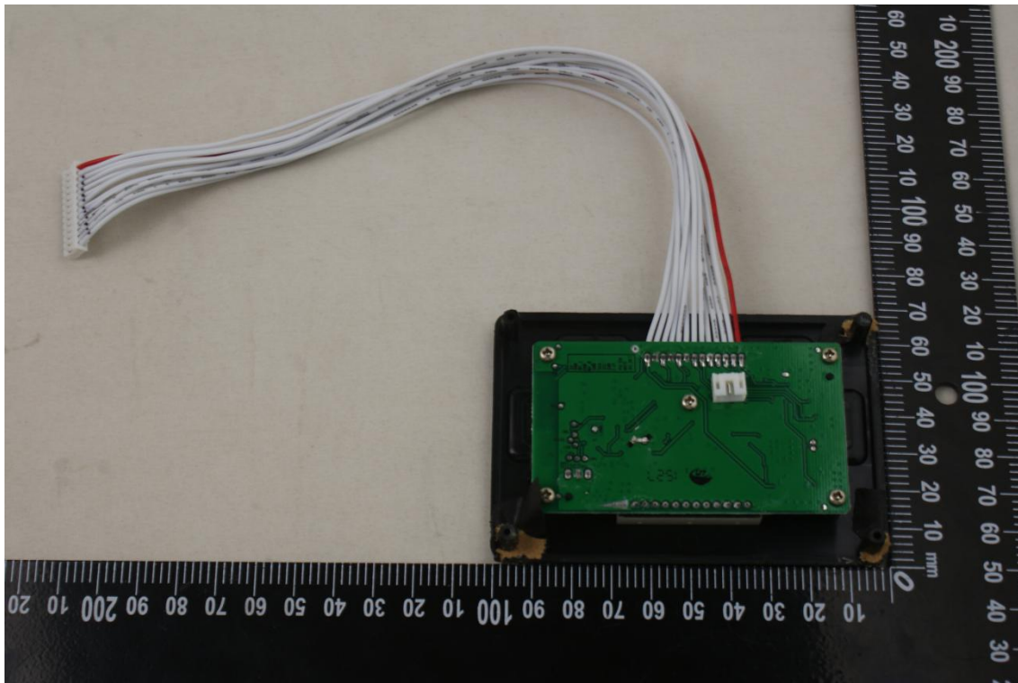
MAIN BOARD UNCOVER VIEW 2
