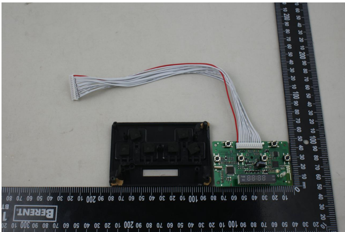
MAIN BOARD UNCOVER VIEW 3
