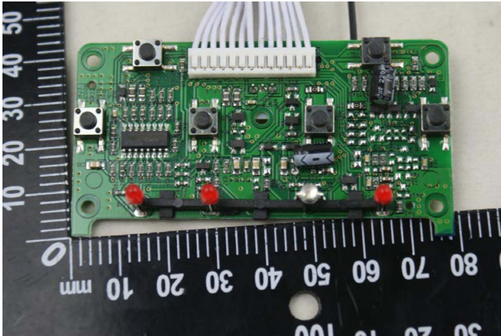
MAIN BOARD BACK TOP 2
