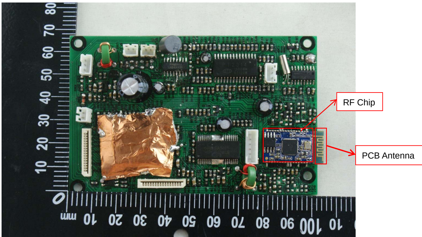
MAIN BOARD TOP VIEW 1
