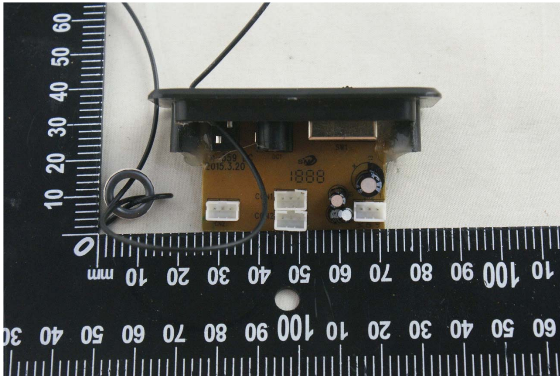
MAIN BOARD TOP VIEW 7
