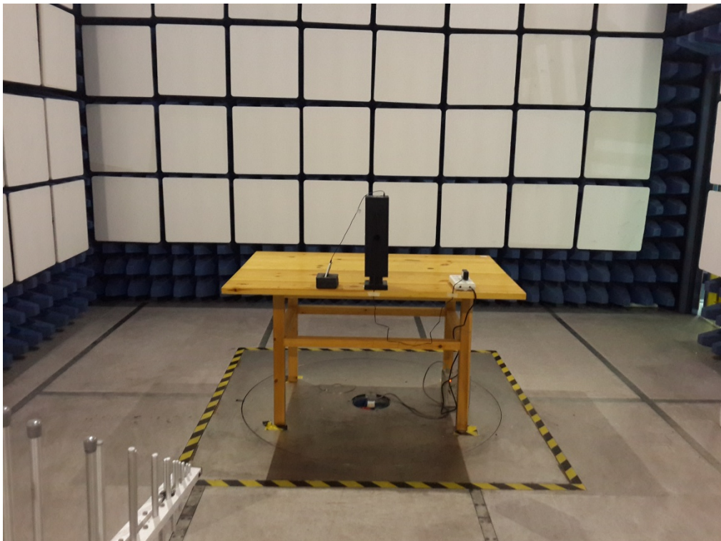
30 MHz-1 GHz (Audio Test Mode Photo)
