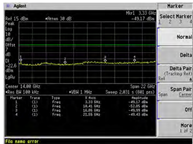
GFSK Hopping Mode, SPURIOUS 30 3GHz ~ 25 GHz
