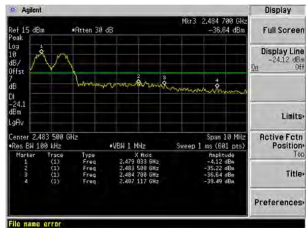
GFSK Hopping BAND EDGE (HIGH)
