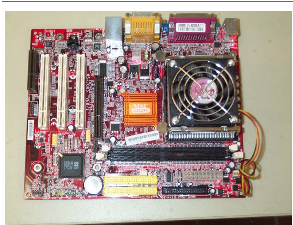
Picture 8. Mainboard, Top side
