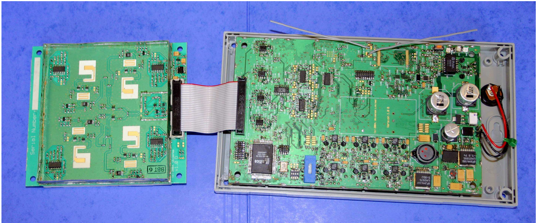
Photograph showing internal circuitry (§15.249 transceiver and Class A digital device)
