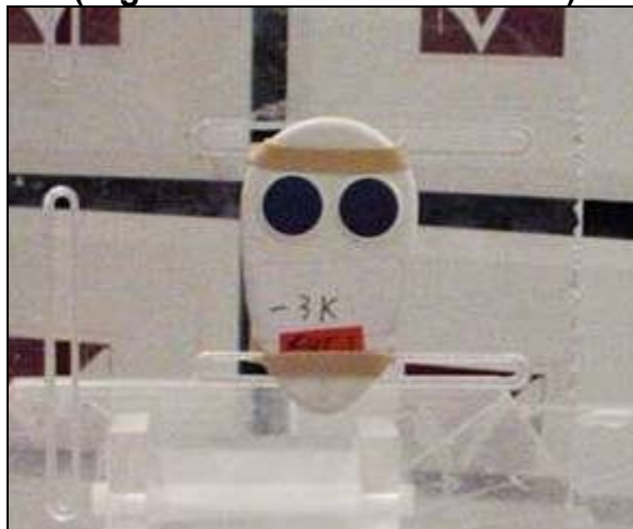
View of the EUT setup in vertical orientation (Highest emissions measured)
