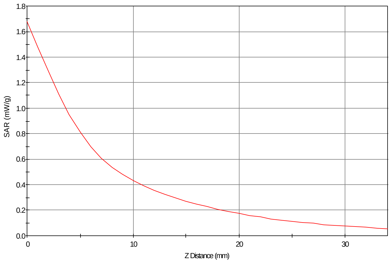
SAR - Z Axis at Hotspot x:9.0 y:41.0
