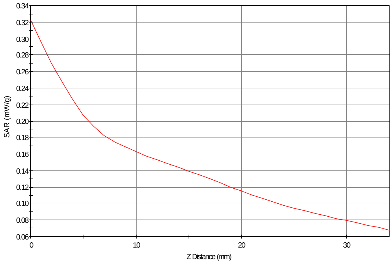
SAR - Z Axis at Hotspot x:28.0 y:43.0
