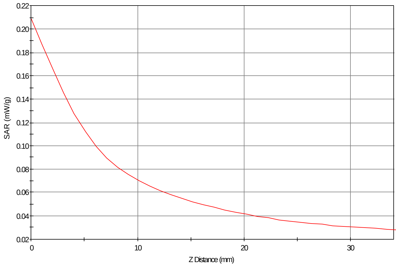
SAR - Z Axis at Hotspot x:25.0 y:43.0
