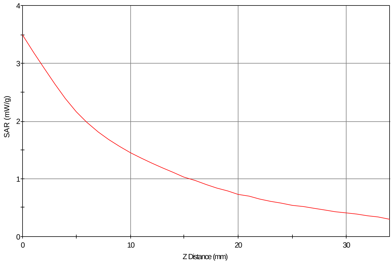
SAR - Z Axis at Hotspot x:-10.0 y:-2.0
