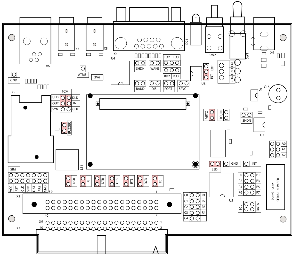
Figure 14.3 Developer's board overlay
