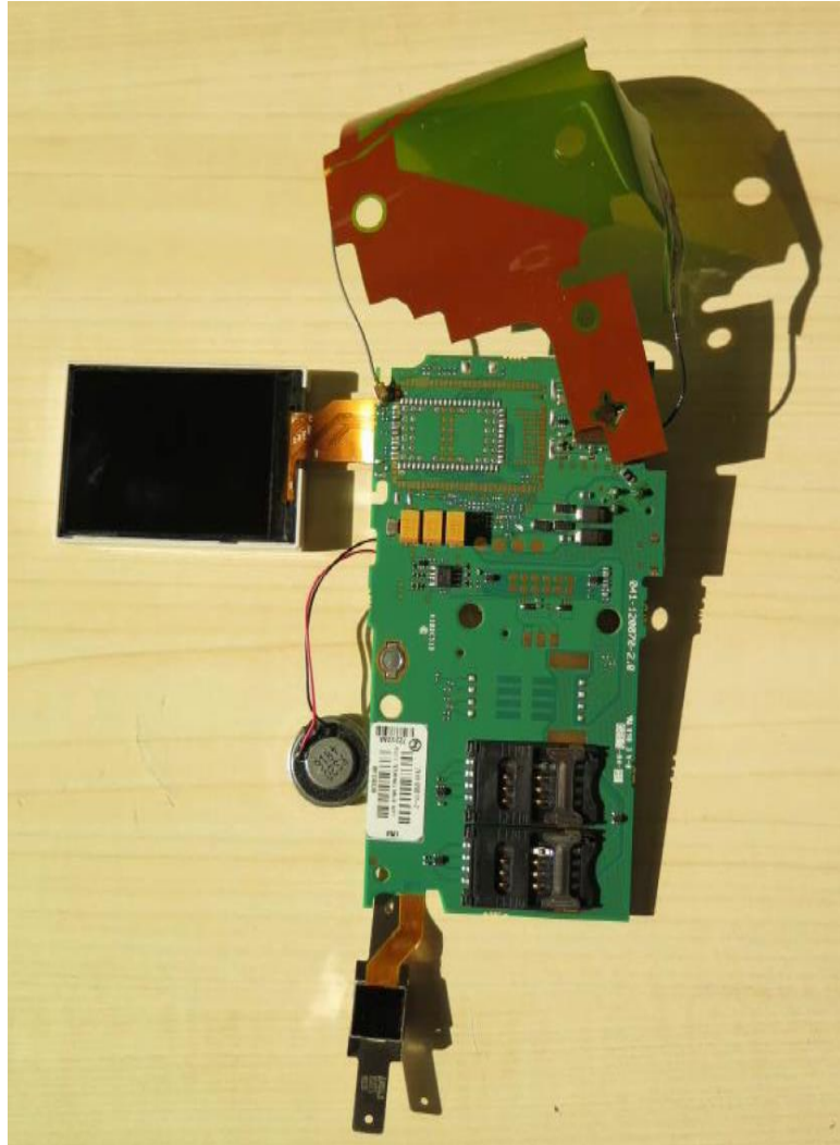
Photo 4: Main PCB 041-120070-xx back side view
