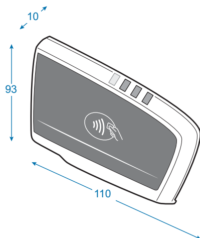
Figure 20. Contactless reader dimensions
