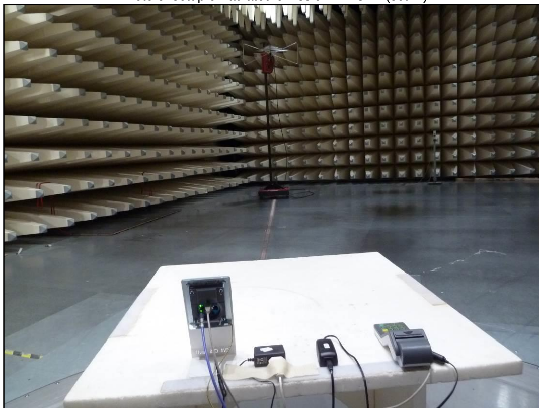
Photo 4: setup of radiated emission < 1 GHz (set. 2)
