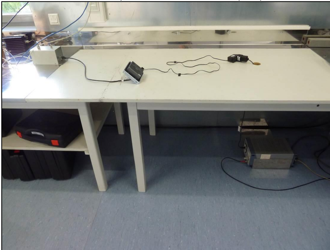
Photo 1: setup of conducted emission on AC (set. 1)
