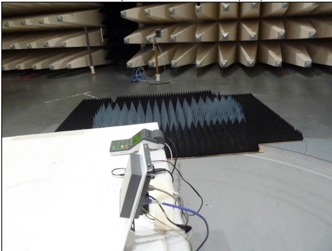
Photo 6: setup of radiated emission > 1 GHz (set. 2)
