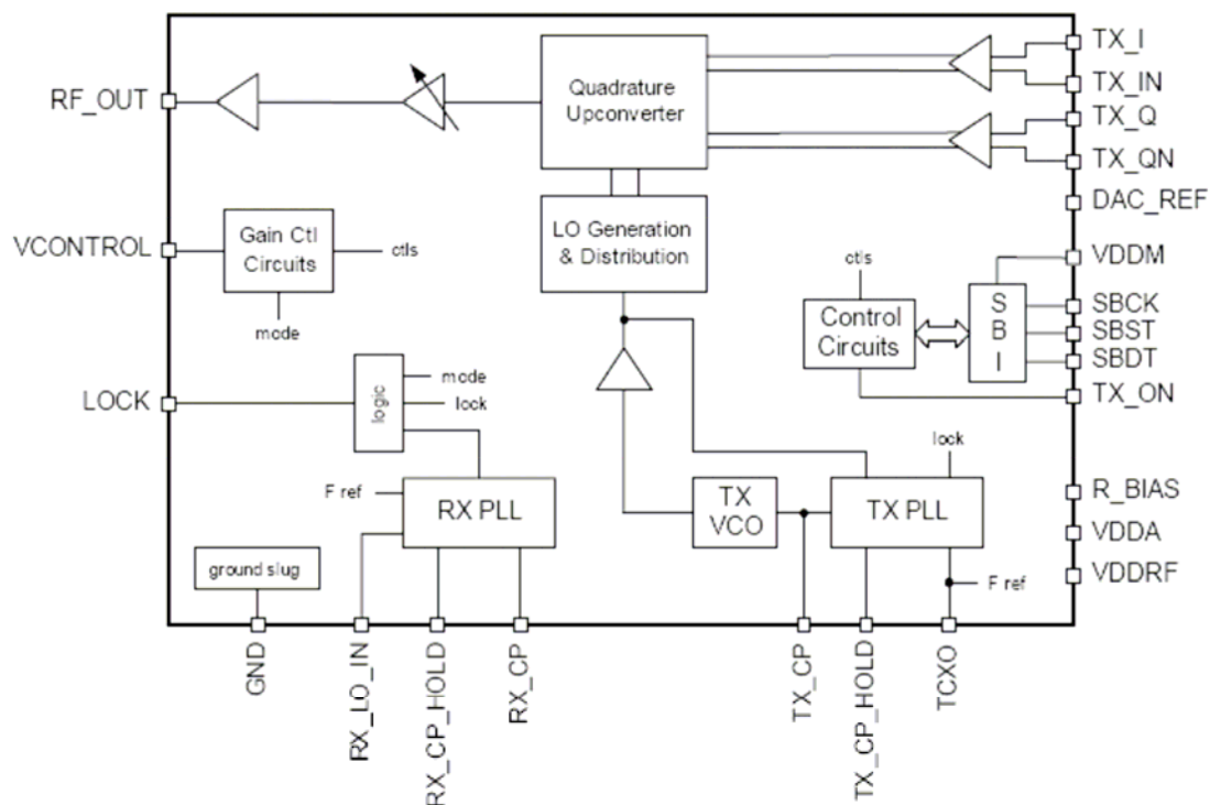
FIG.3-2 RFT6122 IC FUNCTIONAL BLOCK DIAGRAM
