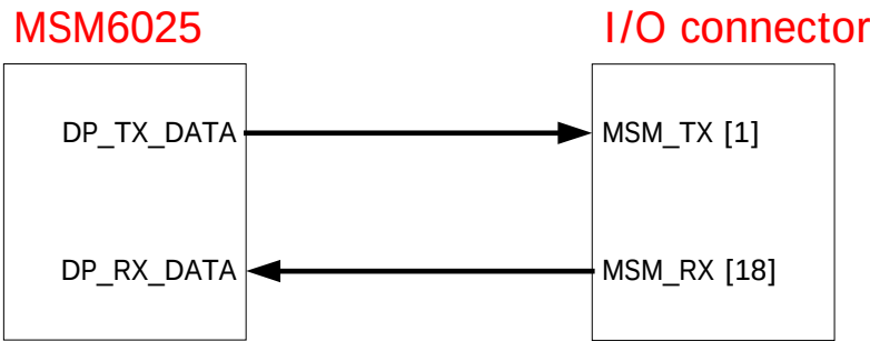
FIG.4-7 UART BLOCK DIAGRAM
