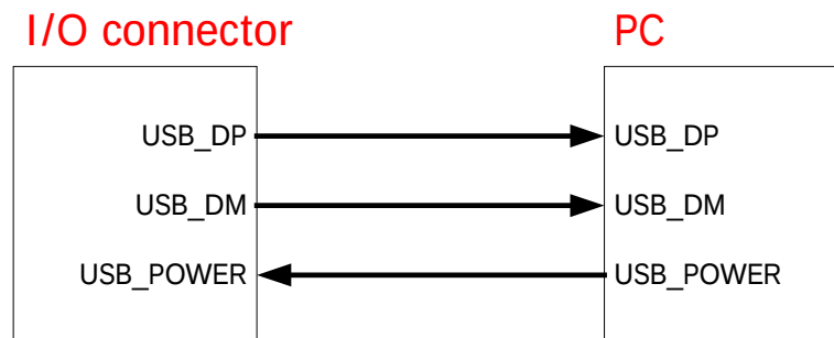
FIG.4-6 USB DATA CABLE PIN MAP
