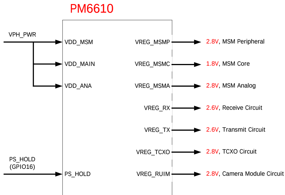
FIG.3-3 PM6610 OUTPUT VOLTAGE
