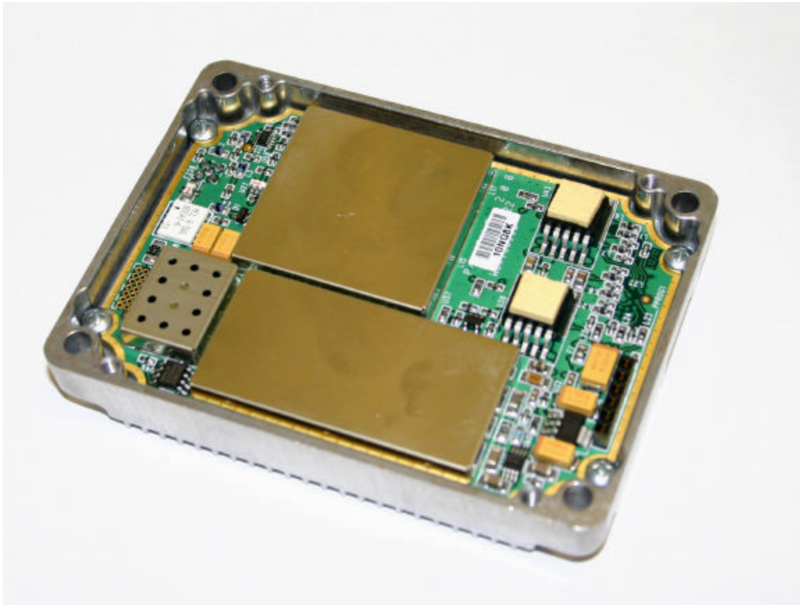
MP9311 Internal Photos – Top Side with Shield Cans
