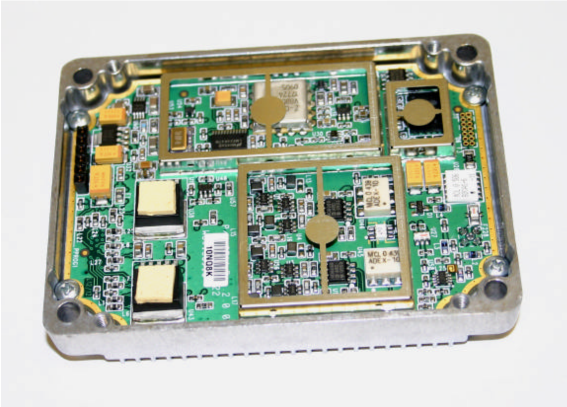
Top Side – Without Shield Cans (Shield fencing in place)
