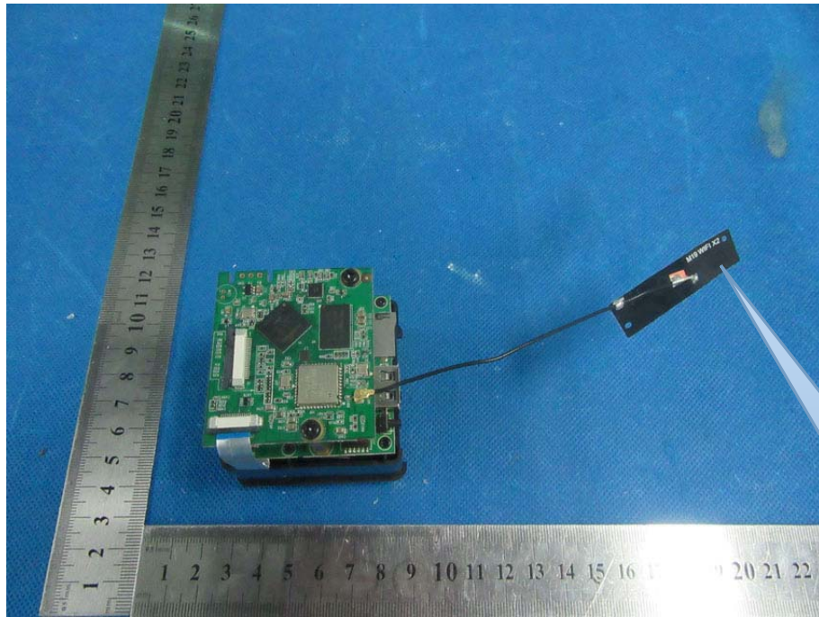
2.4G/5G WIFI Antenna location
