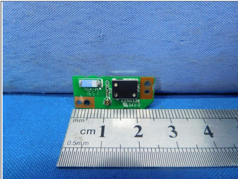
EUT with antenna (RFANT5220110A0T)
